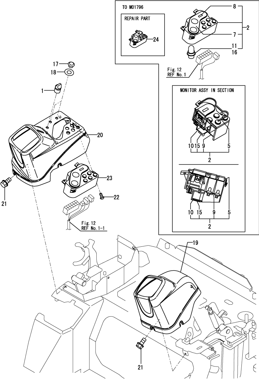
Fig.37. INSTRUMENT PANEL
