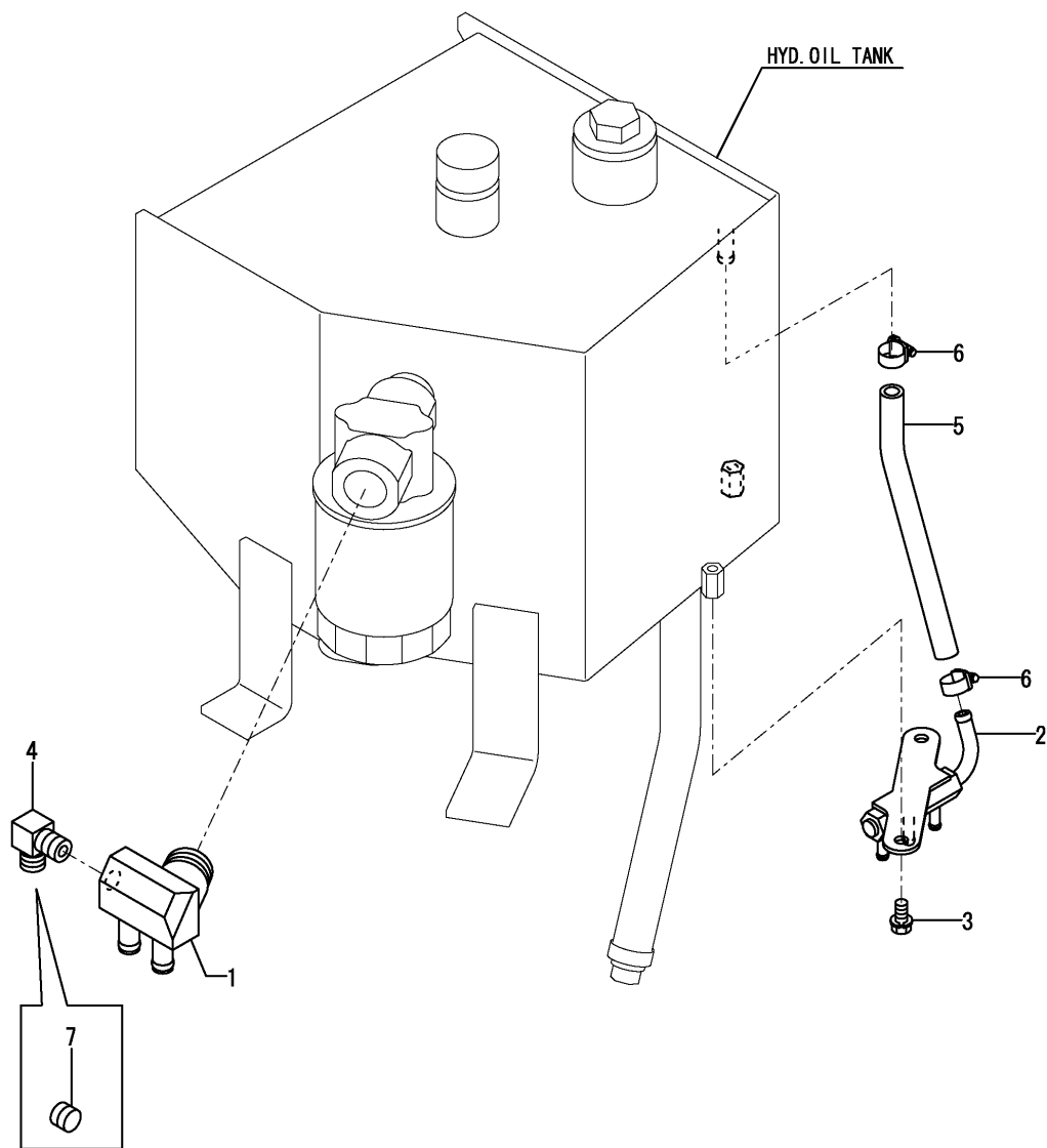
Fig.69. HYD.OIL PIPING(RESERVOIR)
