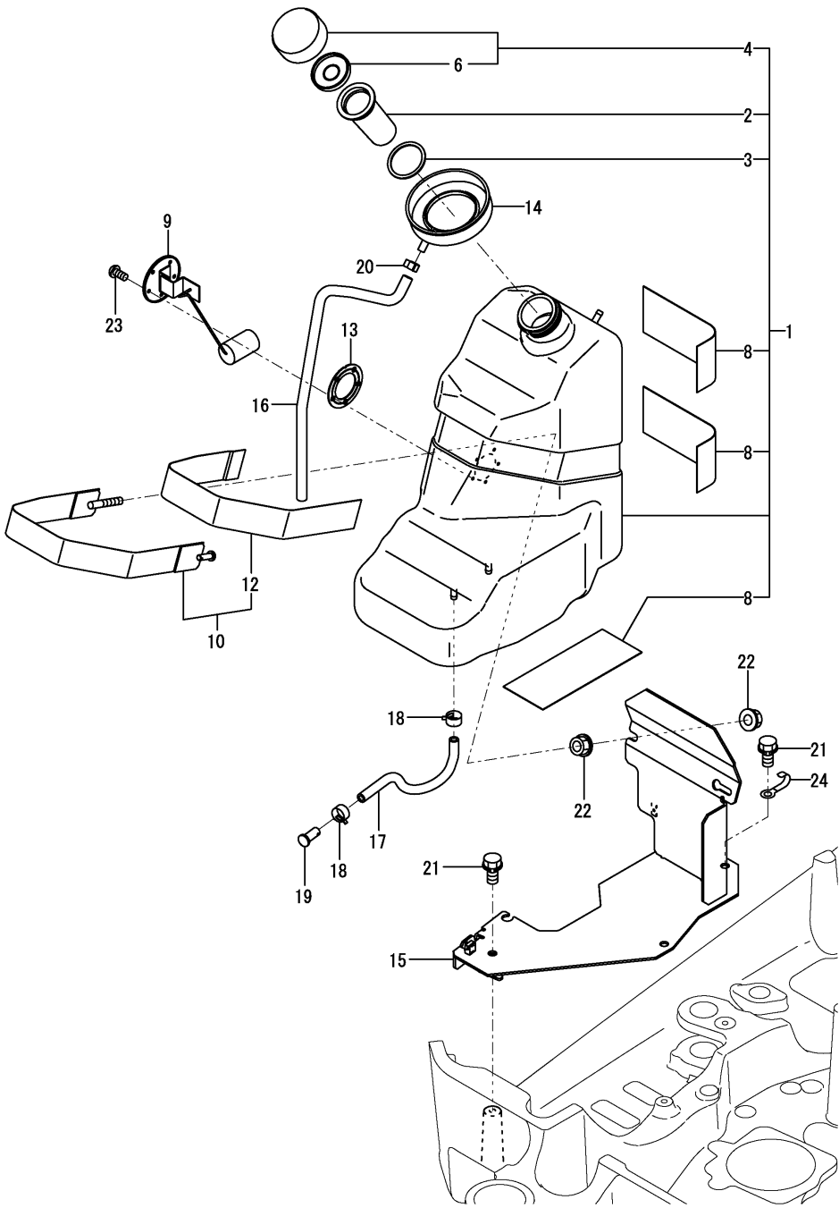
Fig.8. FUEL TANK
