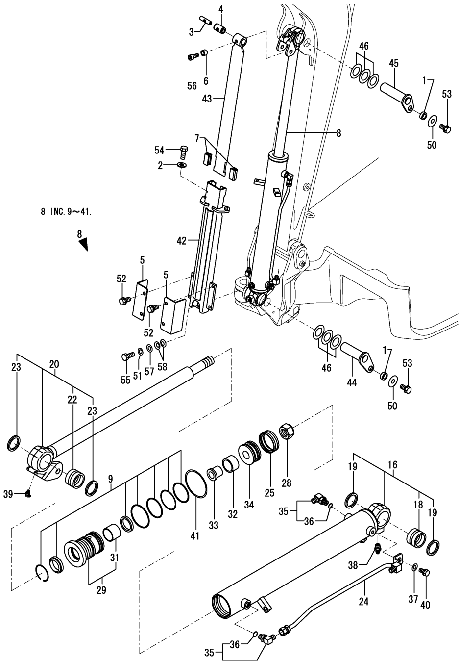
Fig.43. BOOM CYLINDER
