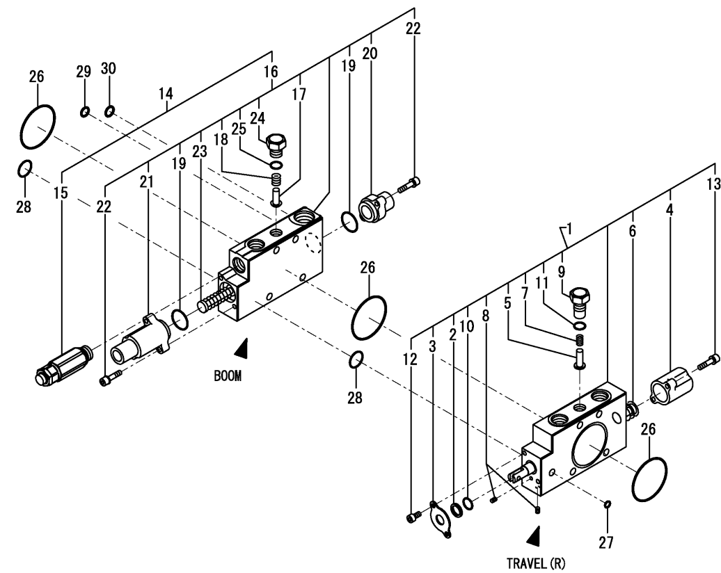
Fig.53. CONTROL VALVE(2/7)
