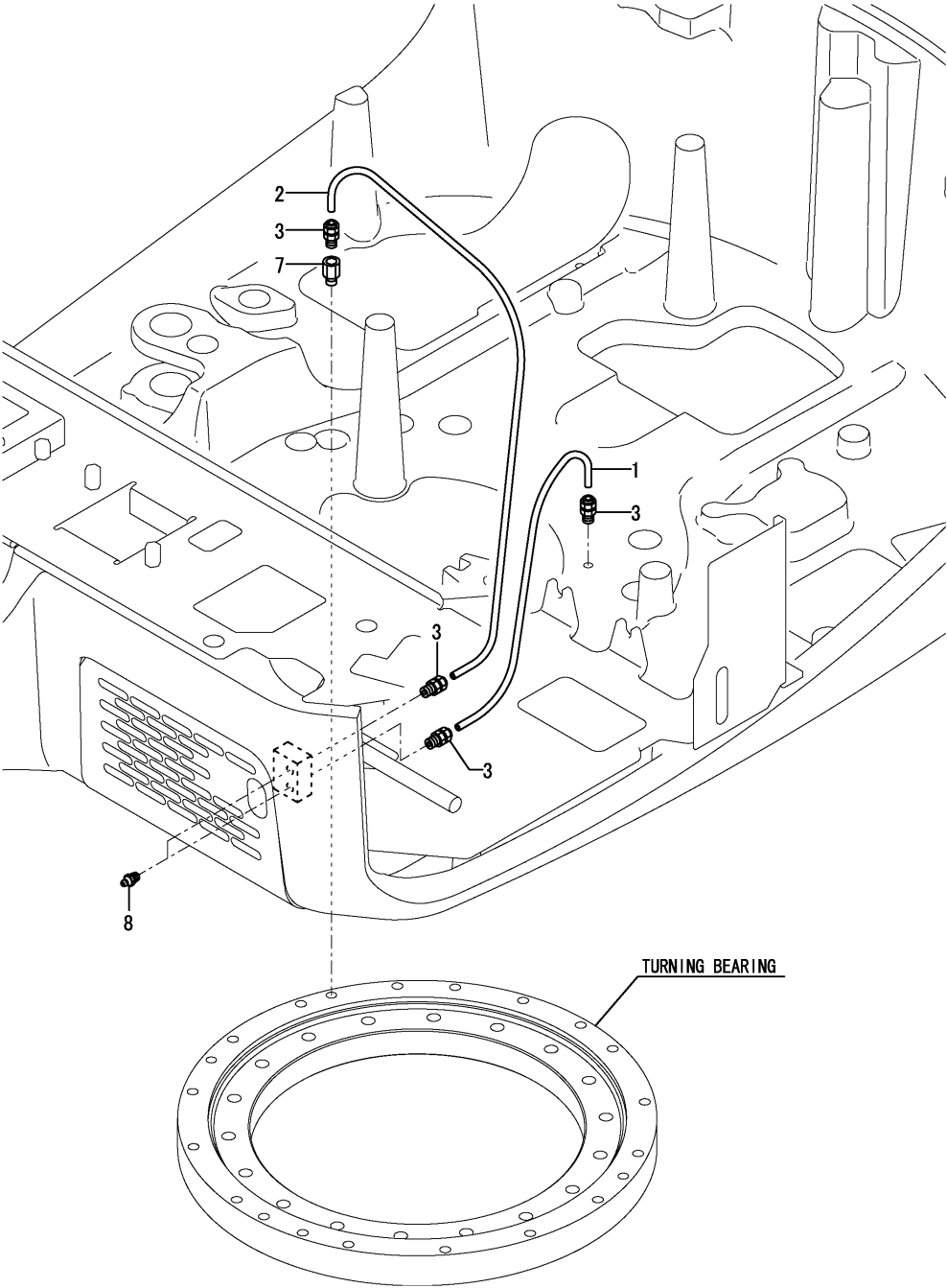
Fig.75. GREASING
