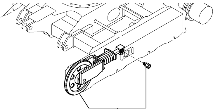
Fig.17. IDLER & ADJUST
