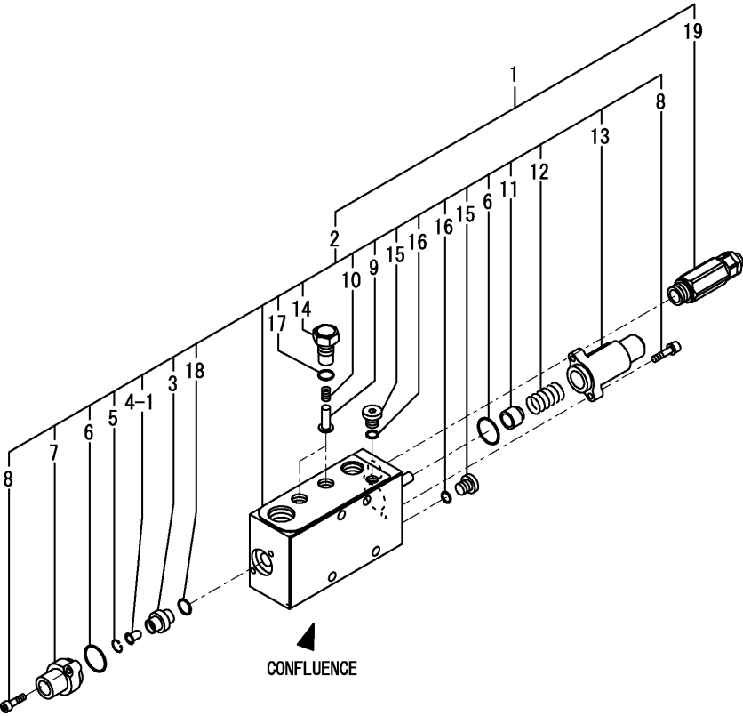
Fig.57. CONTROL VALVE(6/7)
