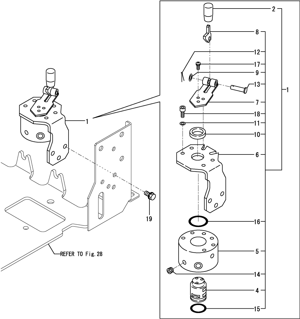
Fig.59. 2-WAY VALVE
