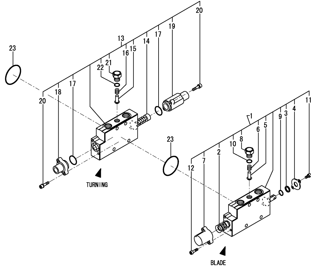
Fig.58. CONTROL VALVE(7/7)
