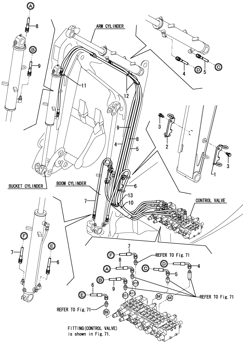
Fig.66. HYD.OIL PIPING(IMP)
