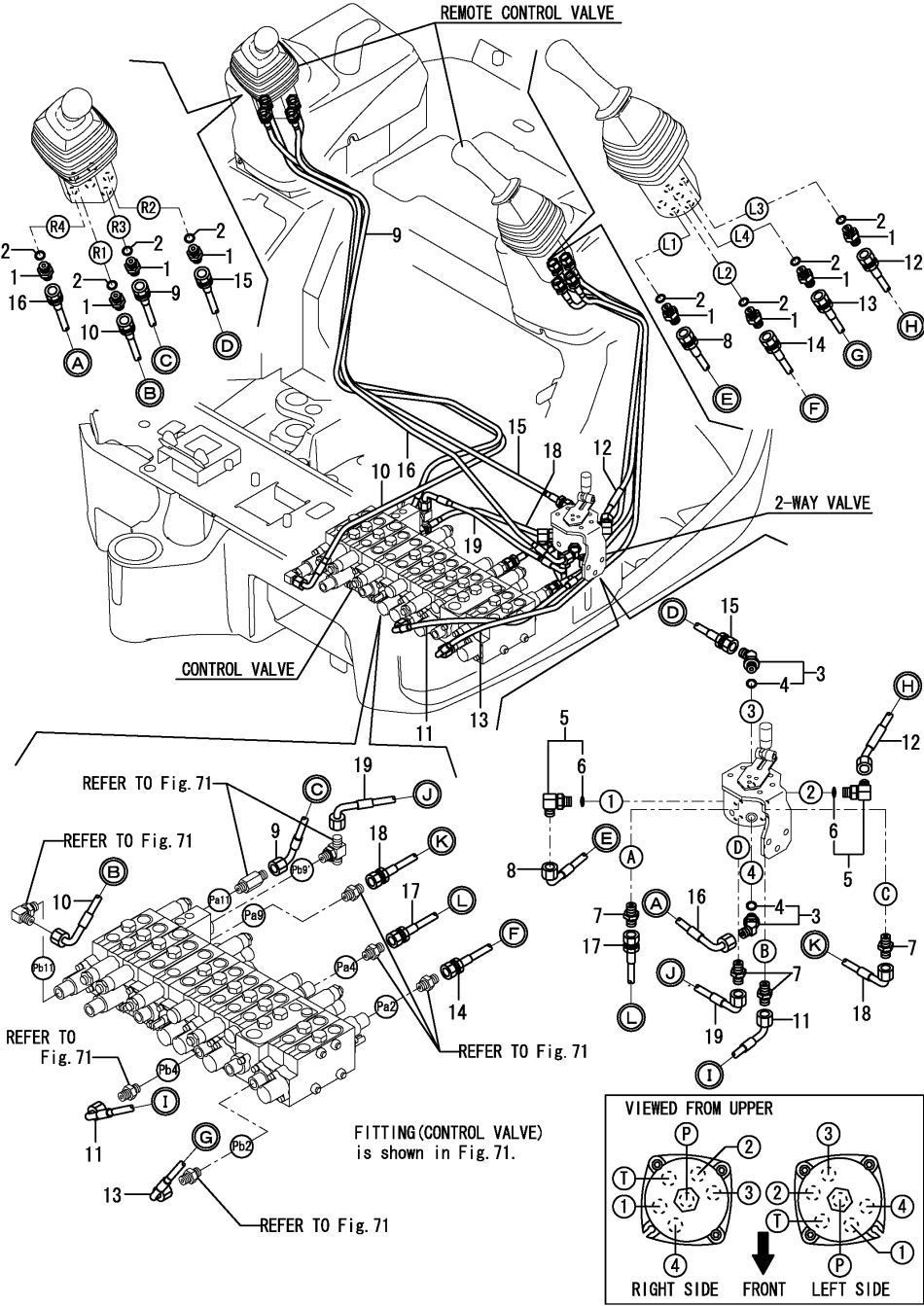
Fig.74. CONTROL PIPING(2 : 2-WAY SPEC.)
