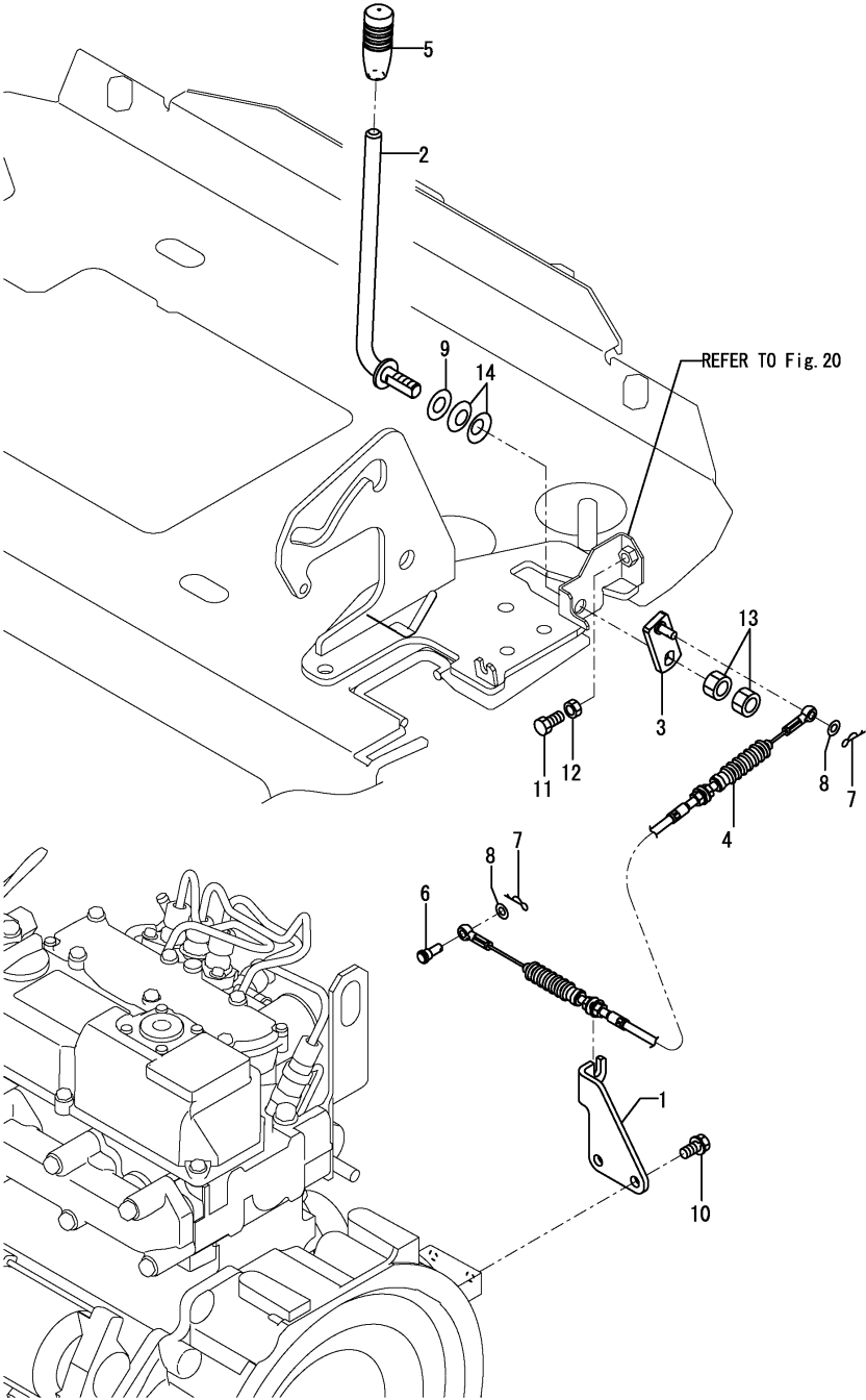
Fig.5. ACCELERATOR LEVER
