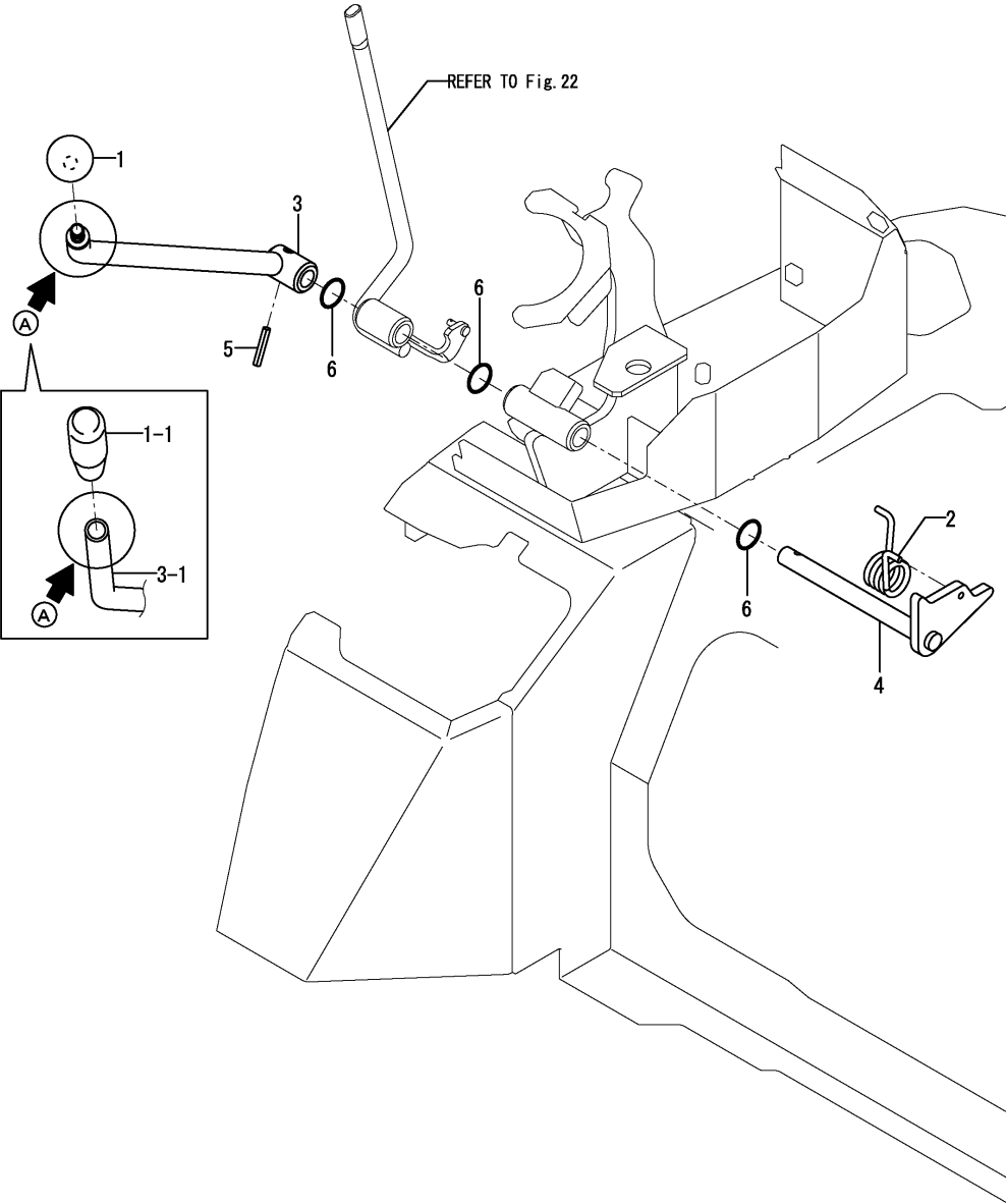
Fig.19. CONTROL EQUIPMENT(LOCK LEVER & STAND)(RIGHT)
