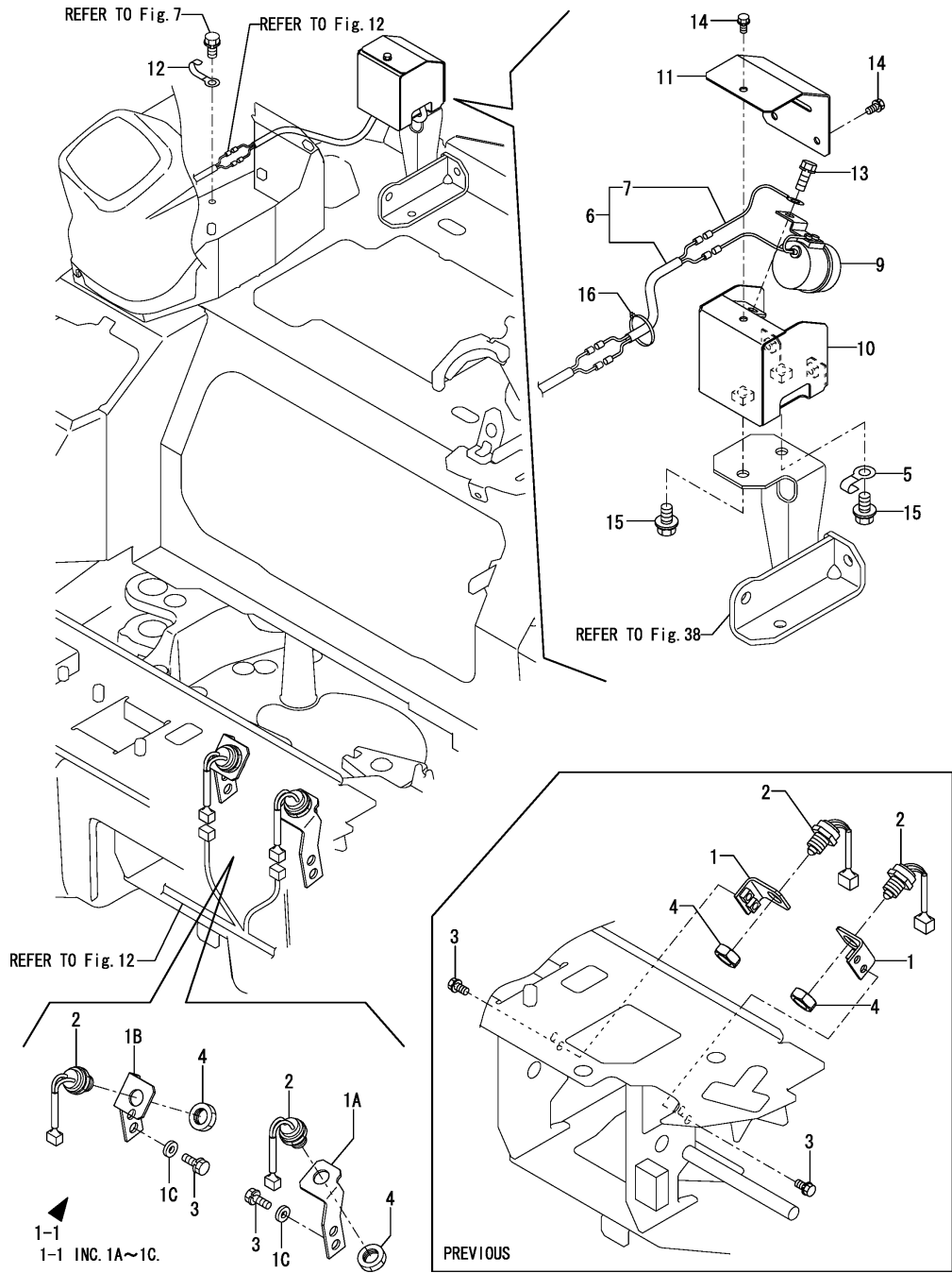
Fig.14. TRAVEL ALARM
