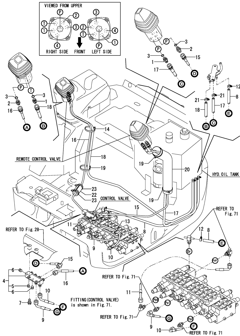
Fig.73. CONTROL PIPING(1)
