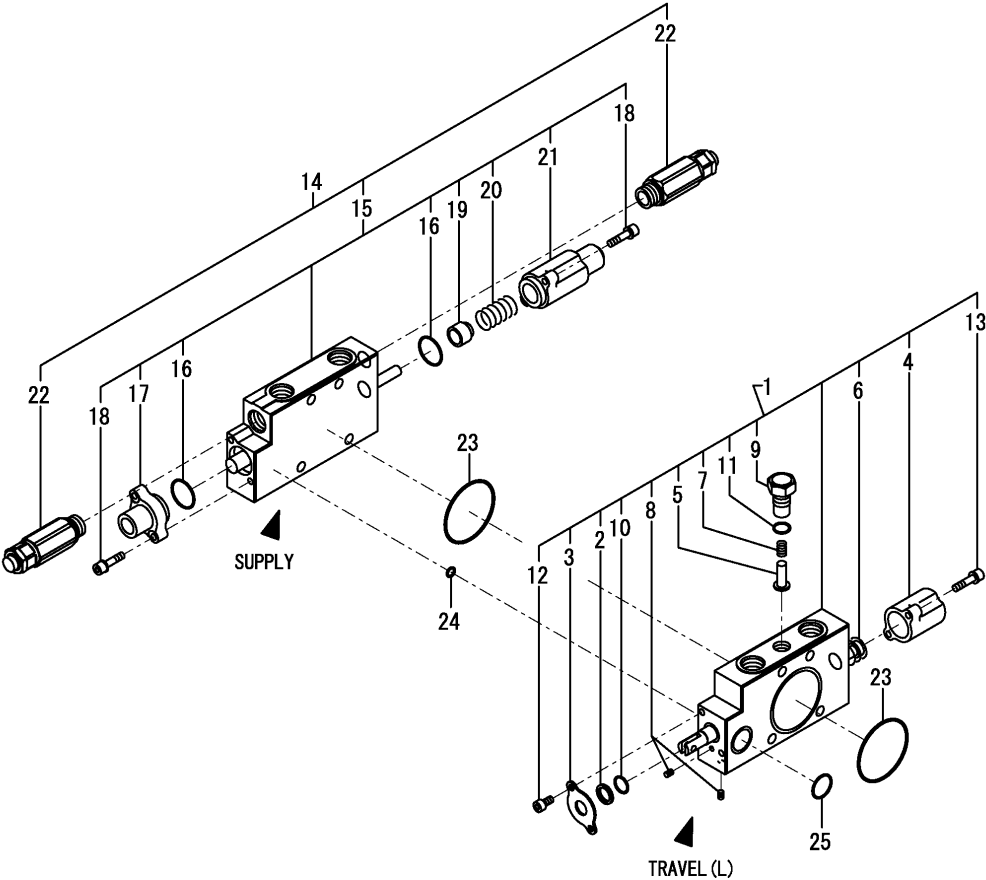
Fig.54. CONTROL VALVE(3/7)
