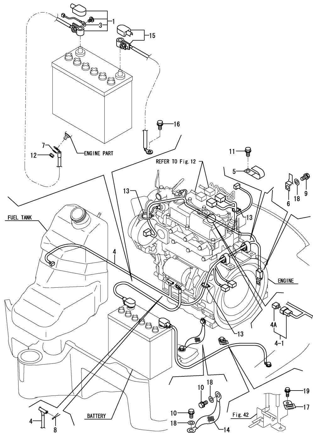
Fig.11. ELECTRIC PART(ENGINE)
