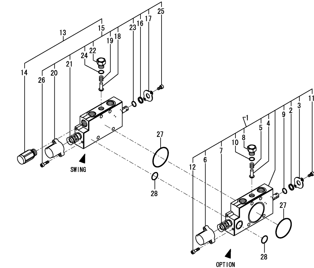
Fig.55. CONTROL VALVE(4/7)
