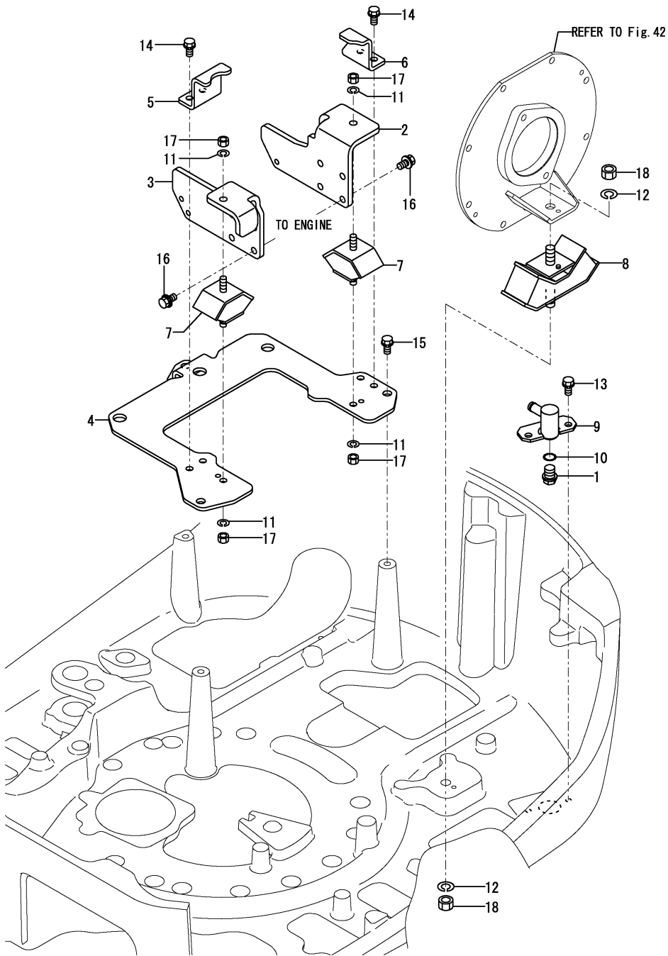
Fig.6. ENGINE MOUNT
