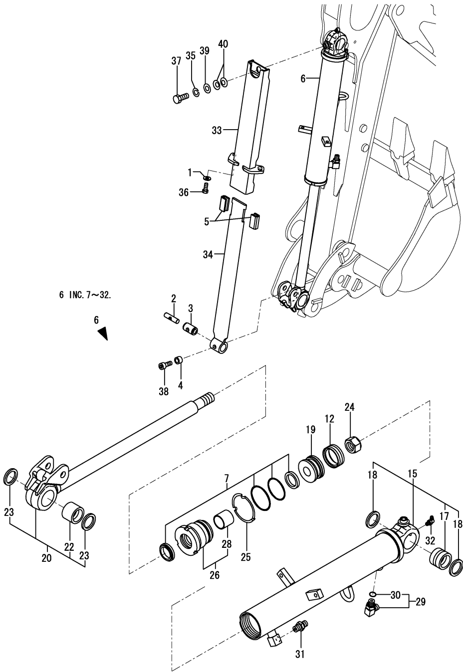
Fig.45. BUCKET CYLINDER
