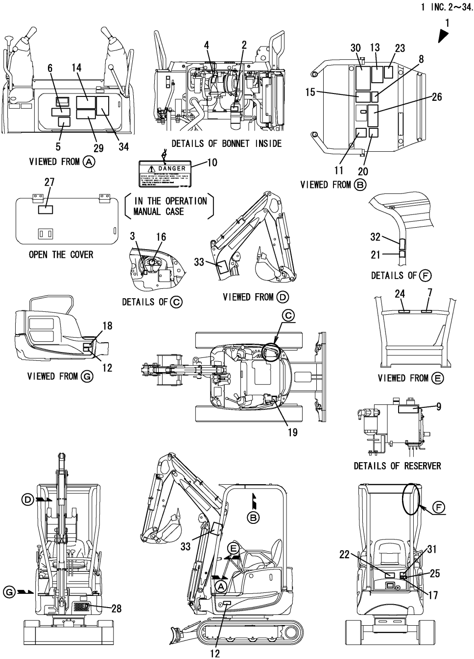
Fig.88. CA LABEL KIT(OPTIONAL)
