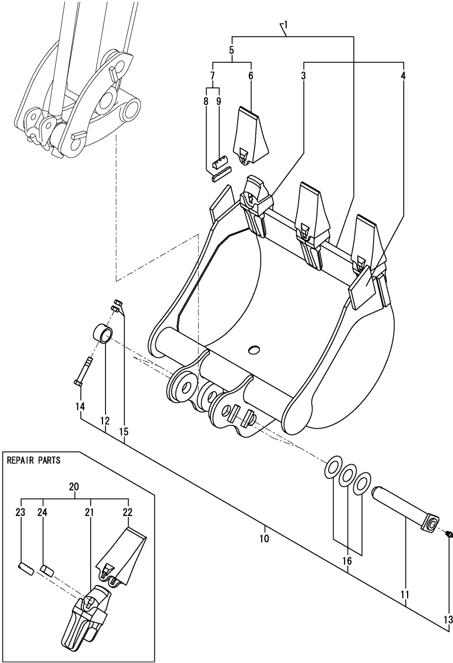
OCS10-G49500 Fig.80. BUCKET
