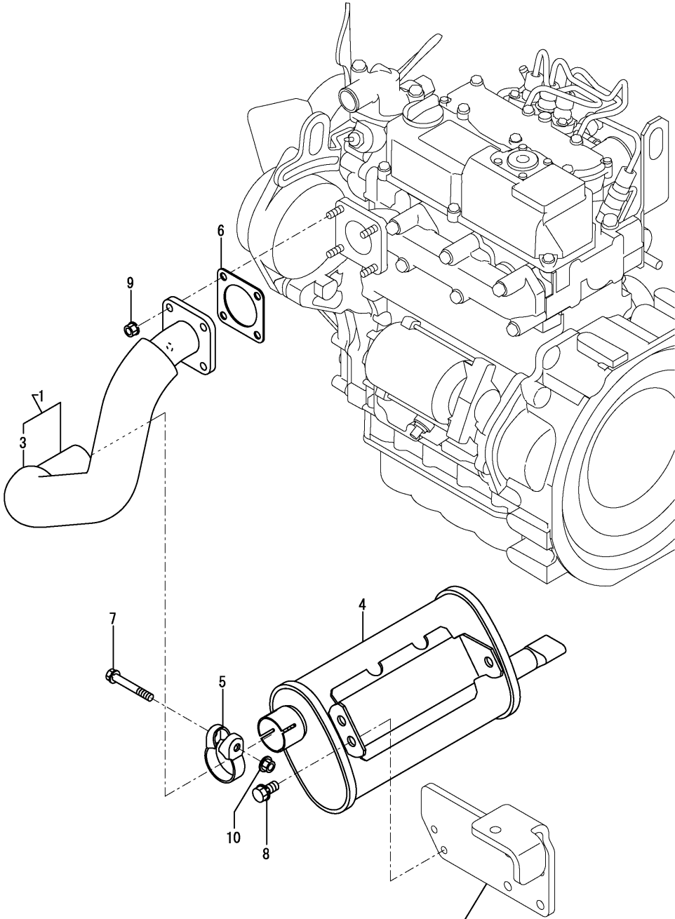
OCS10-G49500 Fig.3. SILENCER
