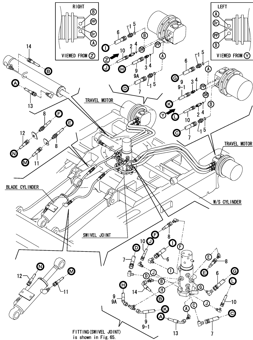
Fig.64. HYD.OIL PIPING(LOWER)
