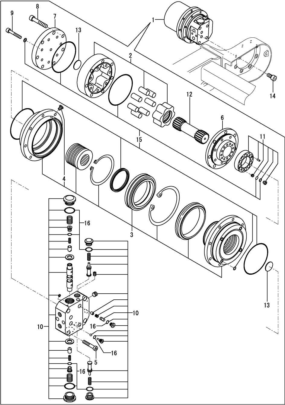
Fig.49. TRAVEL MOTOR
