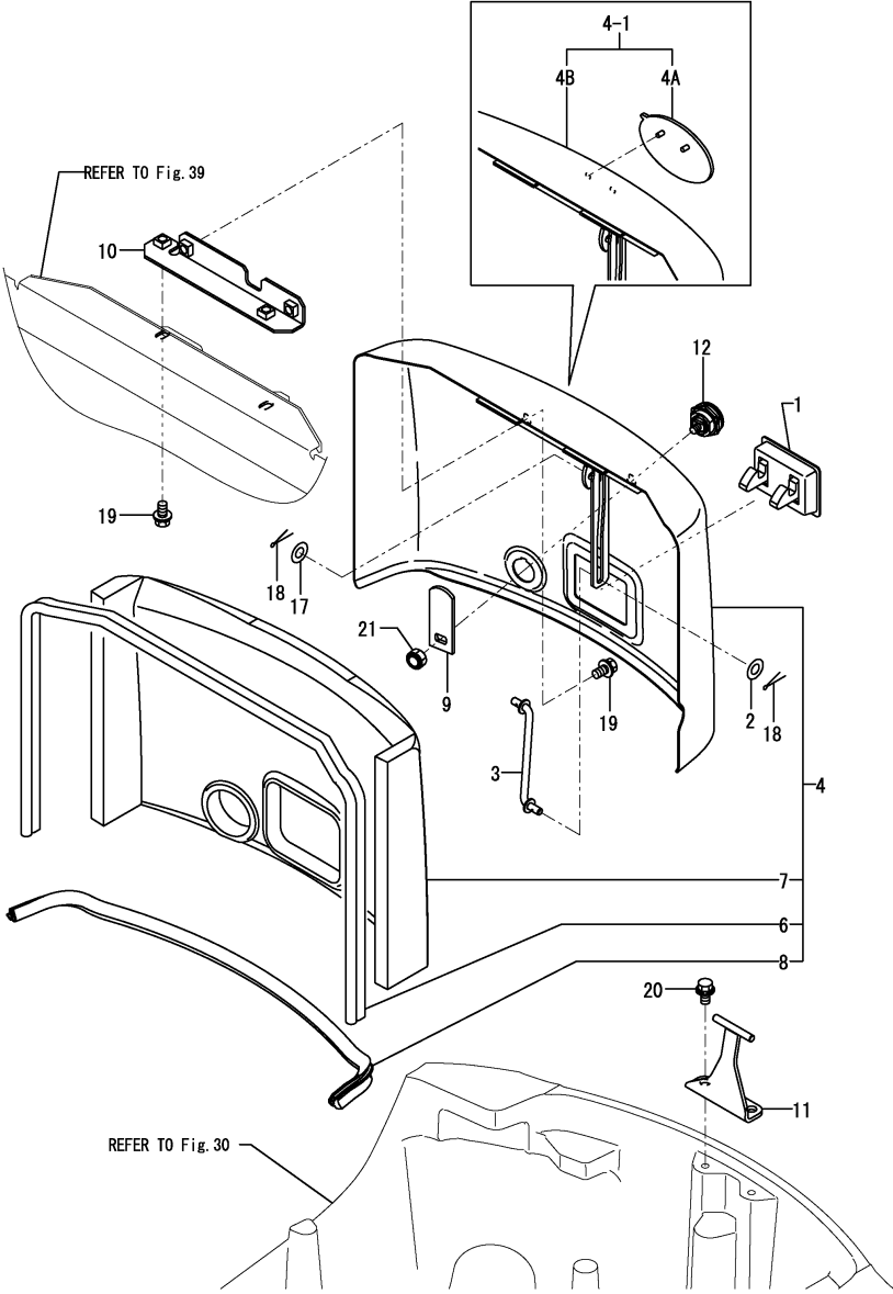
Fig.40. BONNET
