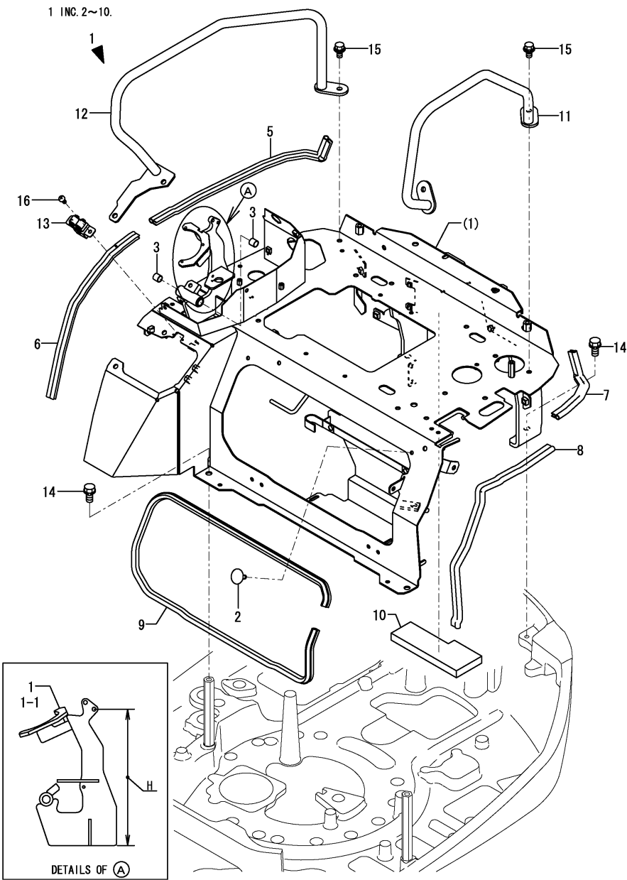
Fig.39. SEAT MOUNT
