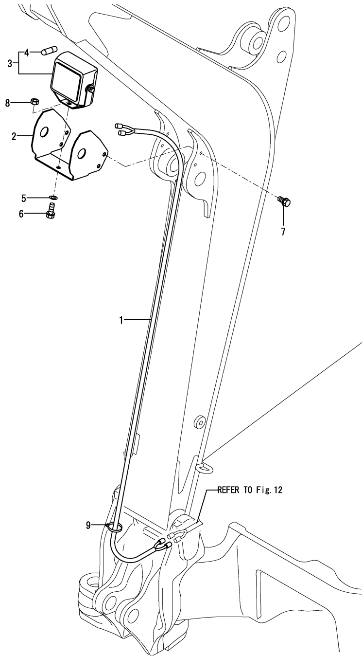
Fig.15. WORK LAMP
