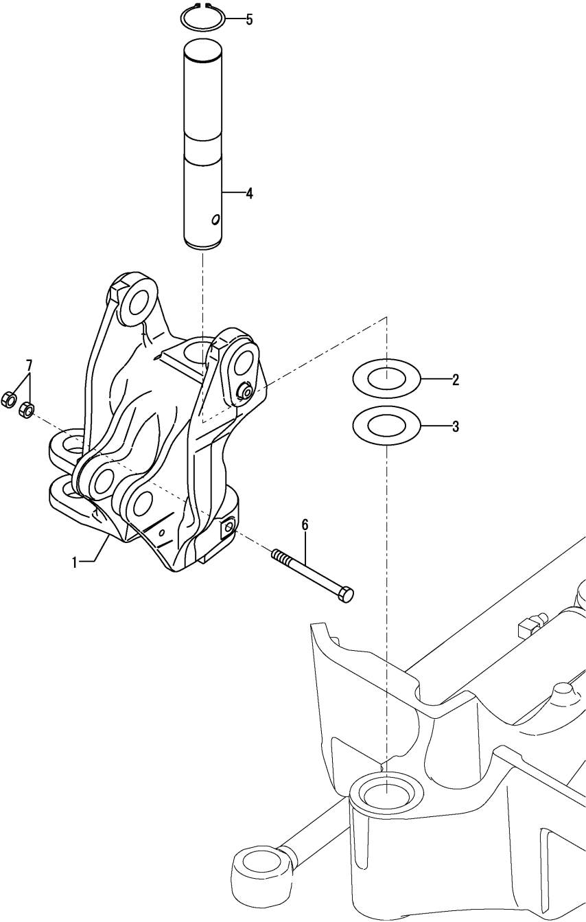
Fig.76. BOOM BRACKET
