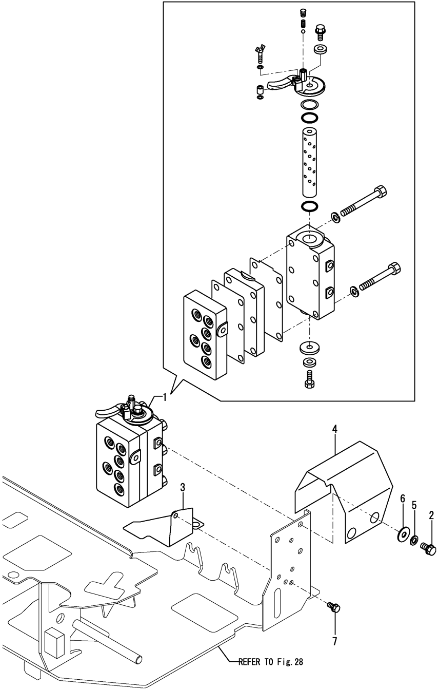
Fig.86. 4-WAY VALVE
