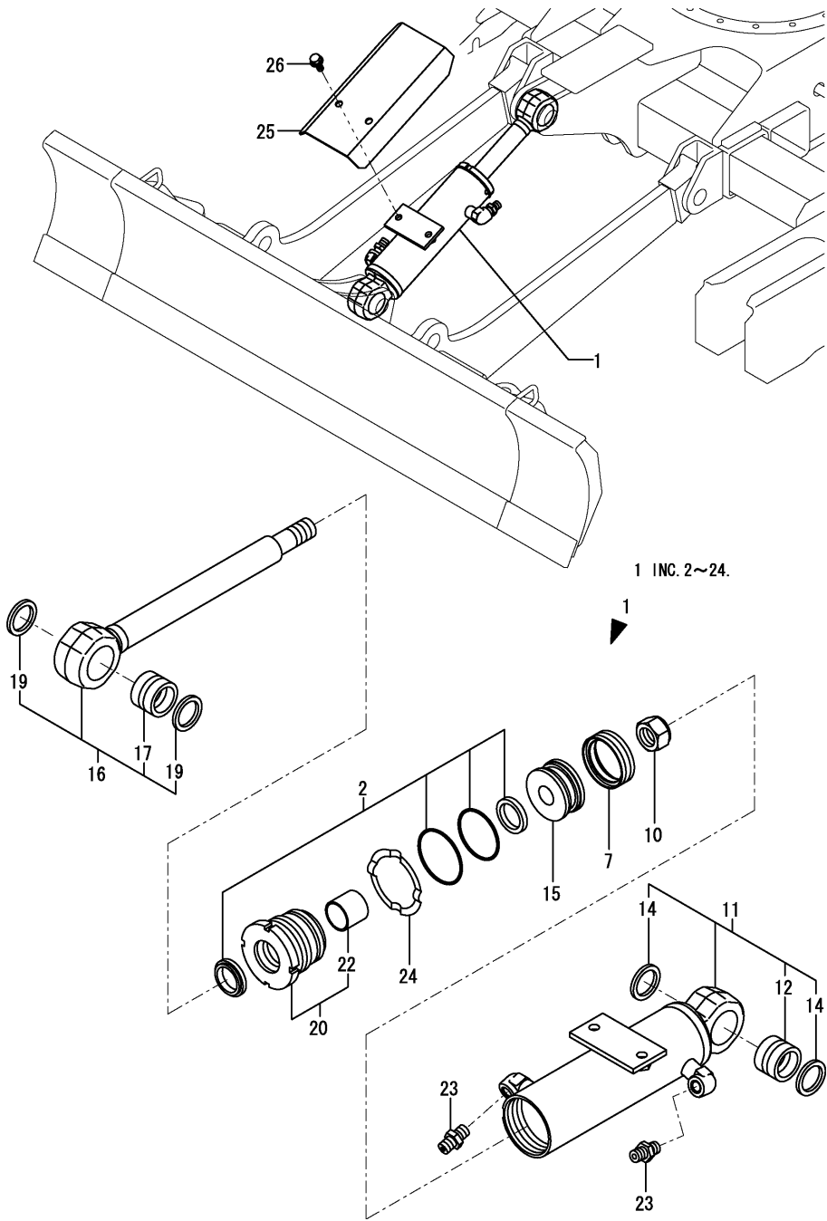
Fig.47. BLADE CYLINDER
