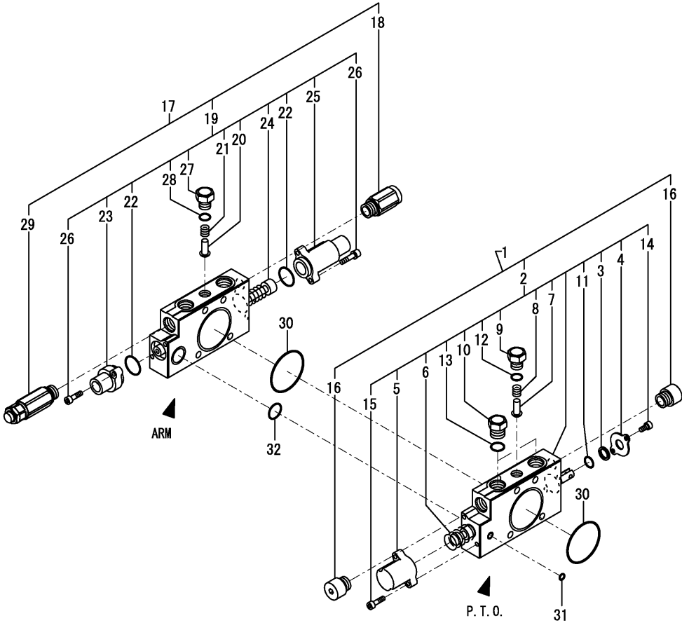
Fig.56. CONTROL VALVE(5/7)
