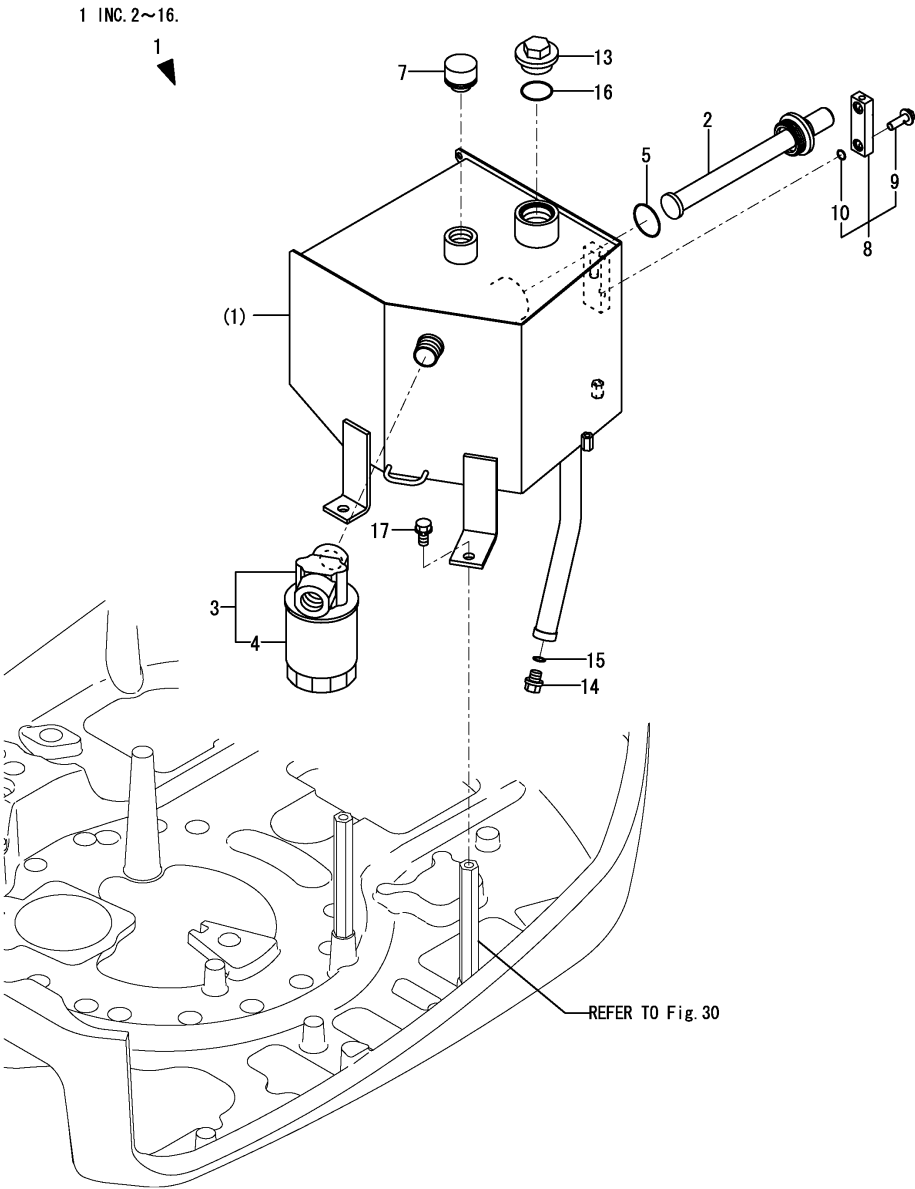
Fig.62. HYD.OIL TANK
