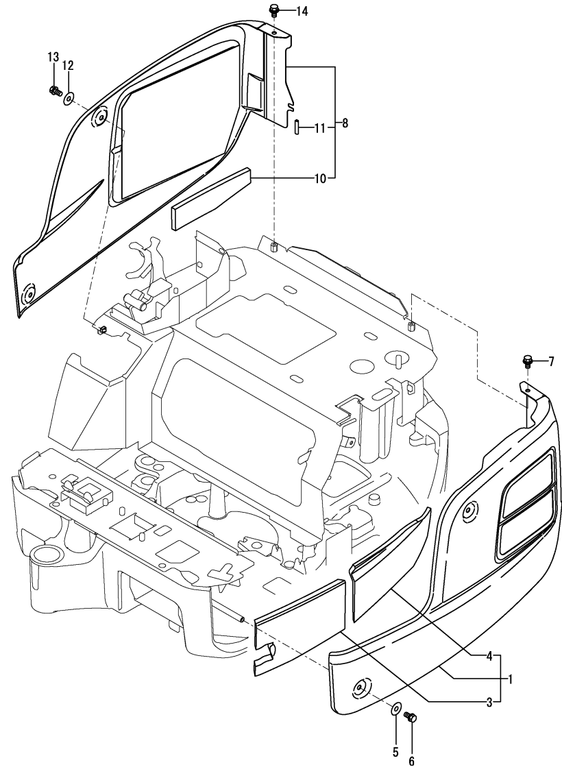
Fig.35. COVER(SIDE)
