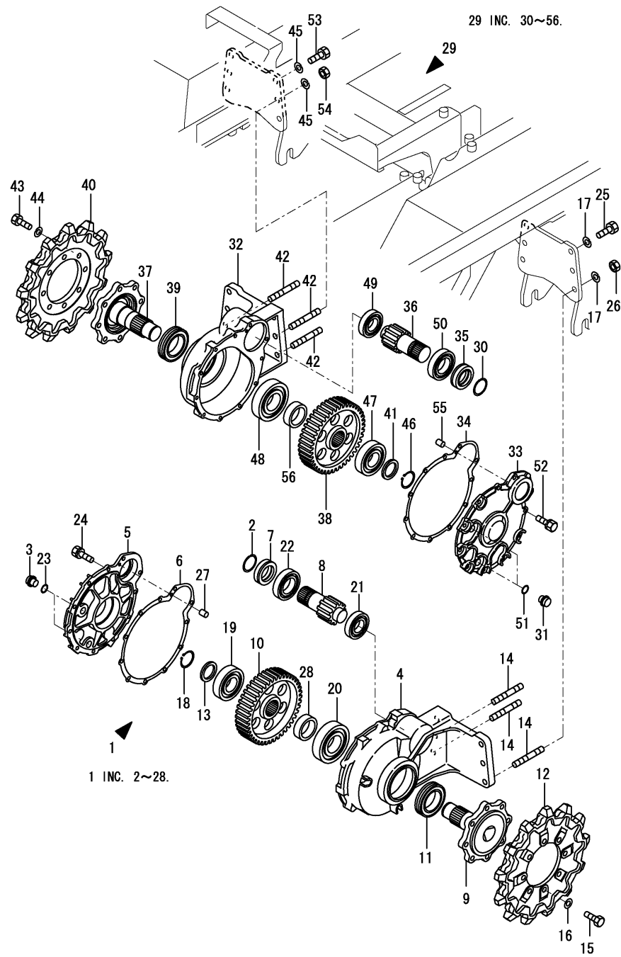
Fig.22. TRAVELLING WHEEL
