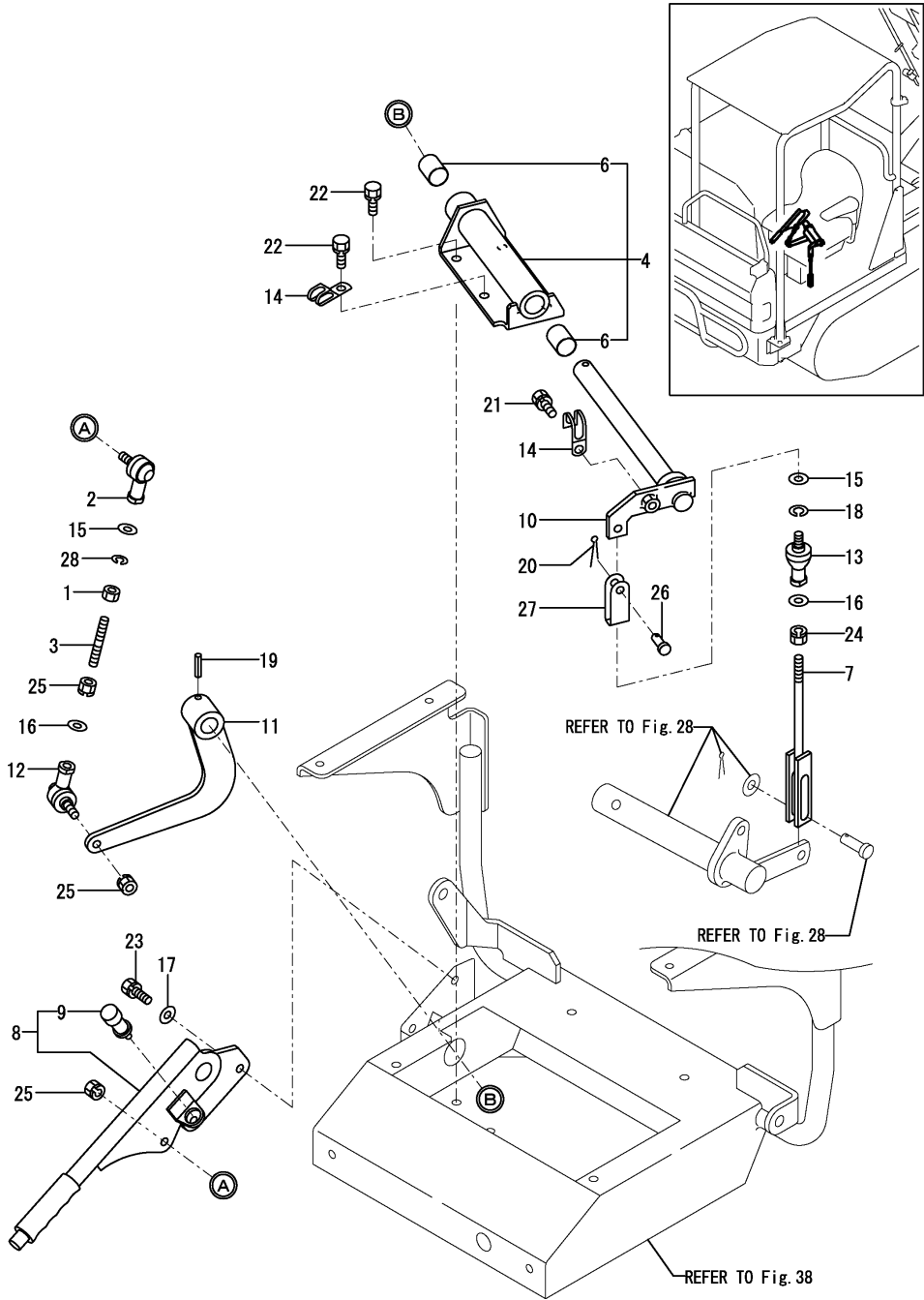
Fig.27. BRAKE(PARKING)
