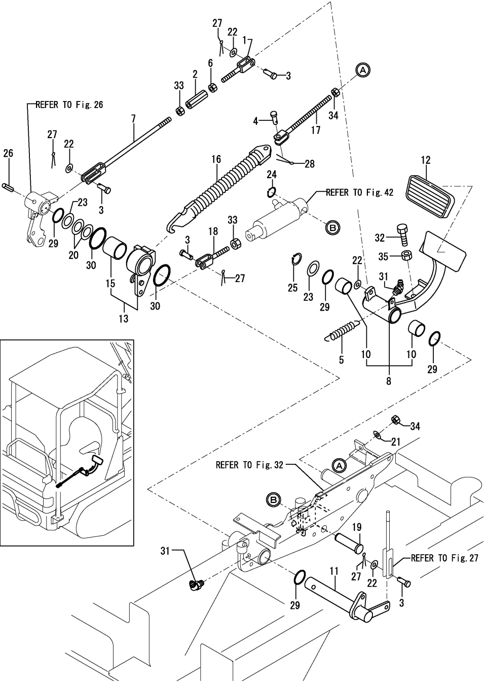
Fig.28. BRAKE(PEDAL & ROD)(REAR)
