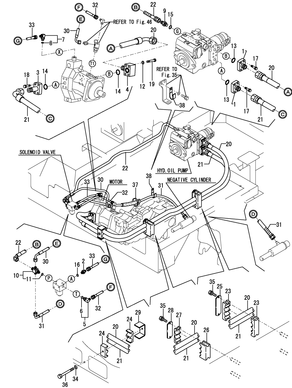
Fig.48. HYD.OIL PIPING(PUMP - TRAVEL MOTOR - NEGATIVE CYLINDER)
