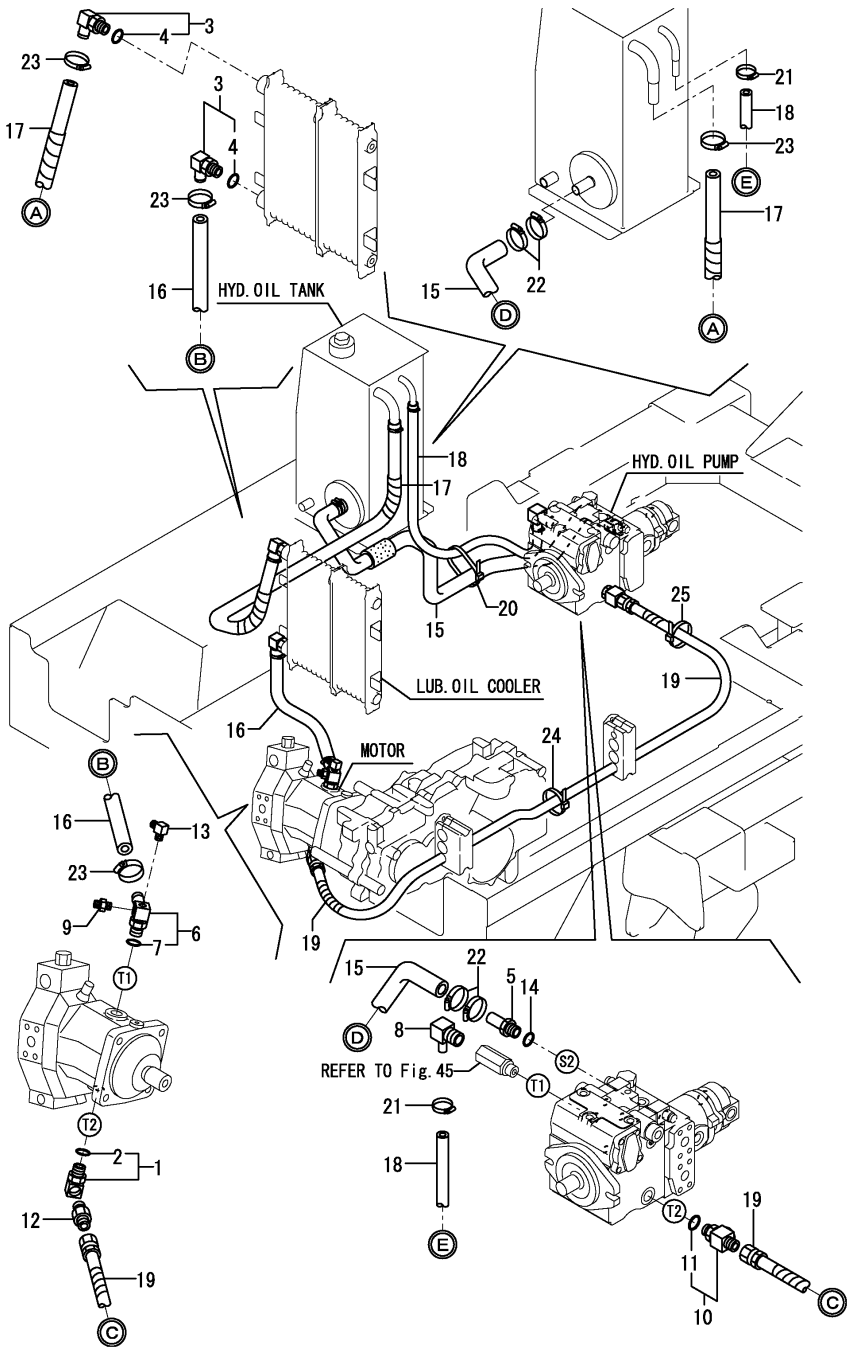
Fig.46. HYD.OIL PIPING(TANK - PUMP , MOTOR)
