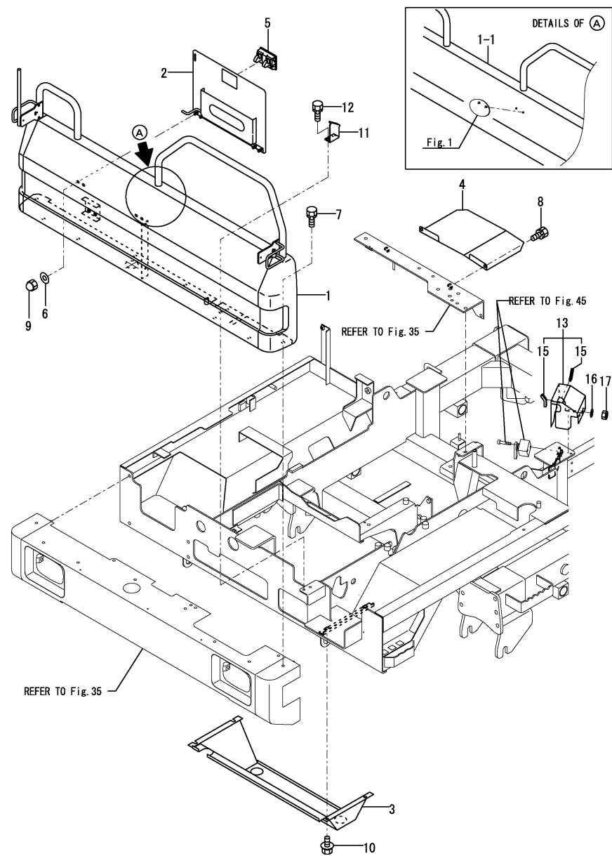
OCS10-G52500 Fig.36. COVER
