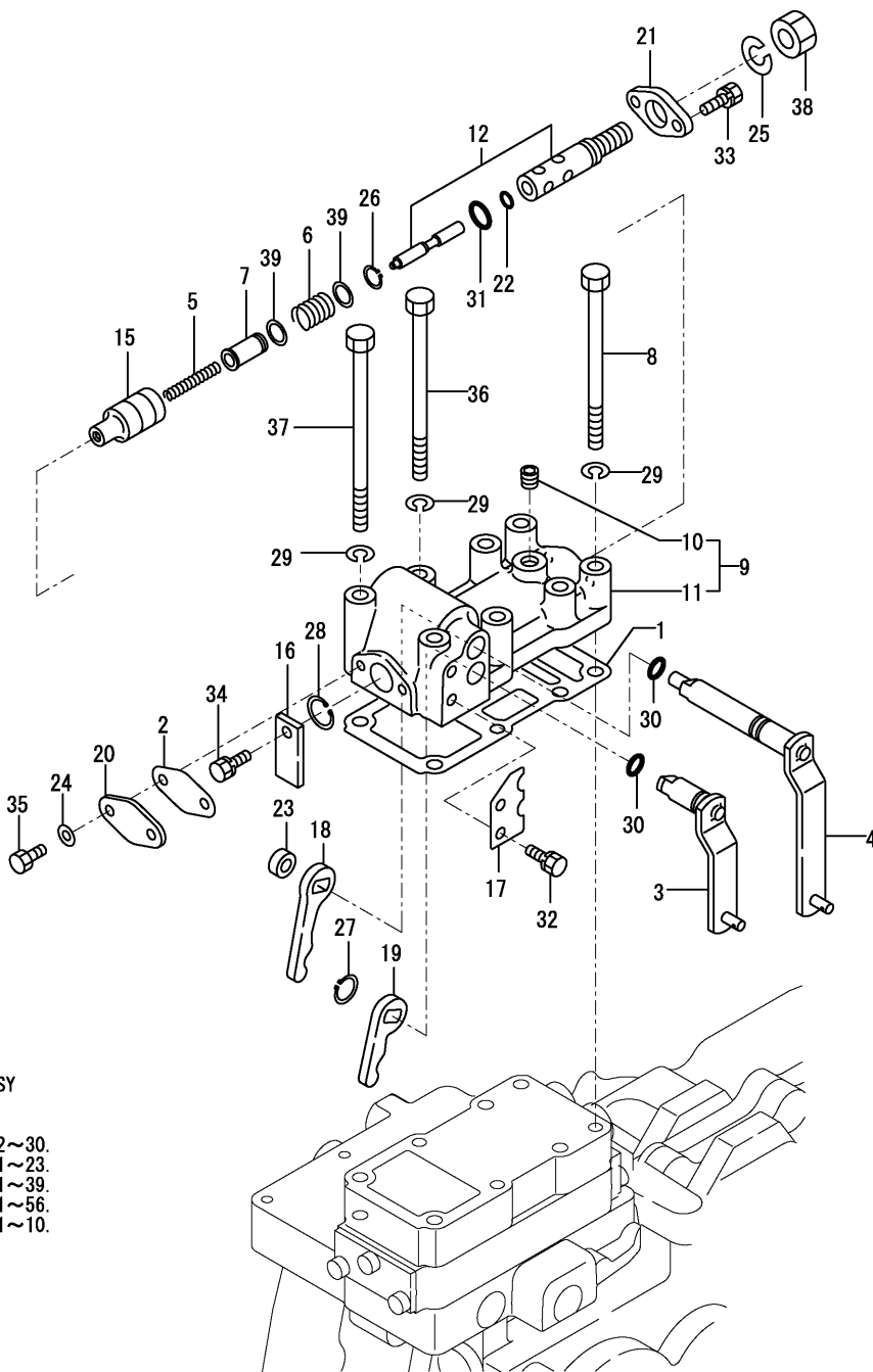
Fig.20. HYD.OIL CONTROL
