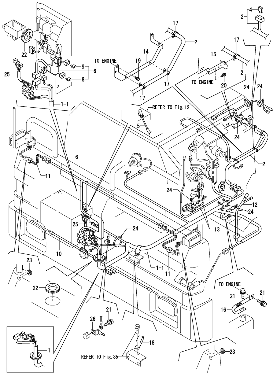
Fig.13. ELECTRIC PART(WIRING)
