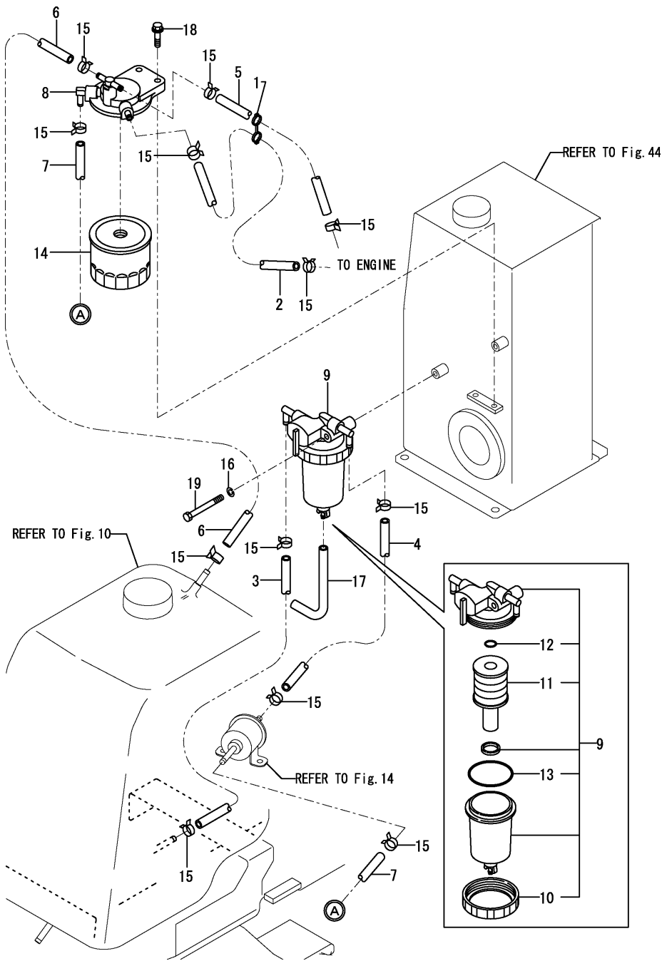
Fig.11. FUEL PIPE
