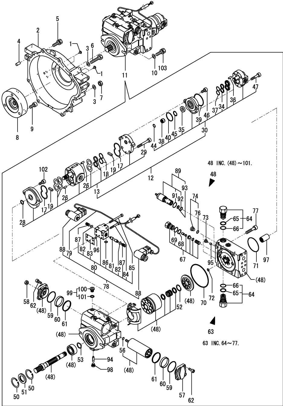
Fig.41. HYD.OIL PUMP & JOINT
