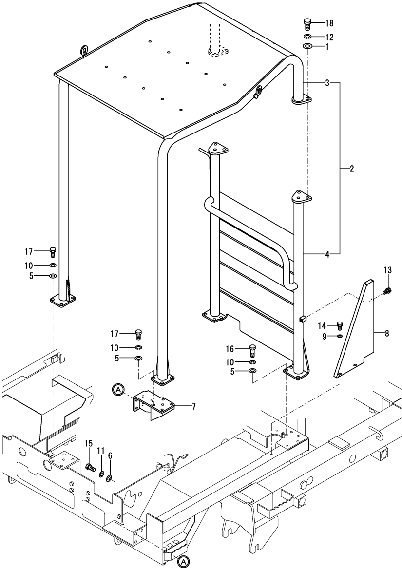
Fig.40. CANOPY(ROPS)
