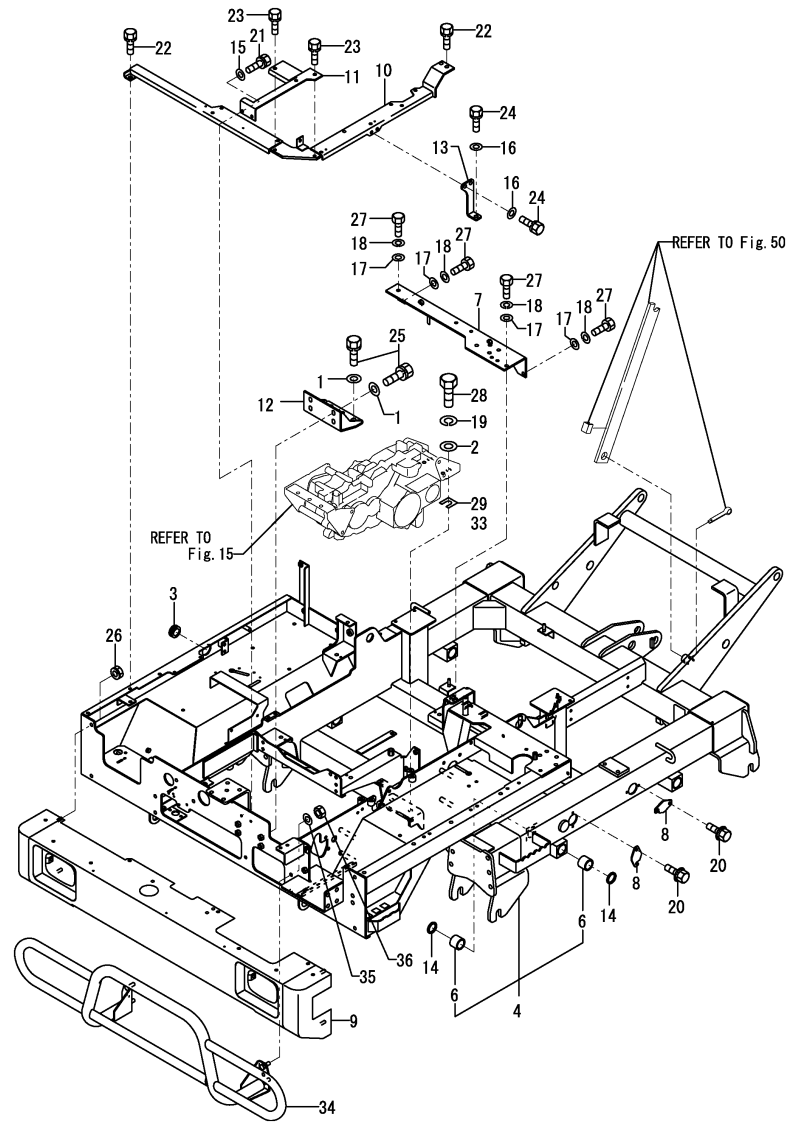
Fig.35. FRAME & BUMPER
