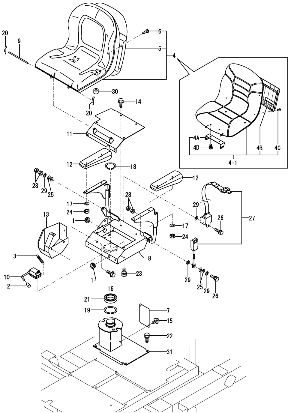
Fig.38. SEAT & MOUNT
