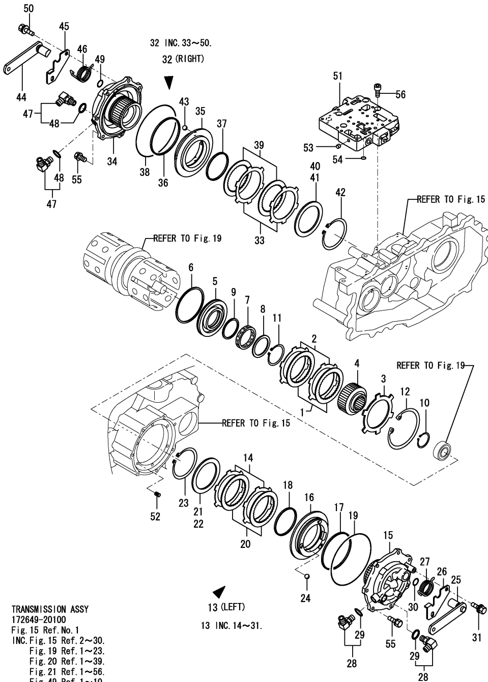
Fig.21. CLUTCH & BRAKE
