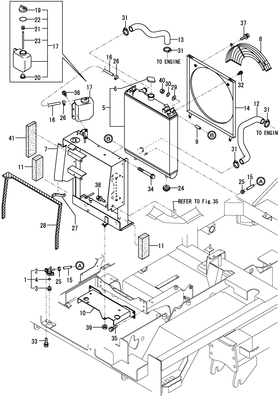
Fig.9. RADIATOR & MOUNT
