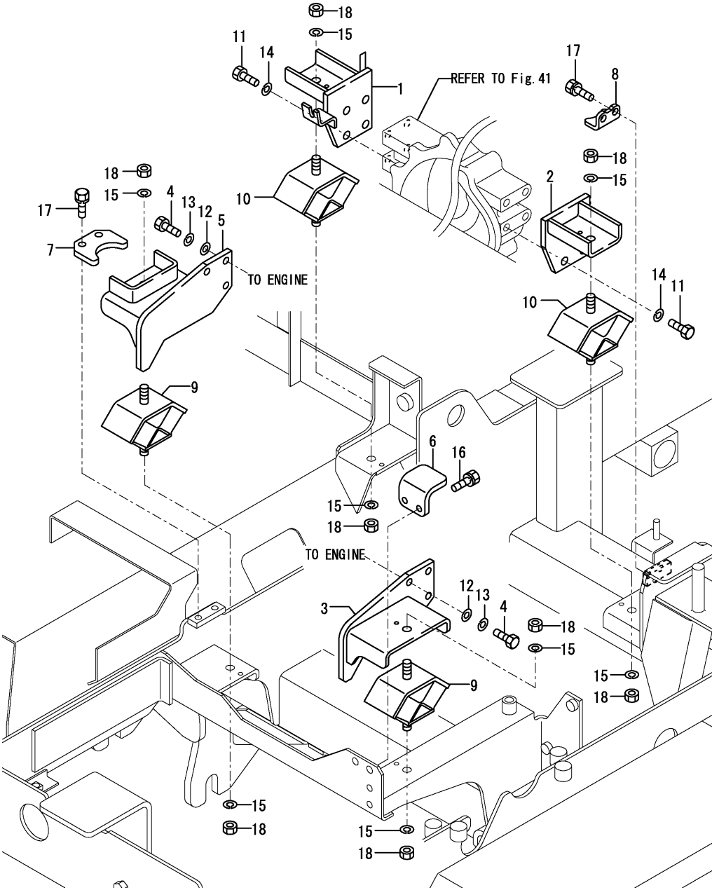
Fig.8. ENGINE MOUNT
