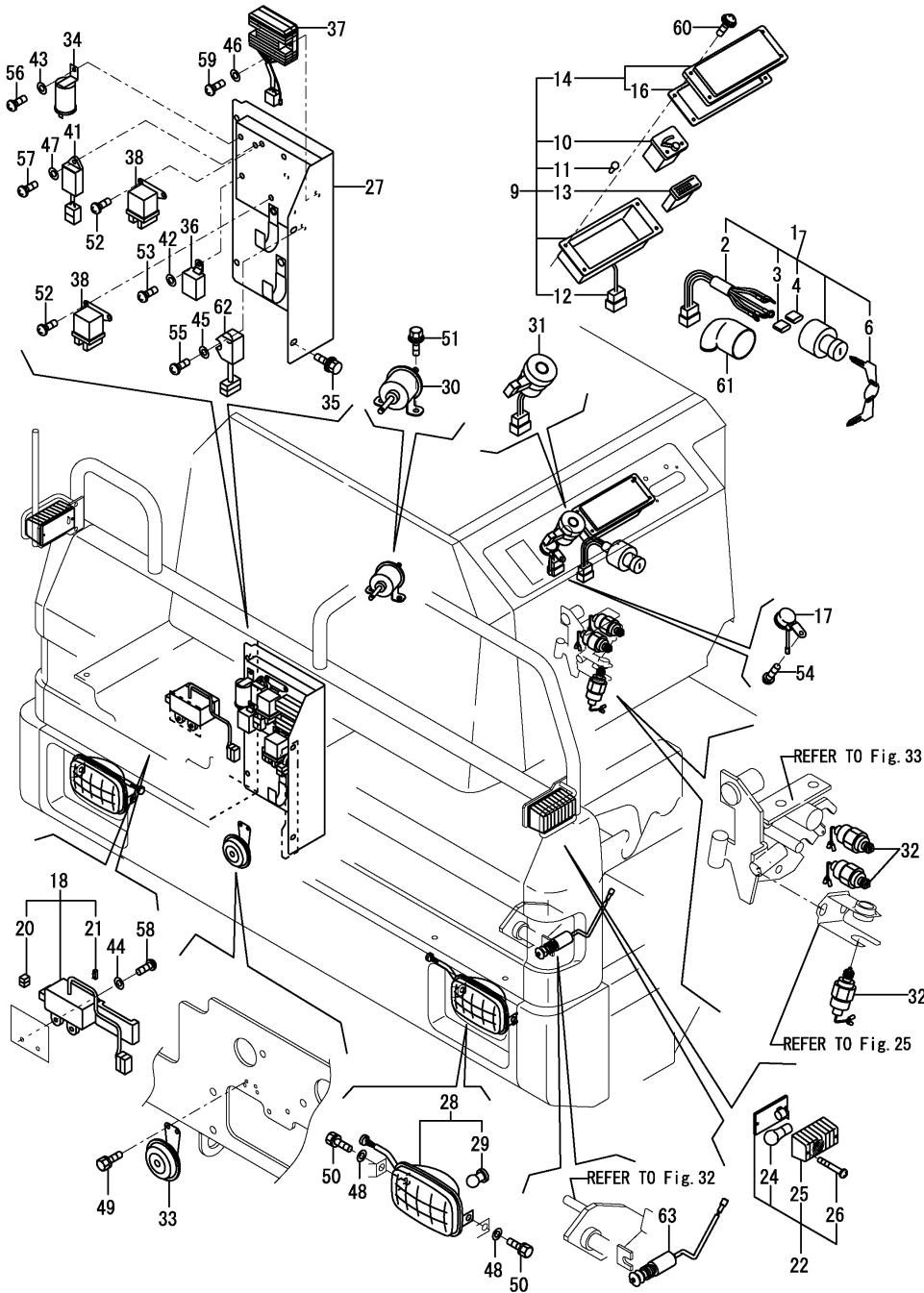
Fig.14. ELECTRIC PART(EQUIPMENT)
