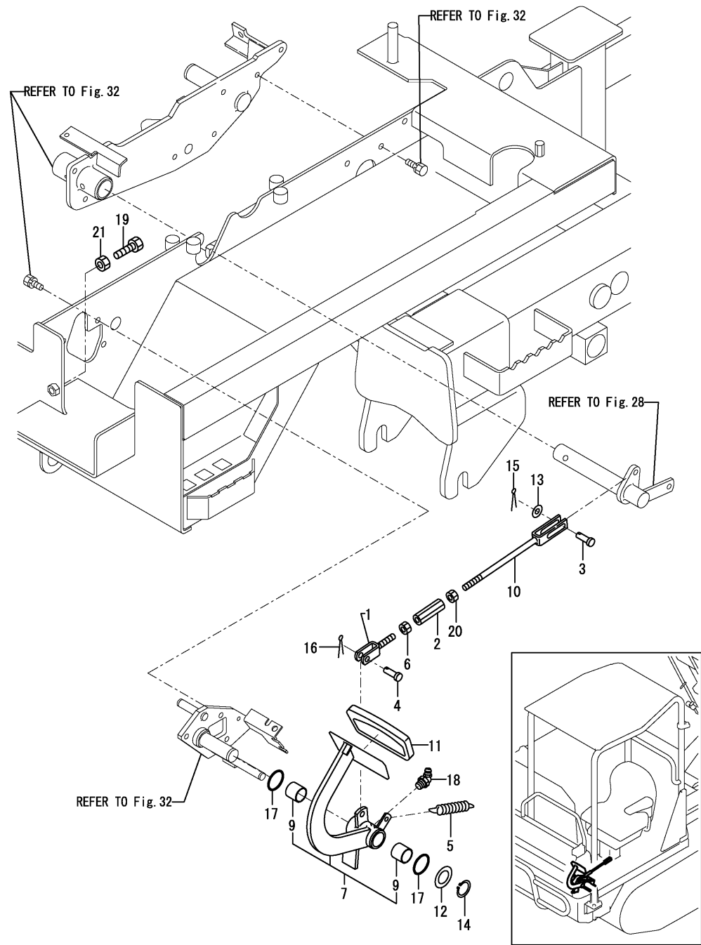
Fig.29. BRAKE(PEDAL & ROD)(FRONT)
