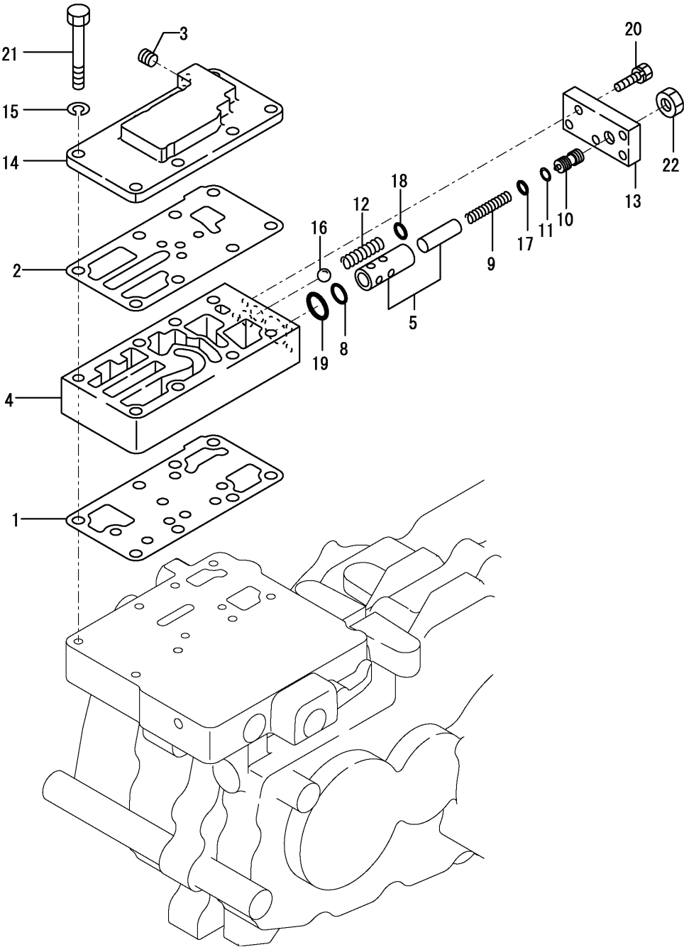
Fig.16. RELIEF VALVE
