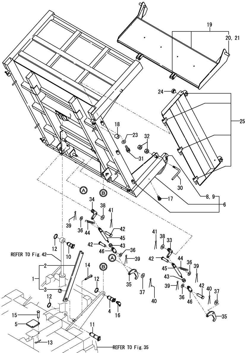
Fig.50. WAGON
