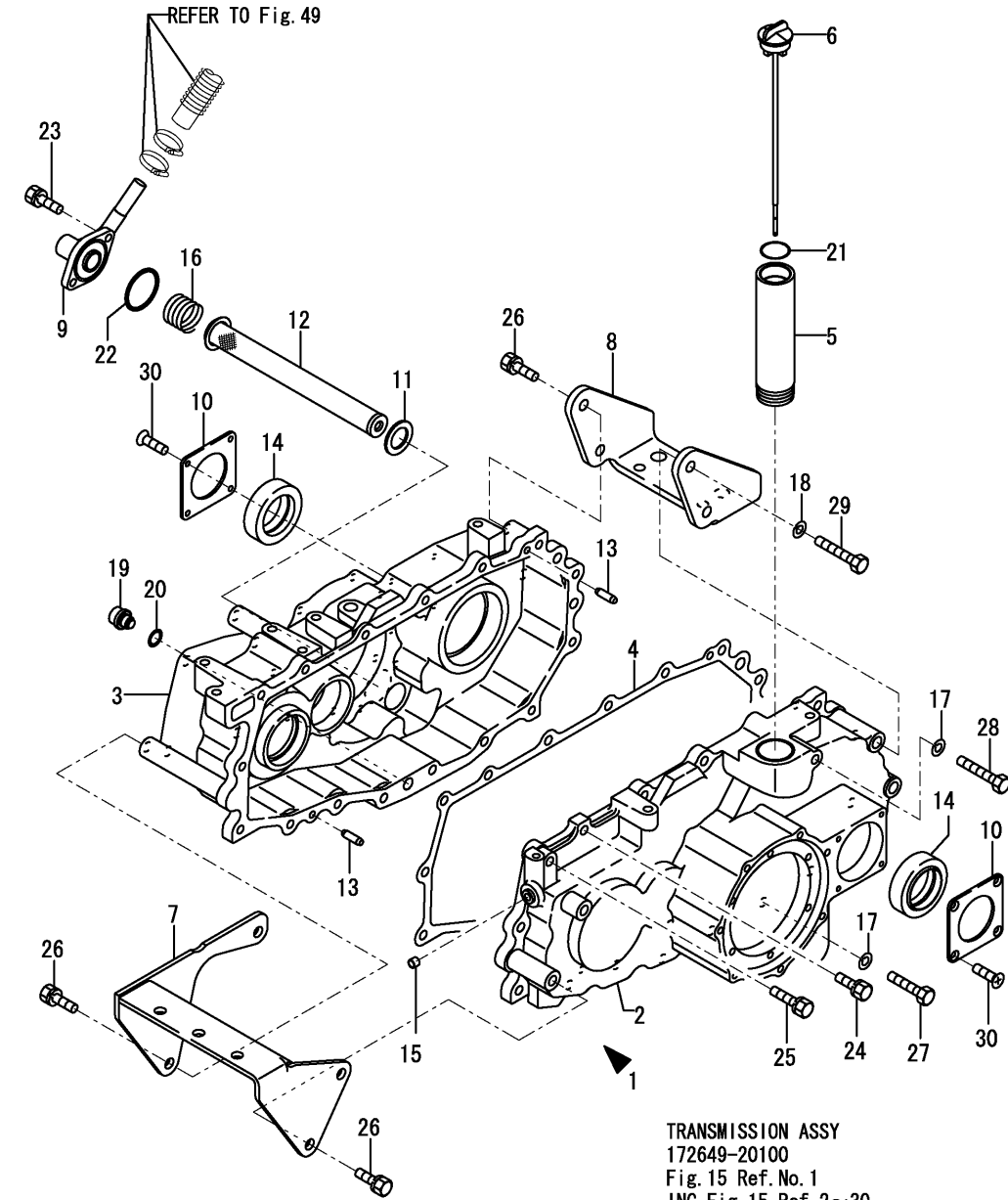
Fig.15. TRANSMISSION CASE
