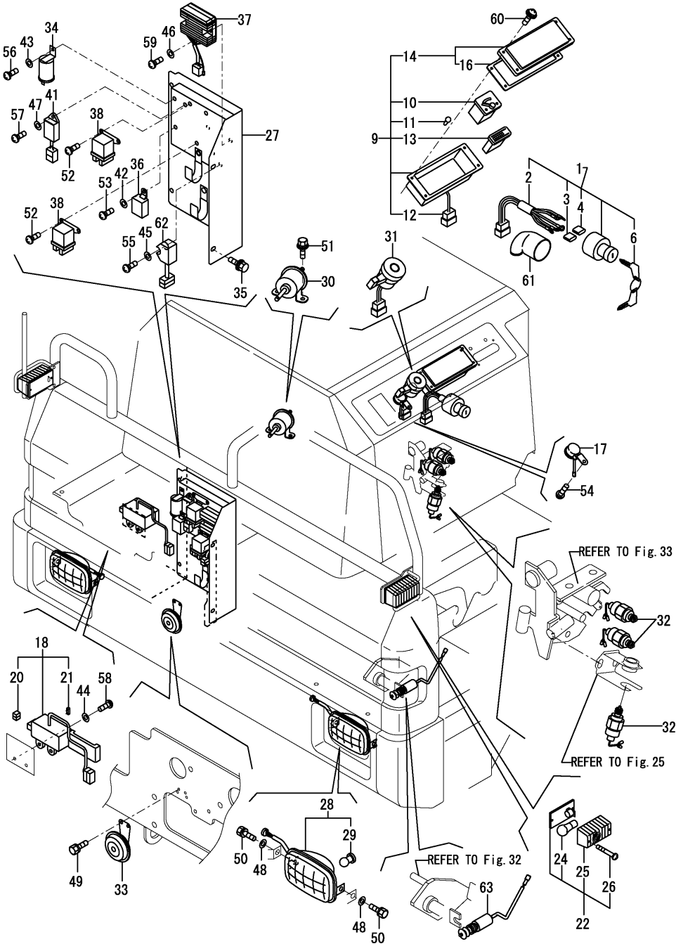
Fig.14. ELECTRIC PART(EQUIPMENT)
