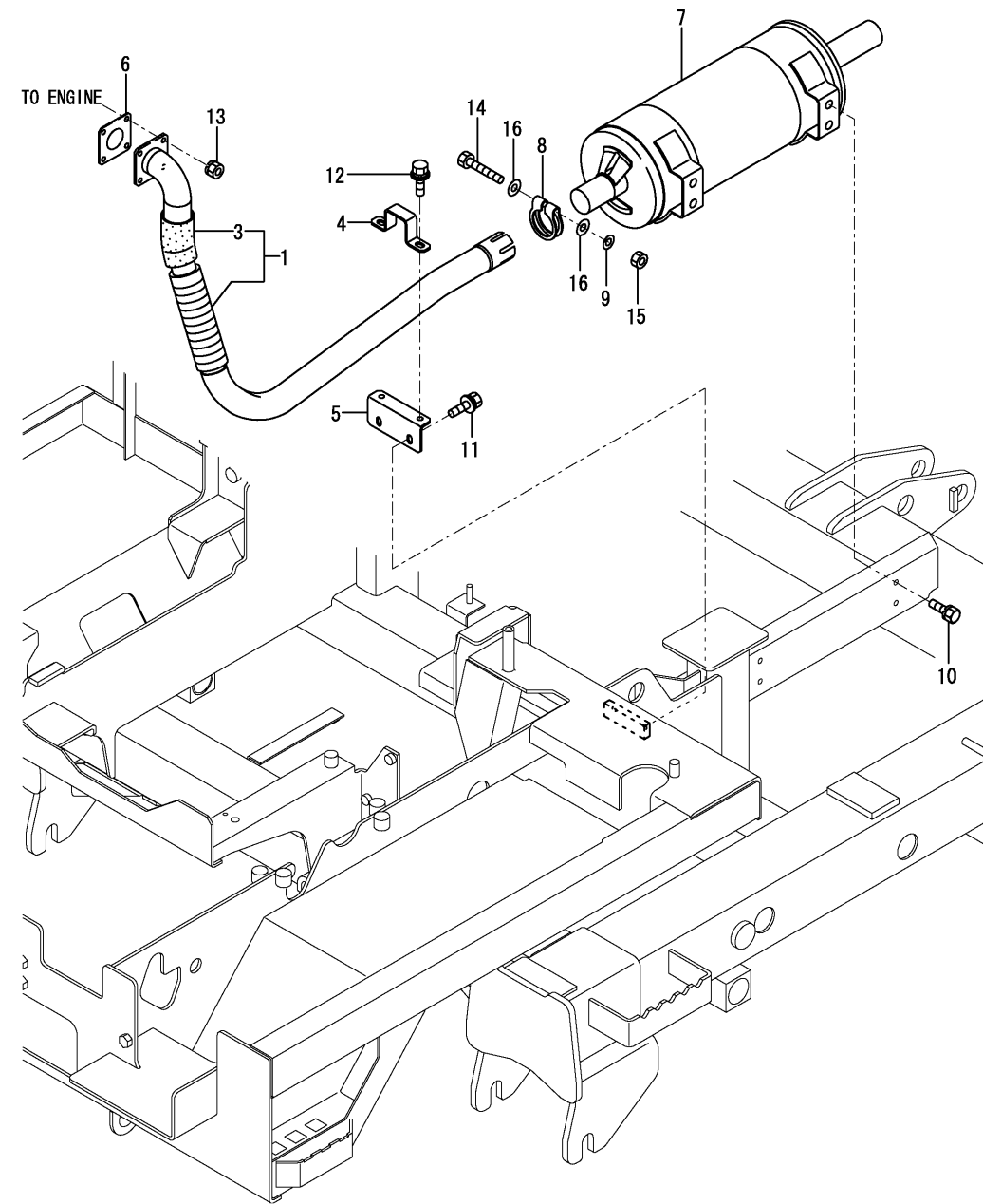
Fig.5. EXHAUST PIPE
