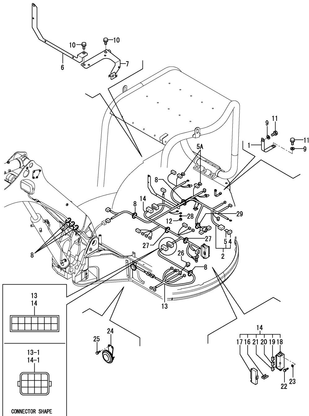
Fig.10. ELECTRIC PART(WIRING)
