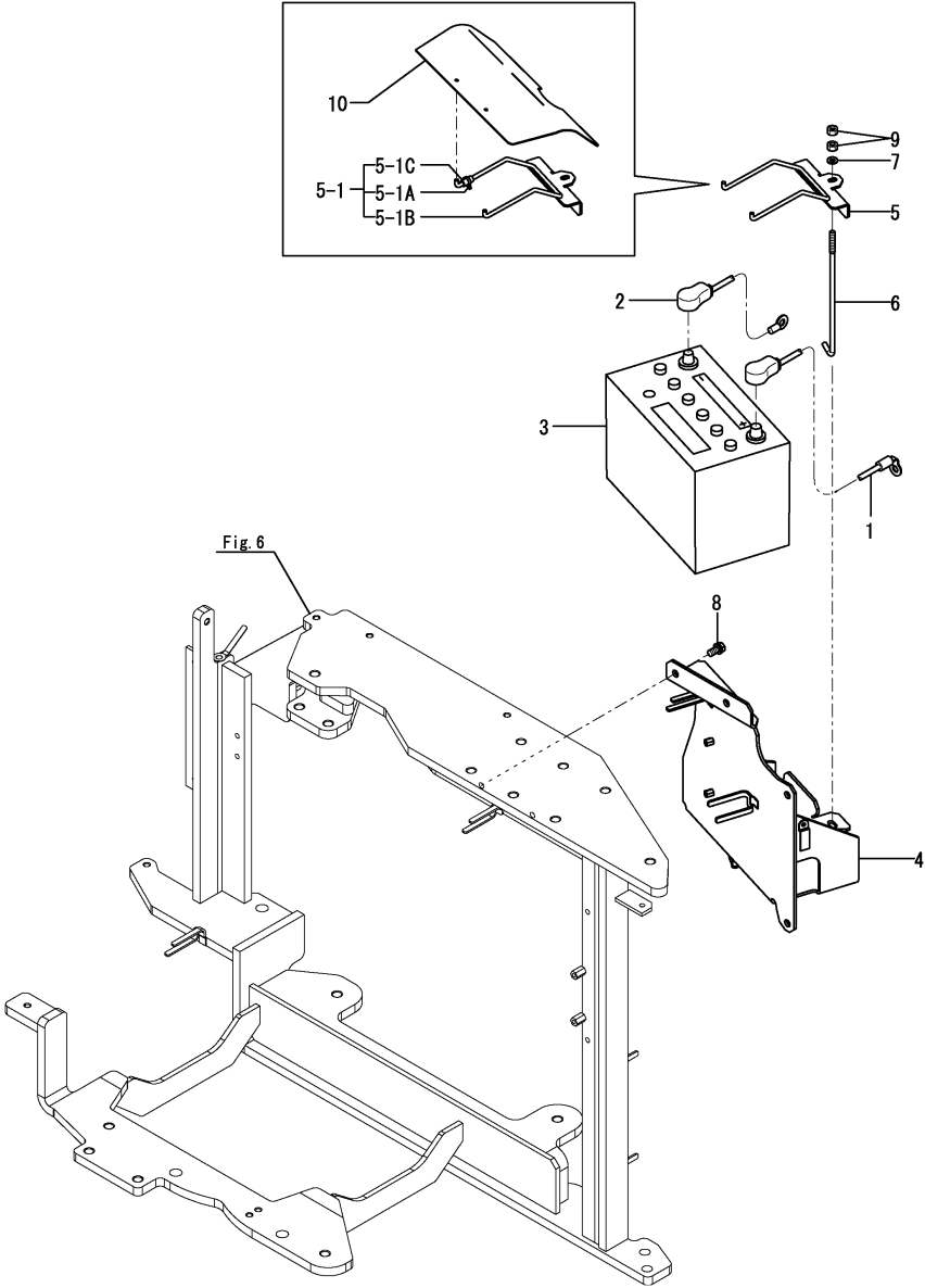
Fig.9. BATTERY
