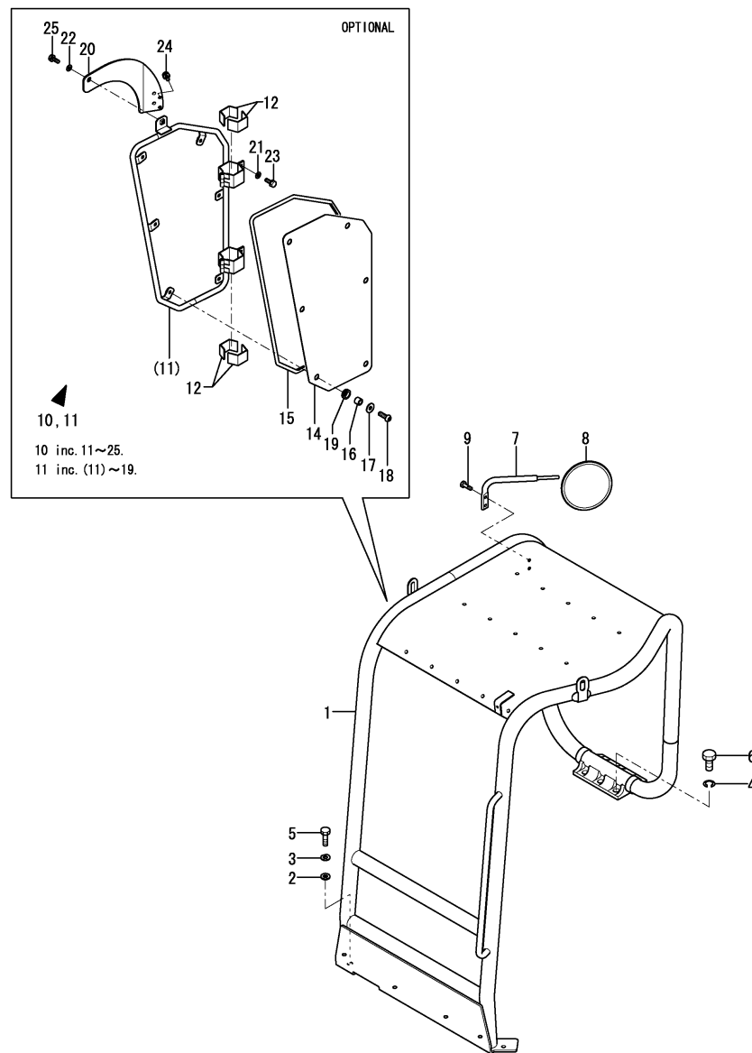
Fig.43. CANOPY
