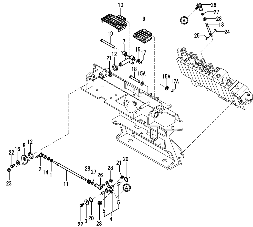
Fig.28. SWING PEDAL
