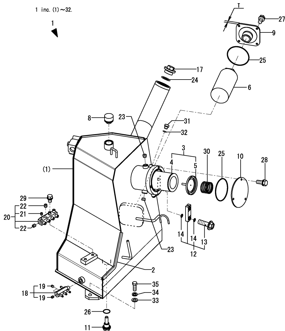
Fig.69. HYD.OIL TANK
