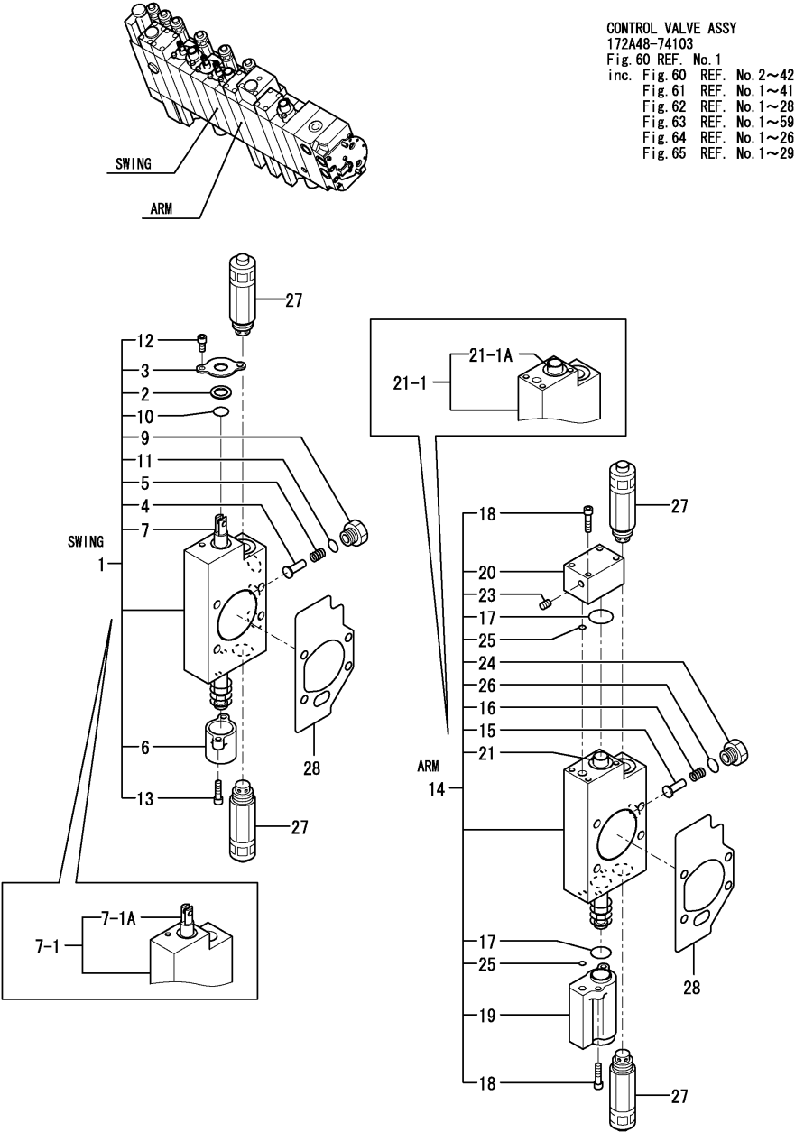
Fig.62. CONTROL VALVE(ARM & SWING)(SG)
