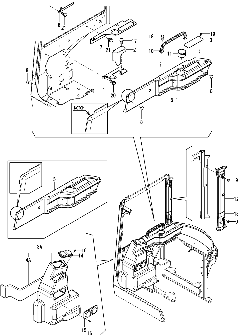
Fig.34. COVER(CABIN : 1)
