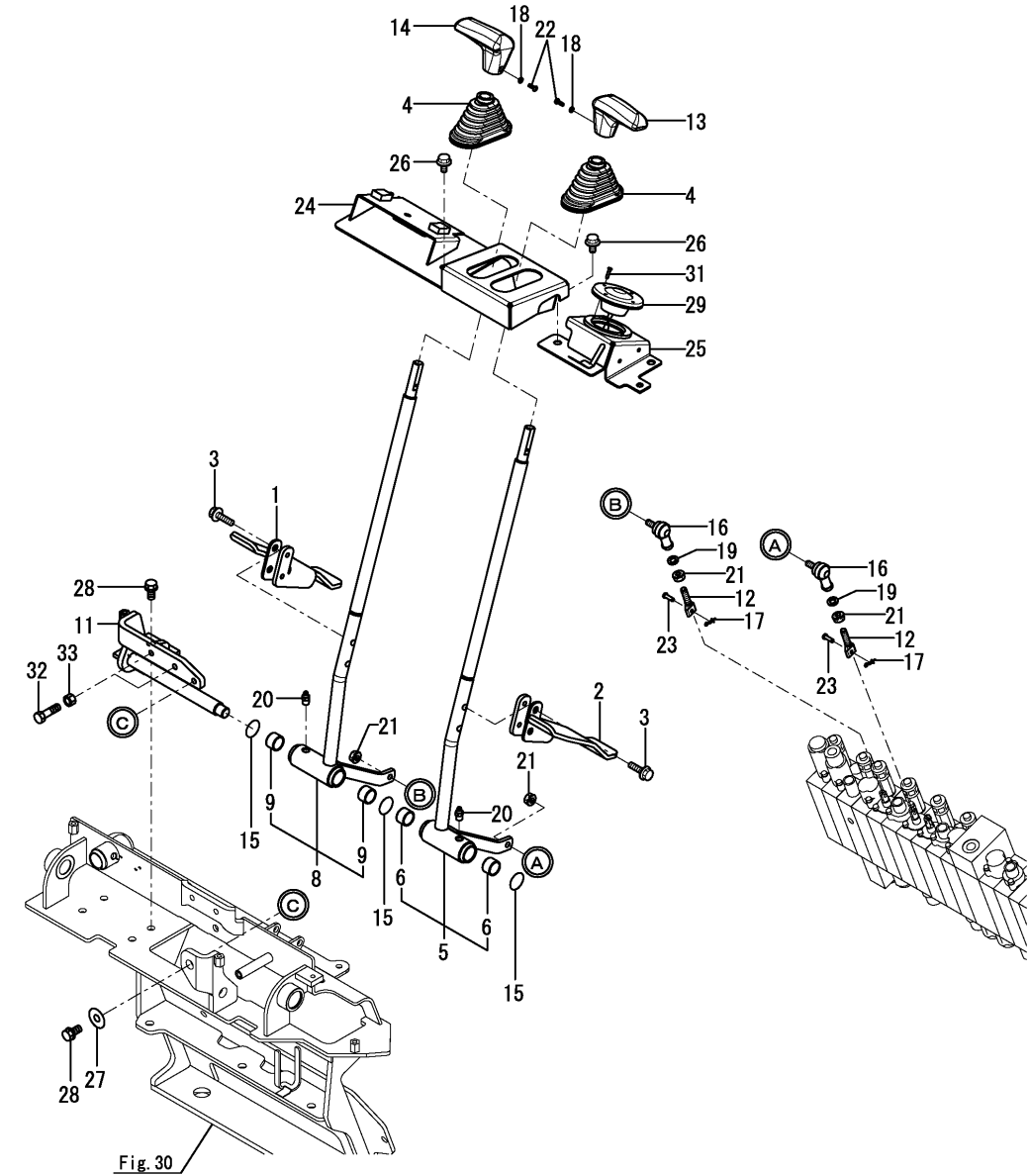
Fig.25. TRAVEL LEVER
