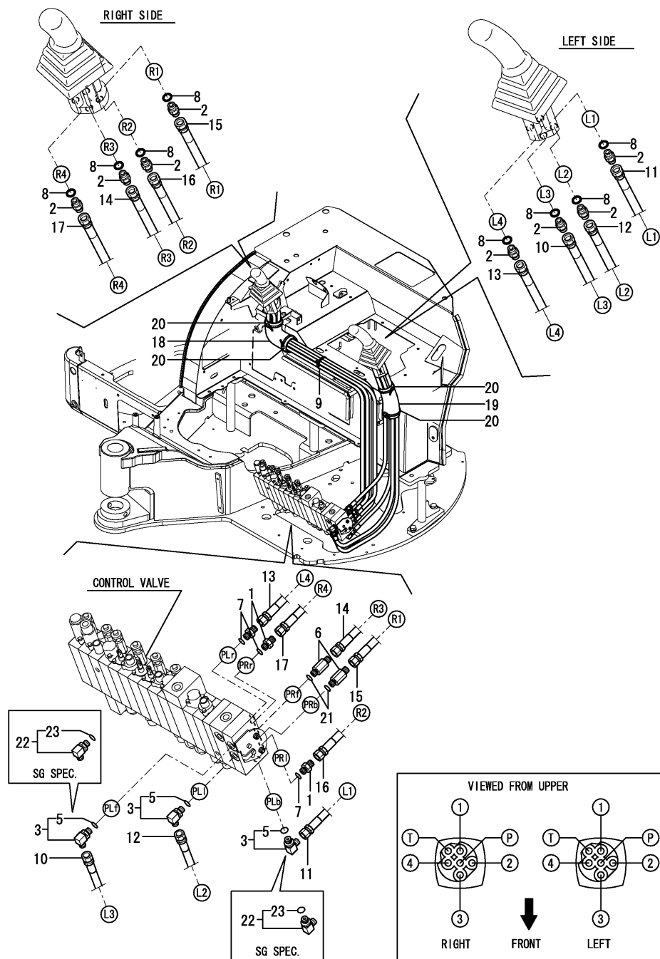
Fig.81. CONTROL PIPING(VAIVE - REMOTE CONTROL VALVE)
