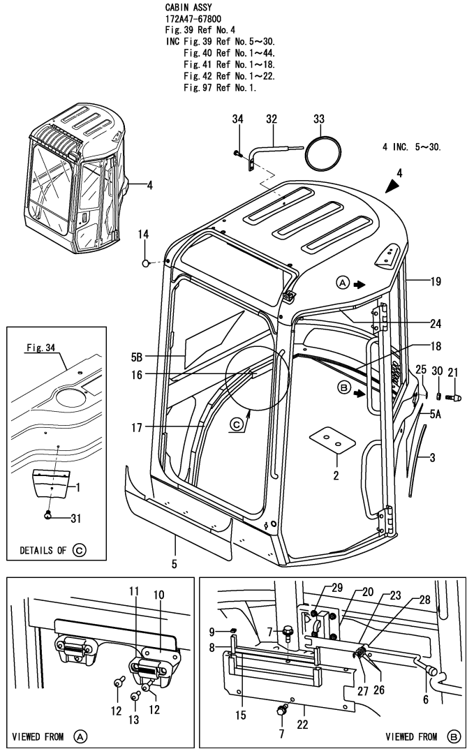
Fig.39. CABIN(BODY)
