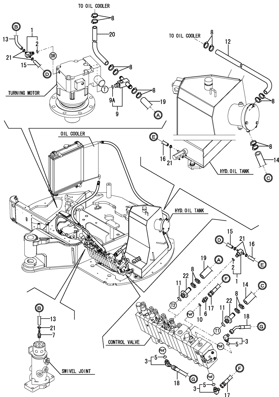
Fig.73. HYD.OIL PIPING(RETURN)
