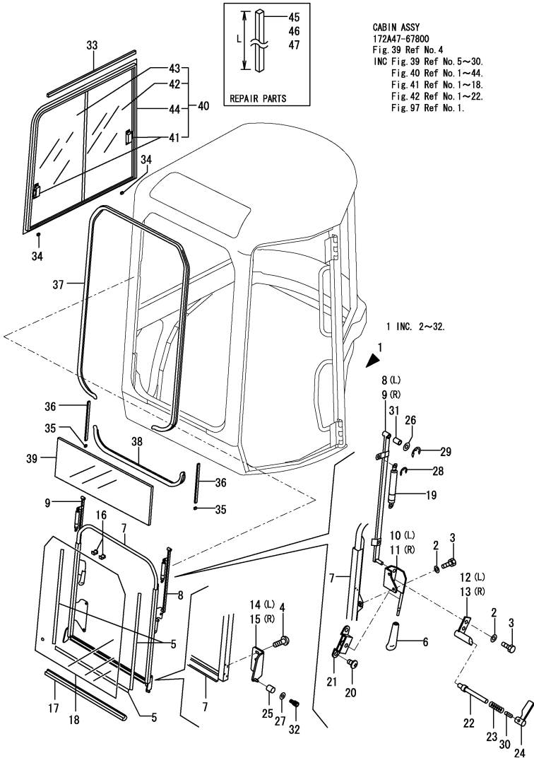
Fig.40. CABIN(GLASS)
