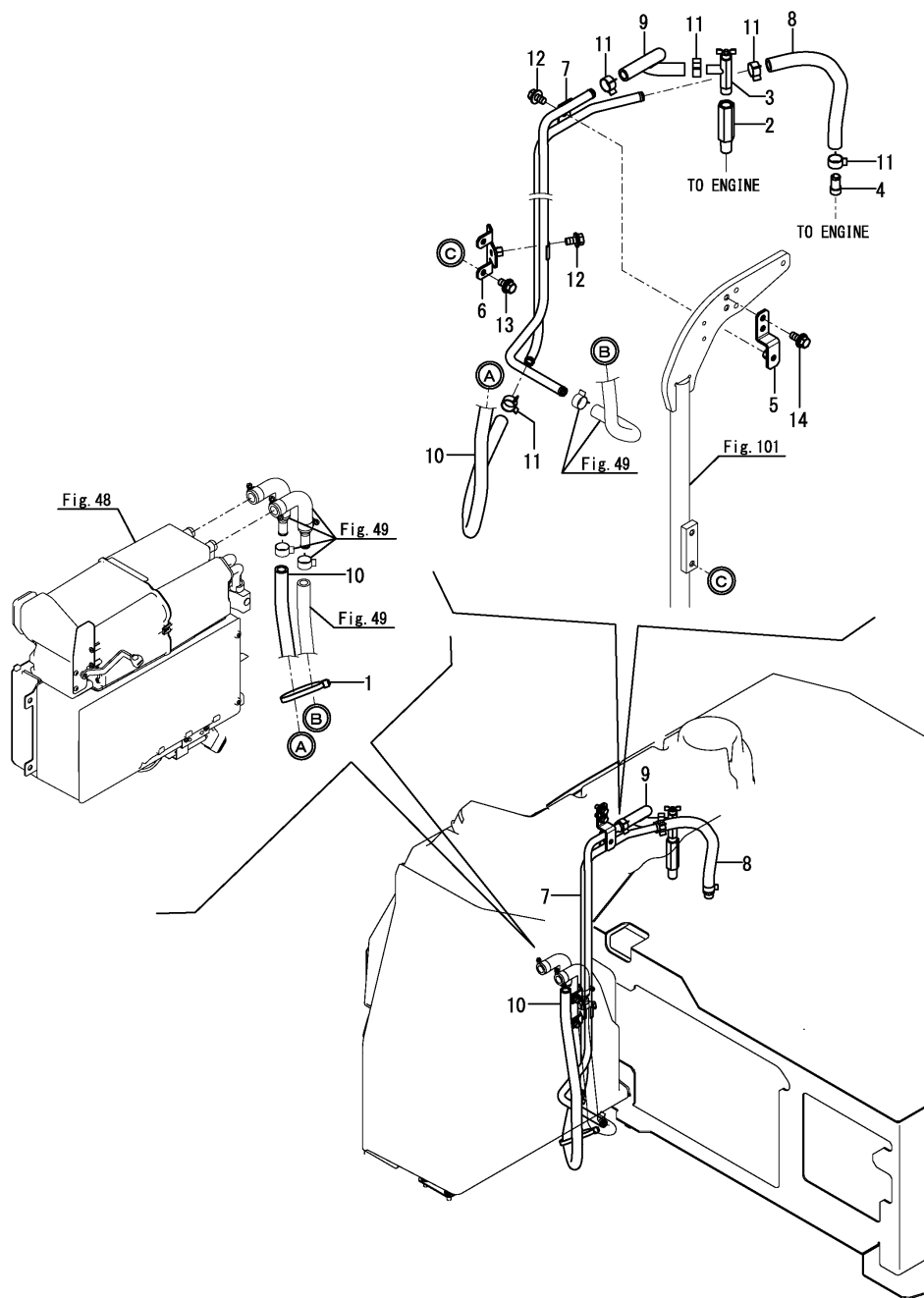
Fig.50. HEATER(PIPING)
