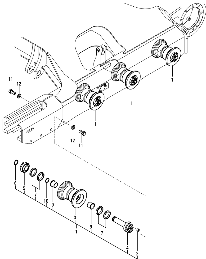
Fig.54. TRACK ROLLER
