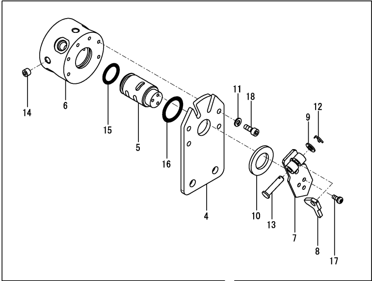
Fig.154. 2-WAY VALVE
