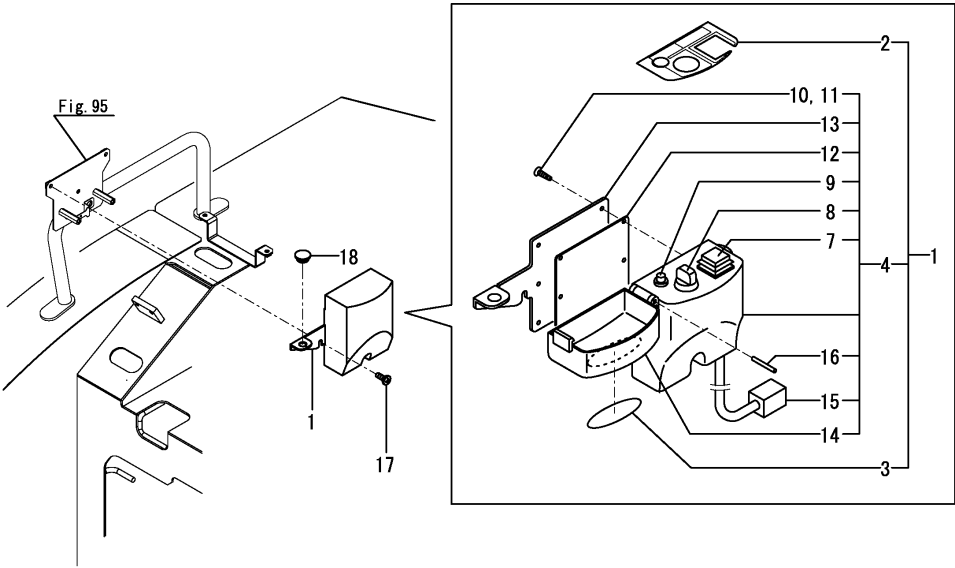
Fig.39. QUICK COUPLER(SWITCH BOX)
