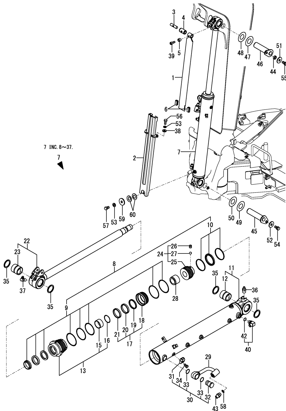
Fig.121. BOOM CYLINDER
