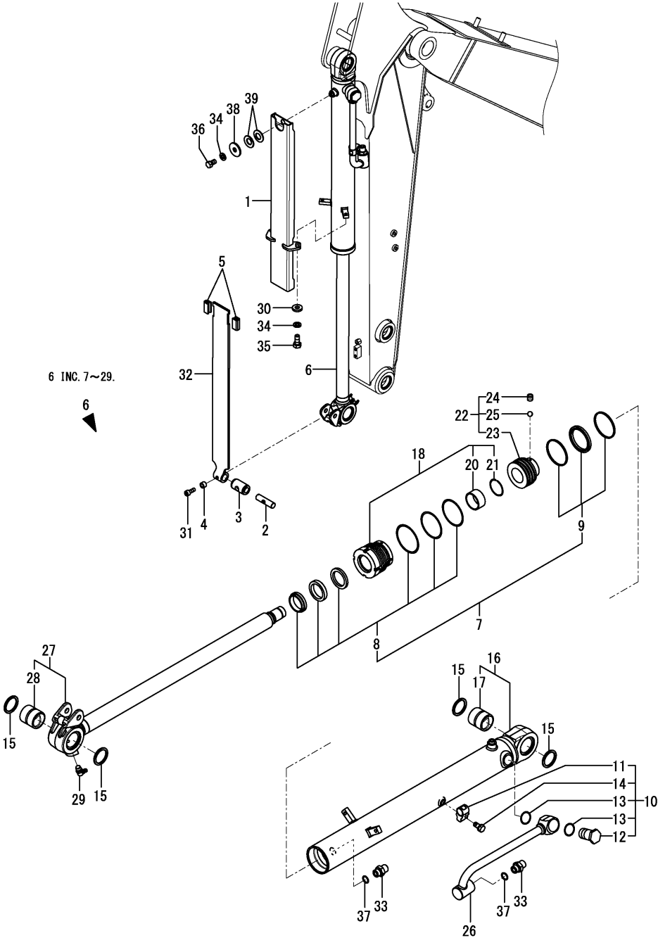
Fig.124. BUCKET CYLINDER
