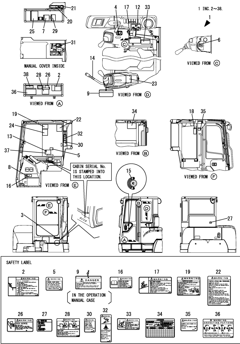
Fig.6. LABEL(CABIN)(ANGLE BLADE SPEC.)
