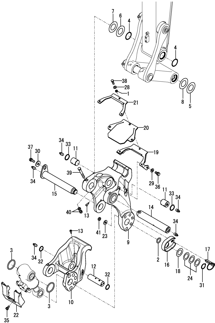
Fig.192. QUICK COUPLER(BODY)
