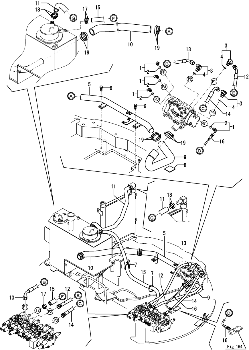
Fig.161. TANK - PUMP & CONTROL VALVE
