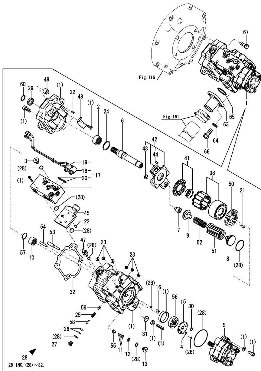
Fig.119. HYDRAULIC PUMP(E.S.S. SPEC.)
