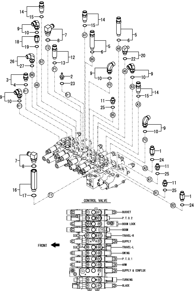
Fig.163. CONTROL VALVE(FITTING)(1)
