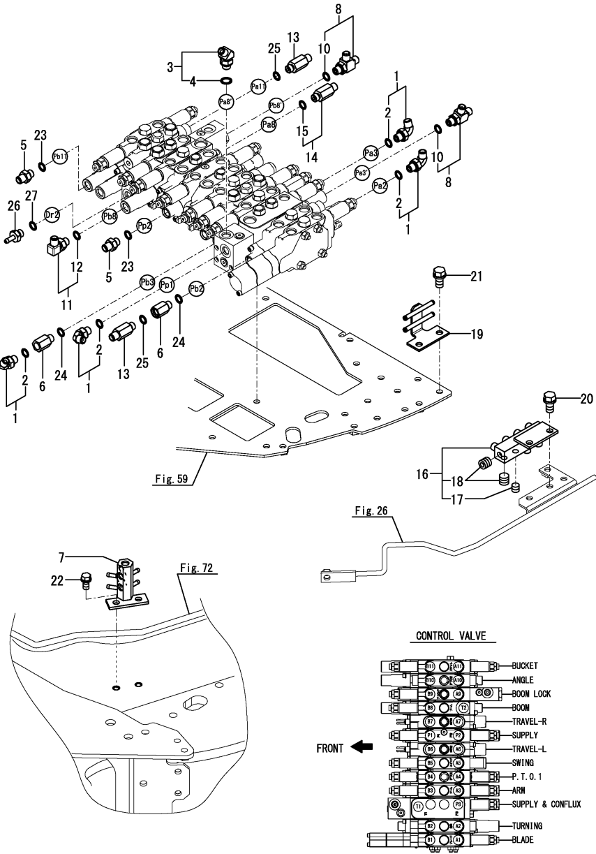
Fig.166. CONTROL VALVE(FITTING)(2)(ANGLE BLADE SPEC.)
