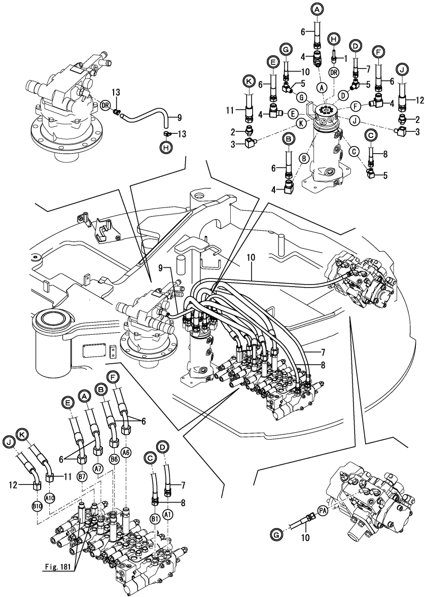
Fig.171. CONTROL VALVE - SWIVEL JOINT(ANGLE BLADE SPEC.)
