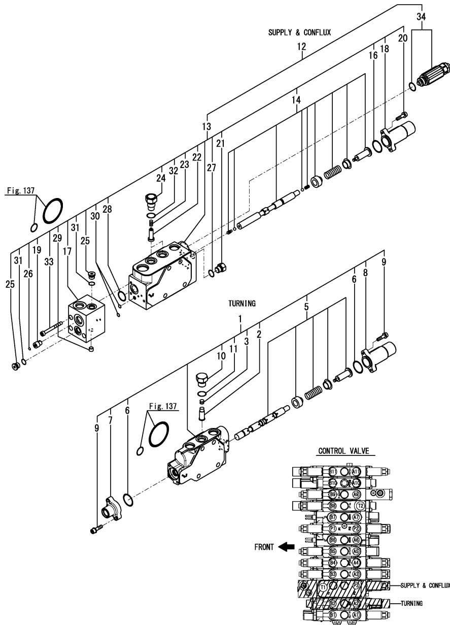
Fig.142. CONTROL VALVE(7/8)
