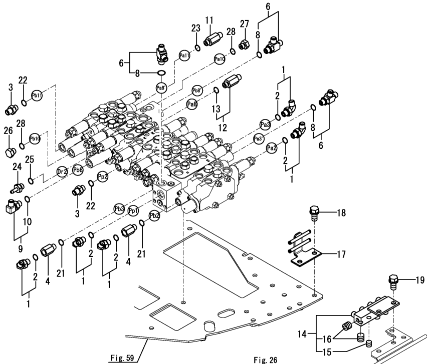
Fig.164. CONTROL VALVE(FITTING)(2)
