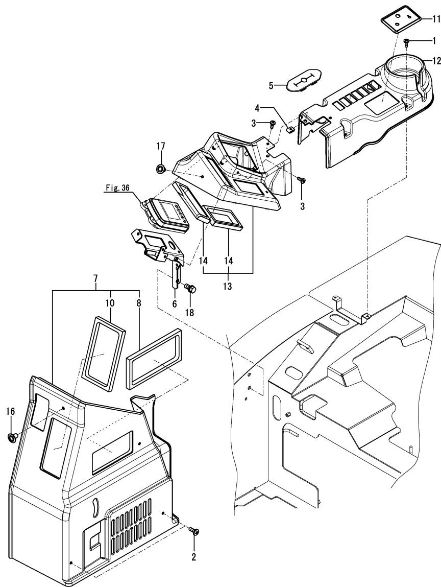
Fig.87. COVER(MONITOR)(CABIN)(AIR CONDITIONER SPEC.)
