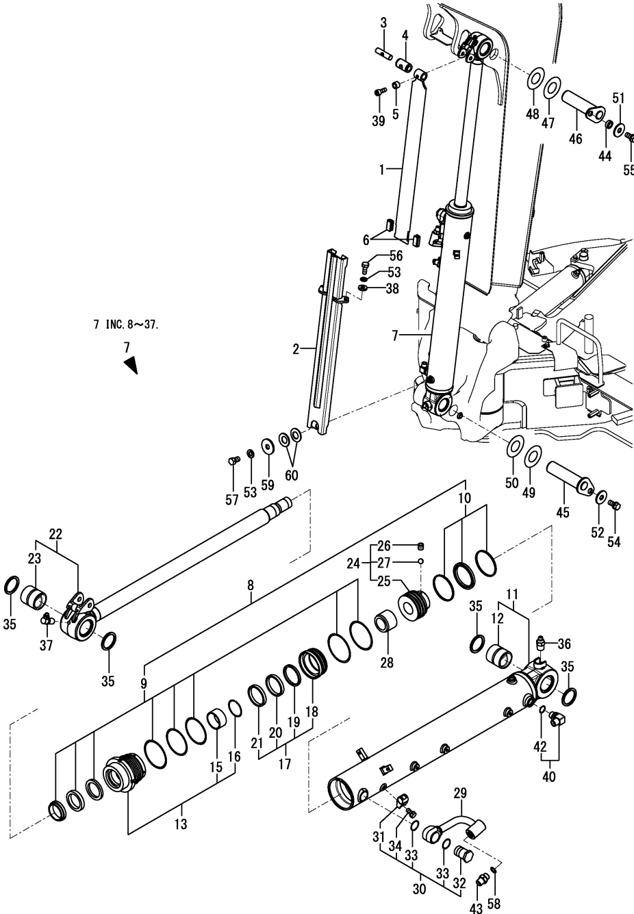
Fig.121. BOOM CYLINDER
