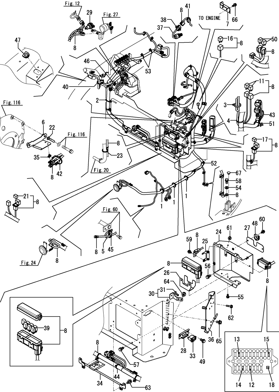
Fig.28. AROUND THE SEAT
