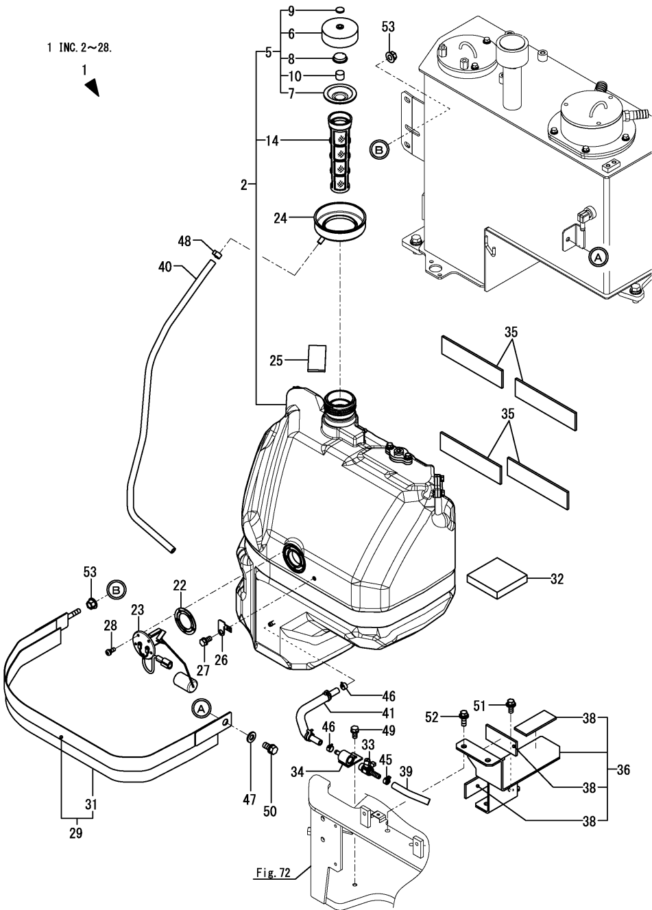
Fig.19. FUEL TANK
