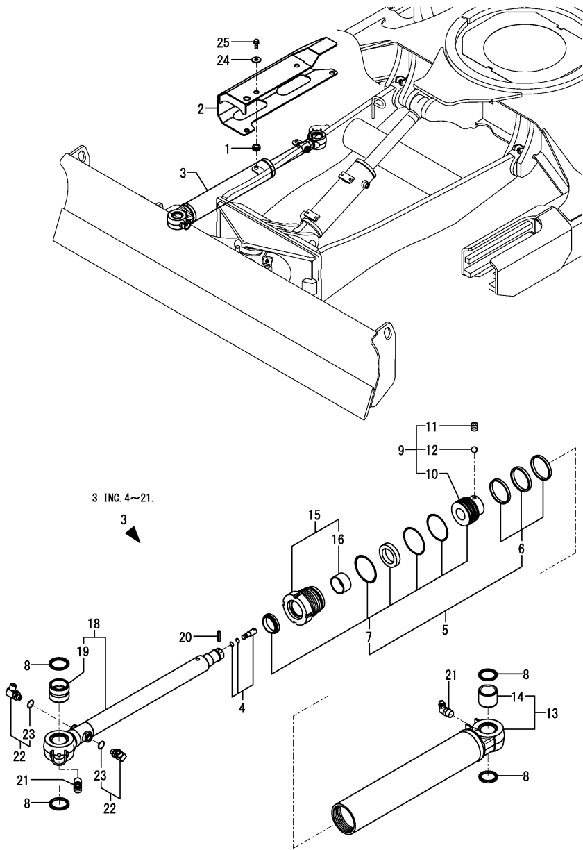
Fig.129. ANGLE CYLINDER(ANGLE BLADE SPEC.)
