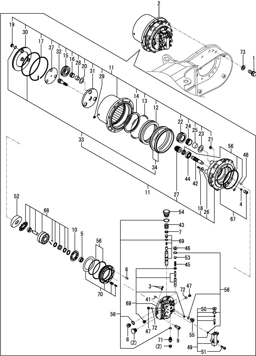
Fig.131. TRAVEL MOTOR
