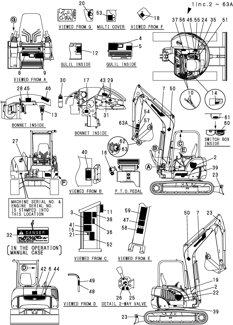
Fig.4. LABEL(CANOPY)(QUICK COUPLER)
