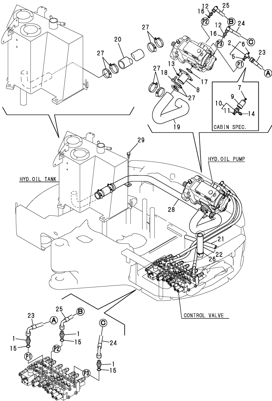
Fig.69. HYD.OIL PIPING(T.-P.-VALVE)
