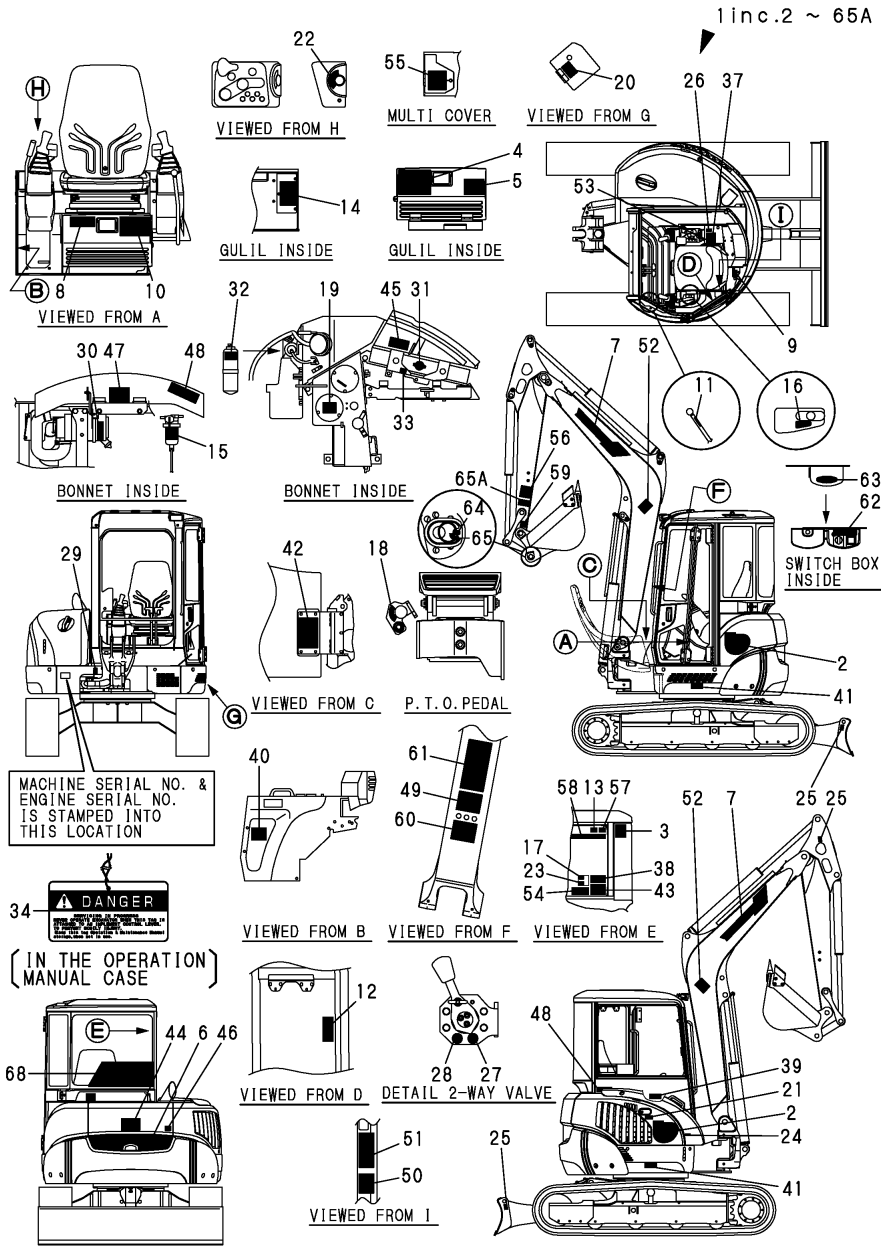
Fig.3. LABEL(CABIN)(QUICK COUPLER)
