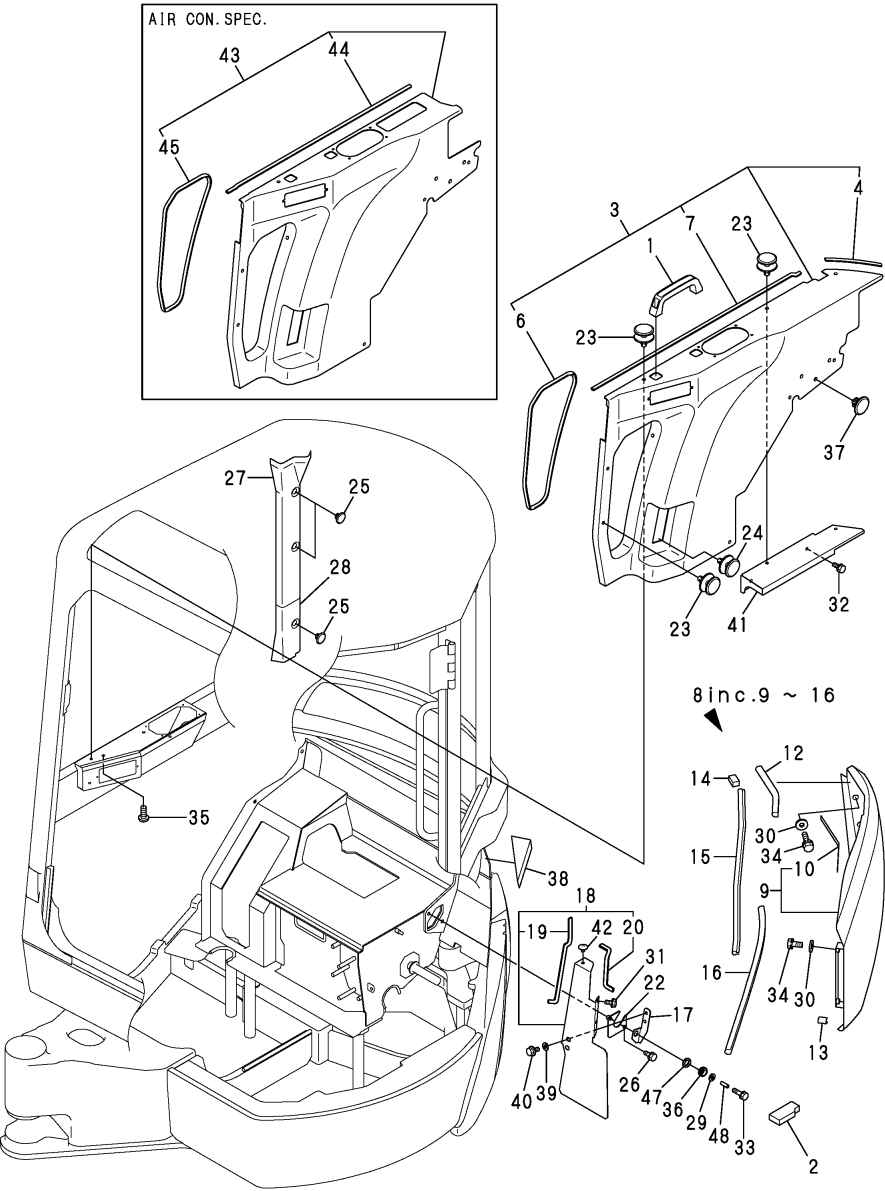
Fig.34. COVER(CABIN)
