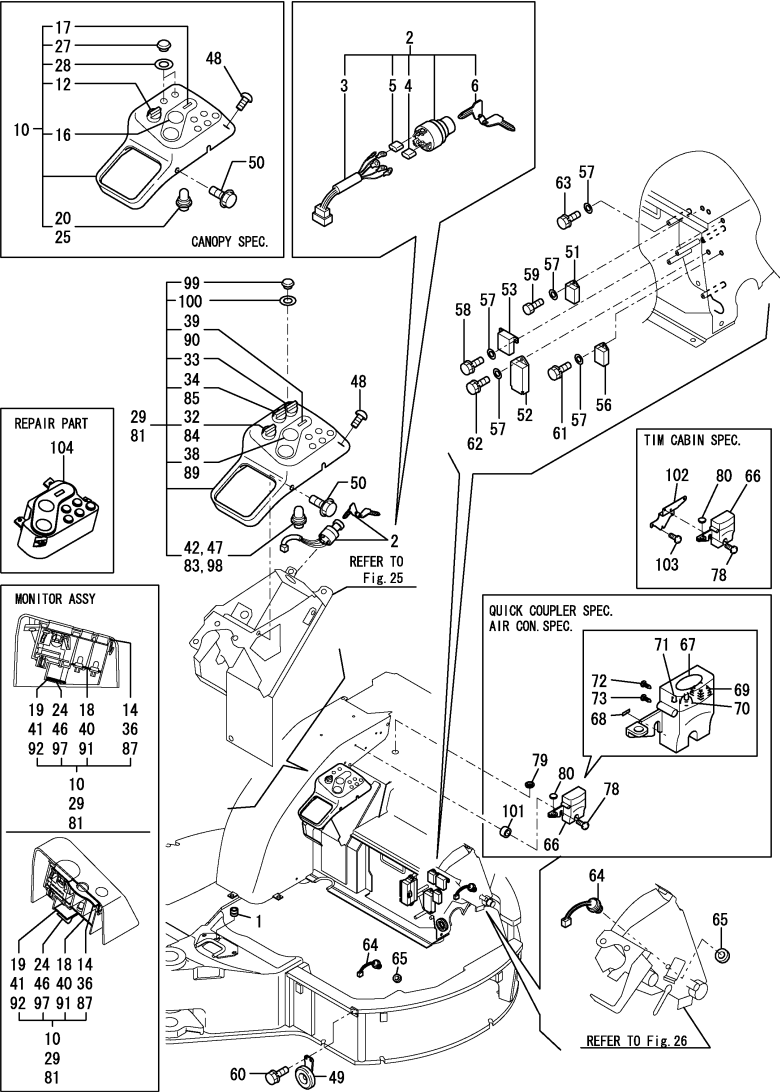
Fig.13. ELECTRIC PART(EQUIPMENT)
