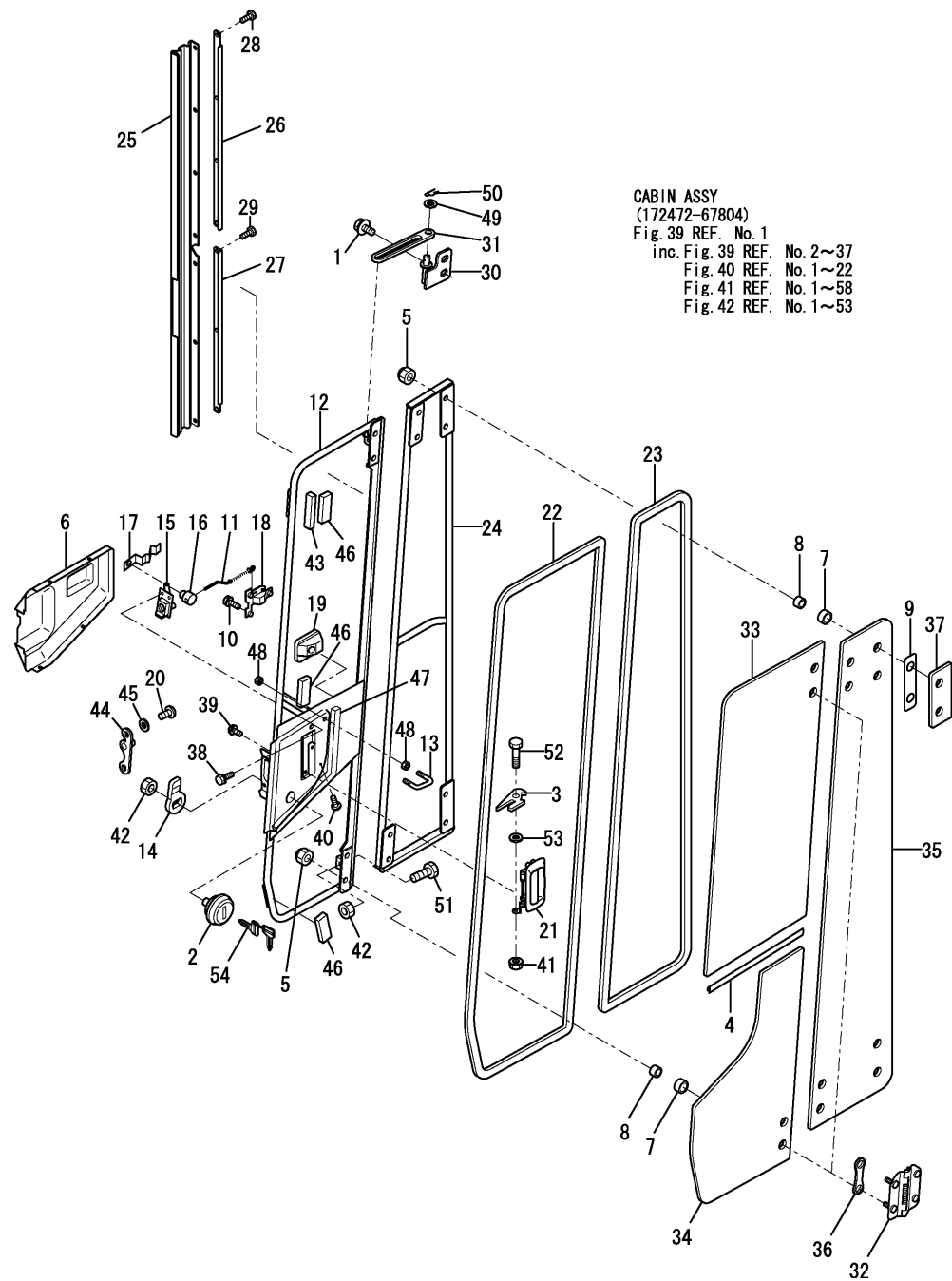
Fig.42. CABIN(DOOR)
