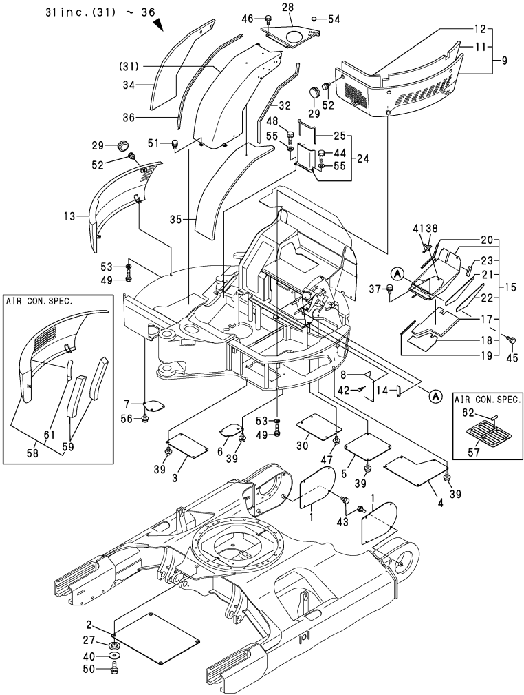
Fig.33. COVER(FRAME)
