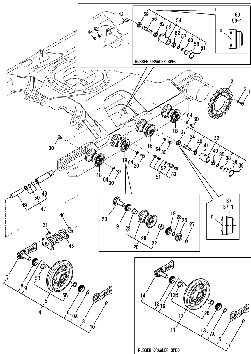
Fig.23. ROLLER & ADJUST
