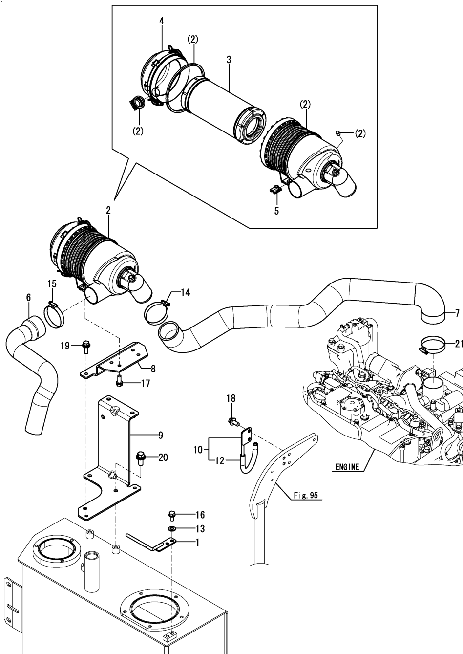
Fig.8. AIR CLEANER
