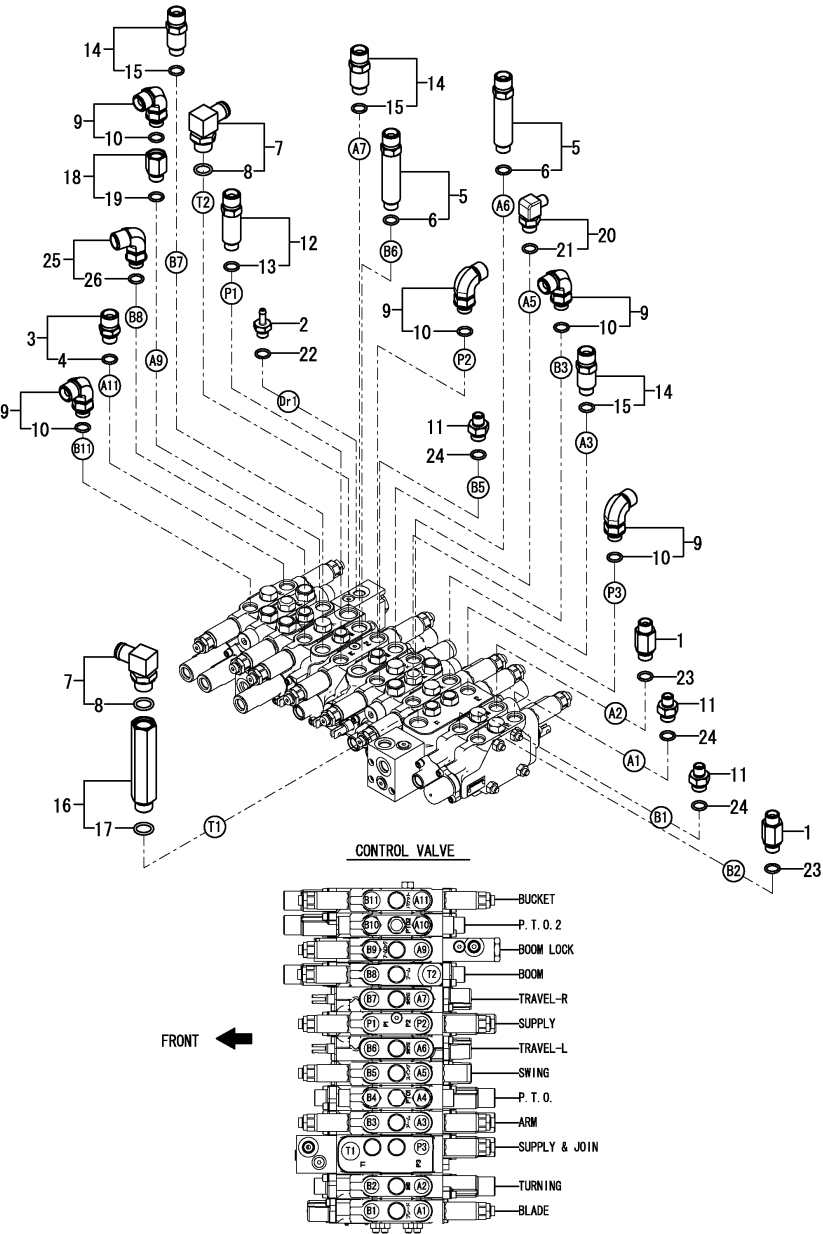
Fig.133. CONTROL VALVE(FITTING)(1)
