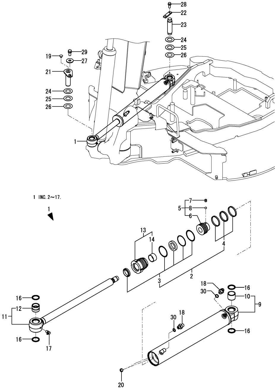
Fig.117. SWING CYLINDER
