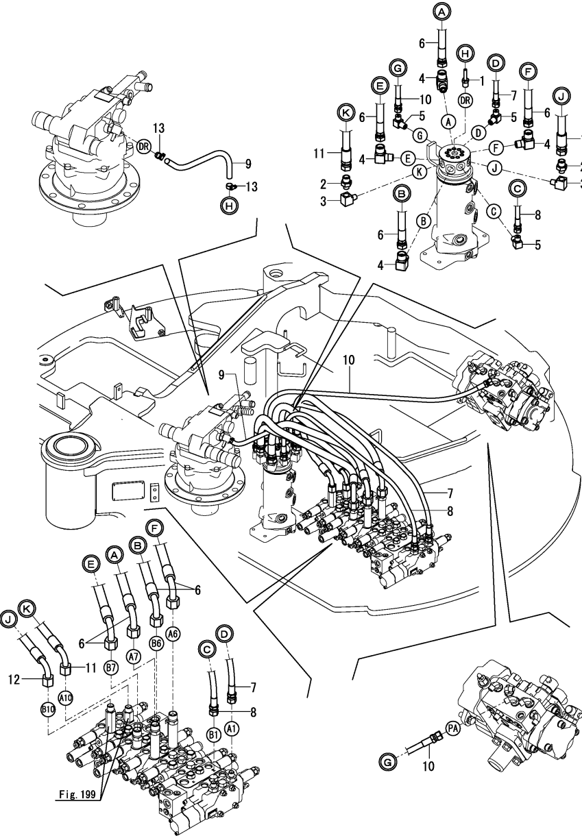
Fig.195. (138A)CONTROL VALVE - SWIVEL JOINT(ANGLE BLADE SPEC.)
