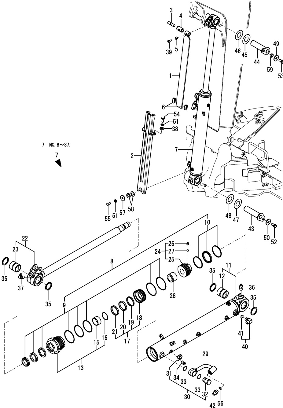
Fig.113. BOOM CYLINDER
