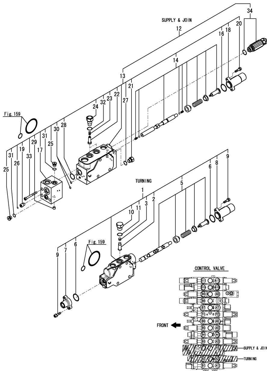
Fig.164. (124F)CONTROL VALVE(7/8)
