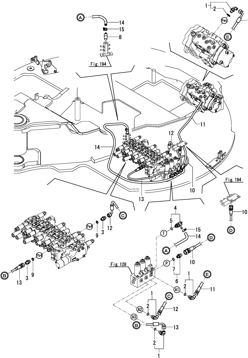
Fig.198. (144A)P.T.O.(SOLENOID VALVE & E.S.S.)(ANGLE BLADE SPEC.)
