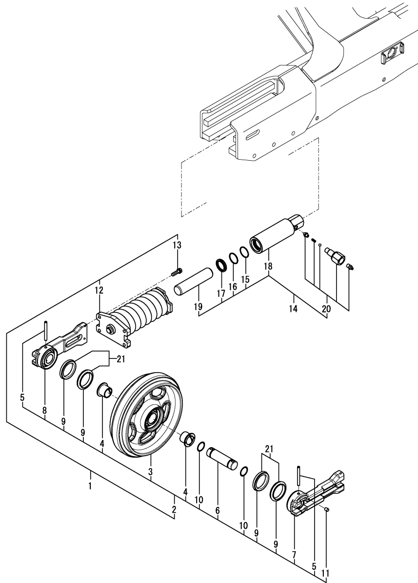
Fig.50. IDLER & ADJUST
