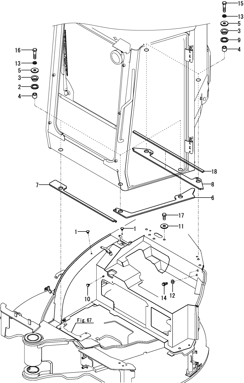
Fig.107. CABIN MOUNT
