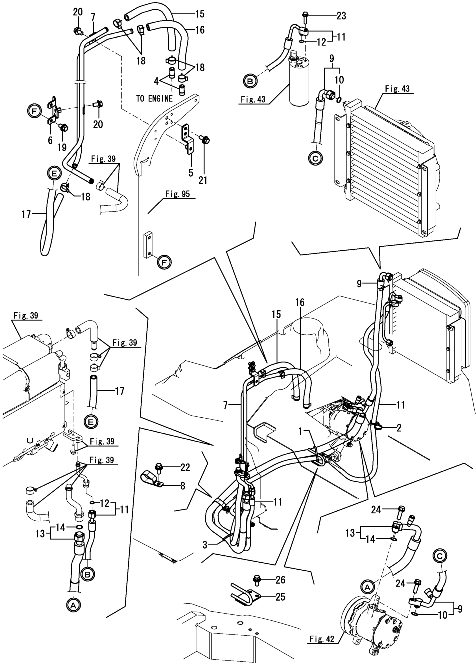
Fig.41. AIR CONDITIONER(PIPING)
