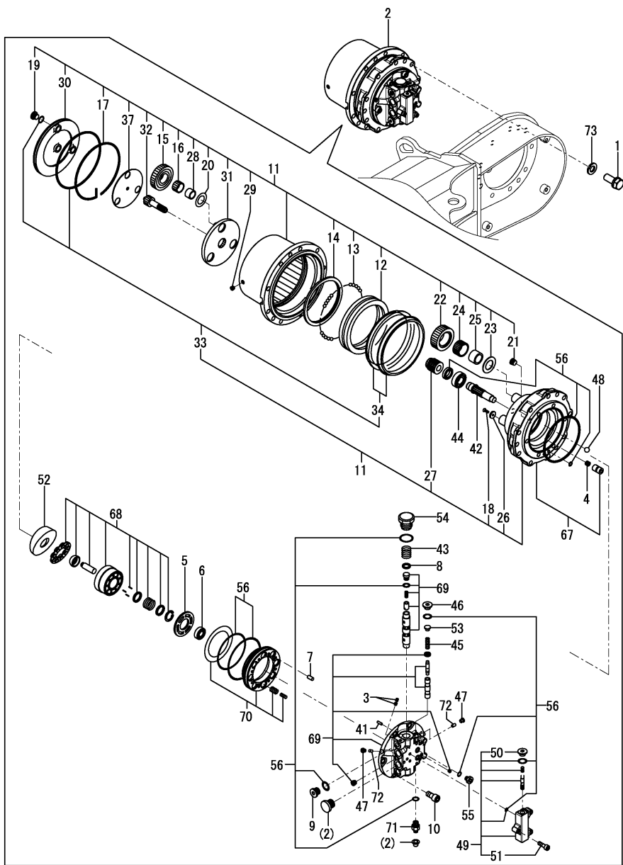
Fig.120. TRAVEL MOTOR
