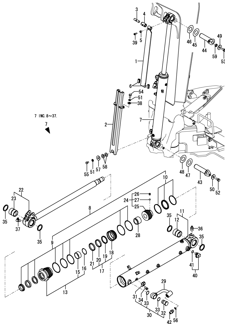
Fig.113. BOOM CYLINDER
