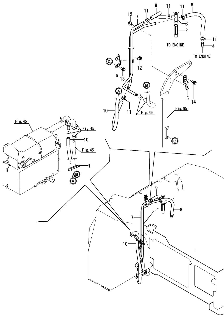
Fig.47. HEATER(PIPING)
