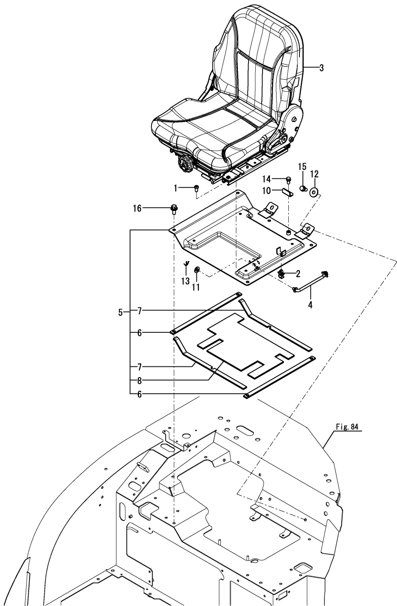
Fig.86. SEAT
