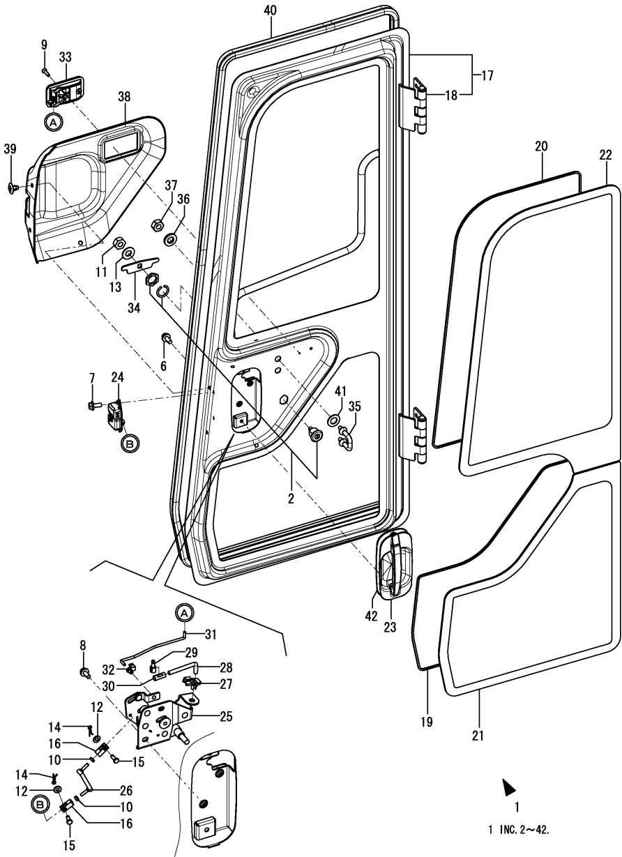
Fig.99. CABIN DOOR(2)
