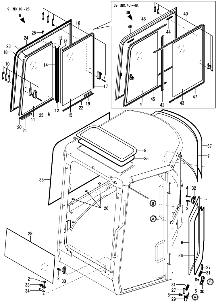
Fig.102. CABIN(GLASS)
