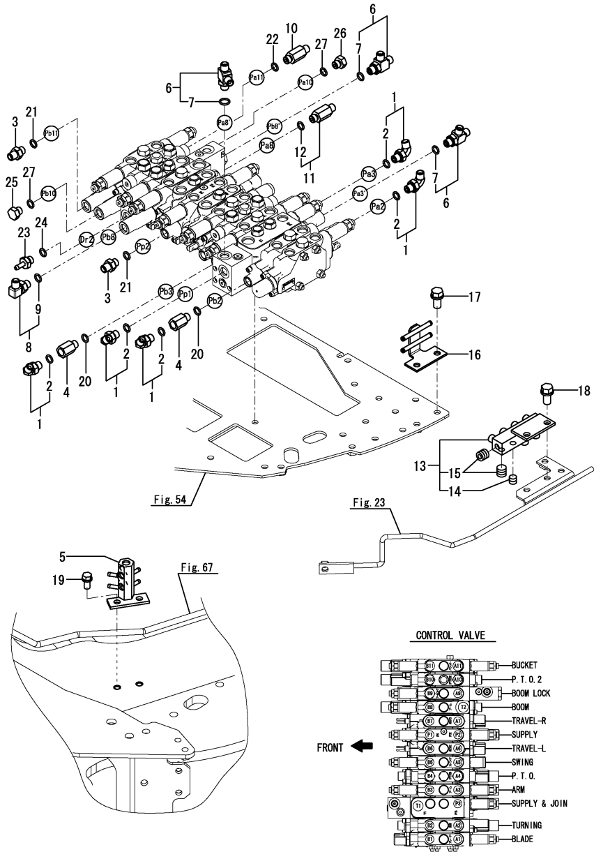
Fig.134. CONTROL VALVE(FITTING)(2)
