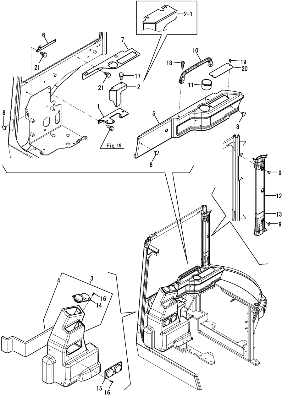
Fig.32. COVER(CABIN)(1)(TO M53273)
