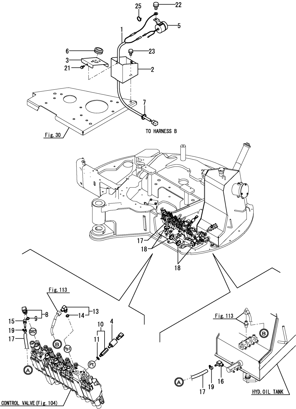
Fig.102. (13A)TRAVEL ALARM(US : FROM M58001)
