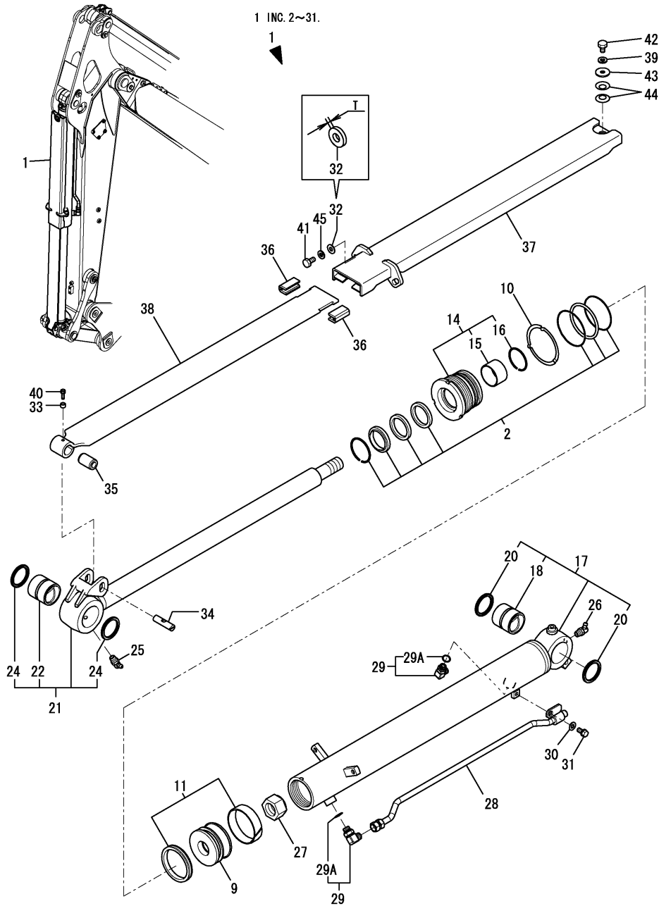
Fig.45. BUCKET CYLINDER
