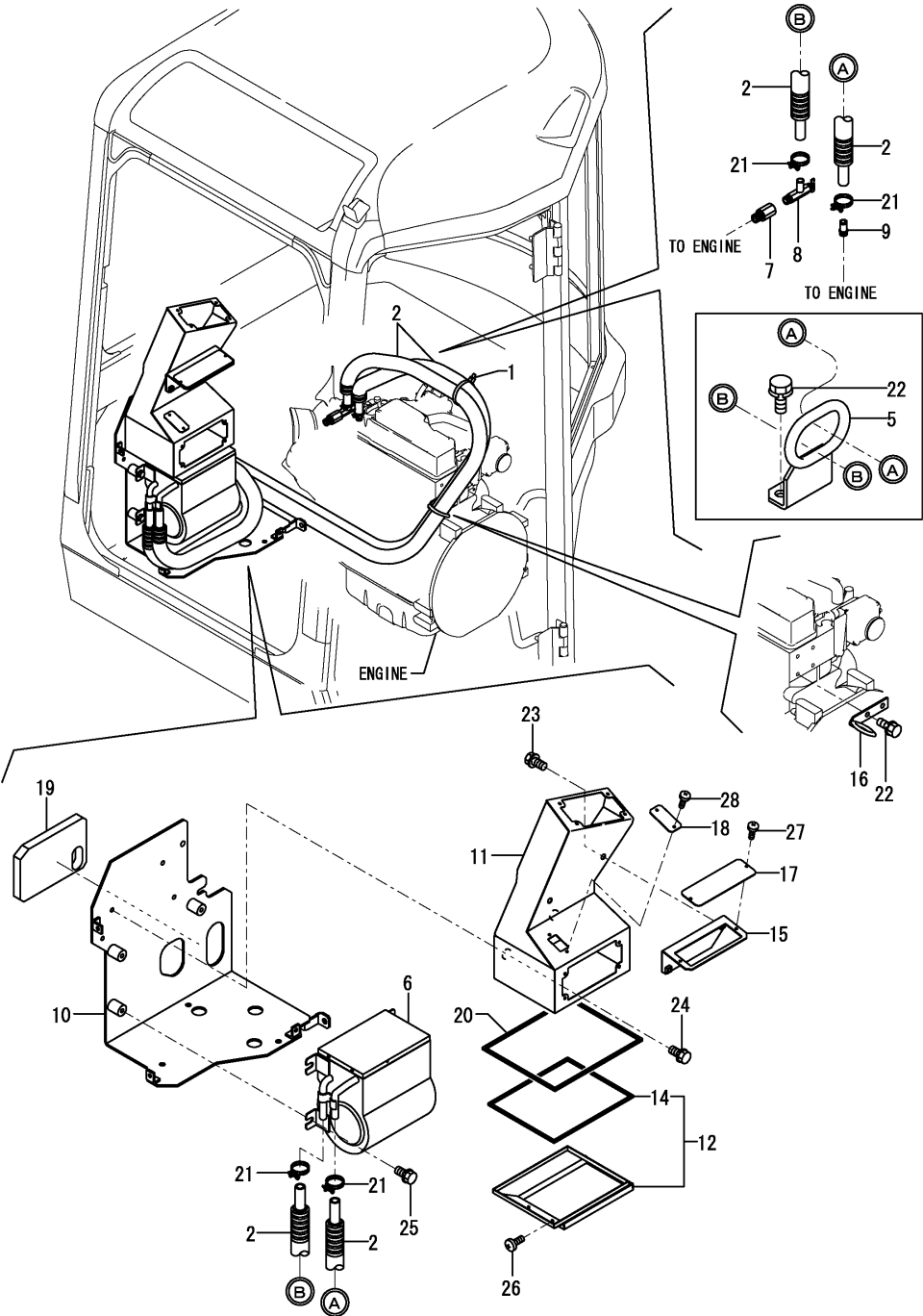
Fig.101. (15B)HEATER(FROM M53274)
