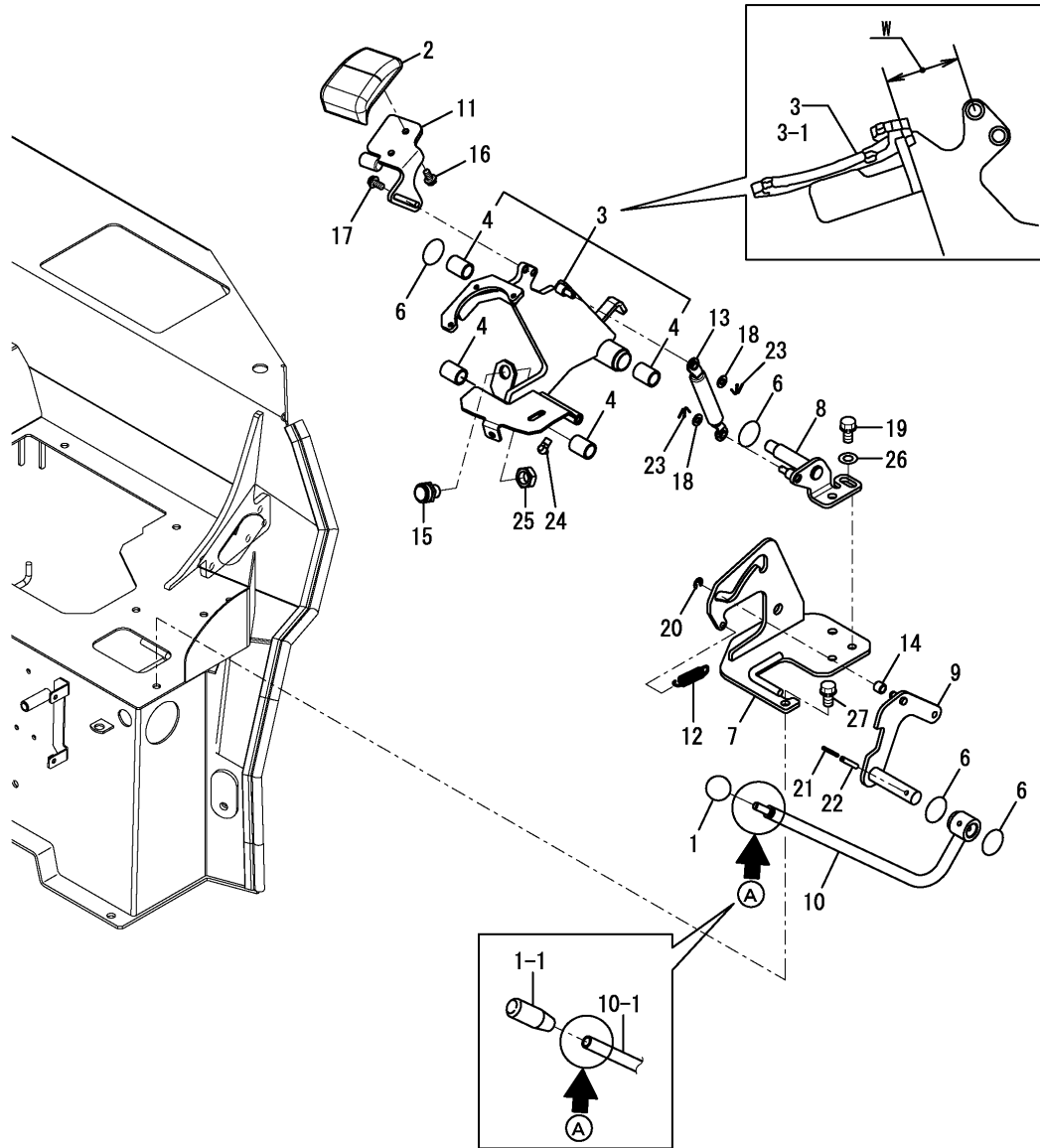
Fig.23. LOCK LEVER & STAND(LEFT)
