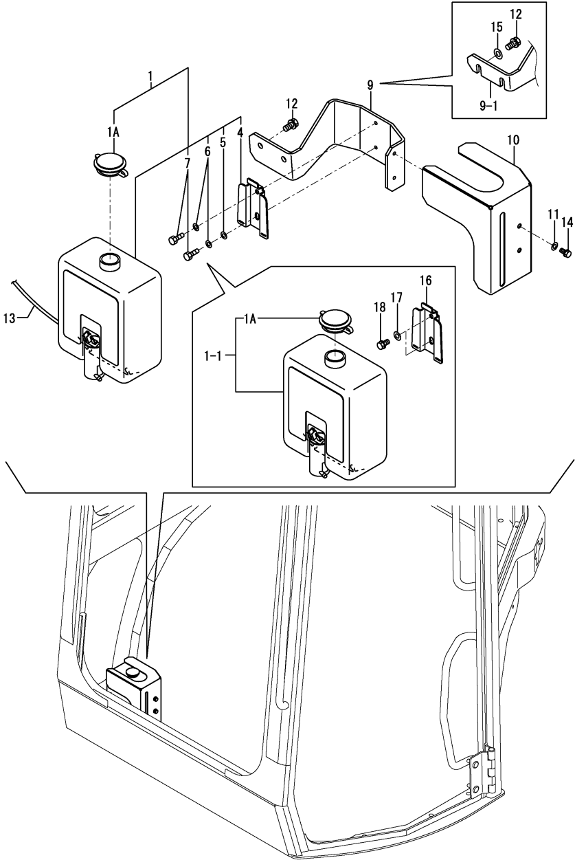
0CS10-M51801 CABIN Fig.16. WINDOW WASHER
