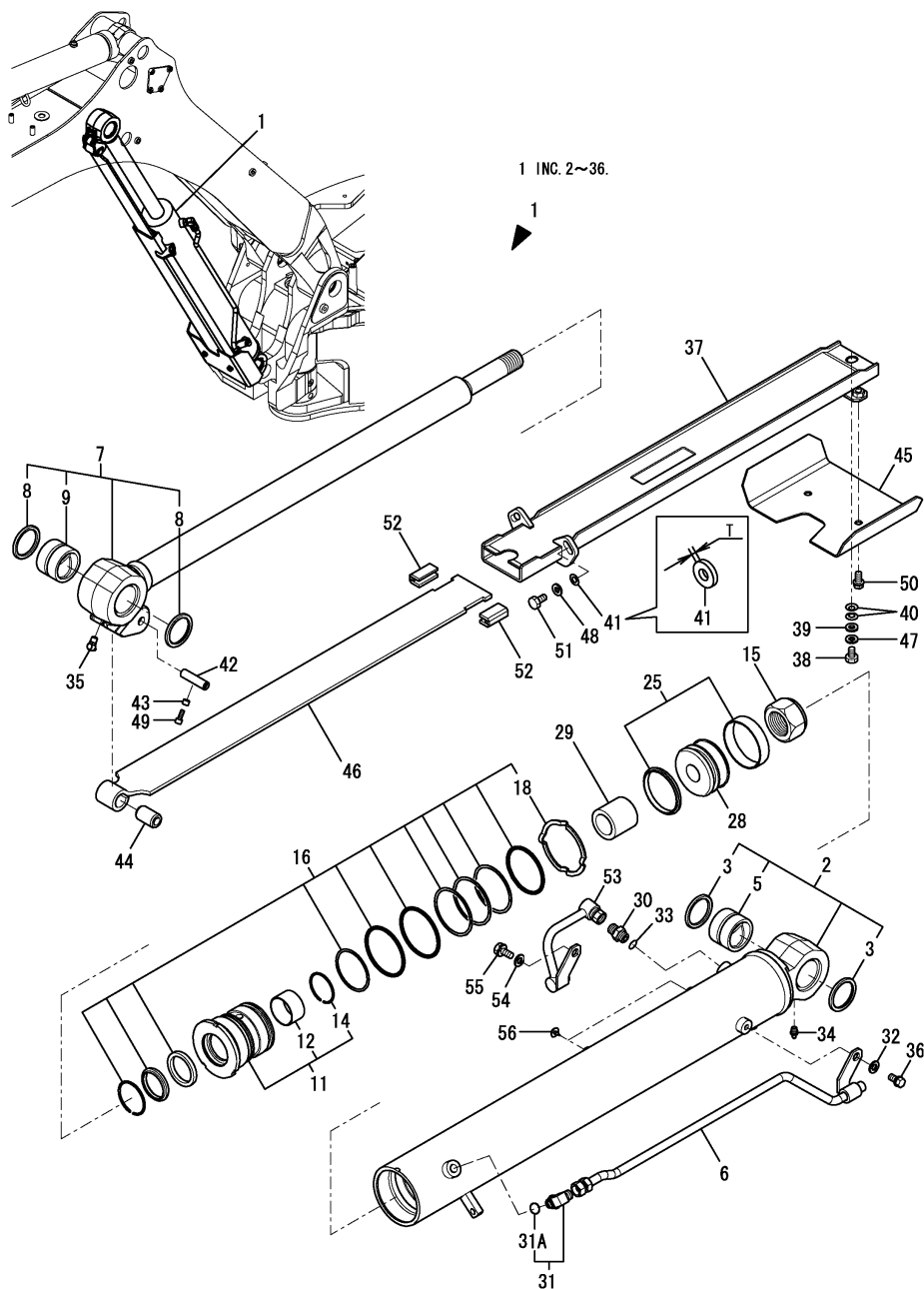
Fig.43. BOOM CYLINDER
