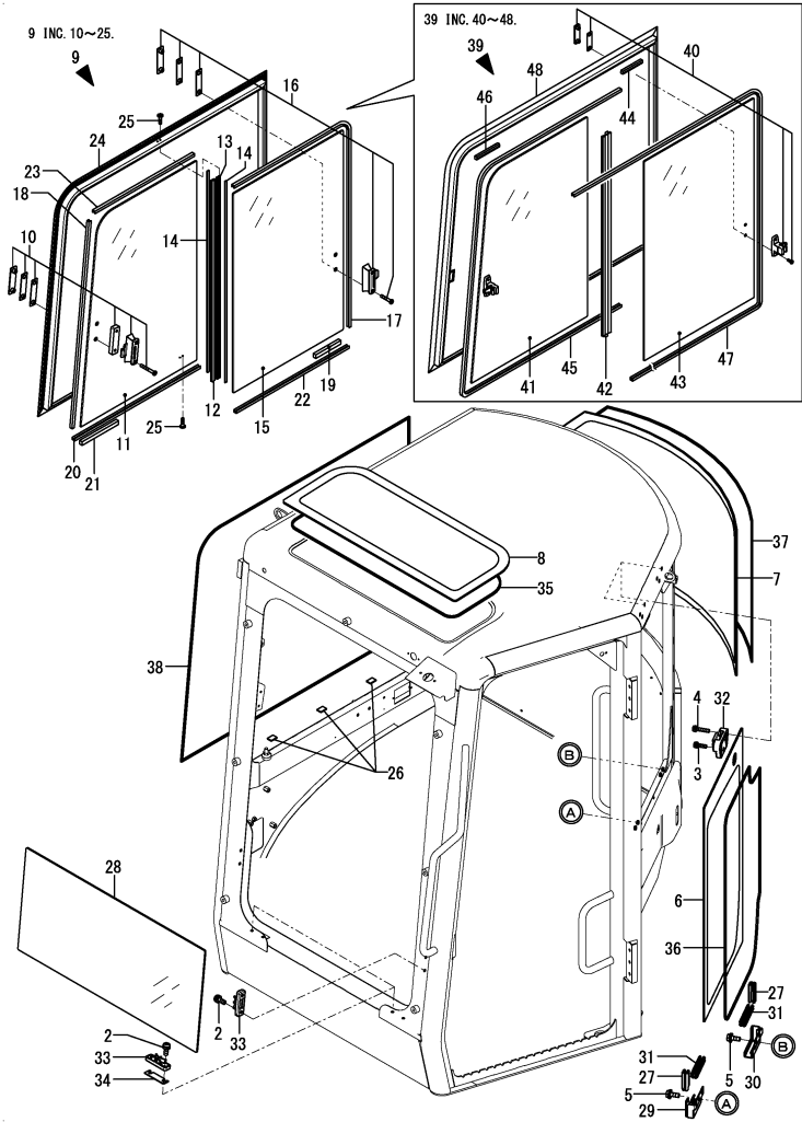
Fig.144. (80E)CABIN(GLASS)
