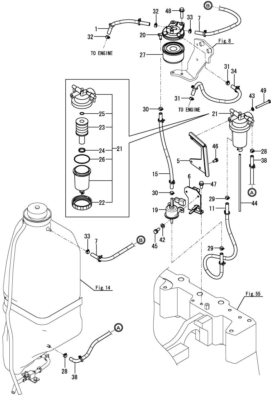
Fig.15. FUEL PIPING
