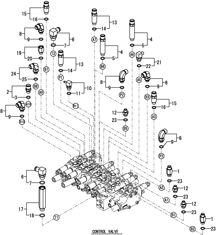
Fig.110. CONTROL VALVE(FITTING)(1)
