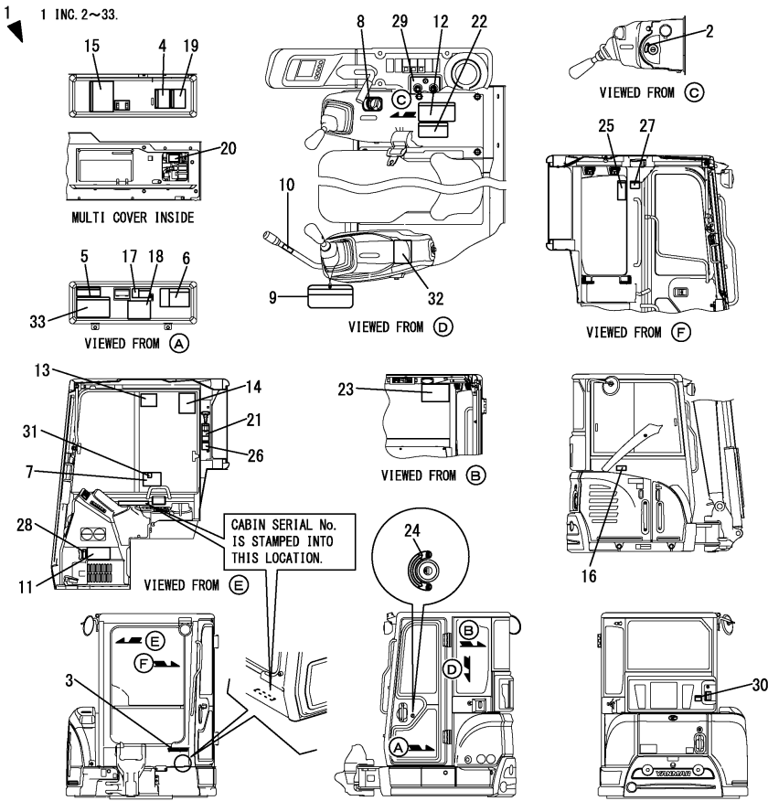
Fig.202. (4A)LABEL(CABIN)(FROM MAF001)
