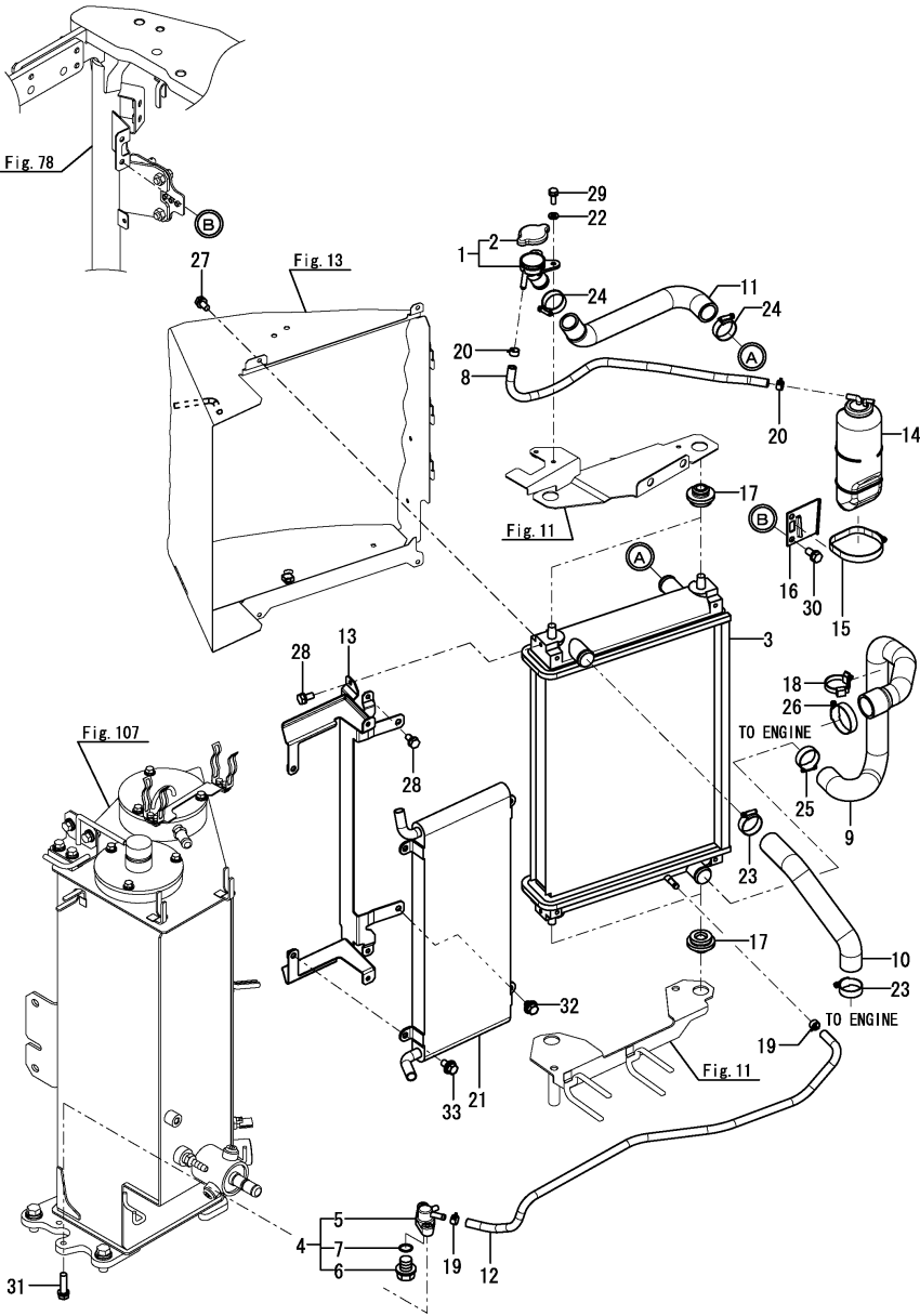
Fig.12. RADIATOR & OIL COOLER
