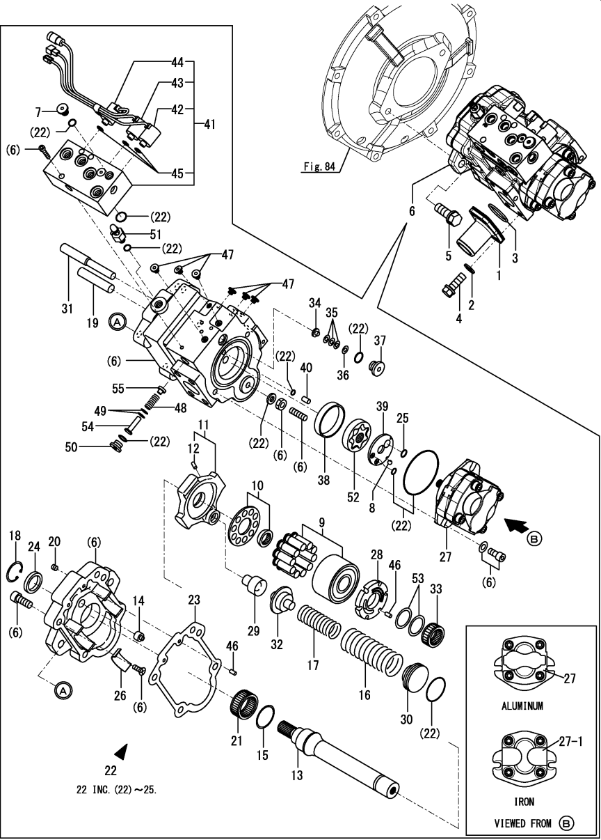
OCS10-M57800 HYDRAULIC OIL EQUIPMENT Fig.86. HYDRAULIC PUMP(ESS SPEC.)
