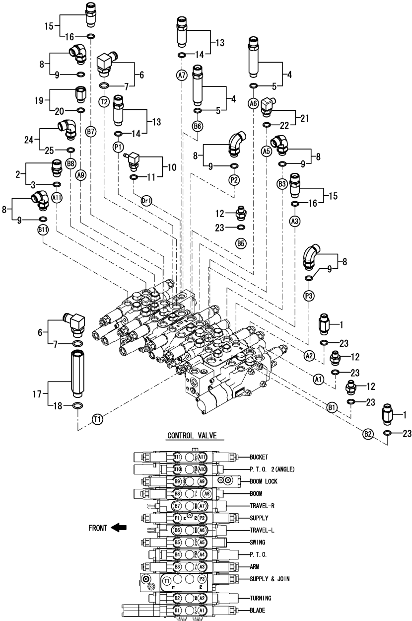
Fig.177. (110A)CONTROL VALVE(FITTING)(1)(ANGLE BLADE SPEC.)
