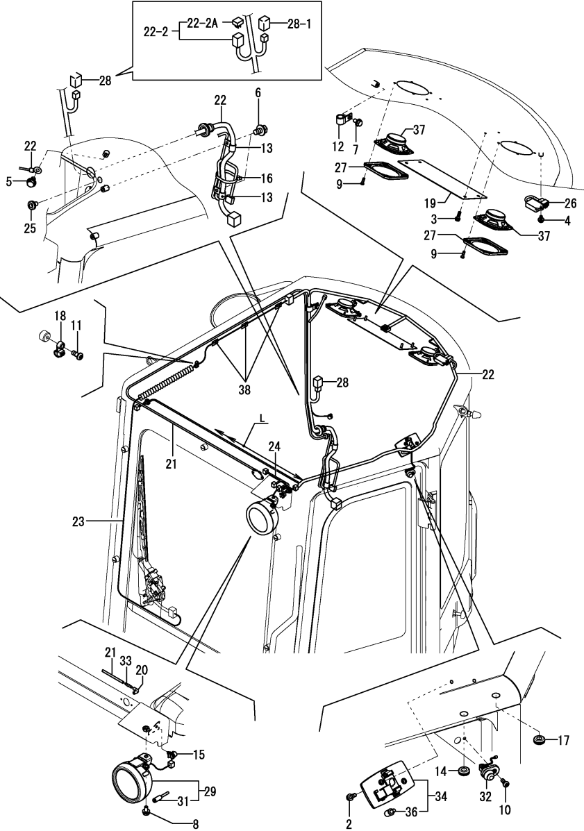
Fig.146. (80G)CABIN(ELECTRIC PARTS)
