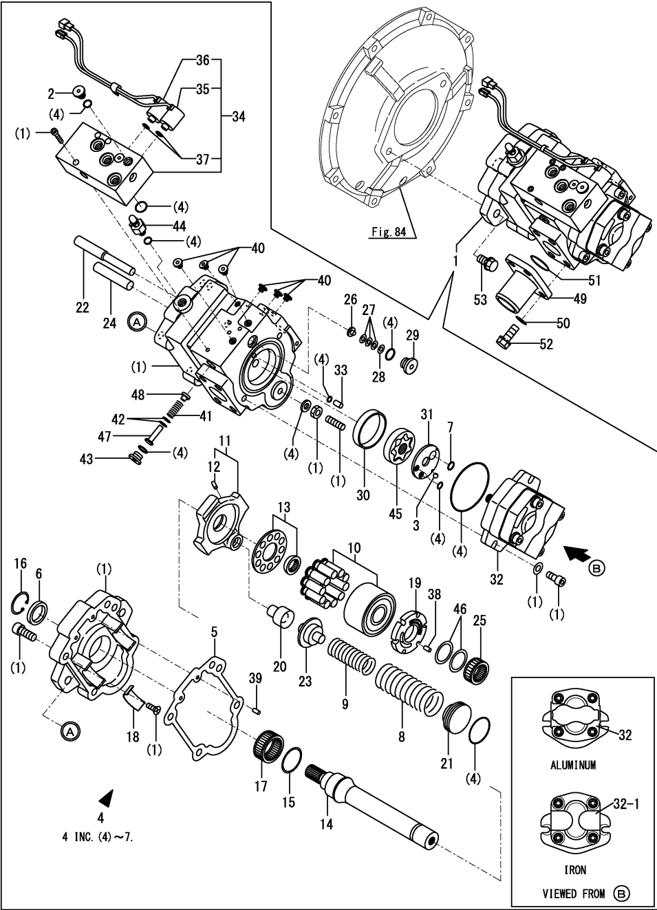
Fig.160. (86A)HYDRAULIC PUMP(STANDARD SPEC.)
