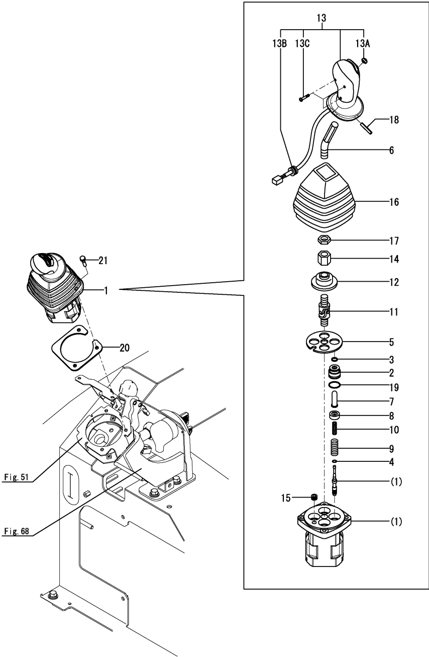
Fig.102. REMOTE CONTROL VALVE(RIGHT)
