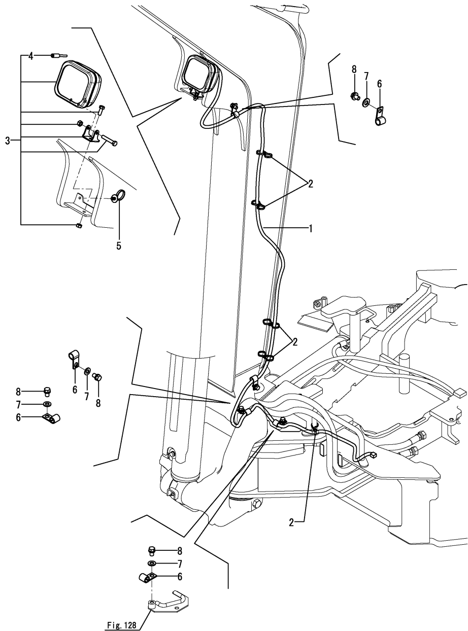
Fig.26. WORK LAMP
