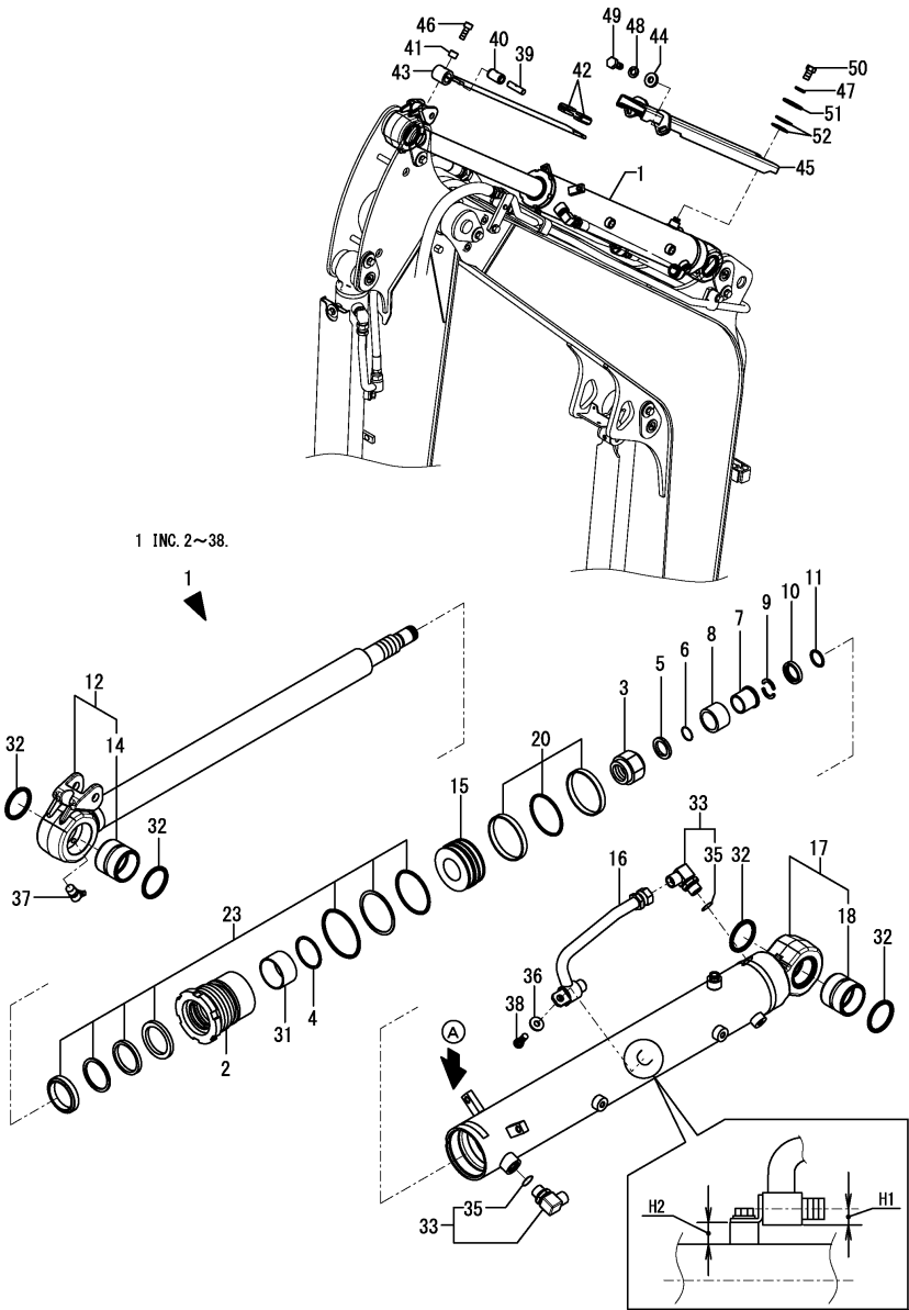
Fig.196. (88C)ARM CYLINDER(STANDARD SPEC.)(K SPEC.)
