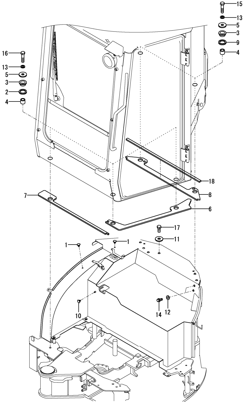
Fig.82. MOUNT(CABIN)
