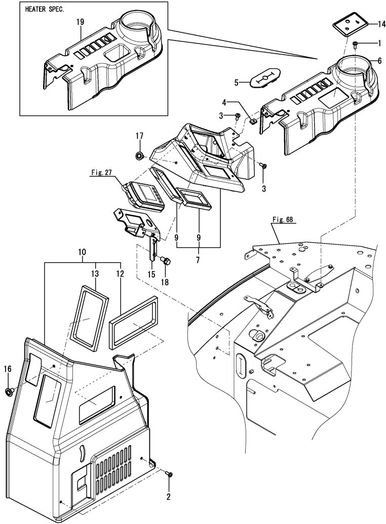
Fig.67. COVER(MONITOR)(CABIN)
