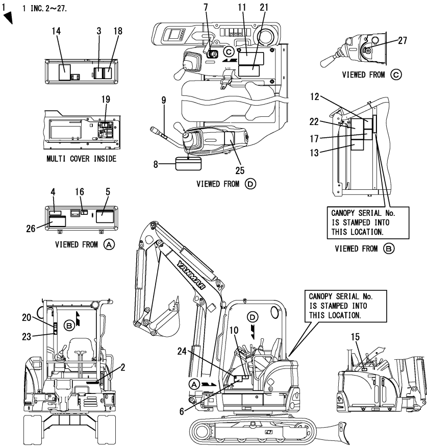
Fig.200. (3A)LABEL(CANOPY)(FROM MAF001)
