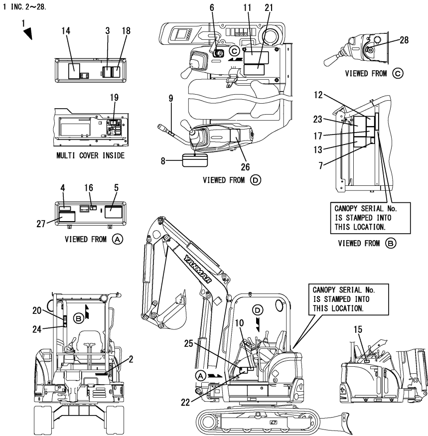
Fig.201. (3C)LABEL(CANOPY)(ANGLE BLADE SPEC.)(FROM MAF001)
