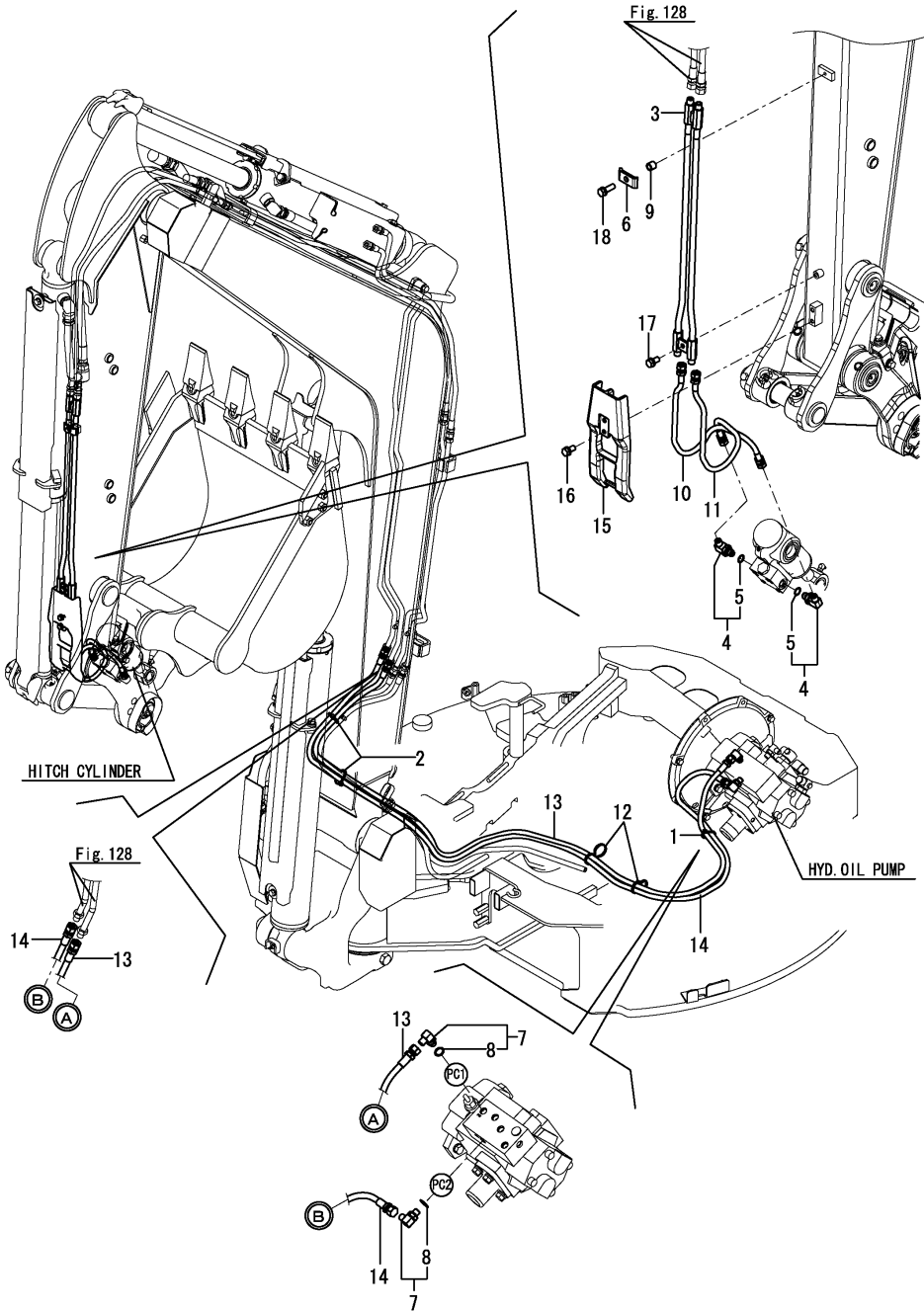
Fig.127. QUICK COUPLER(HYD. OIL PIPING)(1)
