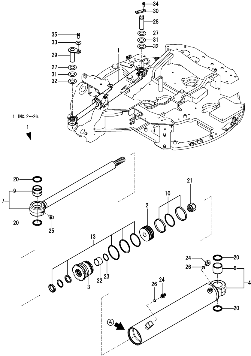
OCS10-M57800 HYDRAULIC OIL EQUIPMENT Fig.194. (90A)SWING CYLINDER(K SPEC.)
