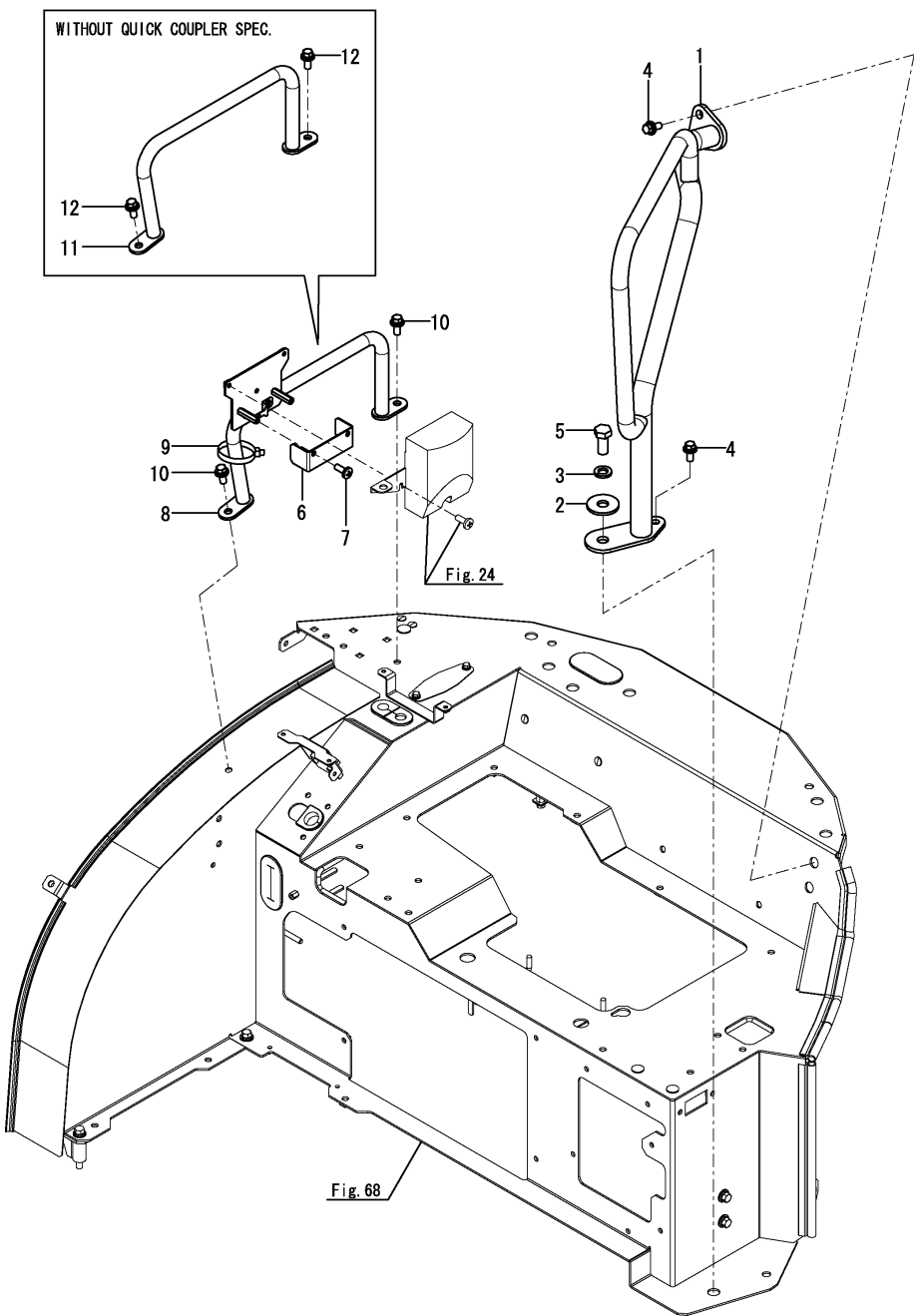
Fig.72. HANDRAIL
