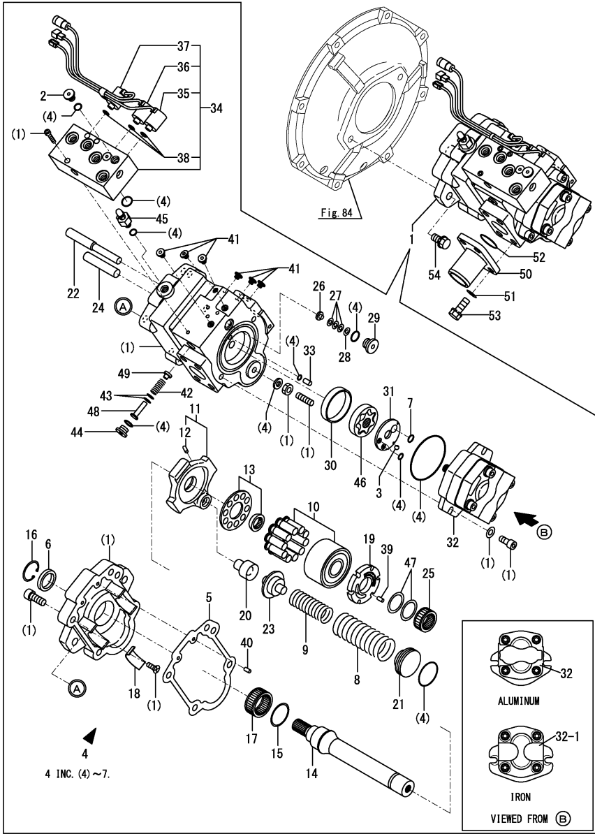
Fig.85. HYDRAULIC PUMP(QUICK COUPLER SPEC.)
