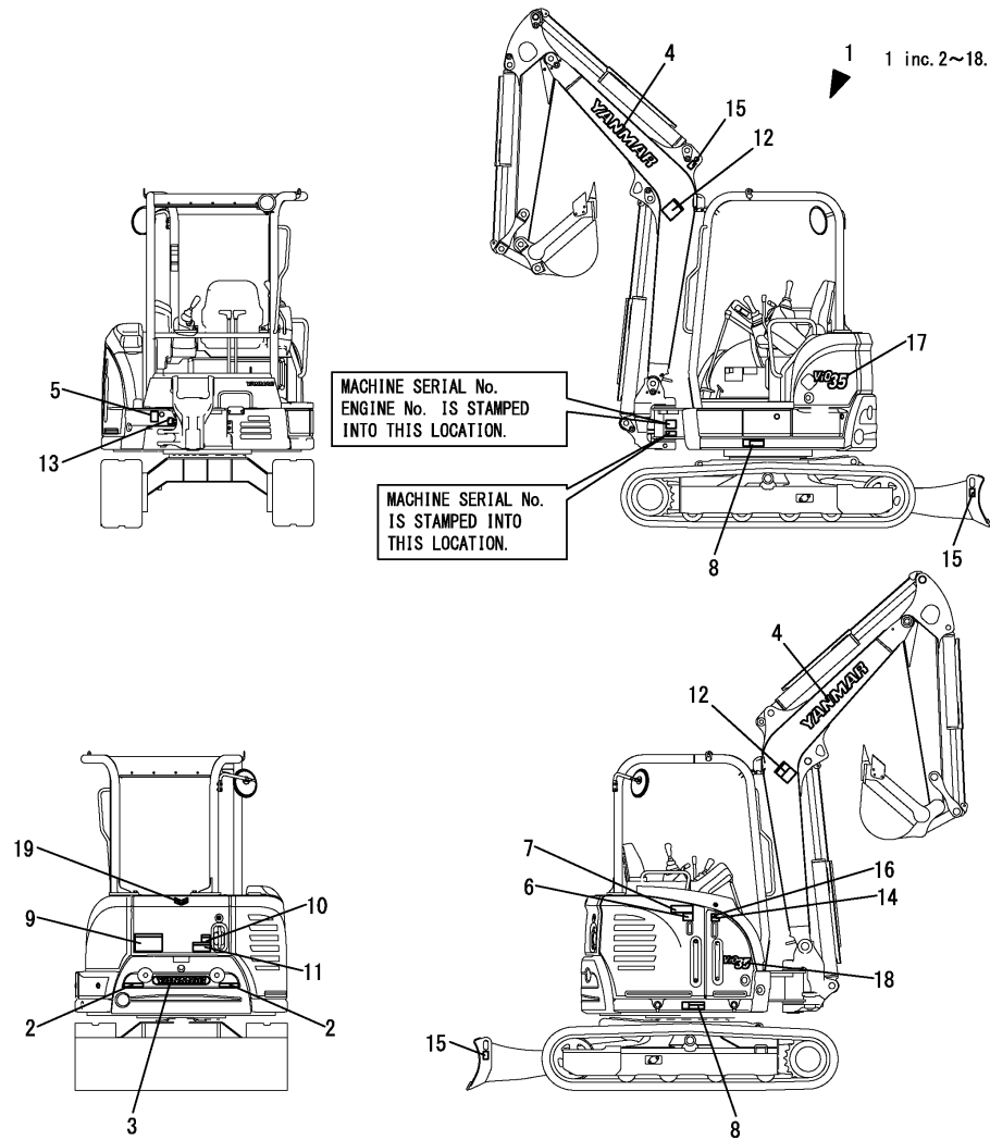
Fig.199. (1A)LABEL(EXTERIOR)(FROM MAF001)
