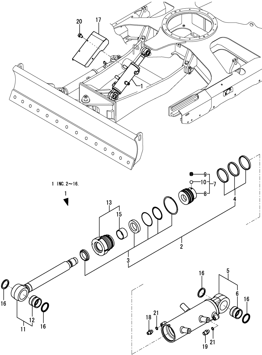
Fig.162. (91B)BLADE CYLINDER(ANGLE BLADE SPEC.)
