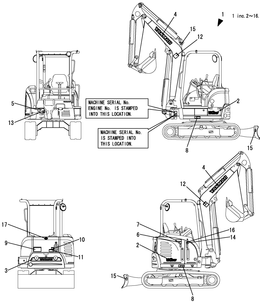
Fig.1. LABEL(EXTERIOR)(TO MAF000)
