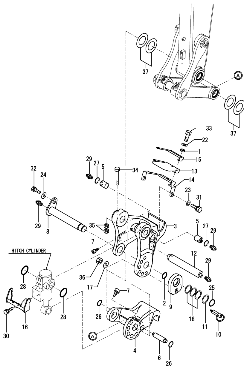
Fig.129. QUICK COUPLER(BODY)
