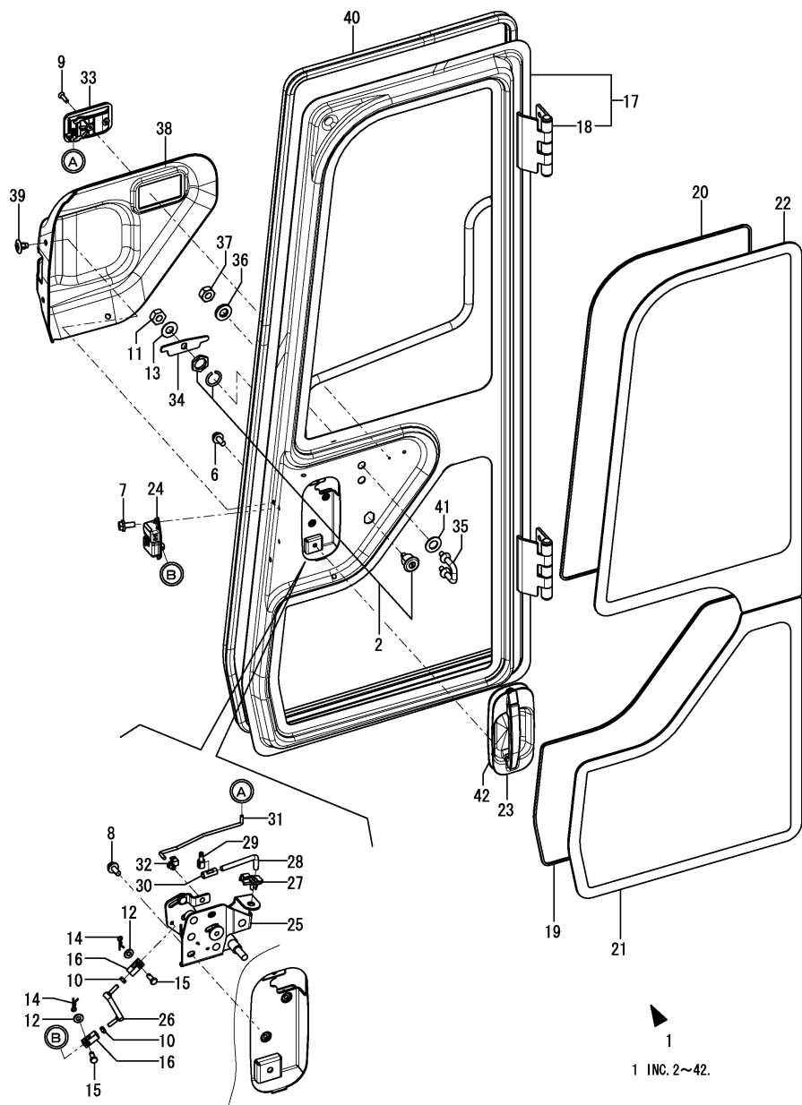
Fig.141. (80B)CABIN(DOOR)(2)
