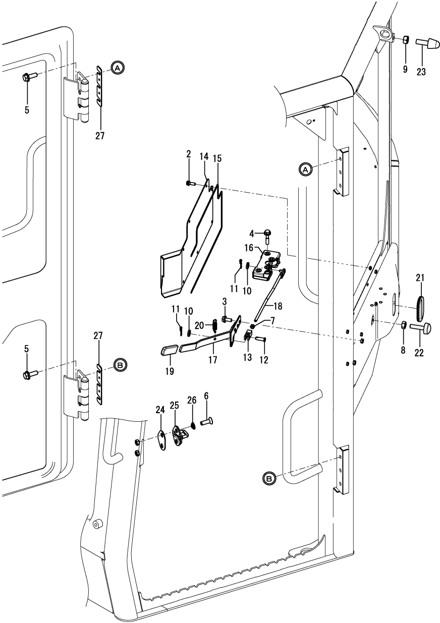
Fig.140. (80A)CABIN(DOOR)(1)
