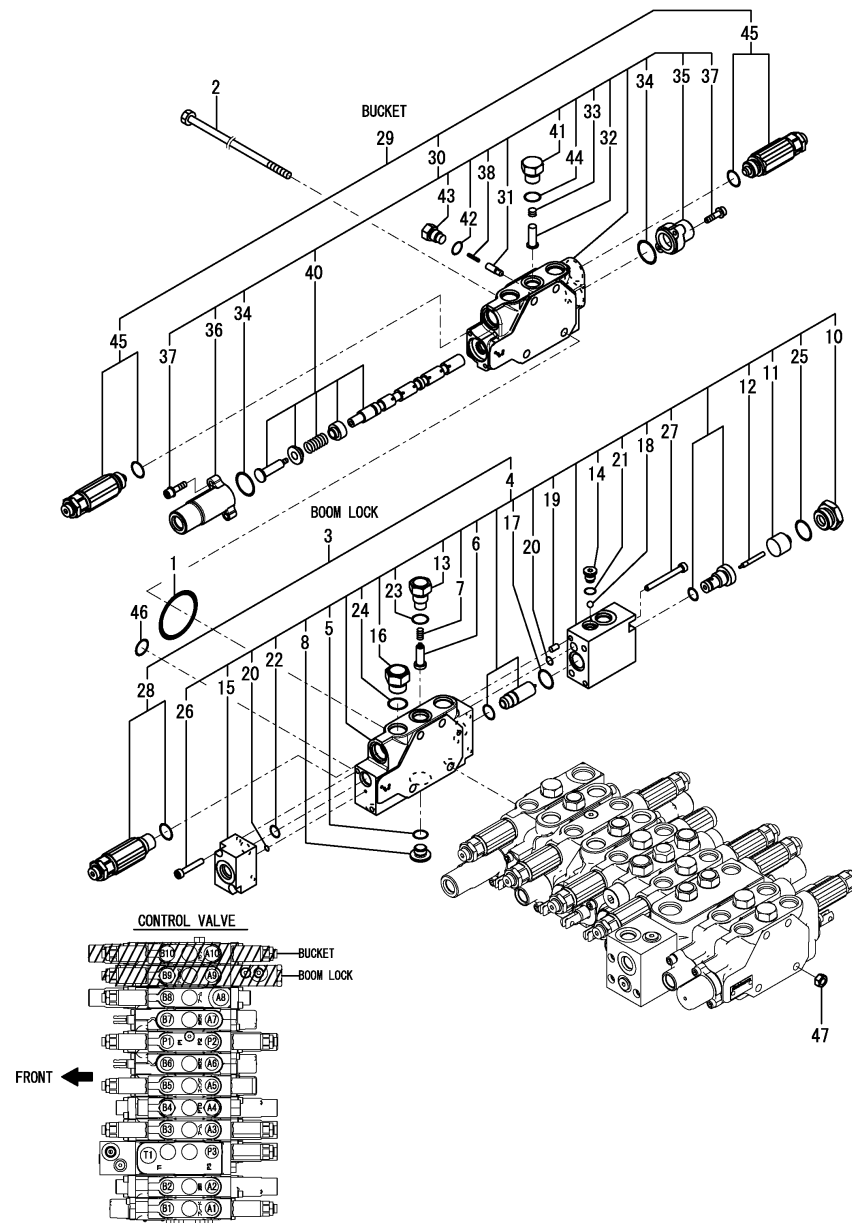
Fig.96. CONTROL VALVE(2/7)
