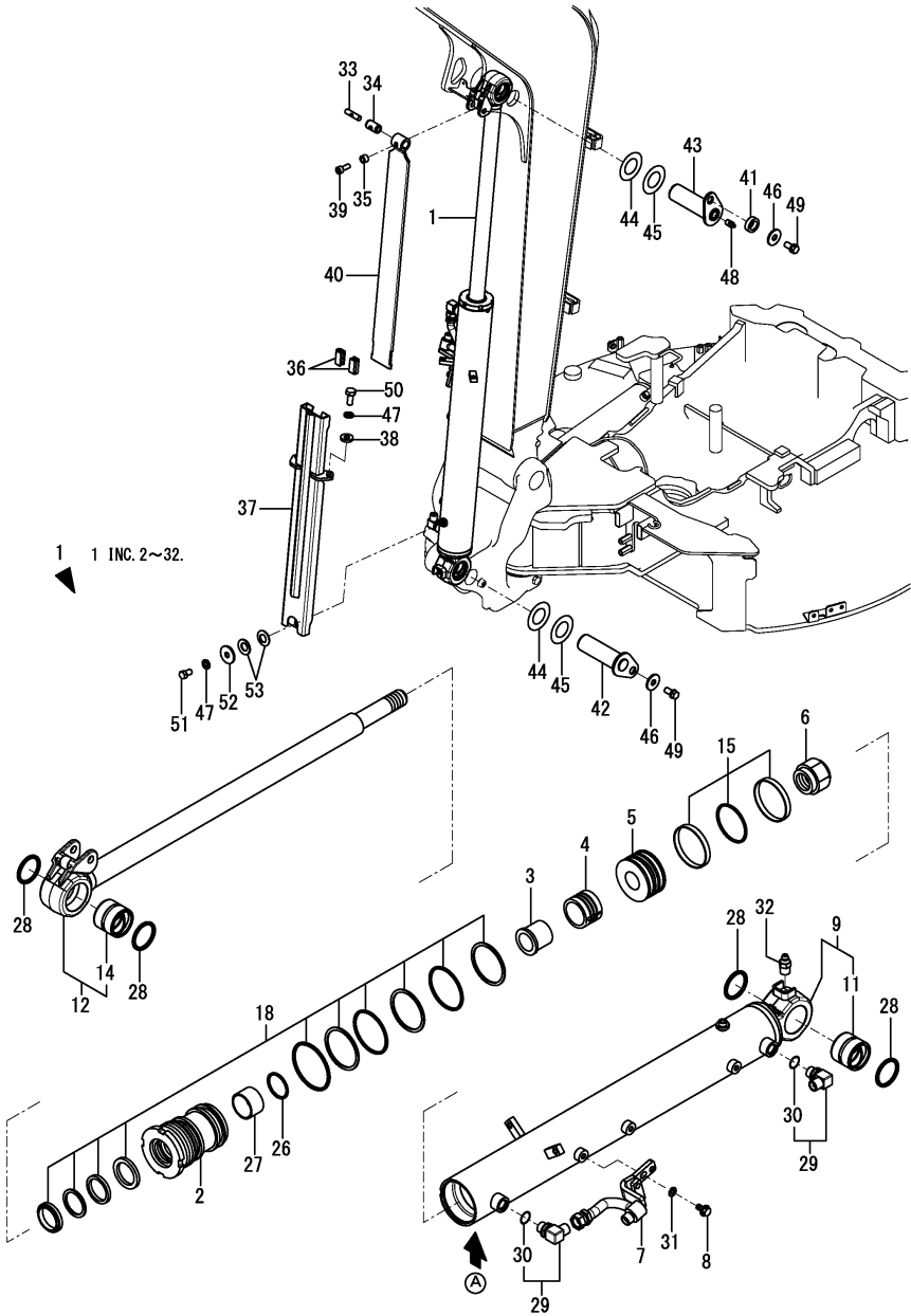
Fig.191. (87A)BOOM CYLINDER(K SPEC.)
