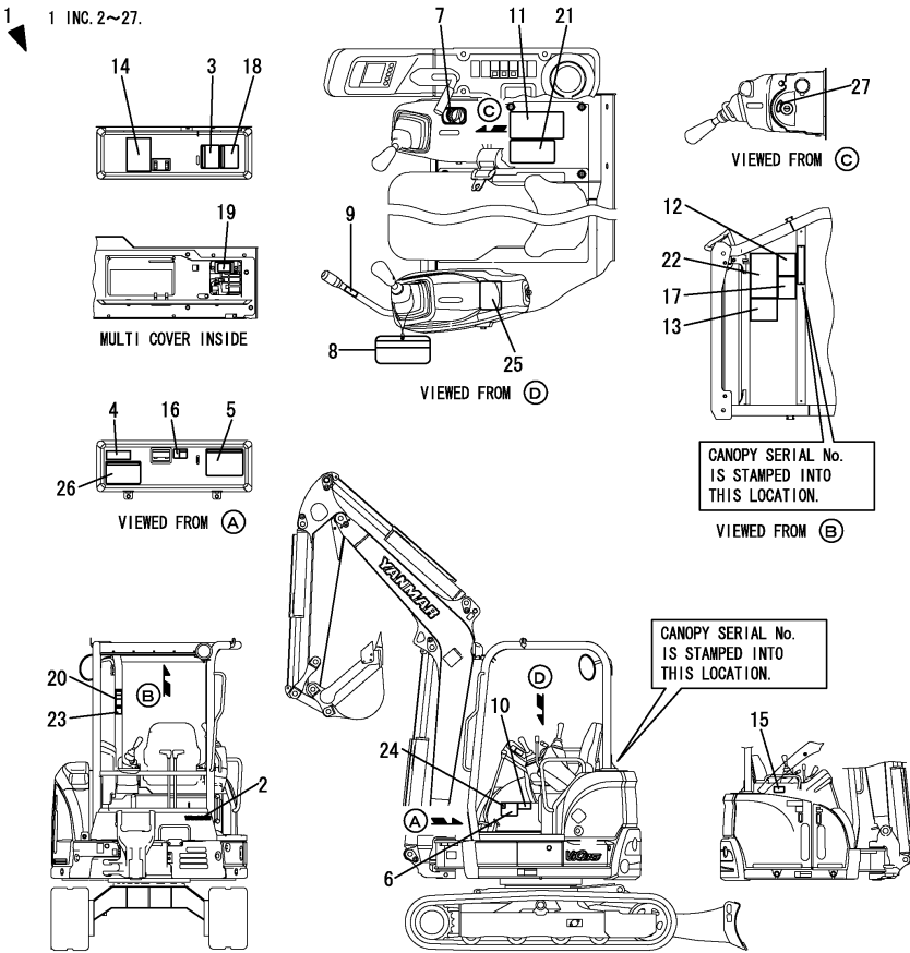
Fig.3. LABEL(CANOPY)(TO MAF000)
