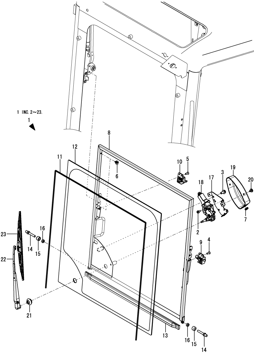
Fig.143. (80D)CABIN(FRONT WINDOW)(2)
