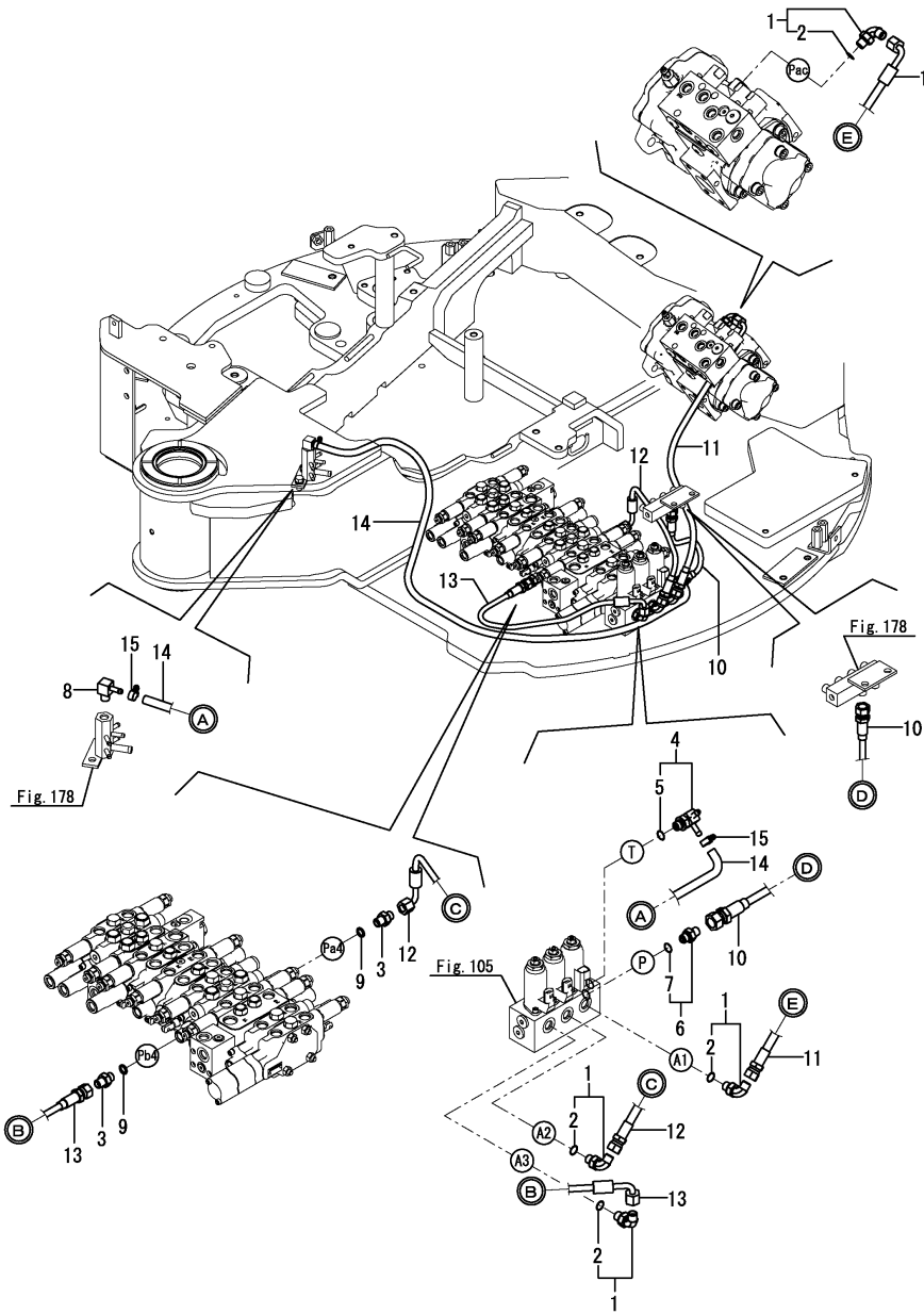
Fig.182. (121A)P.T.O.(SOLENOID VAVLE, ESS)(ANGLE BLADE SPEC.)
