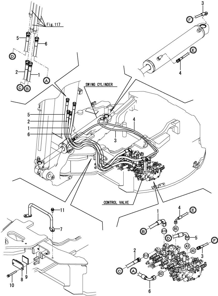
Fig.113. CONTROL VALVE - BOOM BULKHEAD & SWING
