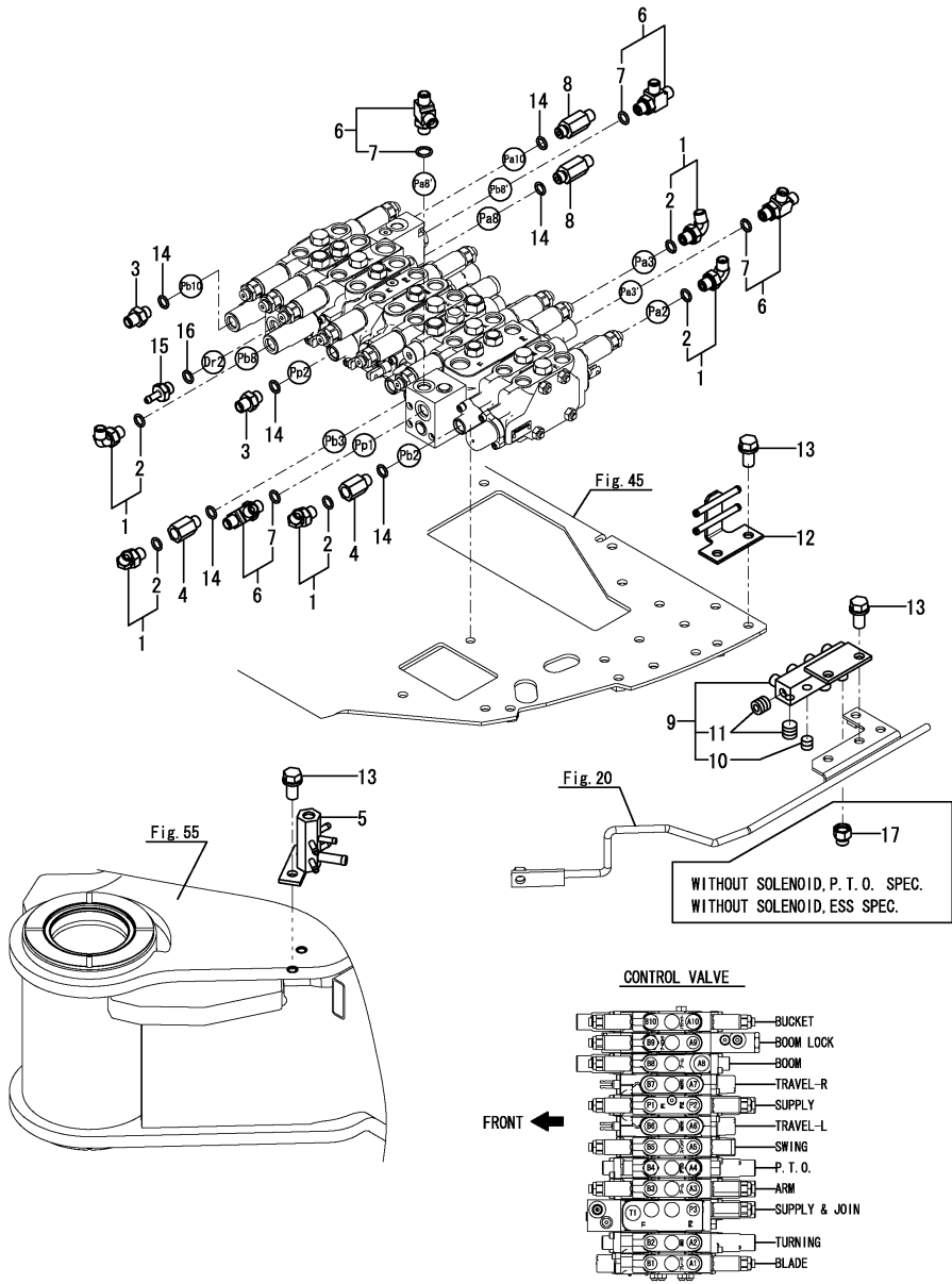
Fig.111. CONTROL VALVE(FITTING)(2)
