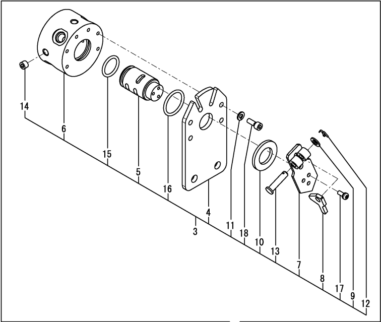
Fig.104. 2-WAY VALVE
