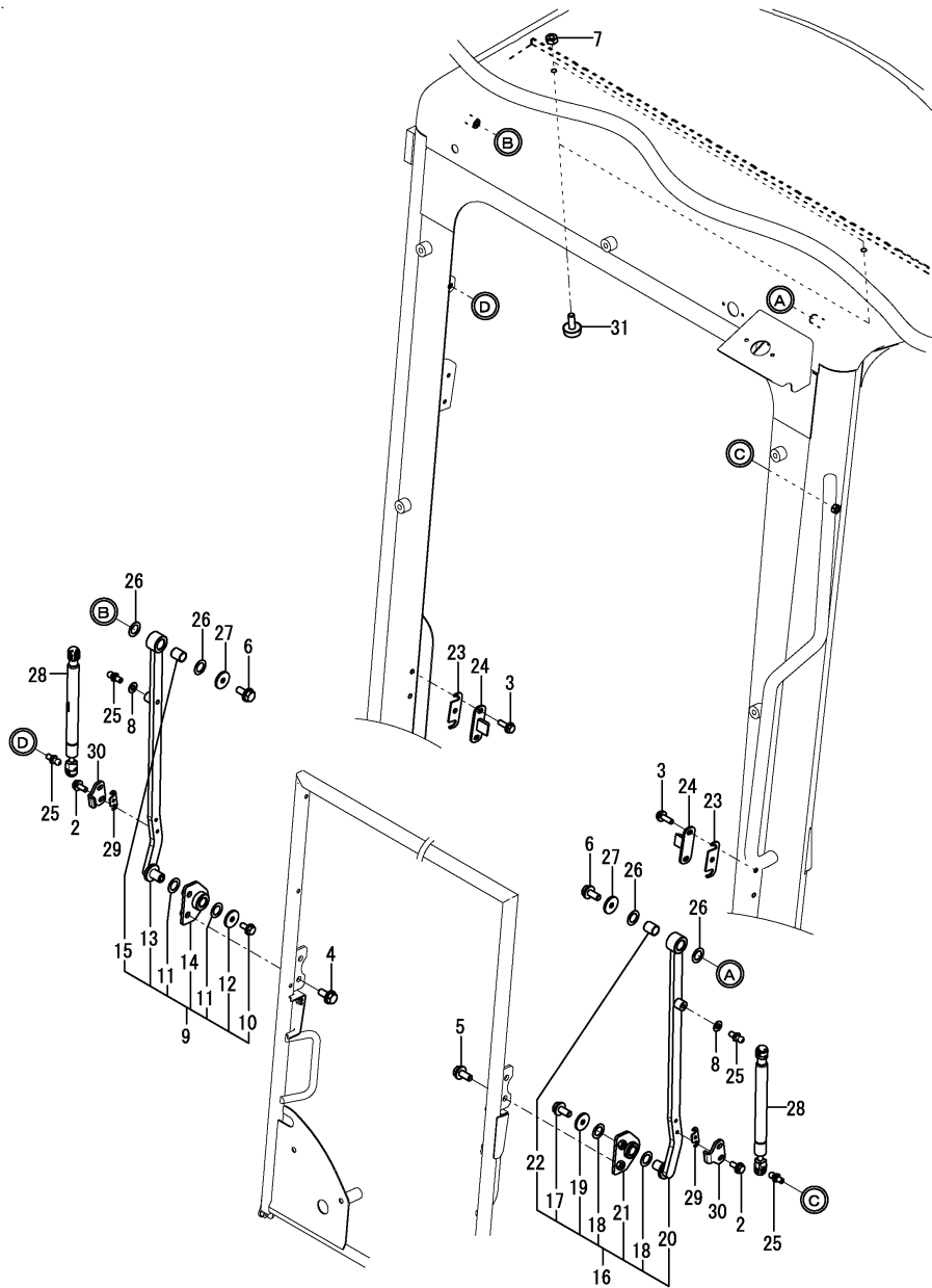
Fig.142. (80C)CABIN(FRONT WINDOW)(1)
