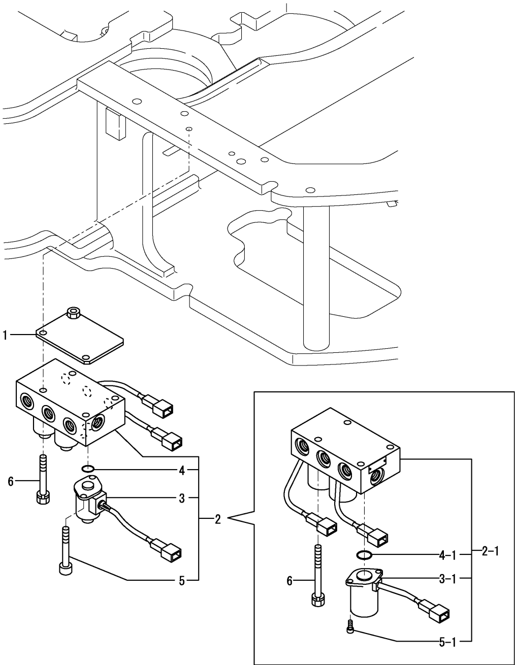
Fig.91. SOLENOID VALVE(CRANE SPEC.)
