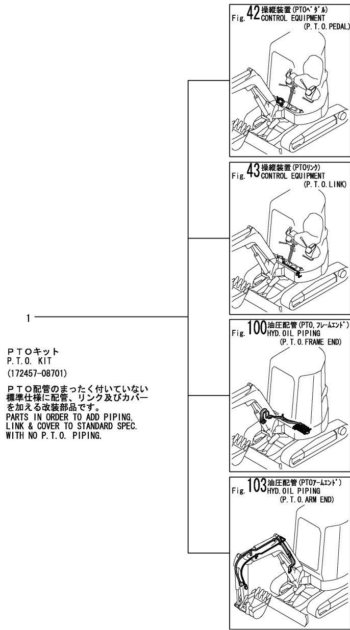
Fig.129. P.T.O. KIT (OPTIONAL)
