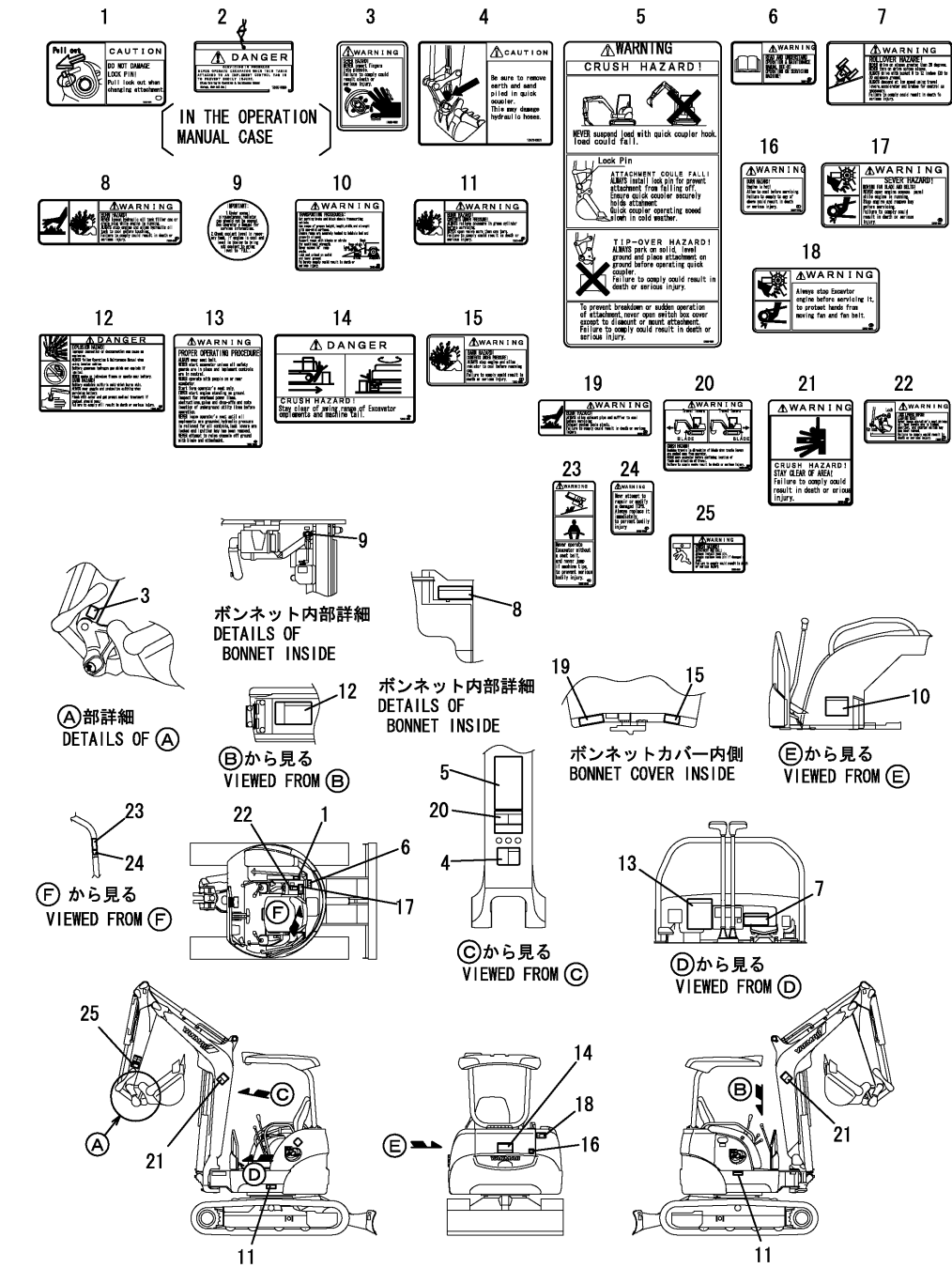
Fig.8. SAFETY LABEL(CANOPY : EX)
