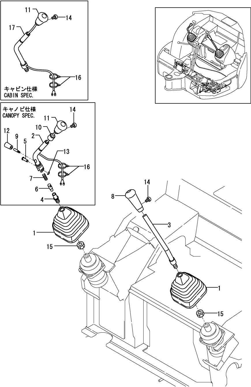
Fig.38. CONTROL EQUIPMENT(OPERATION LEVER)
