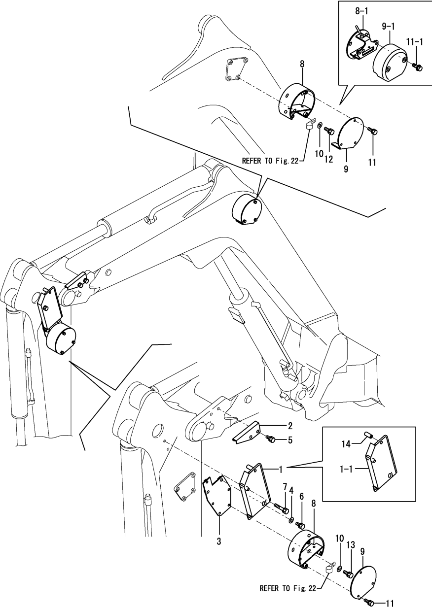
OCK10-M39802 COVER Fig.52. COVER(CRANE)
