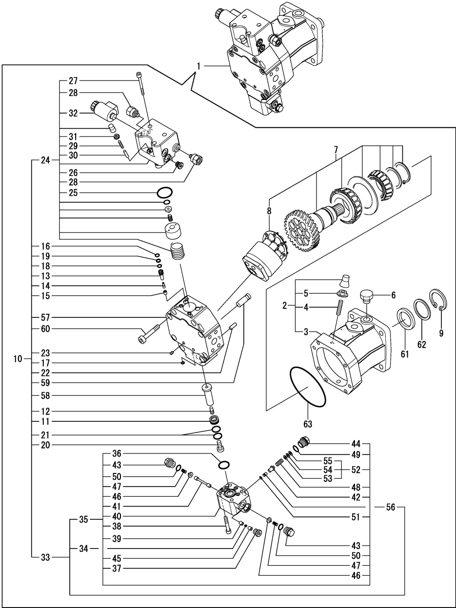
Fig.71. HST MOTOR(COMPONENT PART)
