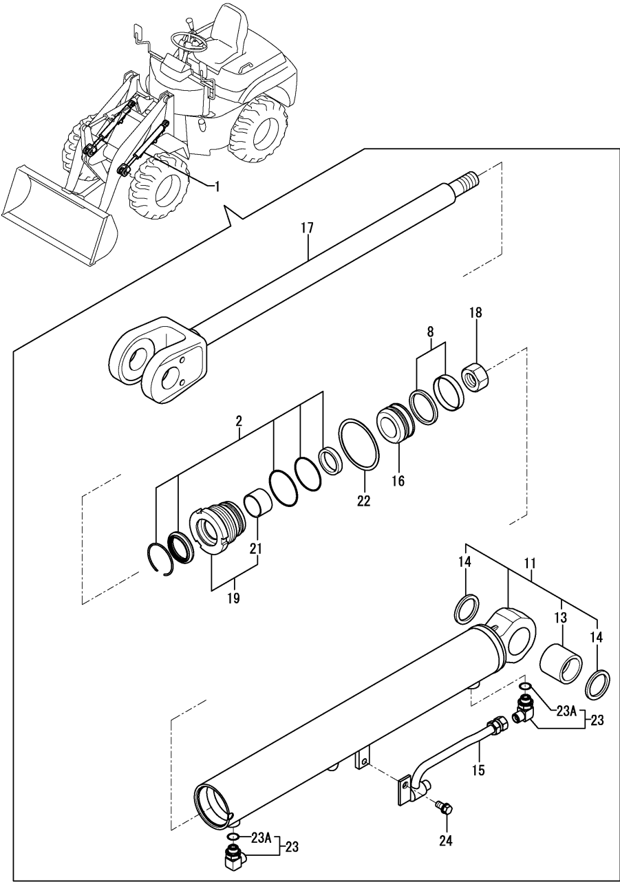
Fig.47. LIFT CYLINDER
