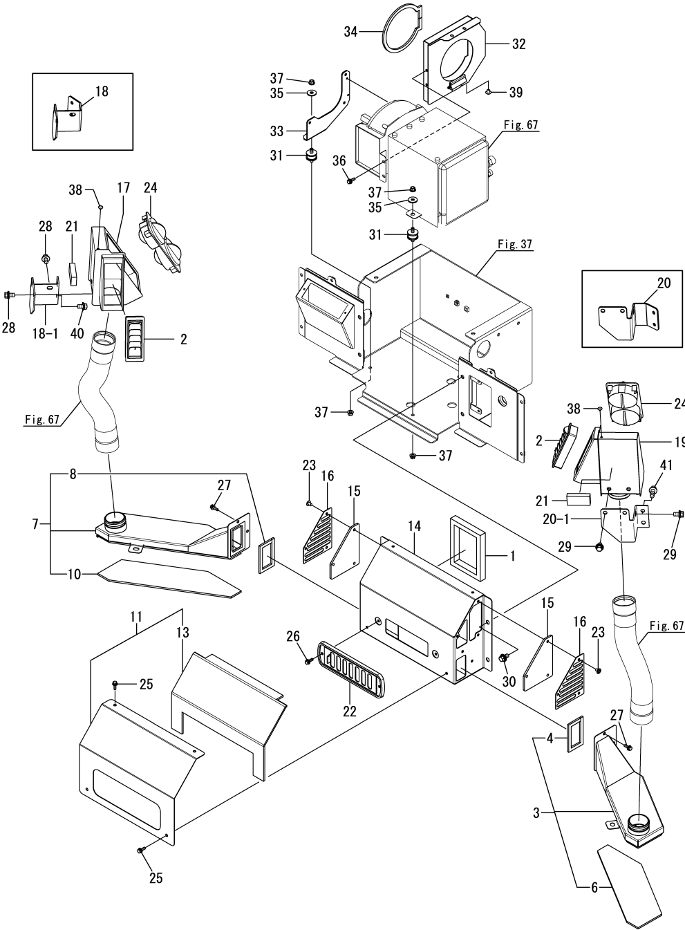
Fig.78. (65A)AIR CON.(DUCT)(ENHANCED DEFROSTER SPEC.)
