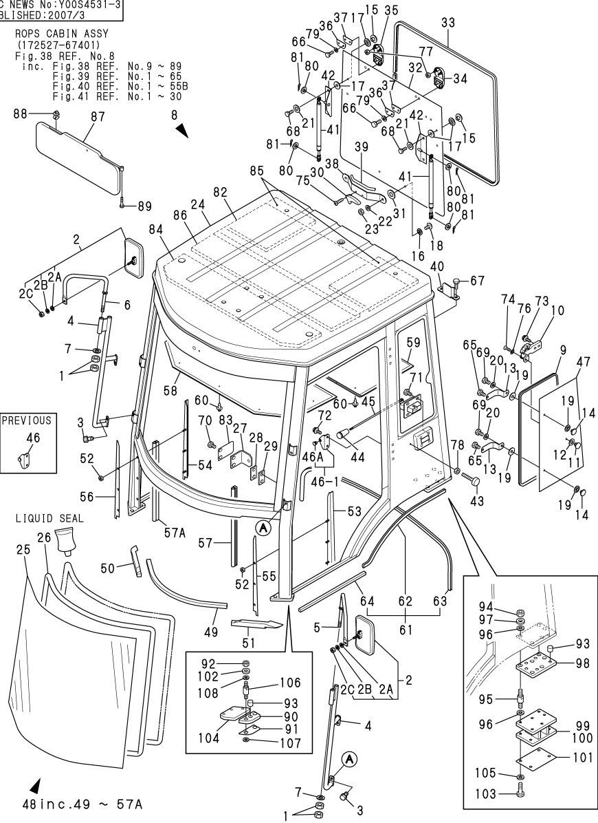
Fig.38. ROPS CABIN
