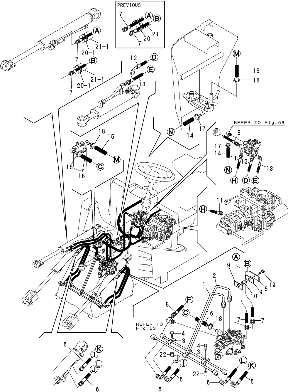
Fig.56. HYD.OIL PIPING(LOADER)
