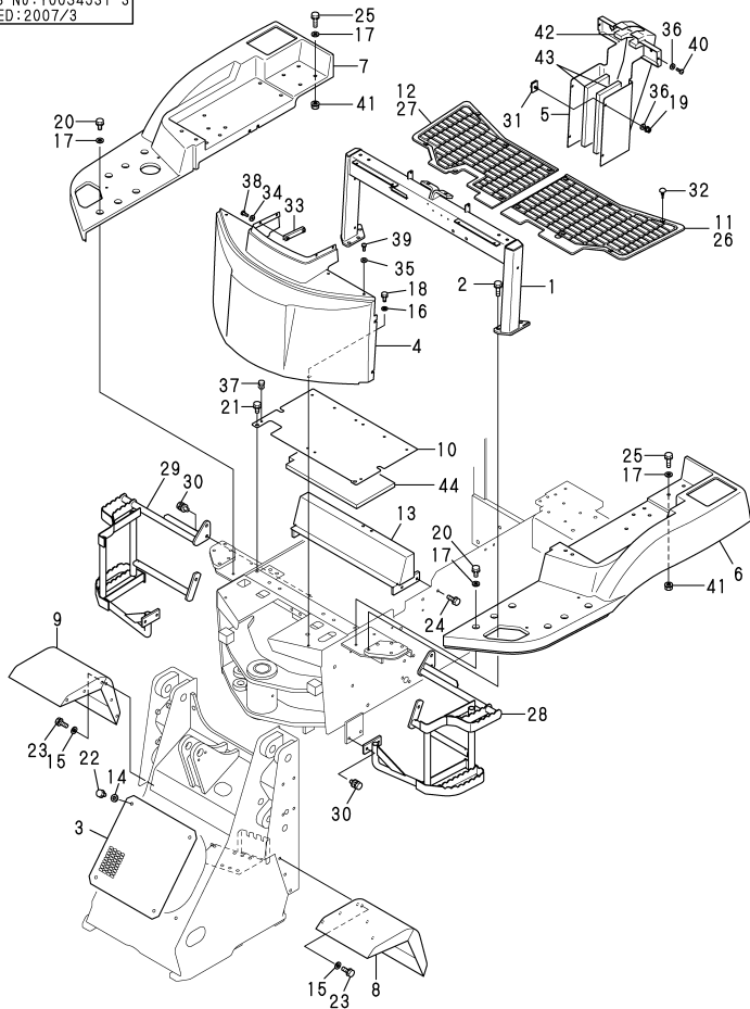
Fig.33. OPERATION FRAME & COVER
