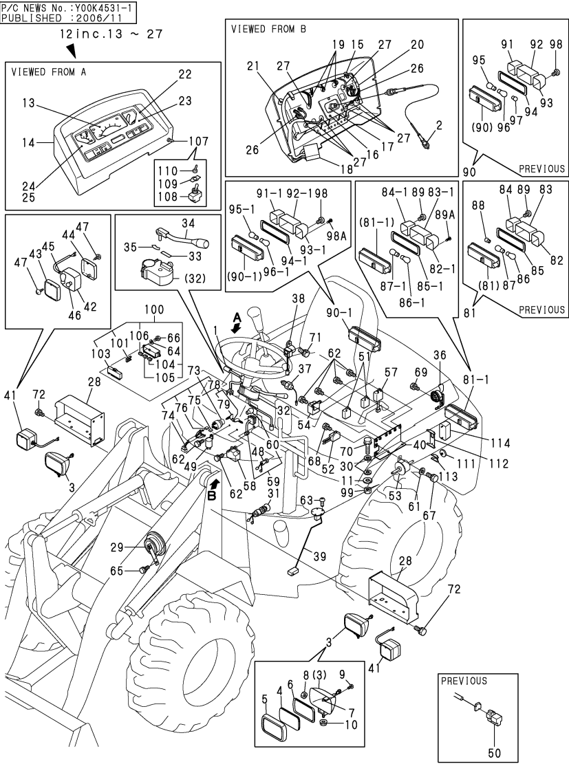
Fig.11. ELECTRIC PART
