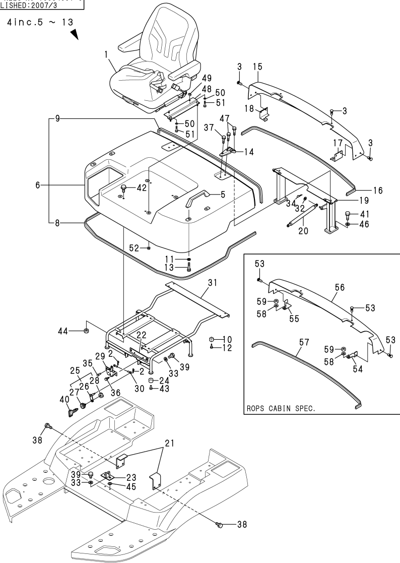
Fig.34. SEAT & BONNET
