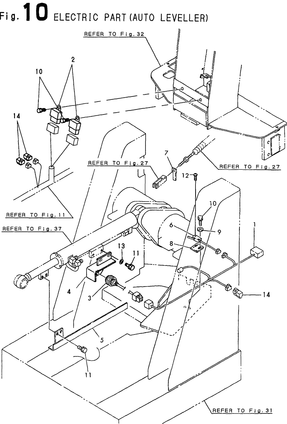
Fig.10. ELECTRIC PART(AUTO LEVELLER)
