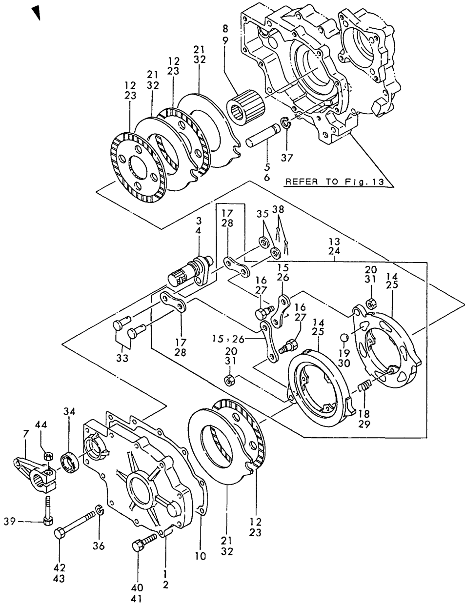
Fig.21 CENTER BRAKE 22inc.23 ~ 32
