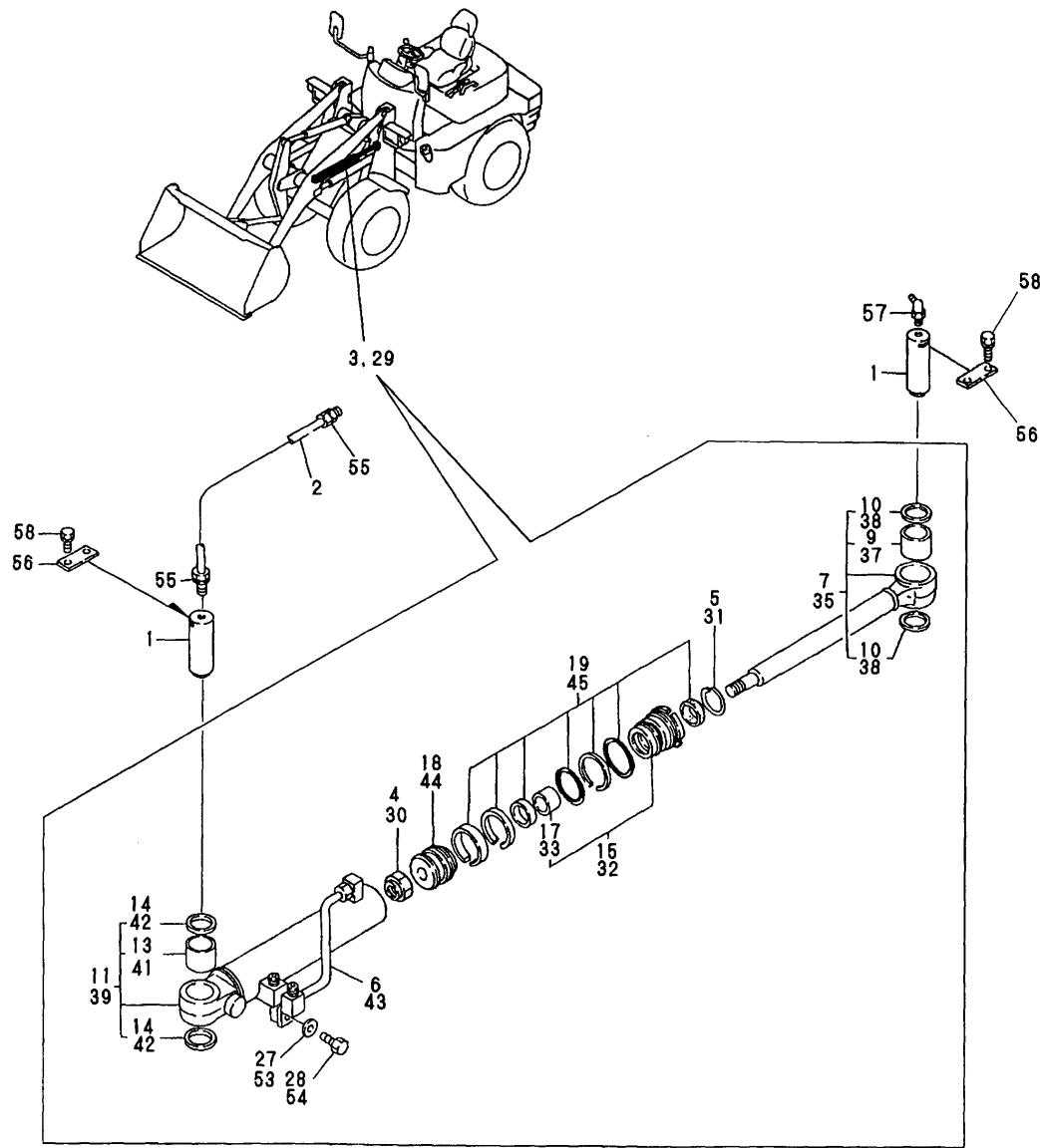
Fig.38 POWER STEERING CYLINDER
