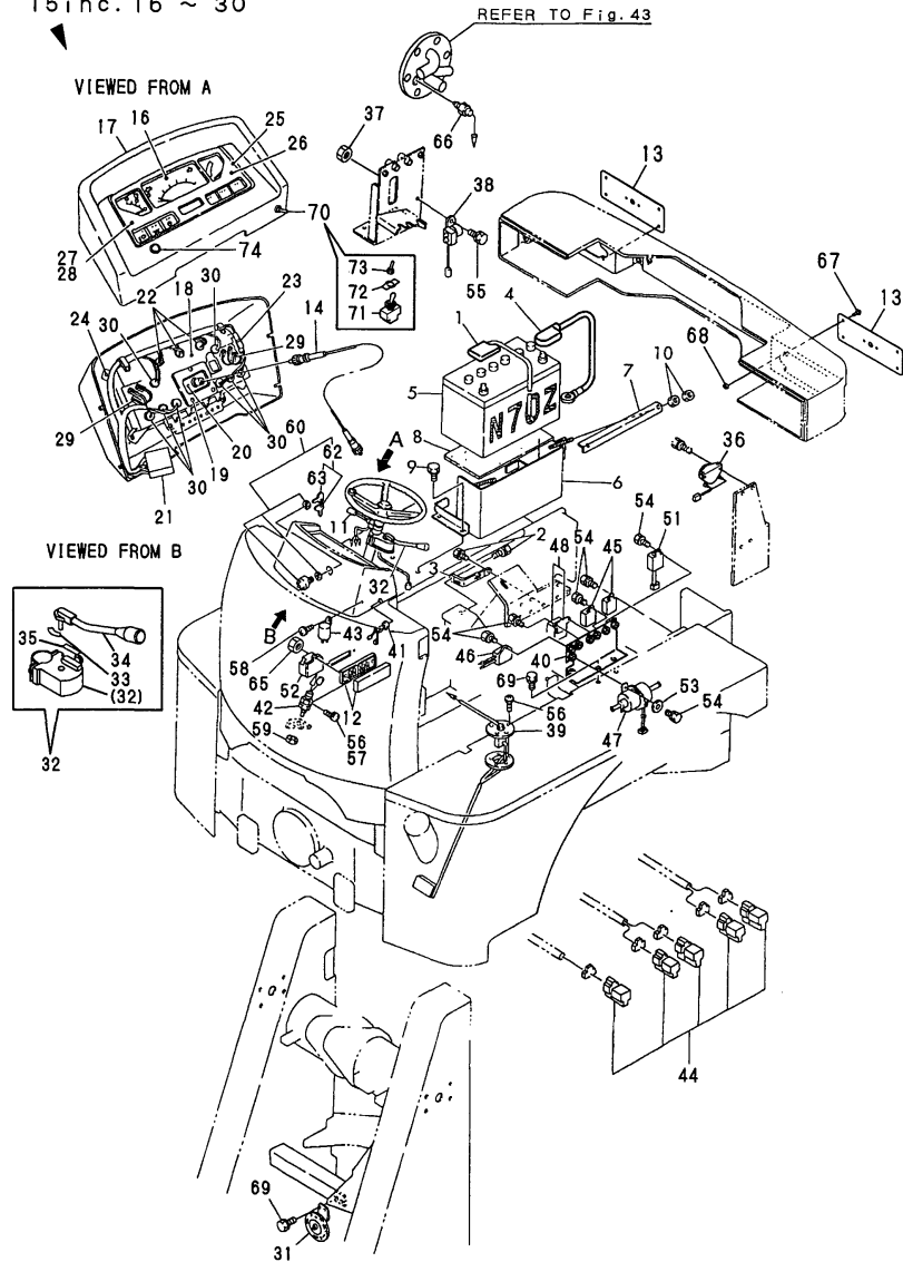
Fig.9 ELECTRIC PART
