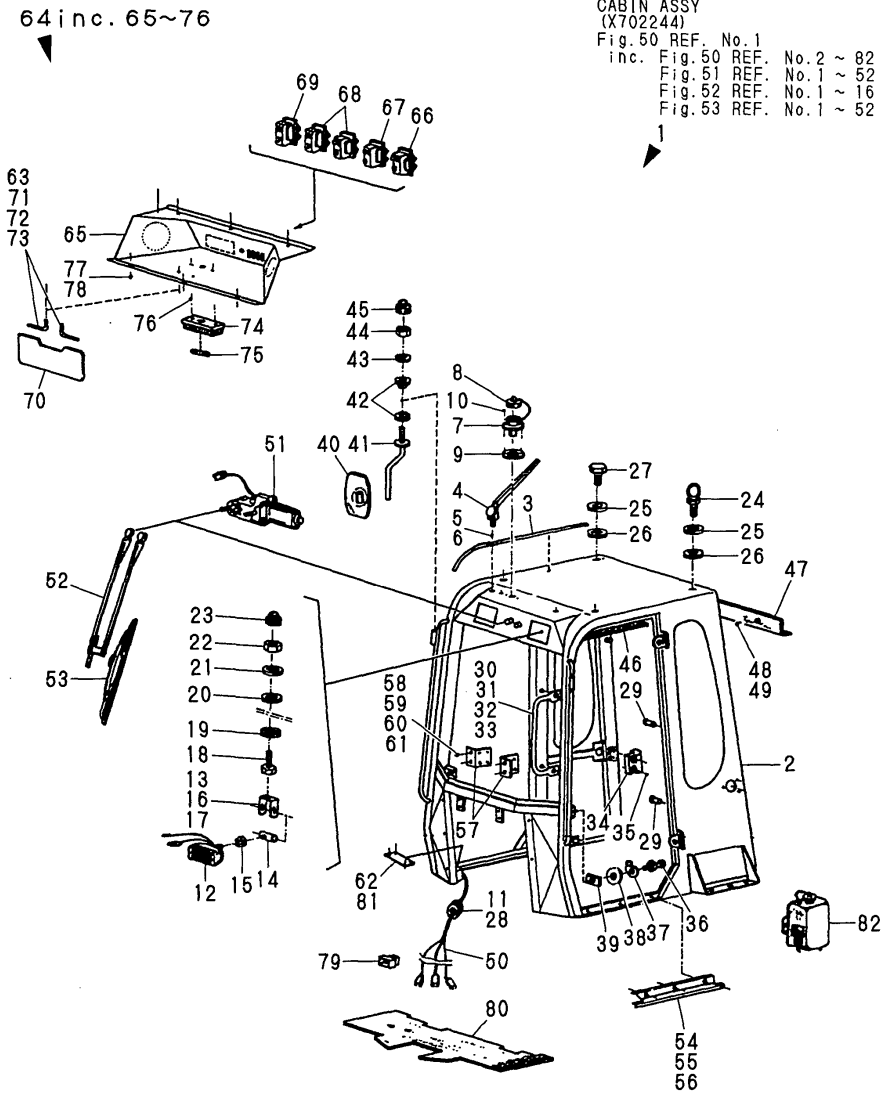
Fig.50 CABIN (1) (BODY)
