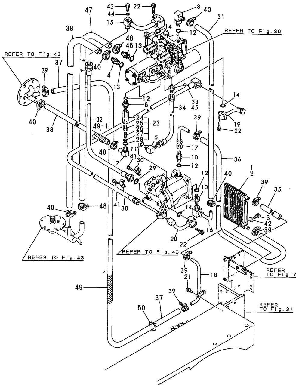
Fig.45 HYD.OIL PIPING (HST)
