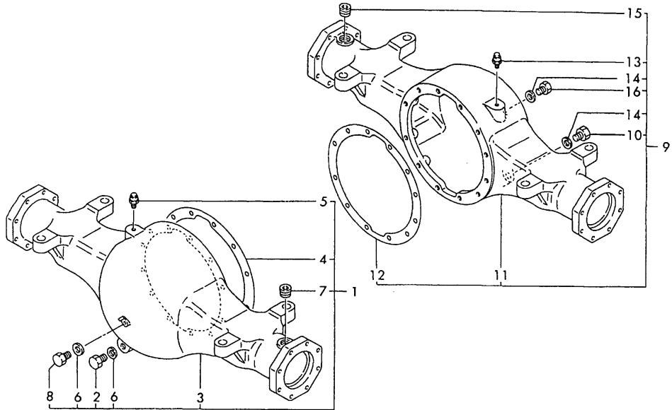
Fig.20 AXLE CASE
