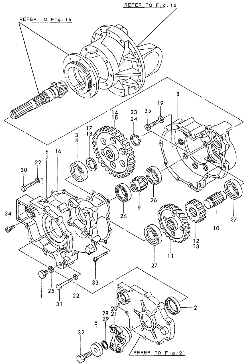
Fig.13 TRANSFER CASE
