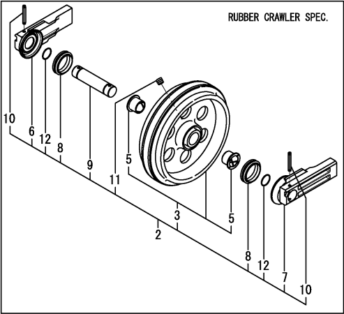
Fig.39. IDLER & ADJUST
