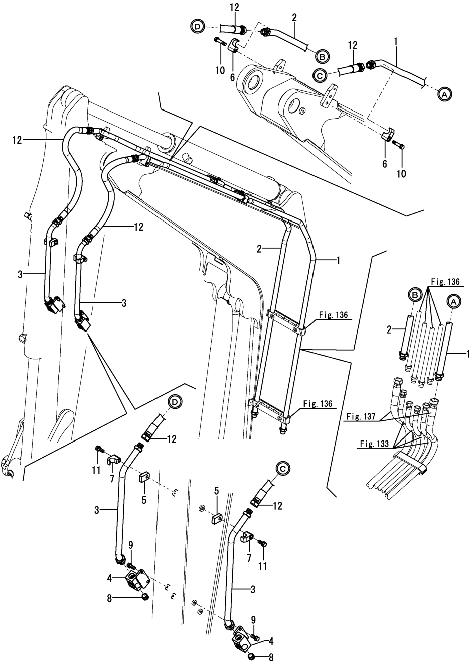
Fig.138. HYD. OIL PIPING(P.T.O. : ARM END)
