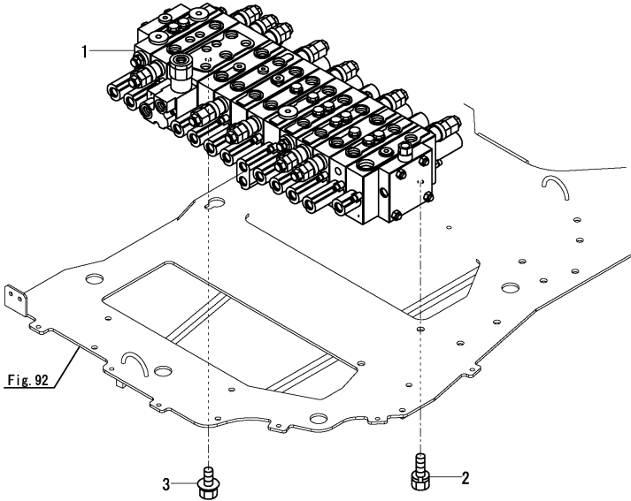
CONTROL VALVE ASSY Fig. 104 Ref. No. 1 Inc. Fig. 105~112.
