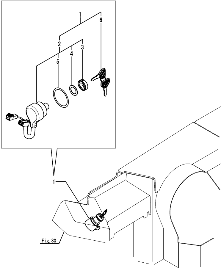
Fig.22. ELECTRIC PART(STARTING SWITCH)
