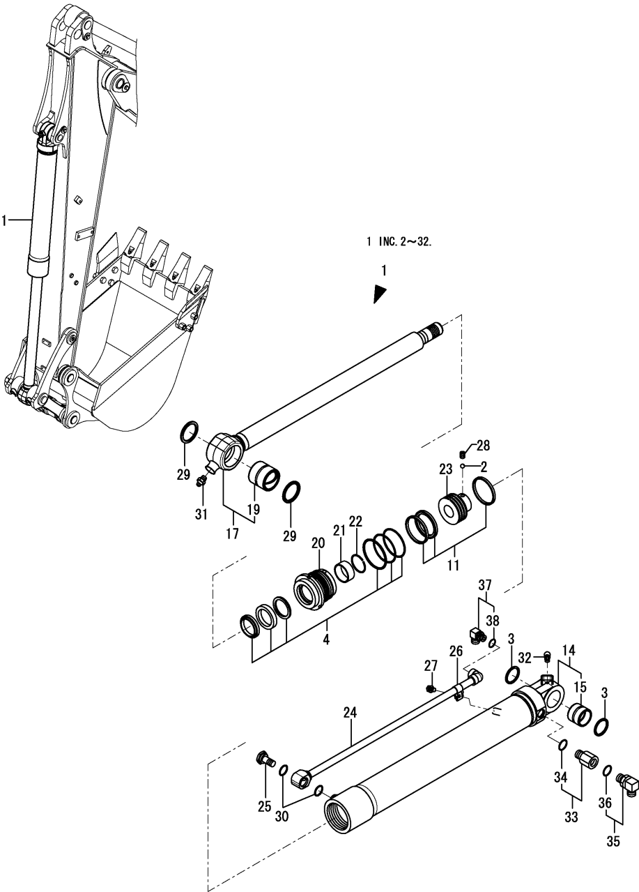
Fig.95. BUCKET CYLINDER
