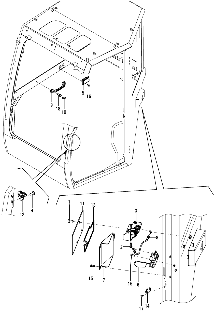
Fig.77. CABIN(BODY ACCESSORY)(2)
