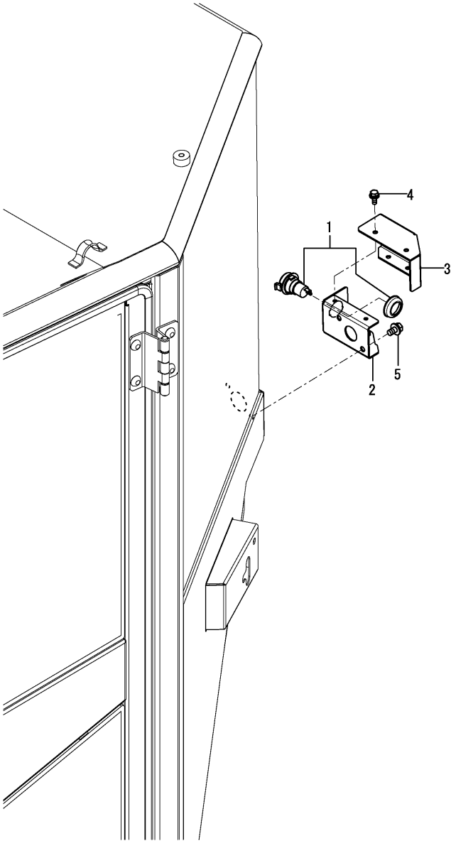
Fig.89. POWER SUPPLY SOCKET
