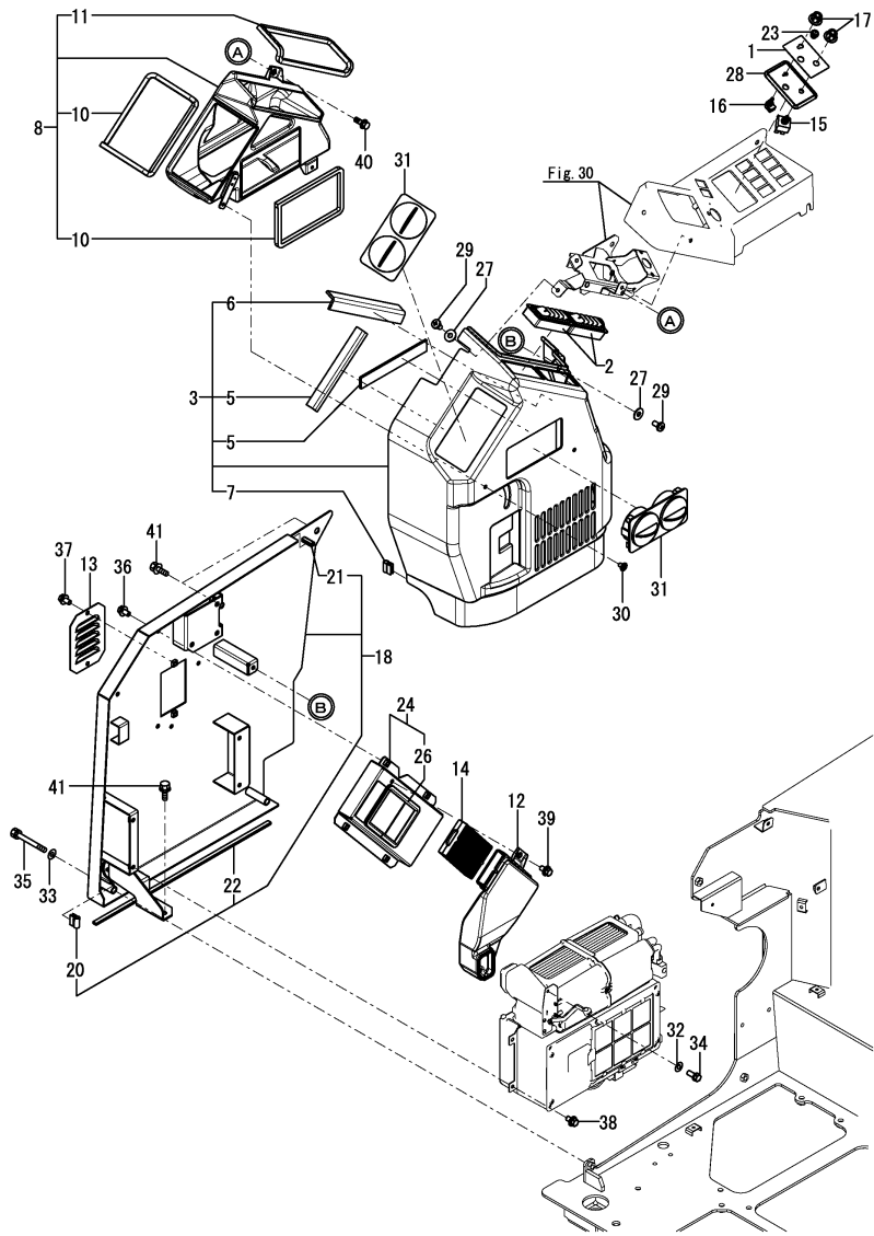
Fig.32. AIR CONDITIONER(CABIN RELATED)
