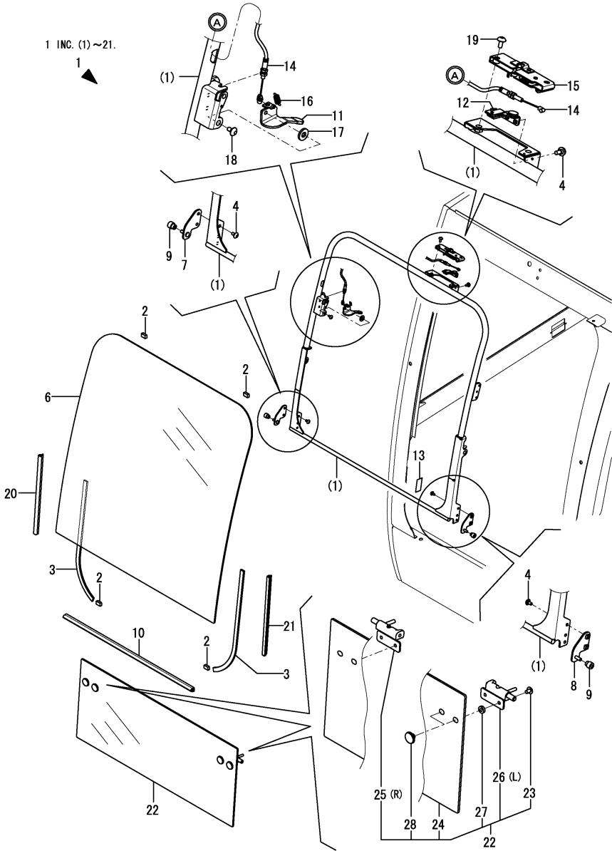
Fig.81. CABIN(FRONT WINDOW)
