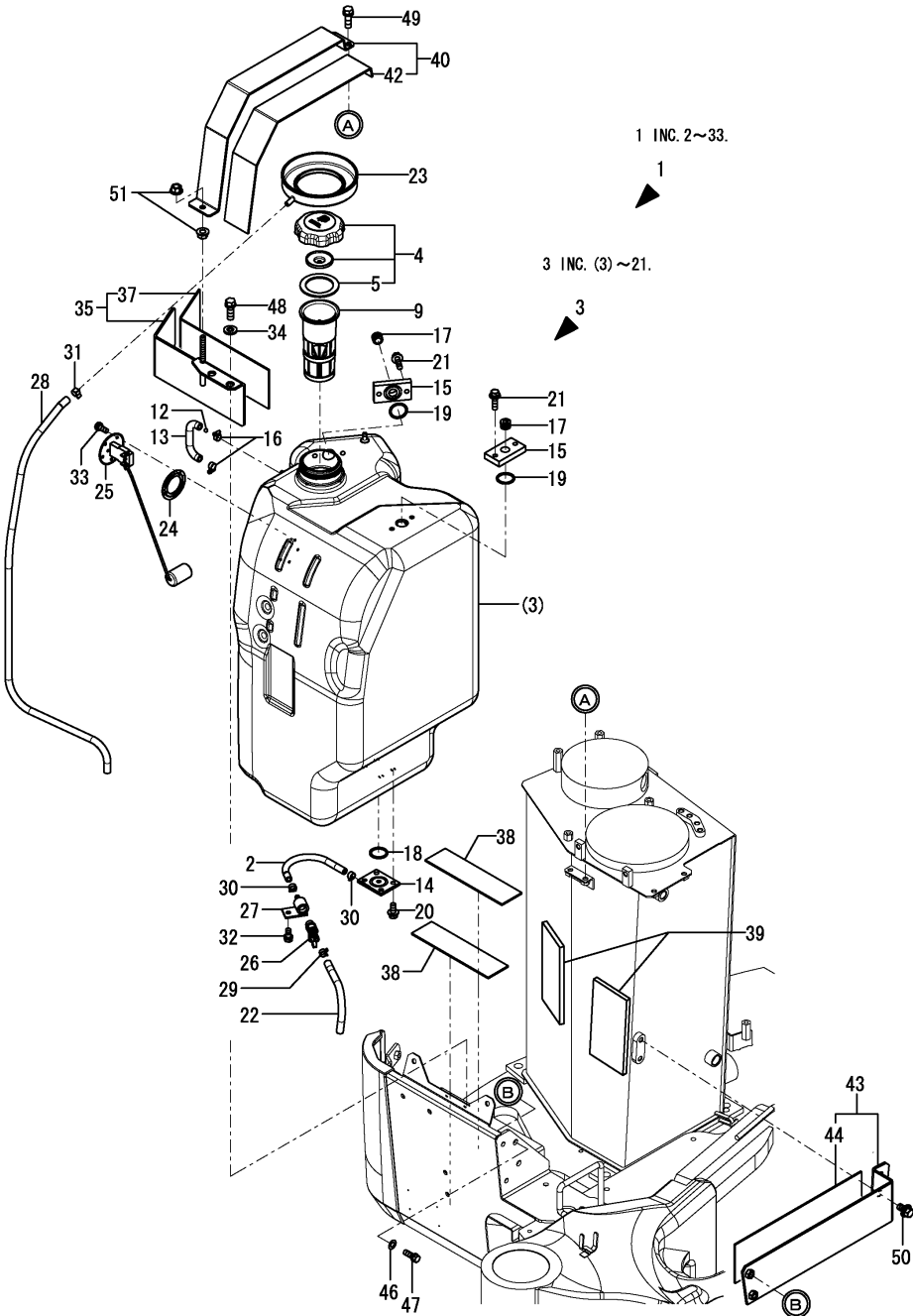
Fig.14. FUEL TANK
