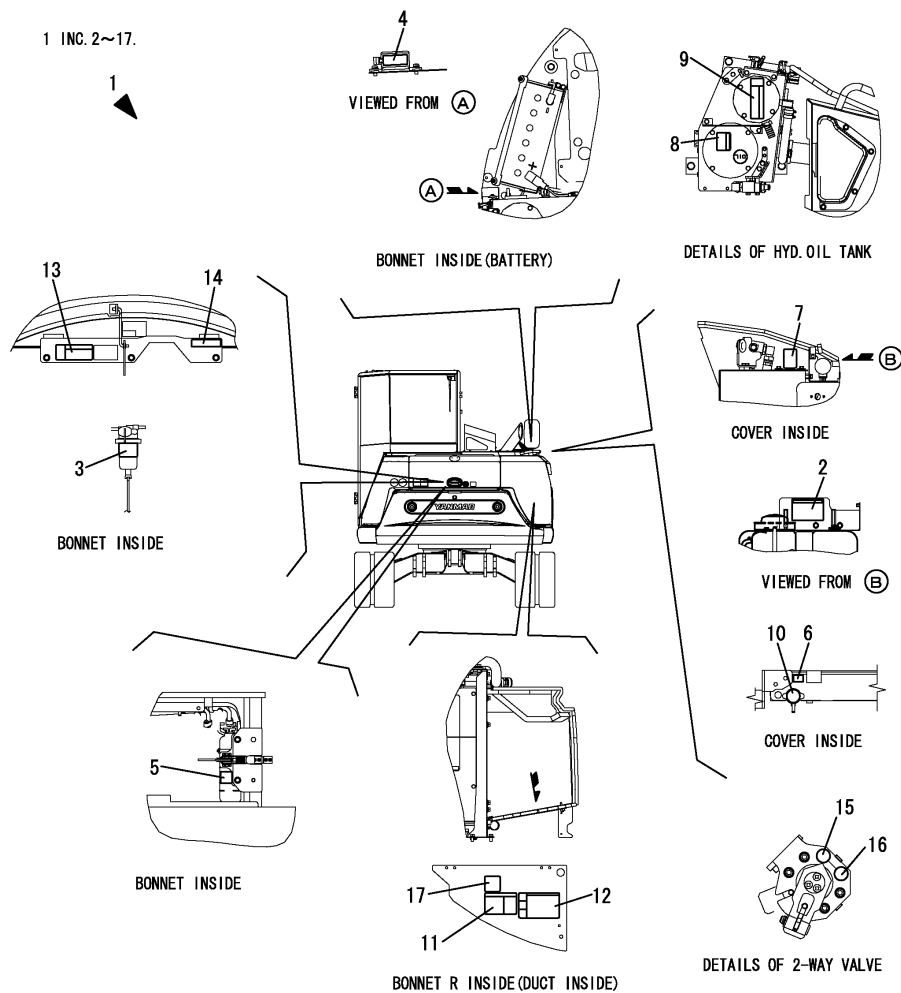
Fig.2. LABEL(BONNNET INSIDE)
