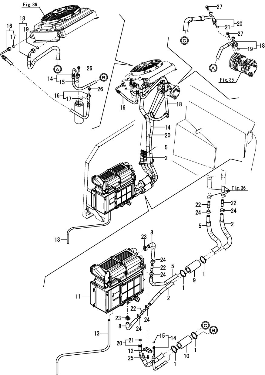
Fig.33. AIR CONDITIONER(PIPING)
