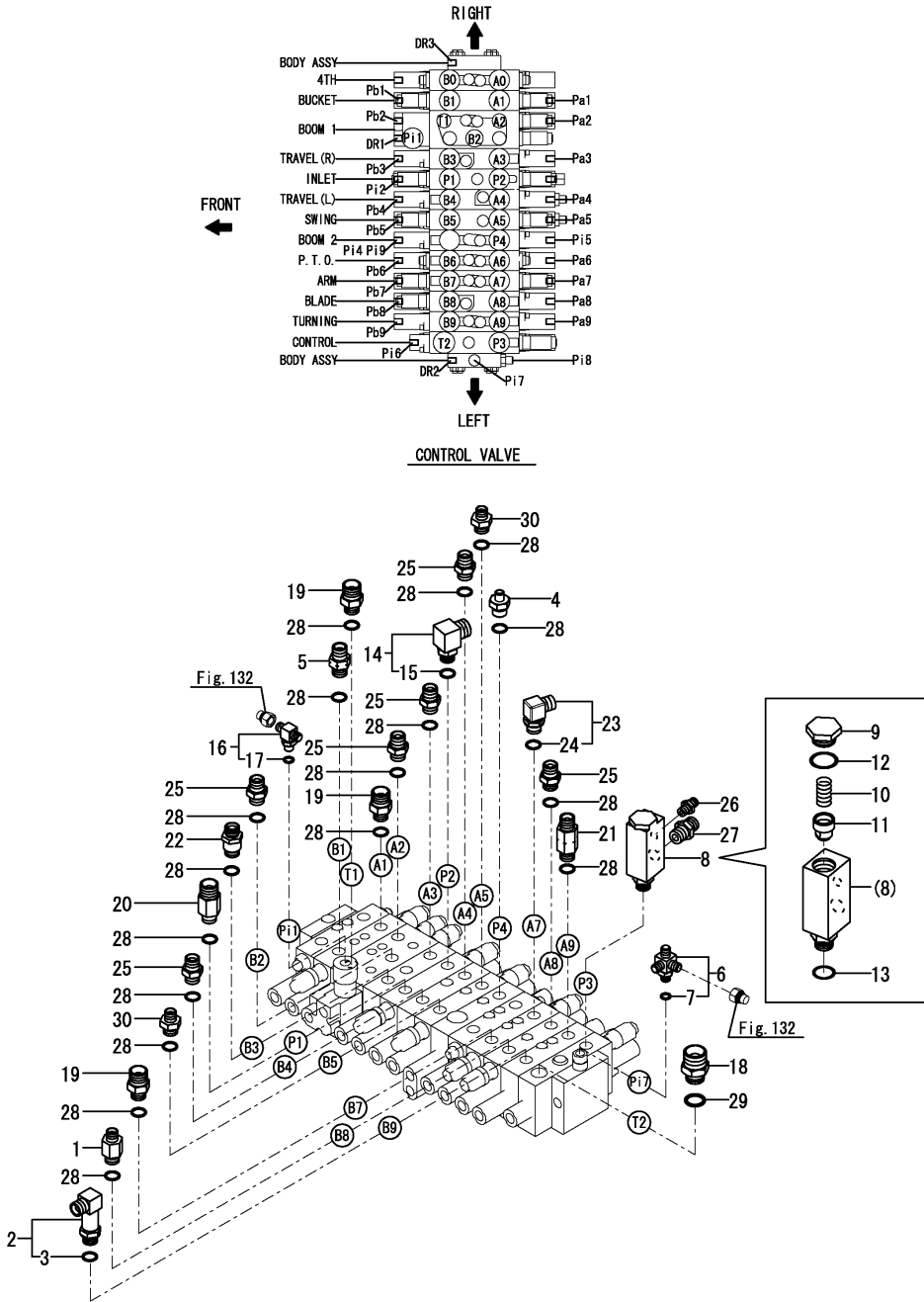
Fig.129. HYD. OIL PIPING(CONTROL VALVE : FITTING, 1)
