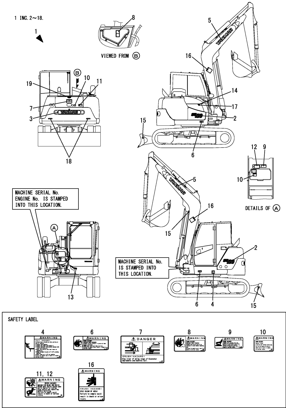
Fig.201. (1A)LABEL(EXTERIOR)(FROM MBF001)
