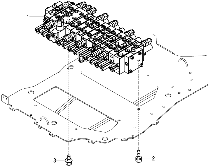
CONTROL VALVE ASSY Fig. 190 Ref. No. 1 Inc. Fig. 191~198.
