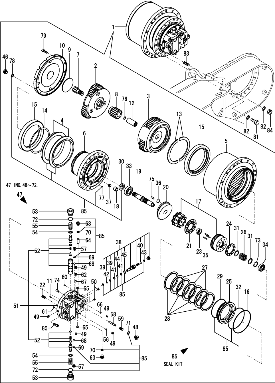
Fig.99. TRAVEL MOTOR
