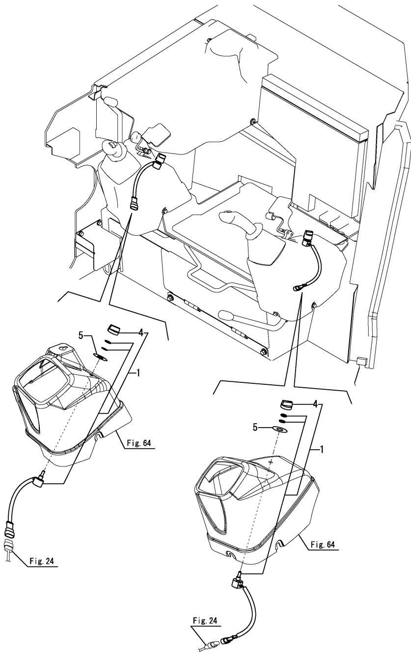
Fig.180. (31A)SENSOR VOLUME
