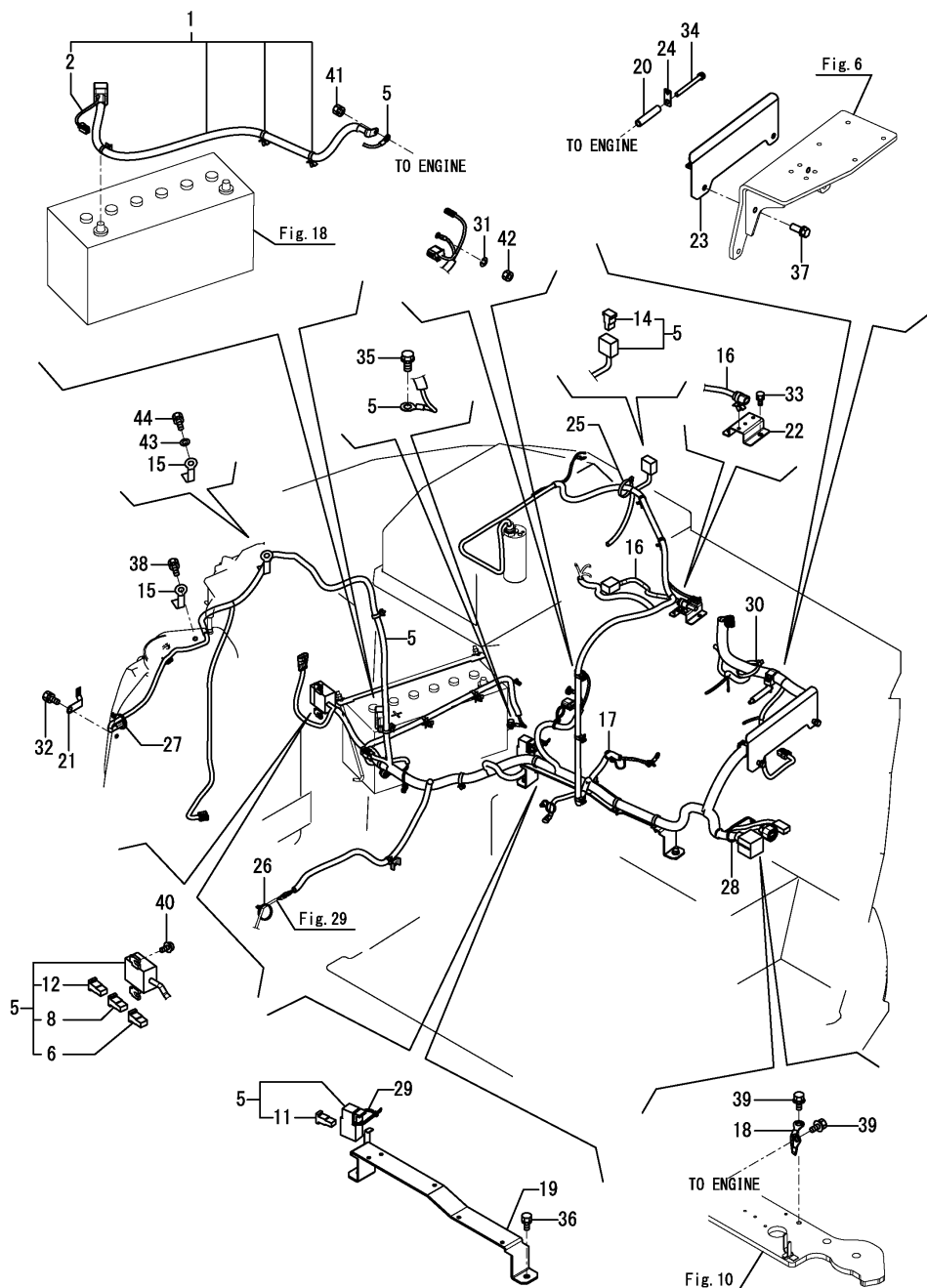
Fig.16. ELECTRIC PART(ENGINE)
