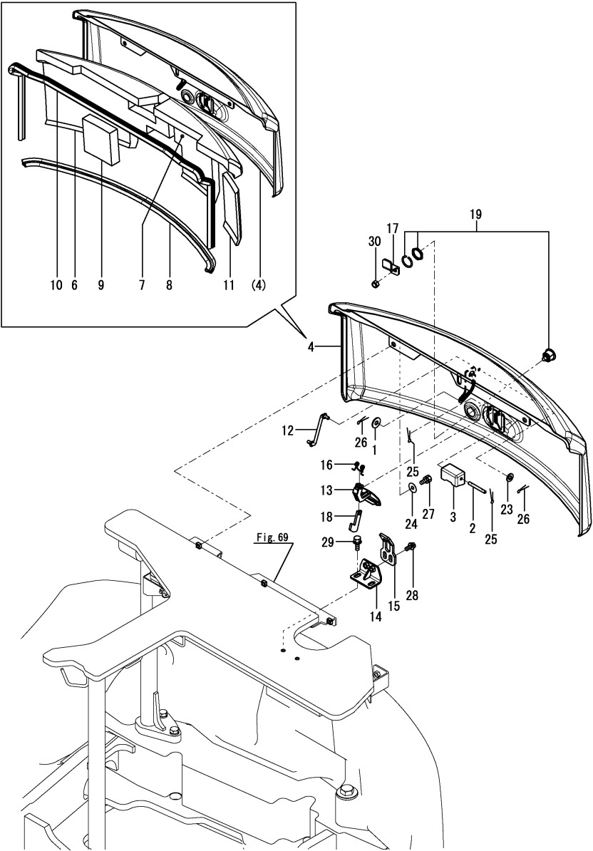
Fig.72. BONNET(REAR)
