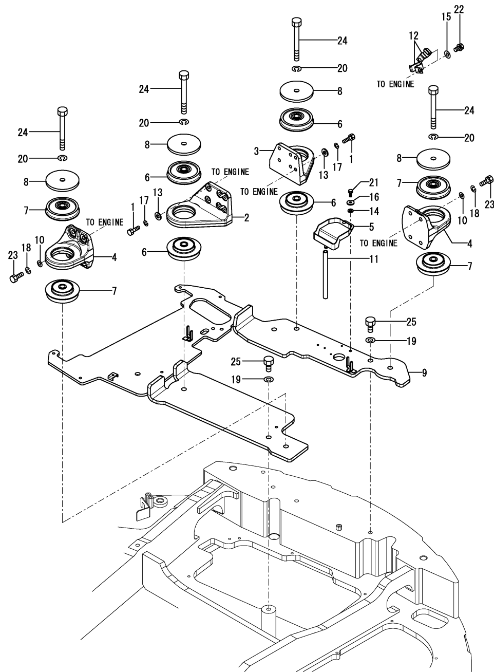
Fig.10. ENGINE MOUNT
