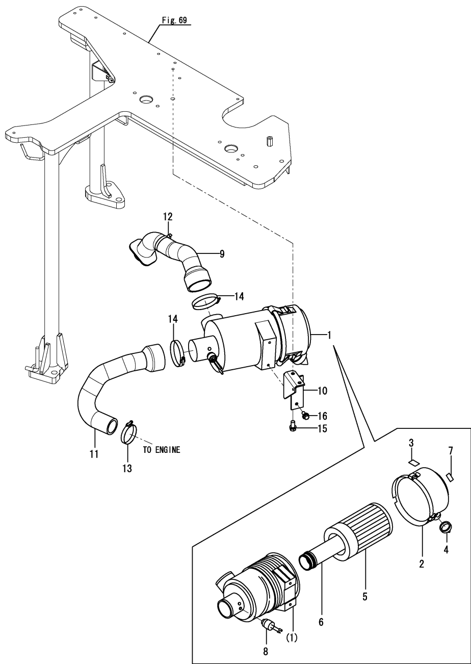
Fig.8. AIR CLEANER(W)
