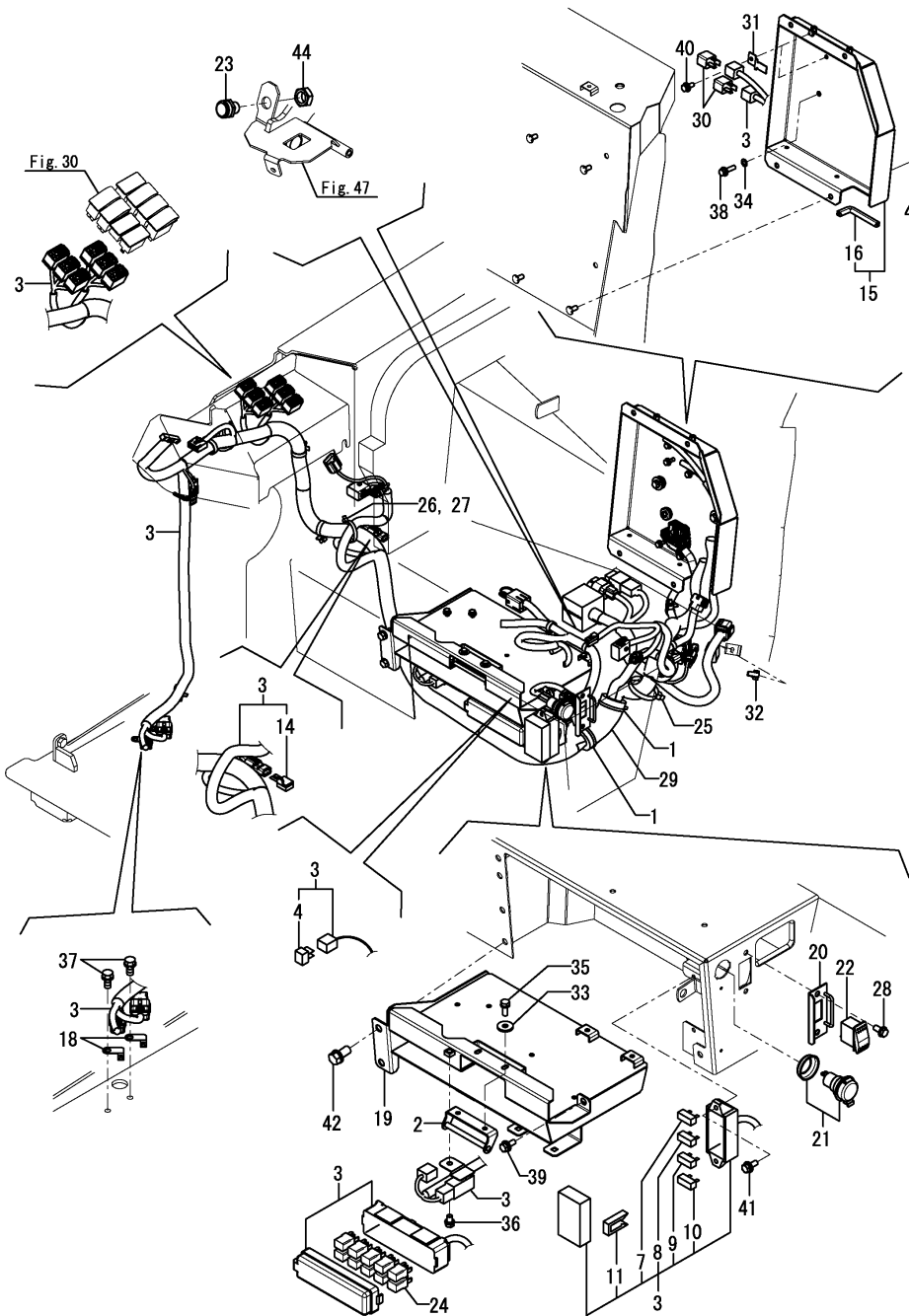
Fig.24. ELECTRIC PART(SEAT MOUNT)(US,AS)
