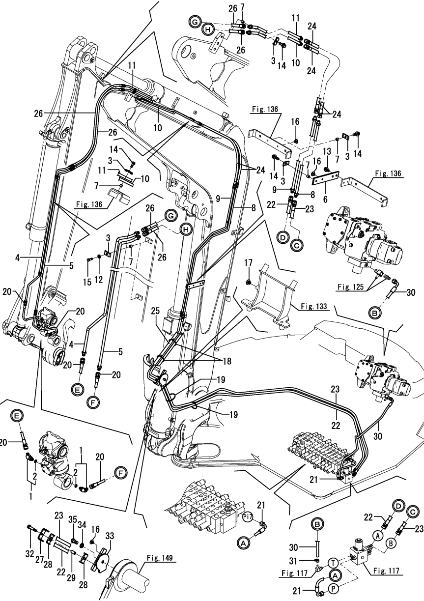
Fig.139. HYD. OIL PIPING(QUICK COUPLER)
