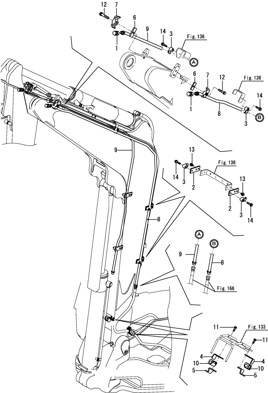
Fig.167. P.T.O. 2 KIT(BOOM END)(OPTIONAL)(7/7)
