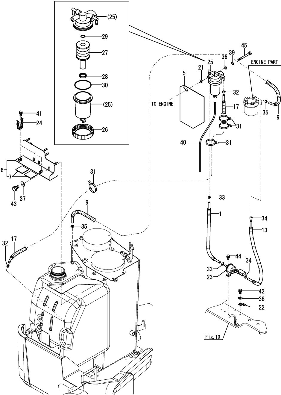
Fig.15. FUEL LINE
