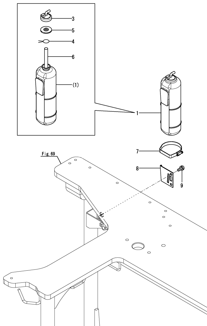
Fig.13. RADIATOR SUB-TANK
