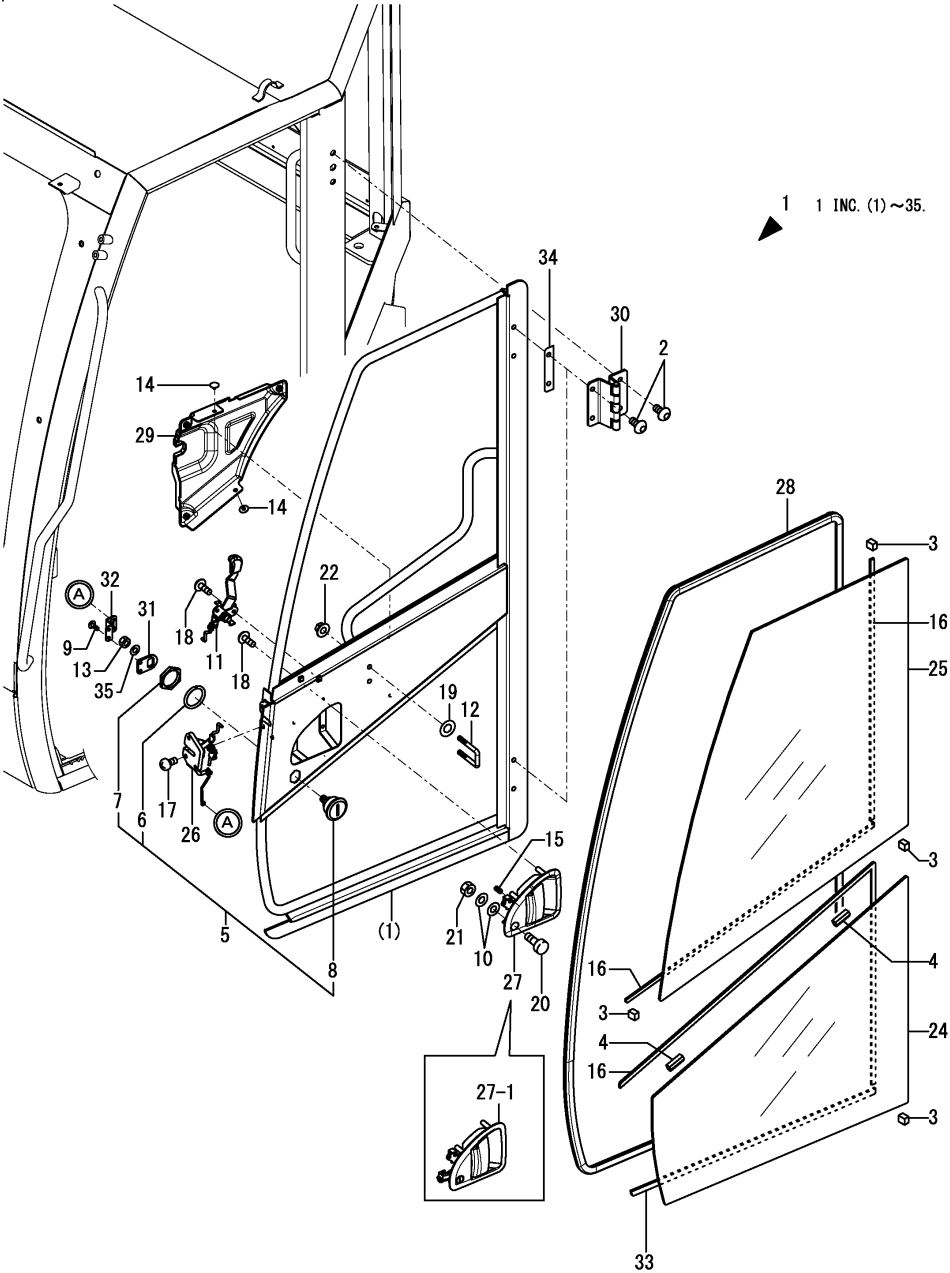
Fig.85. CABIN(DOOR)
