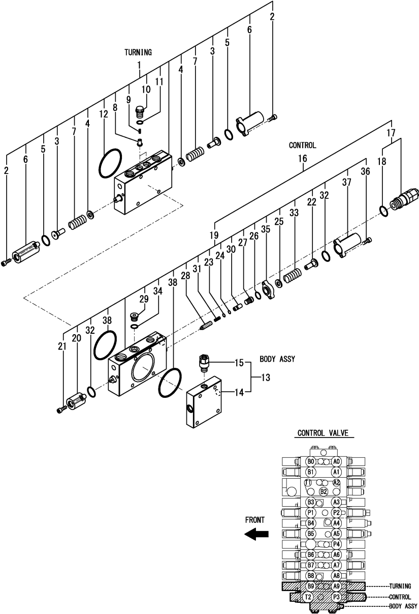
Fig.198. (112I)CONTROL VALVE(B-TYPE)(9/9)(FROM M2A189)
