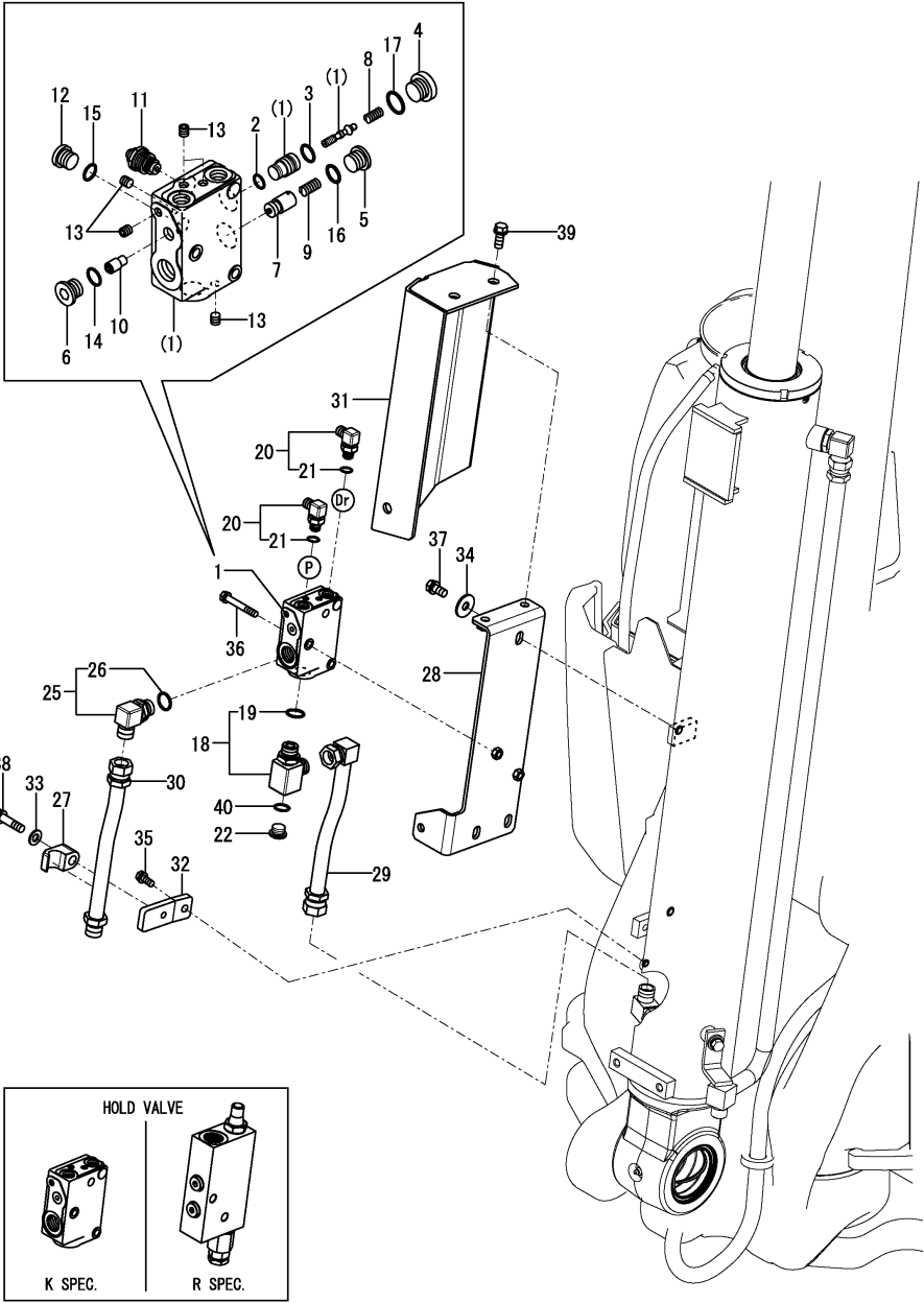
Fig.123. HOLD VALVE(BOOM)(K SPEC.)
