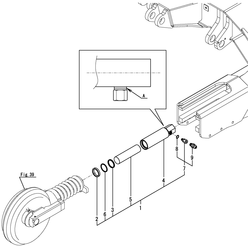
Fig.42. CRAWLER ADJUST(Y SPEC.)(TO M2A229)
