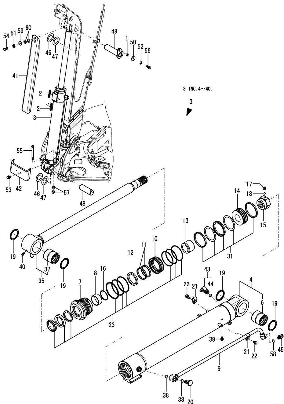
Fig.93. BOOM CYLINDER
