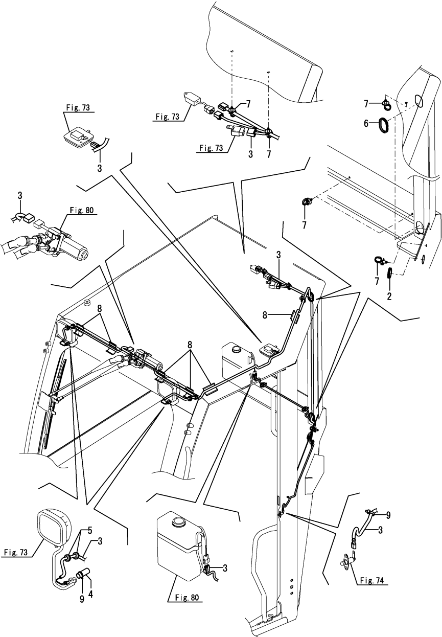
Fig.76. CABIN(ELECTRIC PARTS)
