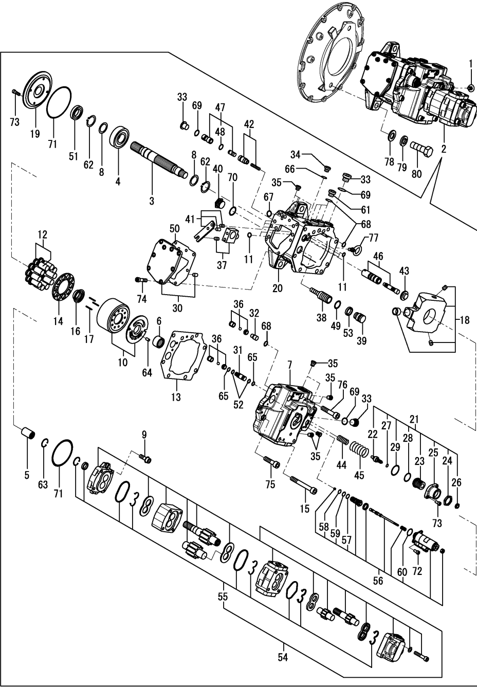
Fig.87. HYDRAULIC PUMP
