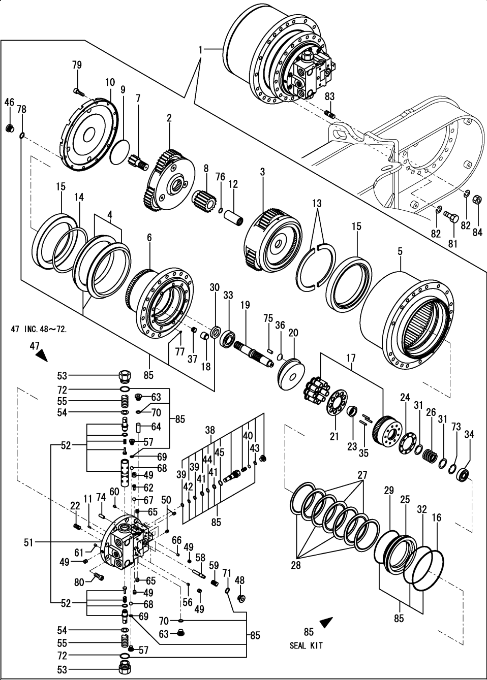
Fig.95. TRAVEL MOTOR
