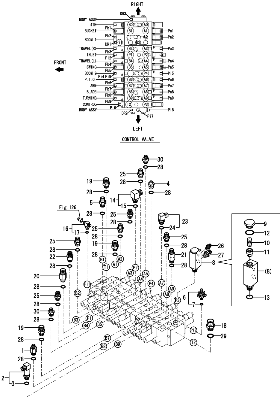
Fig.123. CONTROL VALVE(FITTING)(1)
