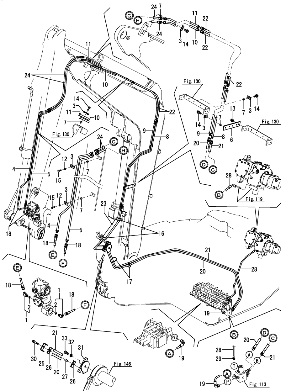
Fig.137. QUICK COUPLER
