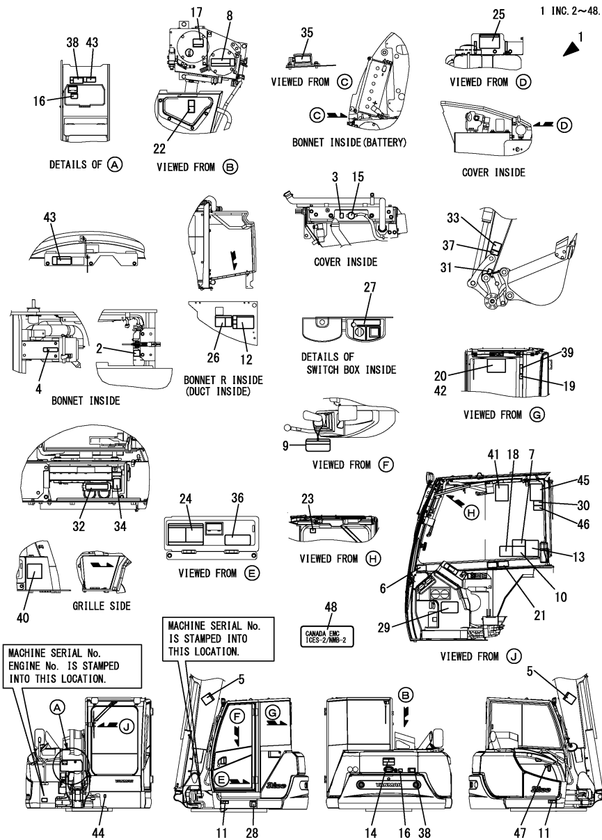
Fig.153. LABEL KIT(FOR CANADA)(OPTIONAL)
