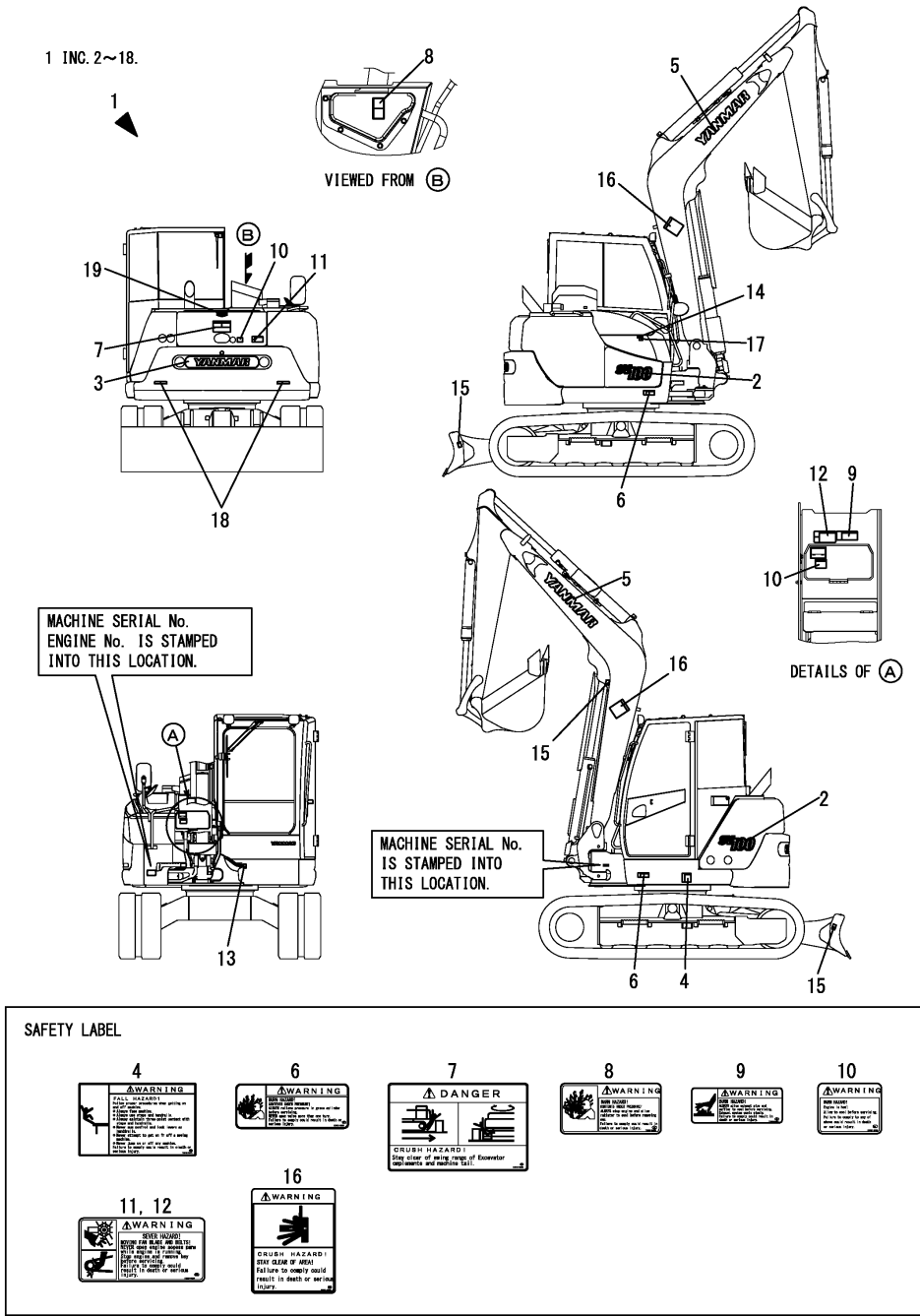
Fig.182. (1A)LABEL(EXTERIOR)(FROM MAF001)
