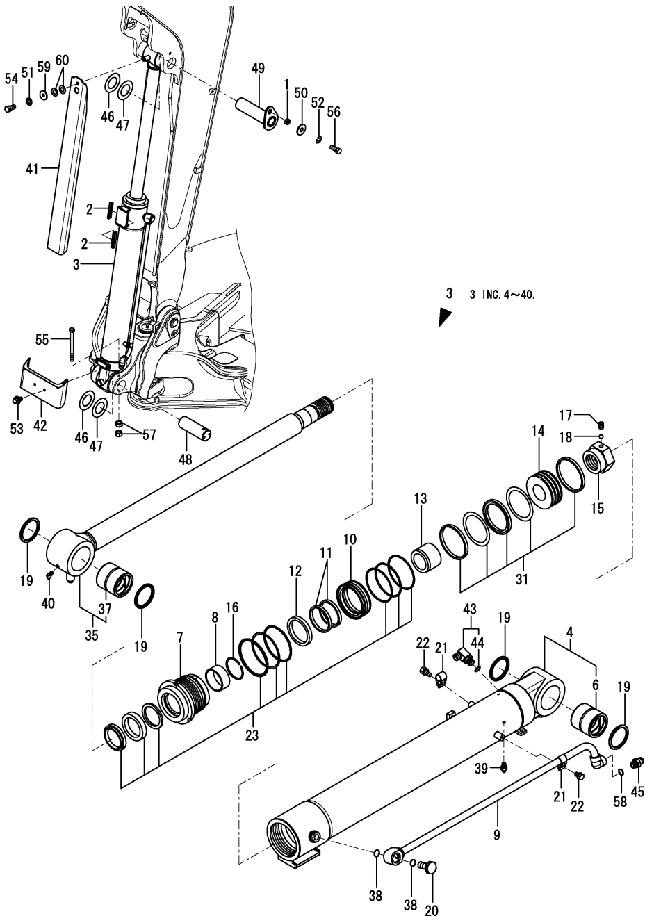
Fig.89. BOOM CYLINDER
