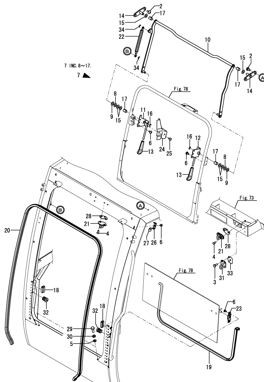
Fig.79. CABIN(FRONT WINDOW)(2)
