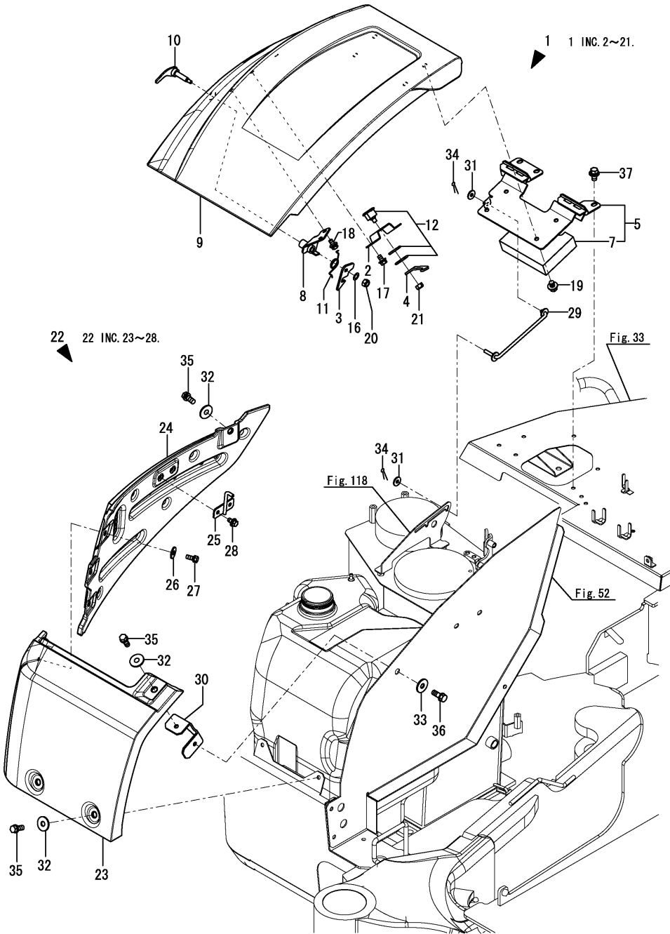
Fig.66. BONNET(FRONT)
