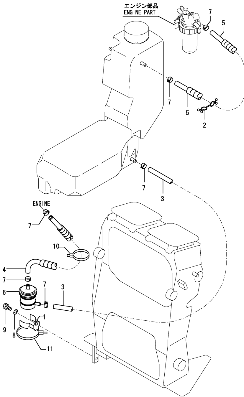
Fig.11. FUEL LINE
