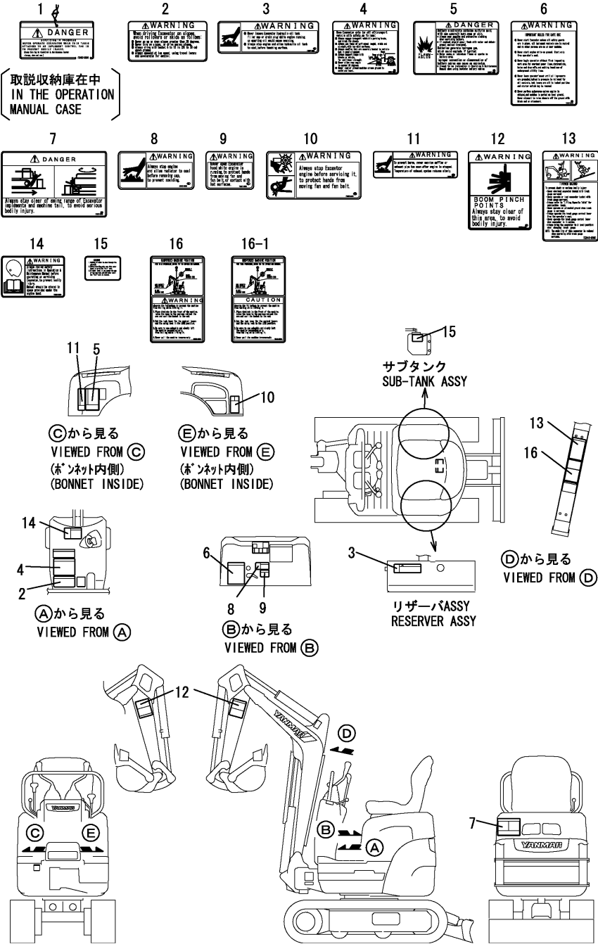
Fig.4. SAEFTY LABEL(EX)
