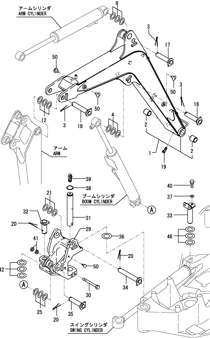
Fig.69. BOOM & BOOM BRACKET
