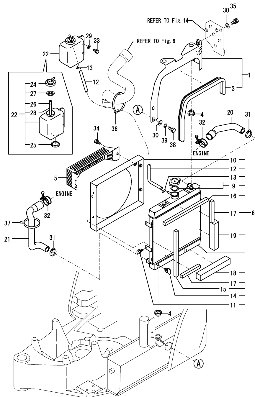
Fig.9. RADIATOR & MOUNT
