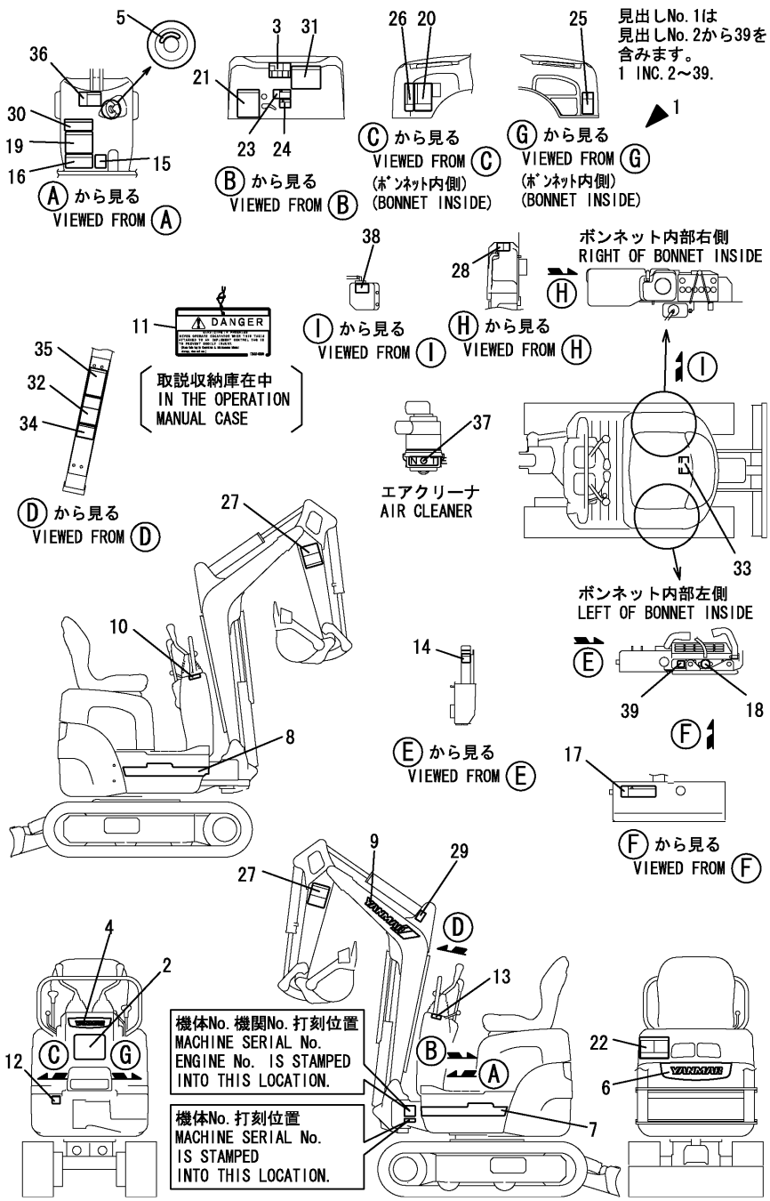
Fig.2. LABEL(EX)
