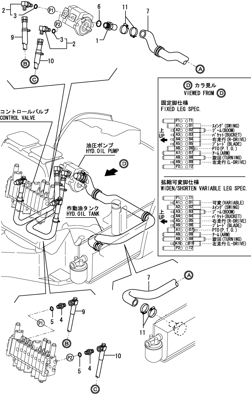
Fig.55. HYD.OIL PIPING(TANK - PUMP - CONTROL VALVE)
