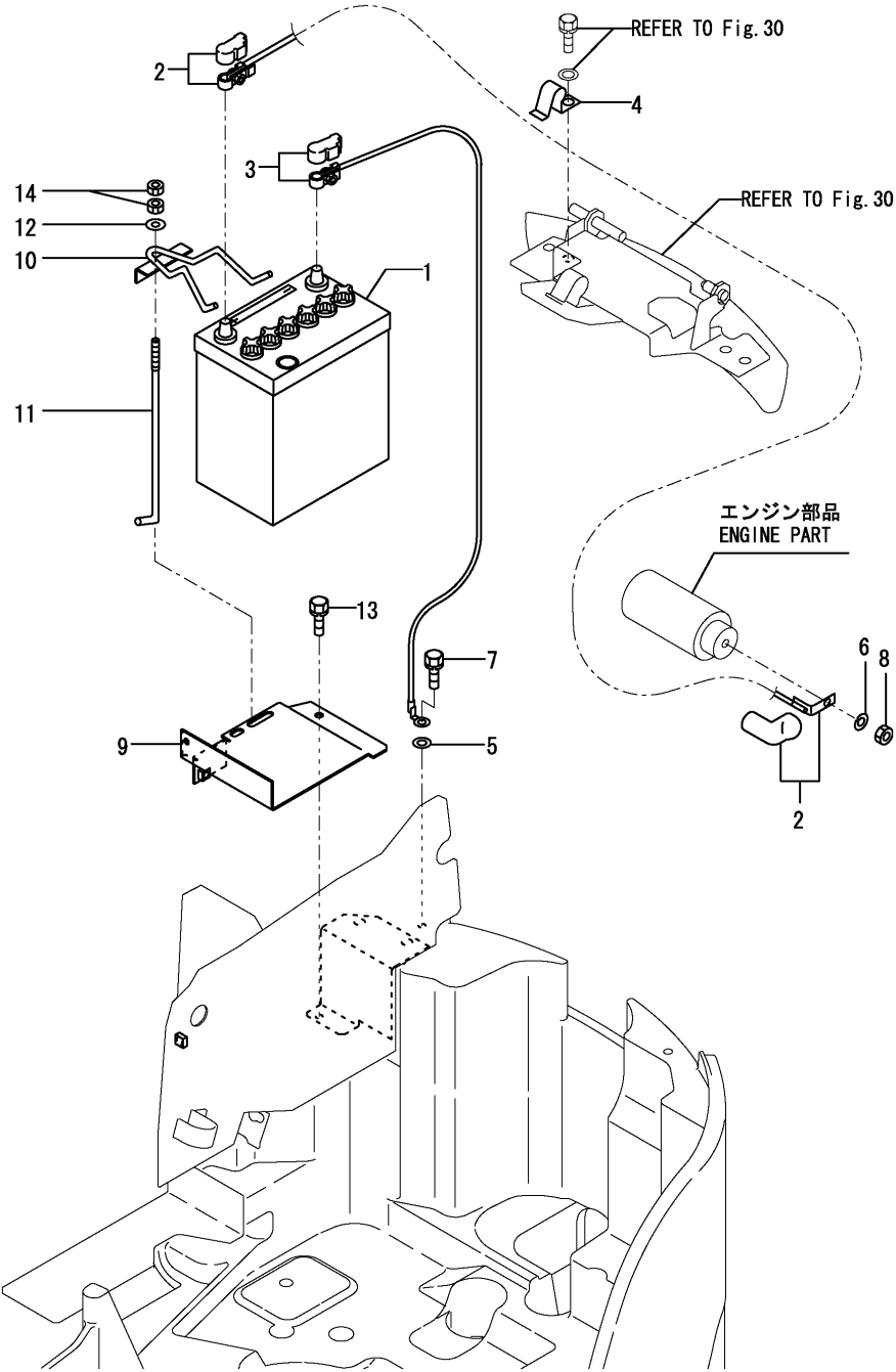
Fig.12. BATTERY
