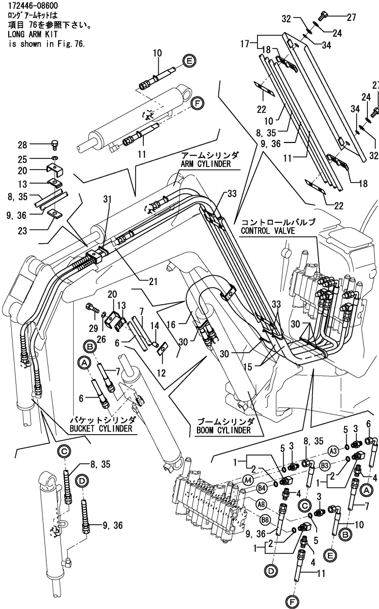
Fig.66. HYD.OIL PIPING(BOOM)VARIABLE LEG SPEC.
