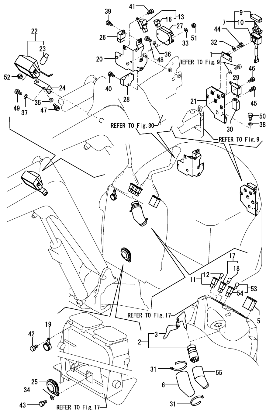
Fig.14. ELECTRIC PART(EQUIPMENT)
