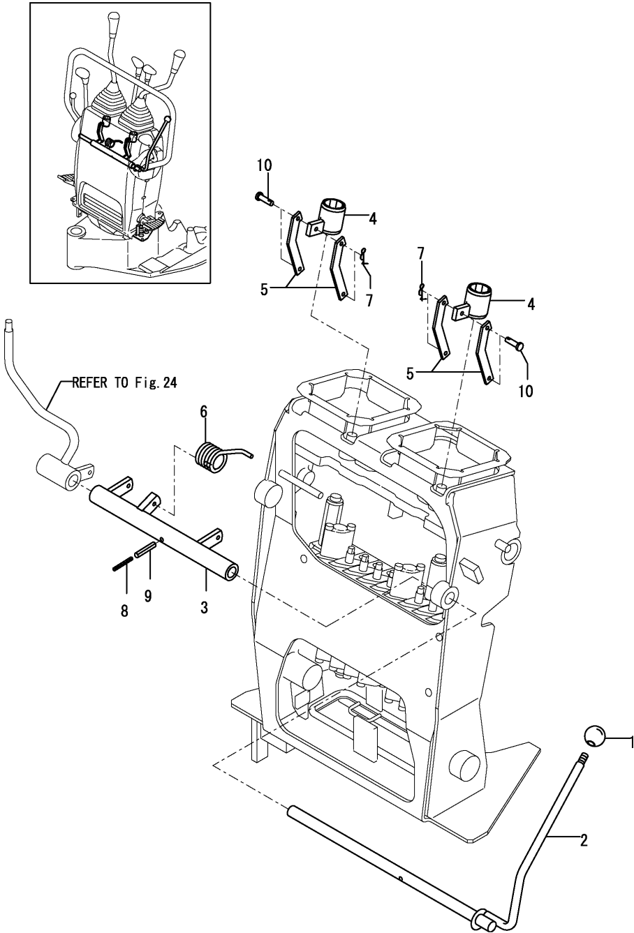
Fig.18. CONTROL EQUIPMENT(STOPPER)
