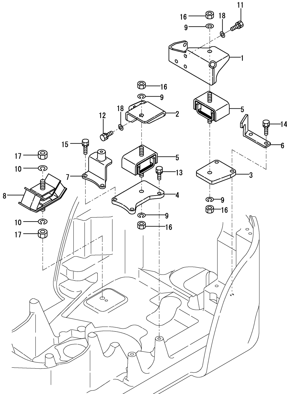
Fig.8. ENGINE MOUNT
