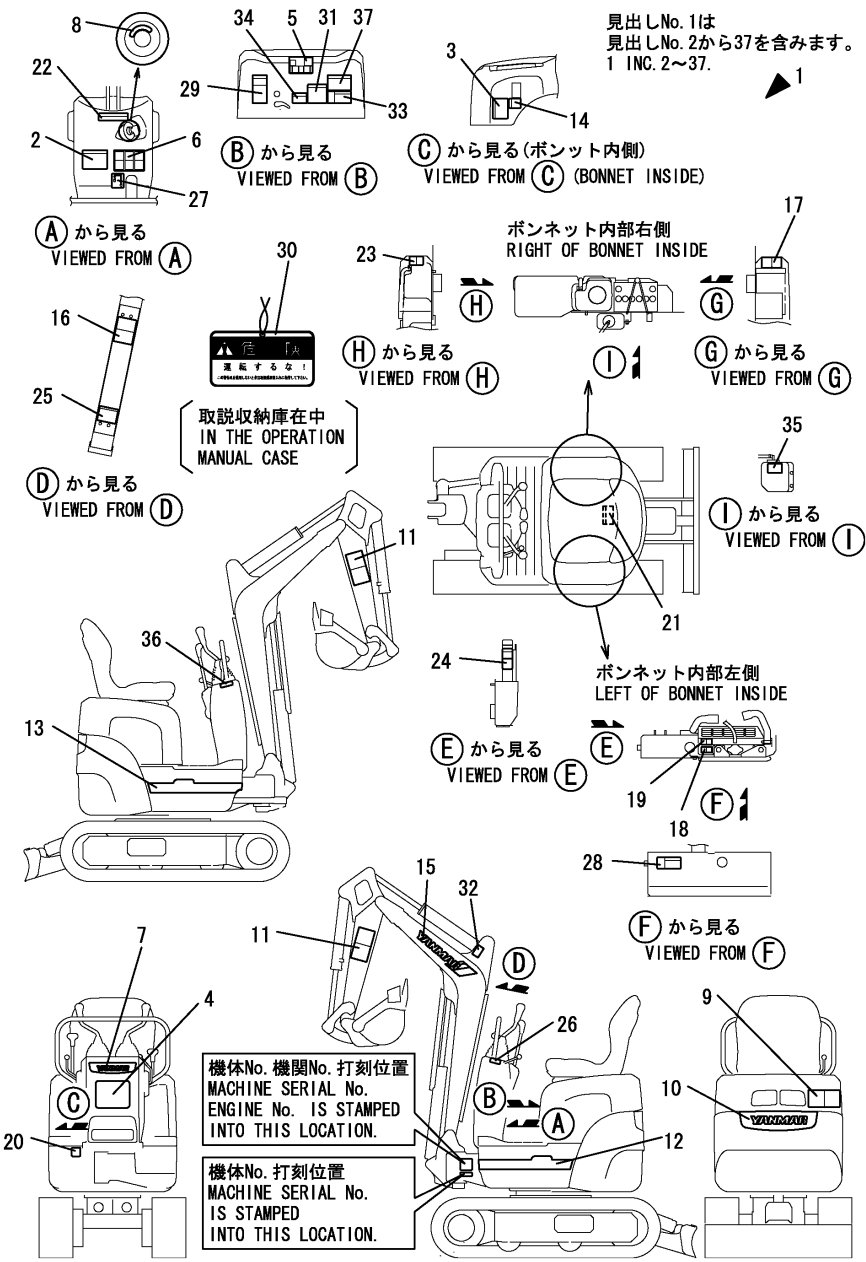
Fig.1. LABEL(JP)
