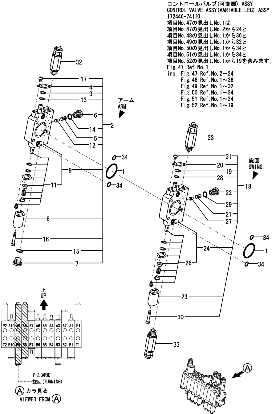
Fig.51. CONTROL VALVE(WIDEN/SHORTEN VARIABLE LEG SPEC. : 5/6)
