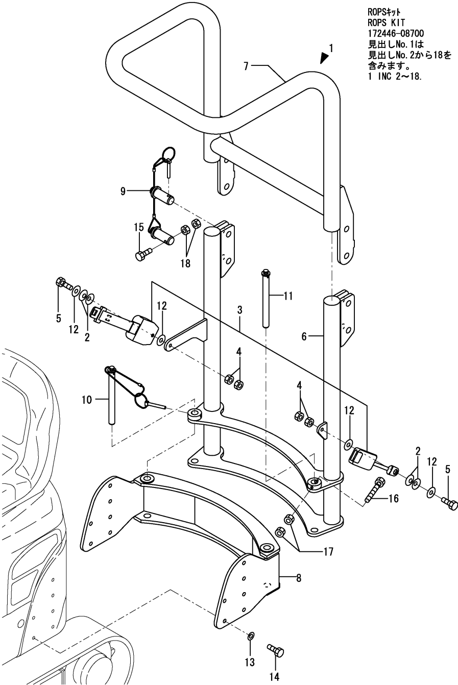
Fig.77. ROPS KIT
