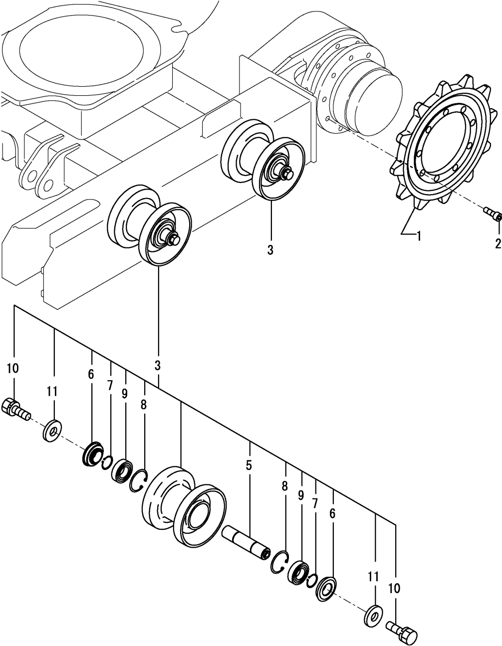
OCK10-M37402 TRAVELING Fig.15. SPROCKET & ROLLER
