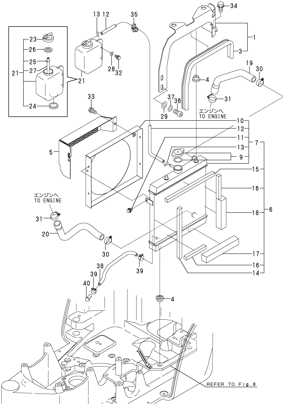
Fig.9. RADIATOR & MOUNT
