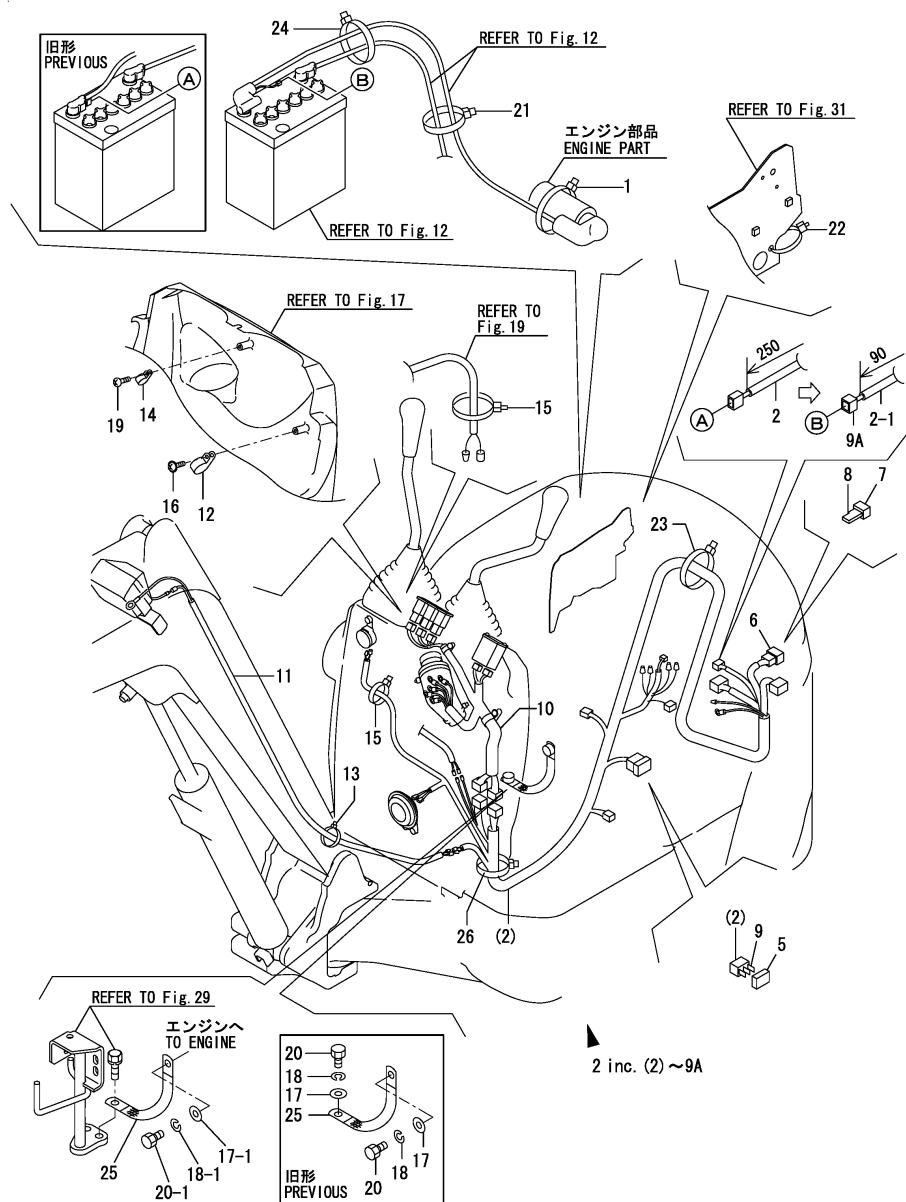
Fig.13. ELECTRIC PART(WIRING)
