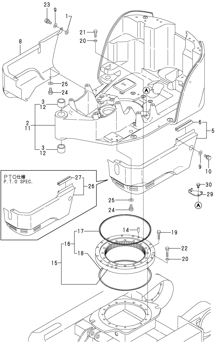
Fig.28. TURNING FRAME
