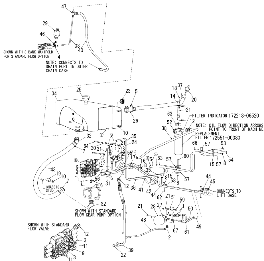
Fig.26. HYDRAULICS - CHASSIS
