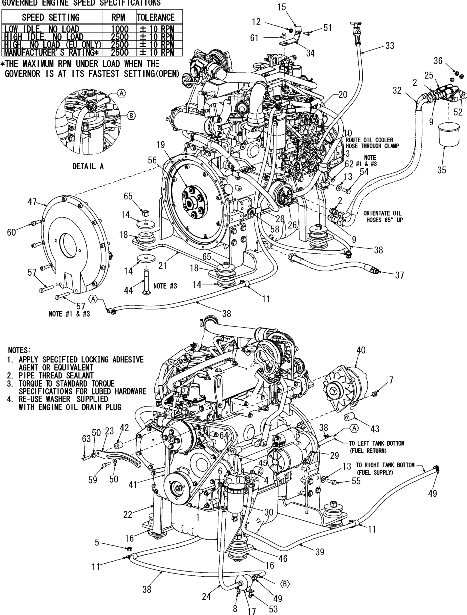
Fig.21. ENGINE
