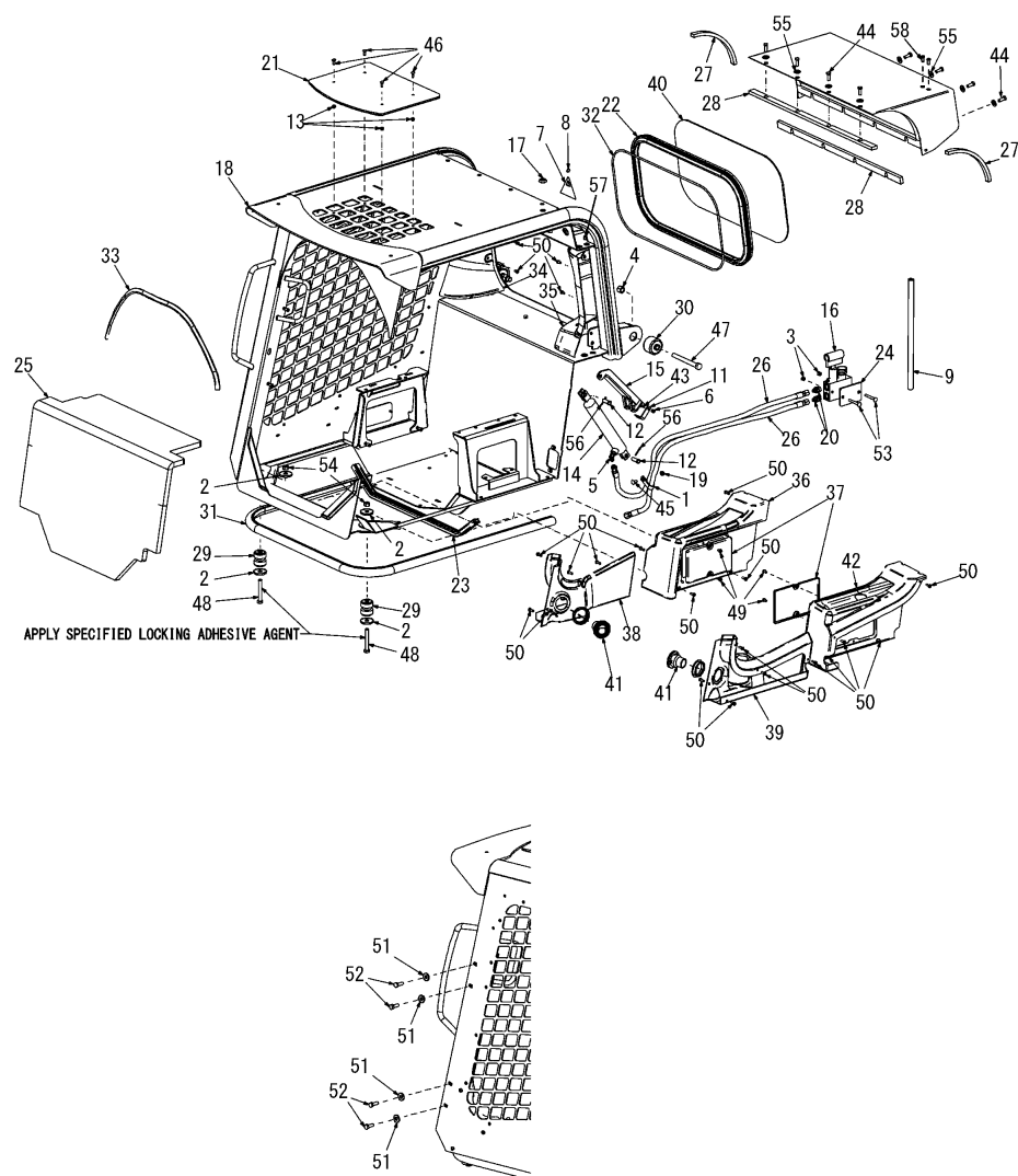
Fig.5. ROPS/FOPS STRUCTURE
