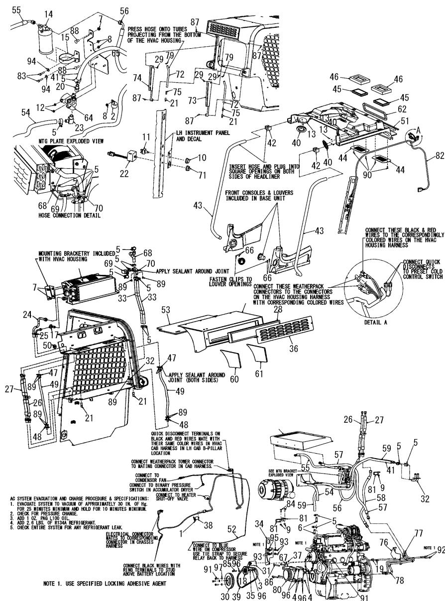
Fig.2. CHASSIS(HVAC COMPLETING)
