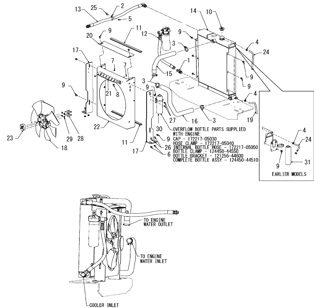
Fig.23. RADIATOR/COOLER
