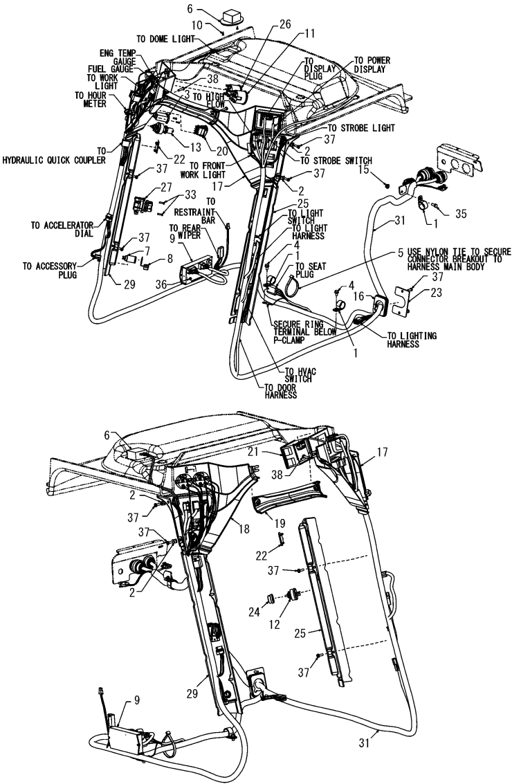
Fig.37. ELECTRICAL - ROPS/FOPS
