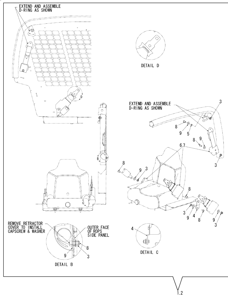
Fig.13. SEATS - THREE-POINT RESTRAINT SEAT BELT OPTION
