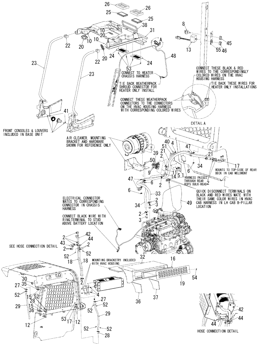
Fig.3. CHASSIS(HEATER-ONLY COMPLETING)
