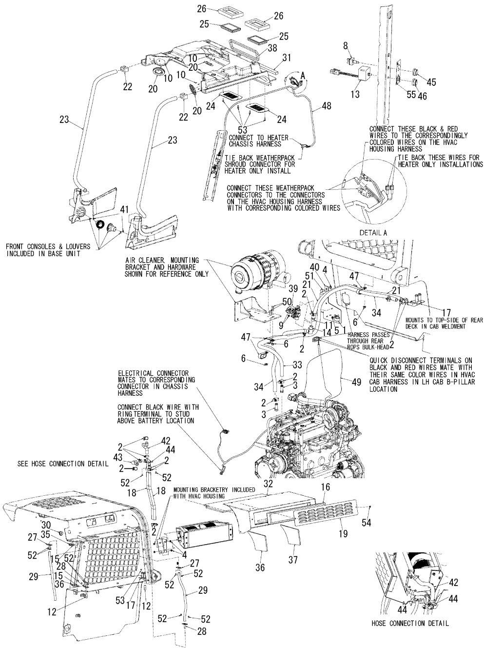
Fig.3. CHASSIS(HEATER-ONLY COMPLETING)
