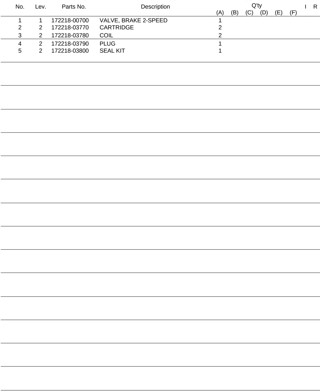
Fig.60. SOLENOID VALVES - BRAKE, JOYSTICK SUPPLY AND BRAKE RELEASE(TWO-SPEED)
