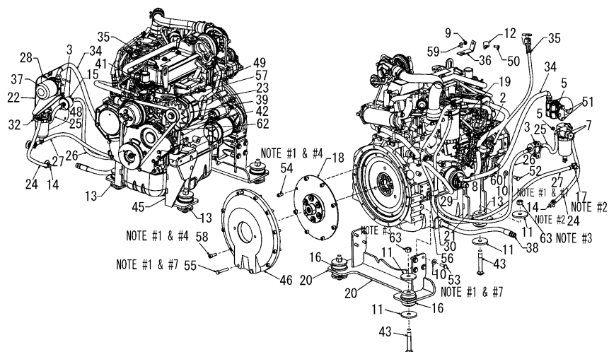
Fig.22. ENGINE
