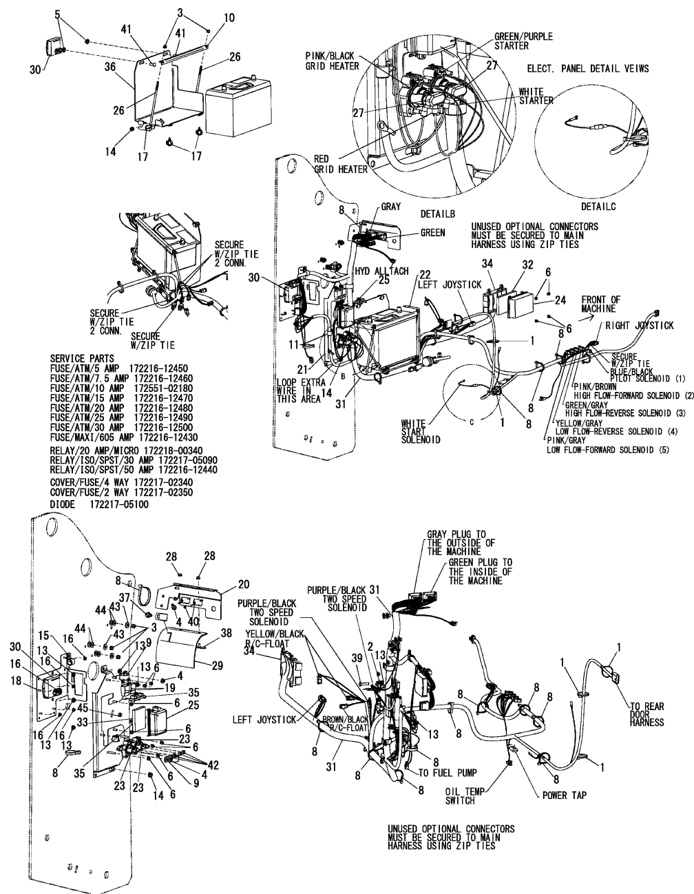
Fig.42. ELECTRICAL - CHASSIS
