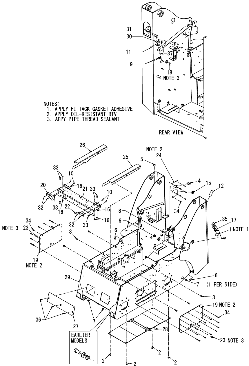
Fig.1. CHASSIS
