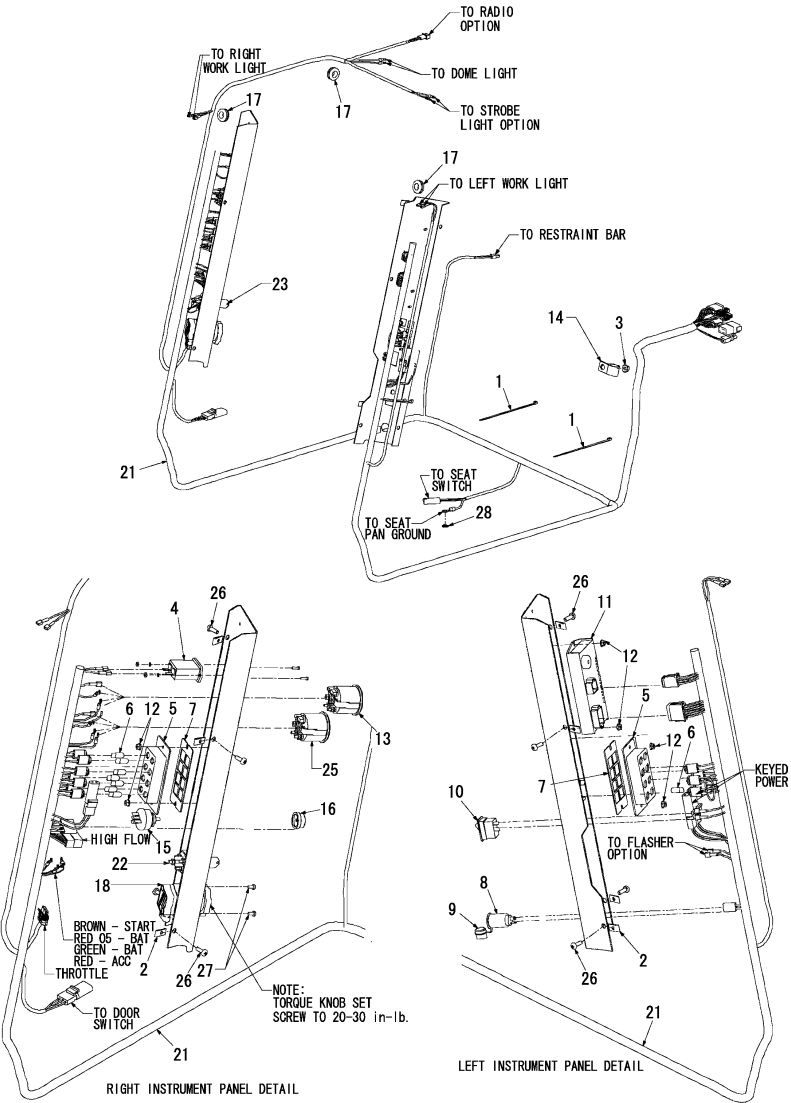
Fig.44. ELECTRICAL - ROPS/FOPS
