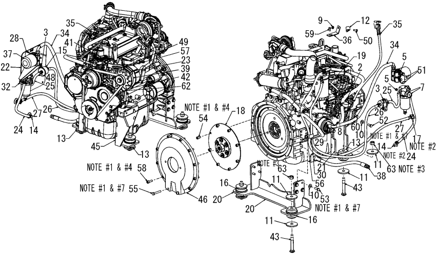
Fig.22. ENGINE
