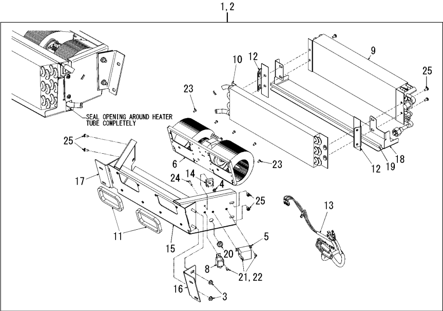
Fig.103. CONDENSOR, HEATER HOUSING AND HVAC HOUSING ASSEMBLY
