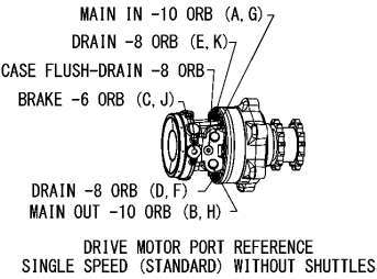
Fig.36. HYDROSTATIC SYSTEM WITH DRIVE MOTORS(S190R SINGLE-SPEED HAND/FOOT AND DUAL JOYST
