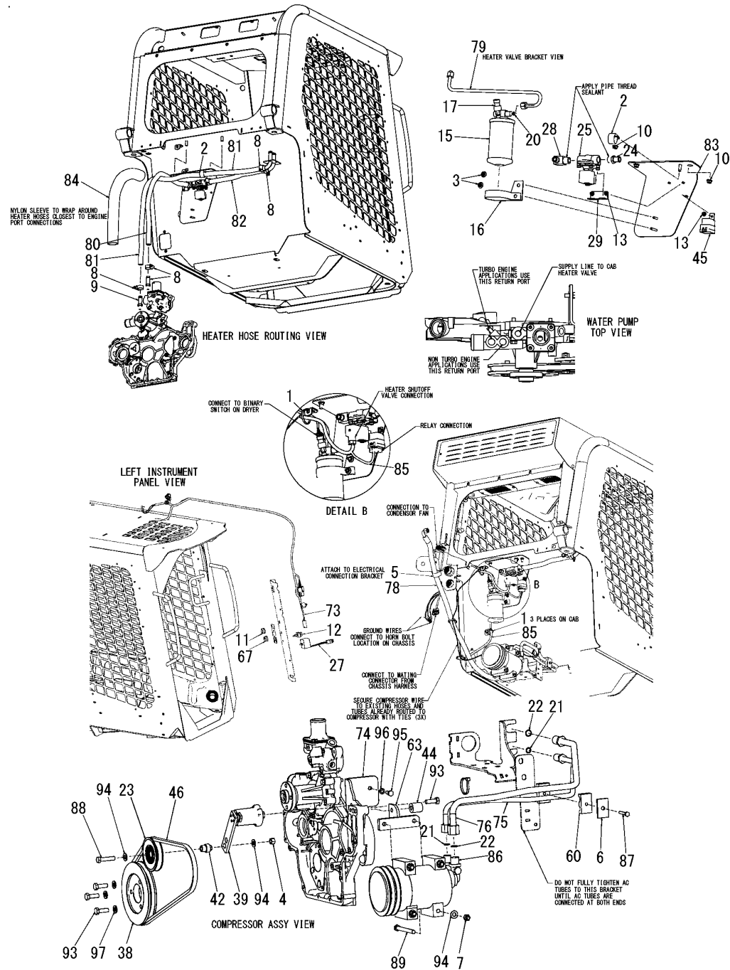
Fig.4. CHASSIS(HVAC
