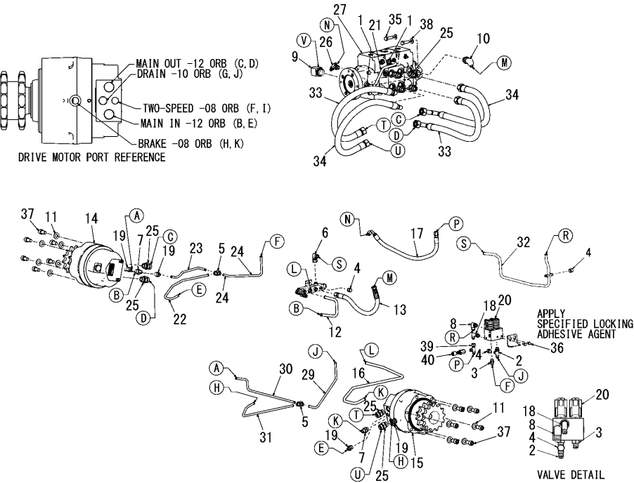
Fig.39. HYDROSTATIC SYSTEM WITH DRIVE MOTORS(S220R TWO-SPEED HAND/FOOT AND DUAL JOYSTICK
