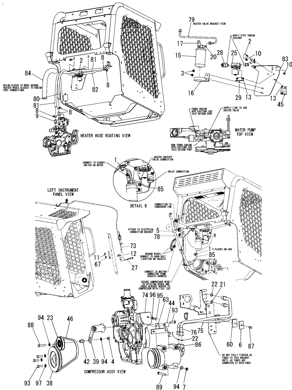
Fig.4. CHASSIS(HVAC
