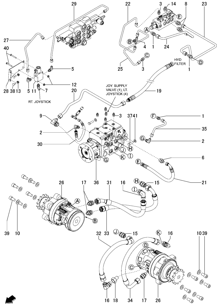
Fig.45. HYDROSTATICS WITH DRIVE MOTORS(1-SPEED JOYSTICK CONTROLS)
