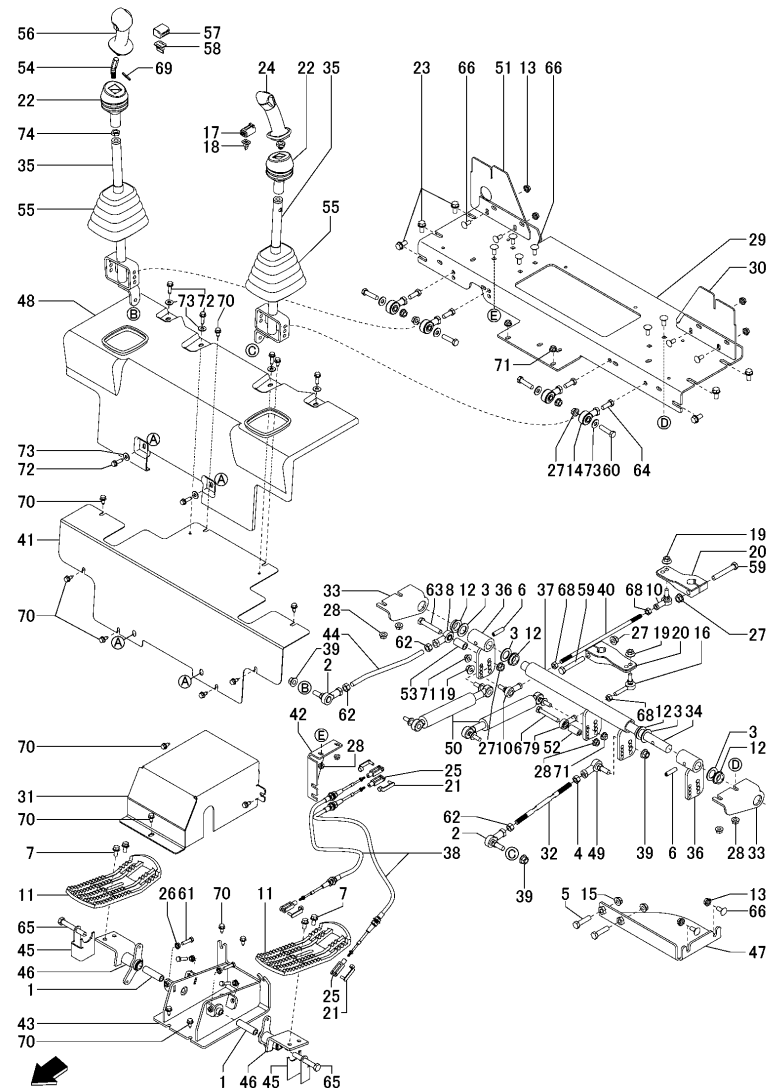
Fig.21. HAND-FOOT CONTROLS(1/2)
