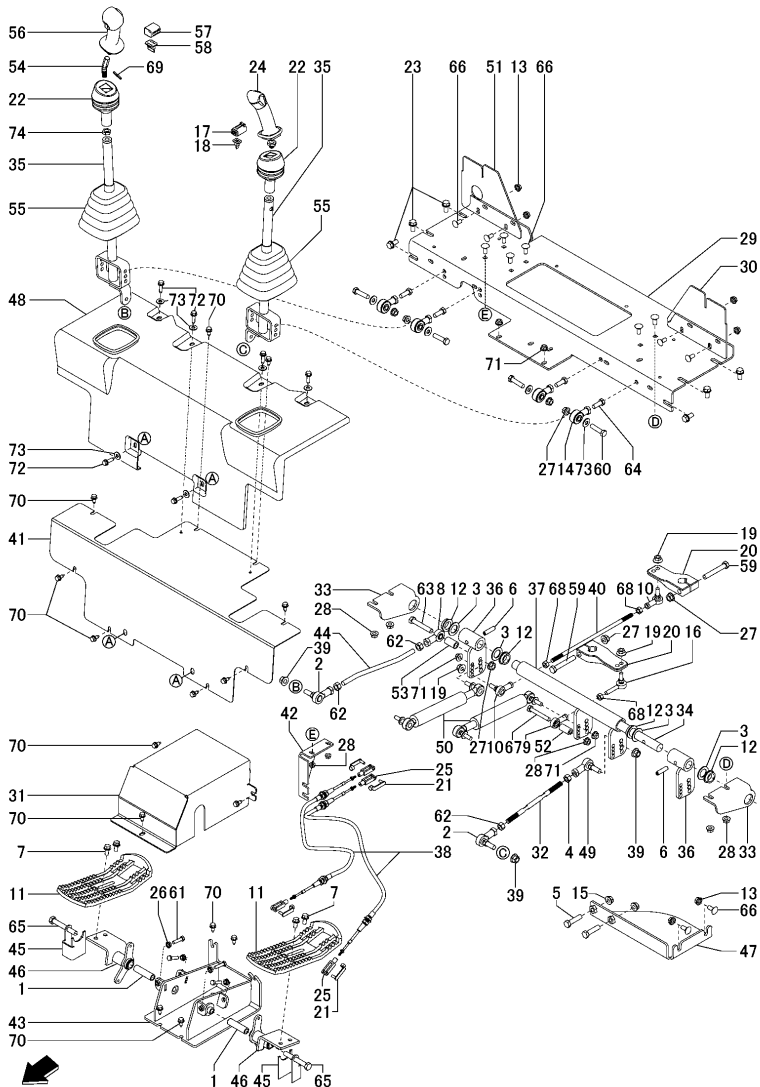
Fig.21. HAND-FOOT CONTROLS(1/2)
