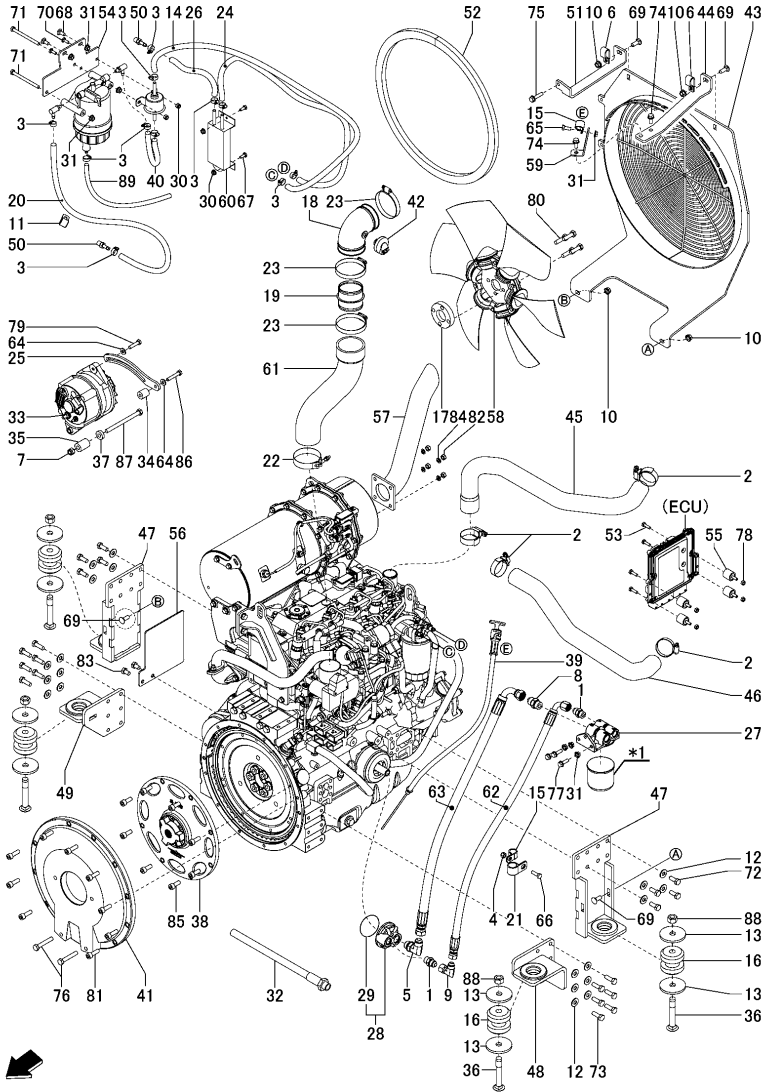
Fig.26. ENGINE
