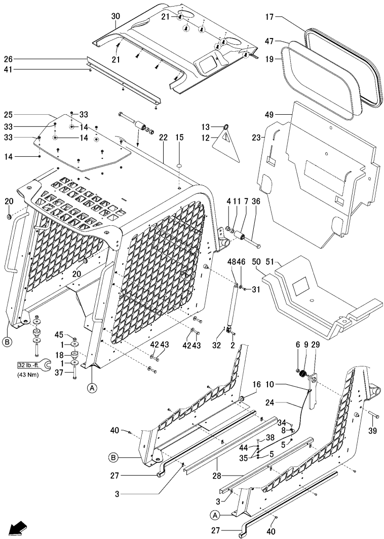
Fig.8. ROPS/FOPS ASSEMBLY
