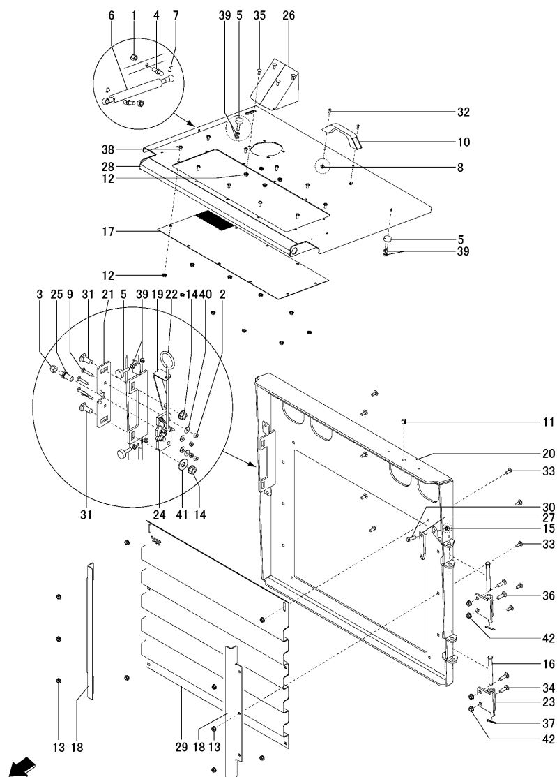
Fig.3. GRILLE & COVERS
