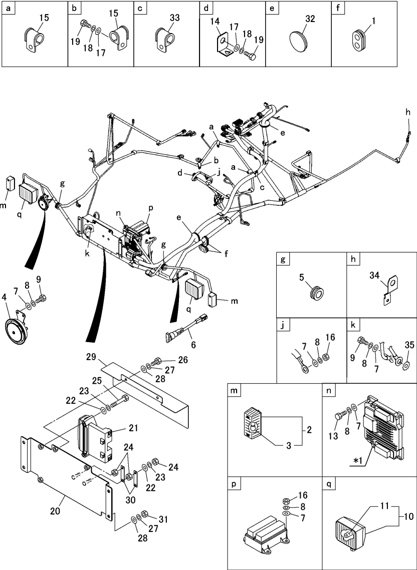
Fig.25. ELECTRIC PART(1/2)
