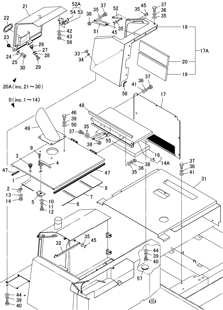
Fig.46. COVER(2/3)(CAB)
