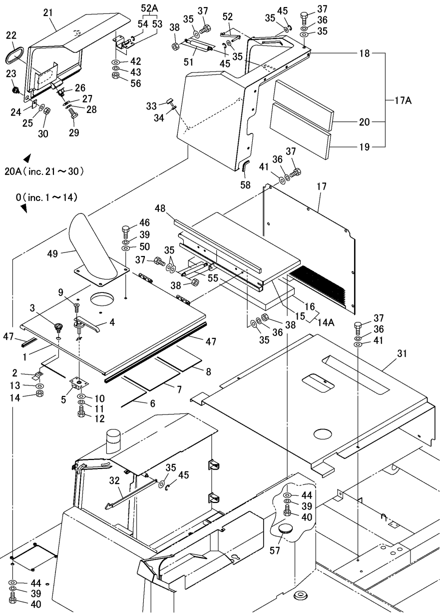
Fig.46. COVER(2/3)(CAB)
