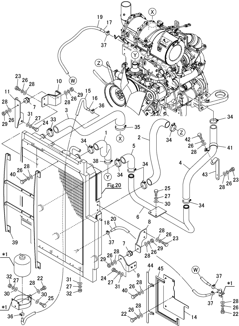
Fig.18. ENGINE & RELATED DEVICE(2/4)
