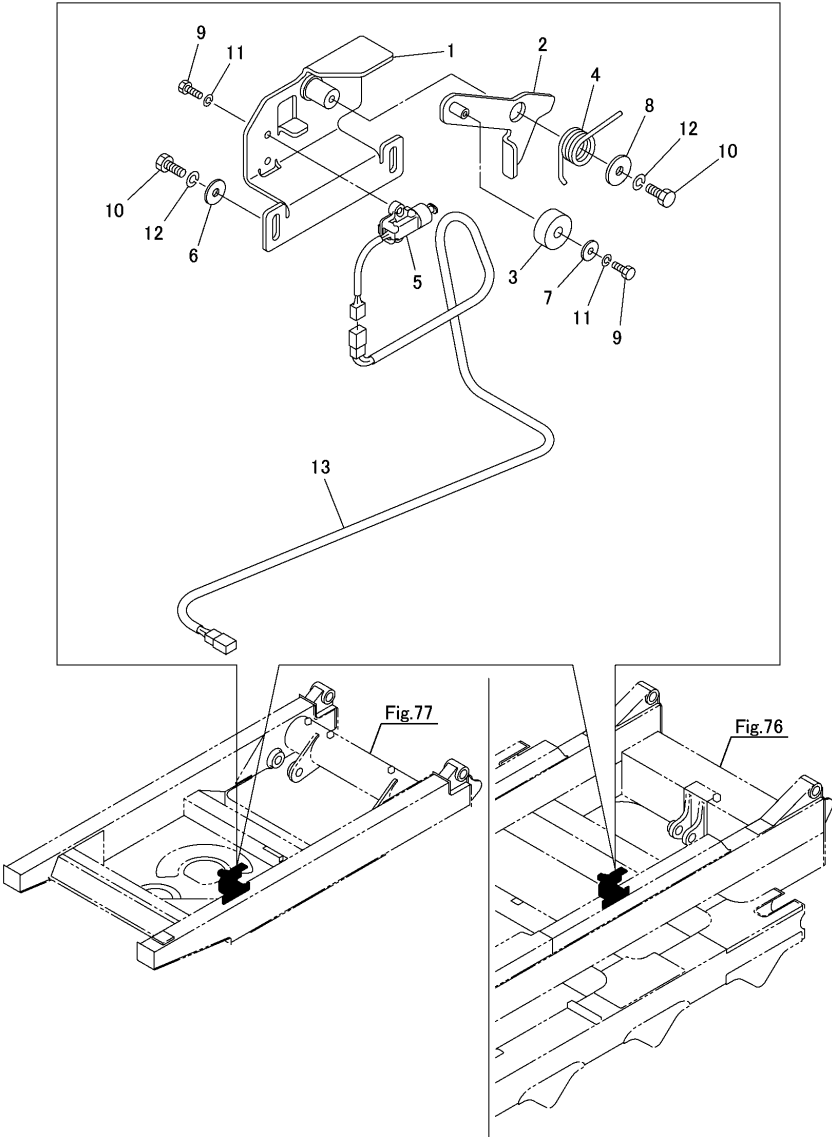
Fig.80. LIMIT SENSOR
