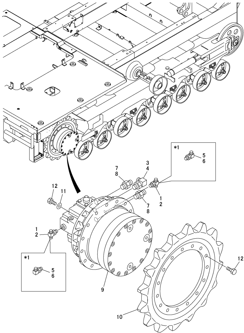
Fig.8. TRAVEL DEVICE
