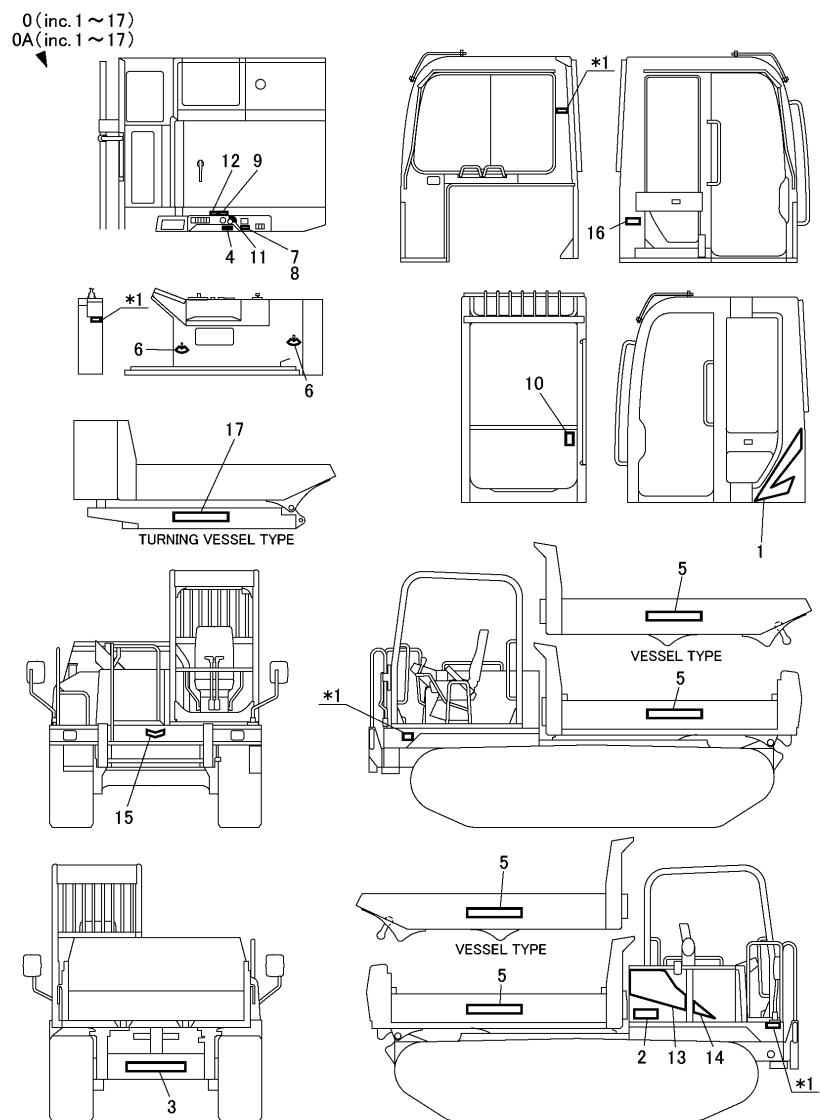
Fig.81. LABEL(1/2)
