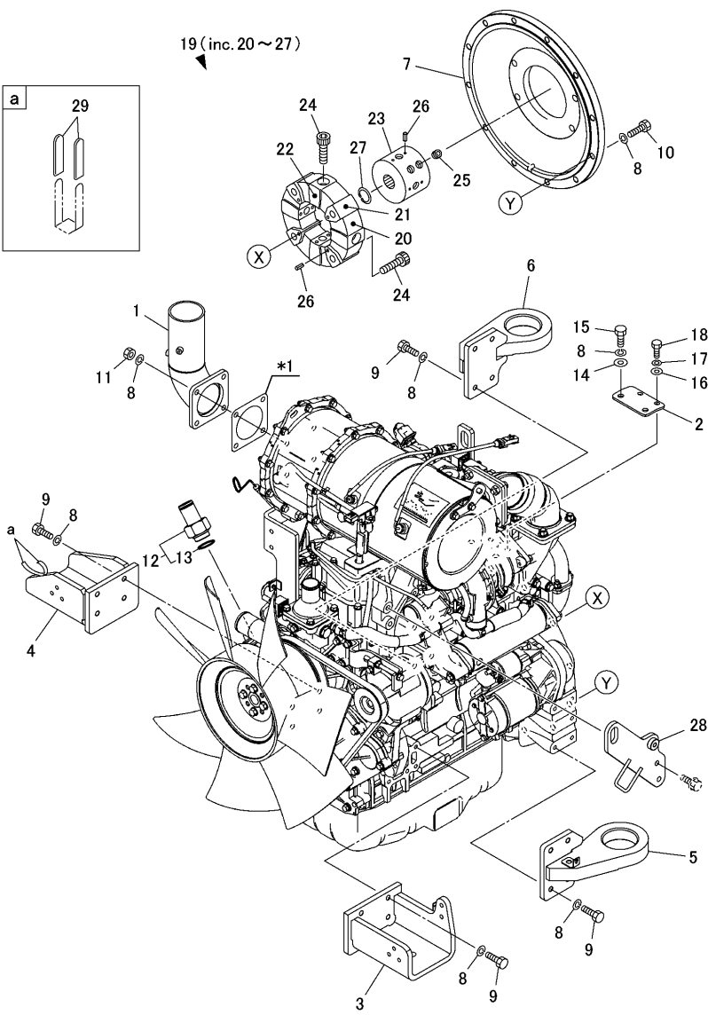
Fig.19. ENGINE & RELATED DEVICE(3/4)
