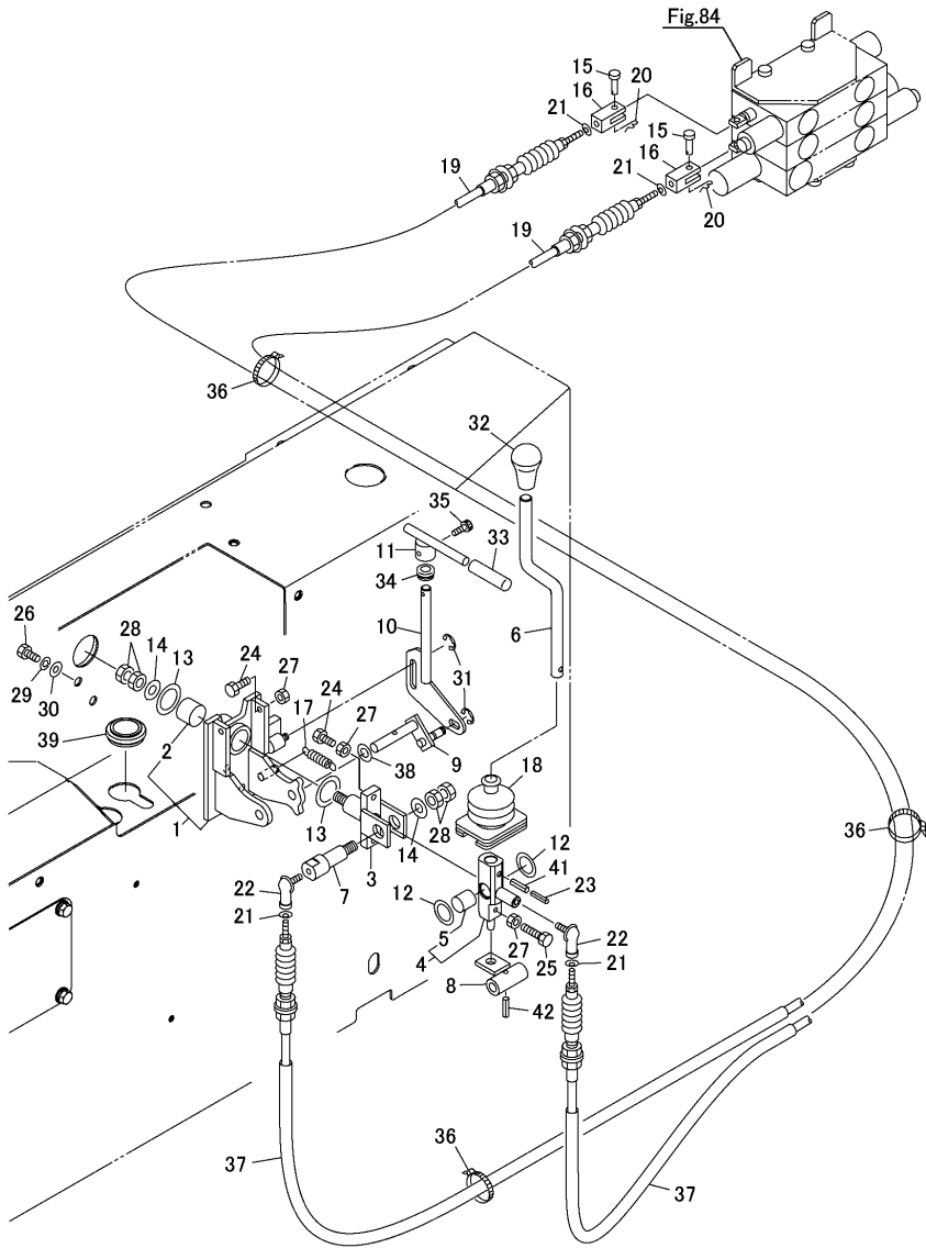
Fig.16. DUMP & TURNING LEVER(TURNING VESSEL SPEC.)
