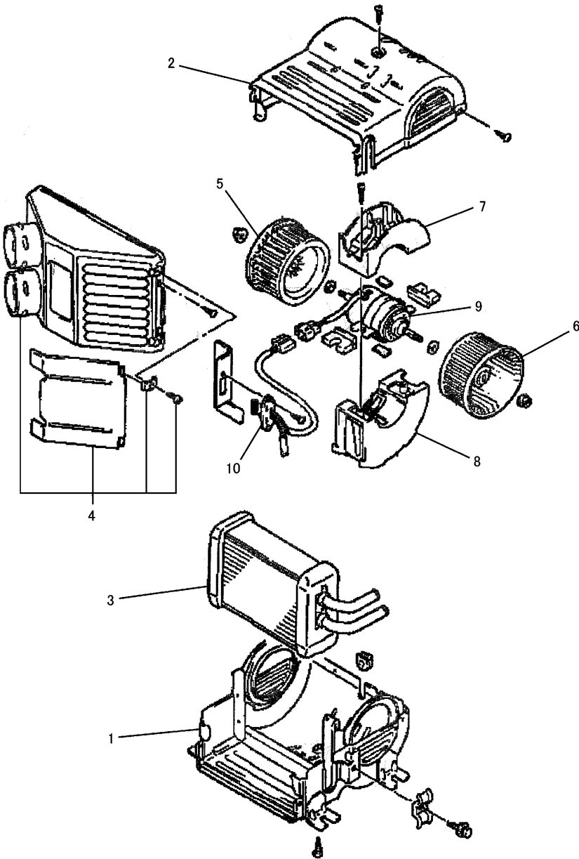
Fig.68. HEATER(2/2)
