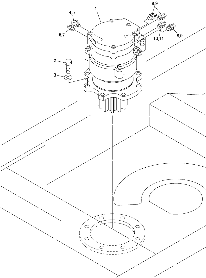
Fig.12. TURNING DEVICE(TURNING VESSEL SPEC.)
