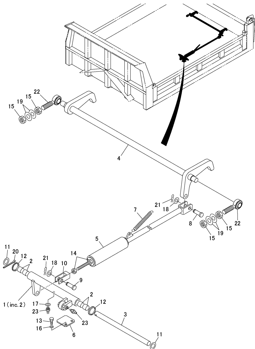
Fig.79. REAR LINK
