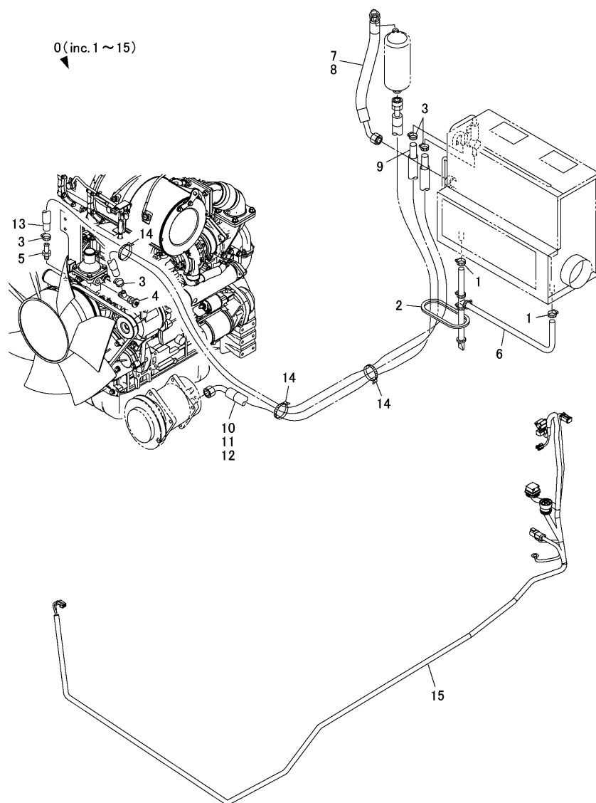
Fig.73. AIR CONDITIONER(3/4)(UNIT-2)
