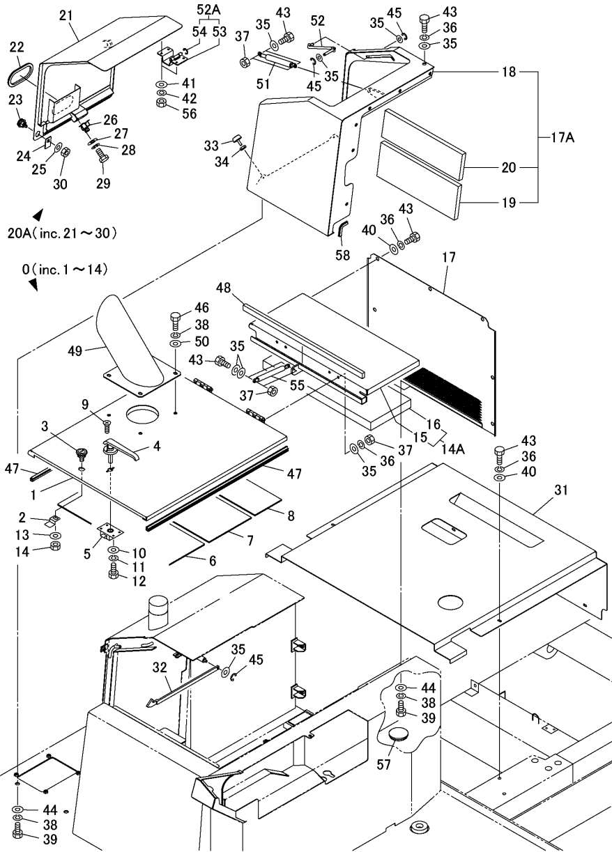
Fig.50. COVER(2/3)(CANOPY)
