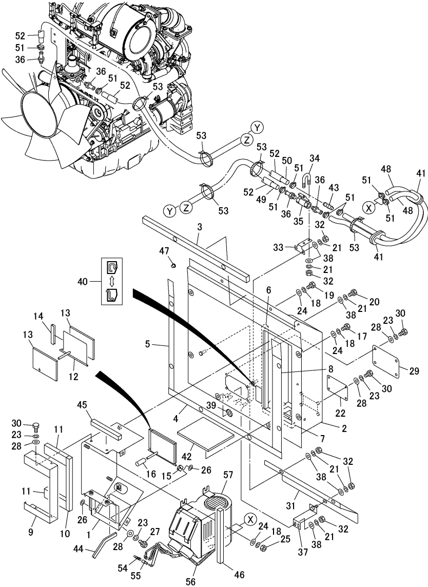
Fig.67. HEATER(1/2)
