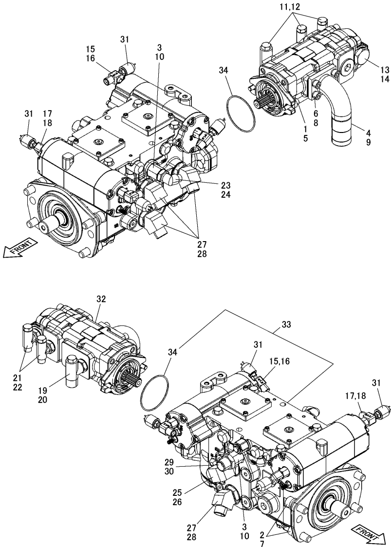
Fig.40. PUMP DRIVE
