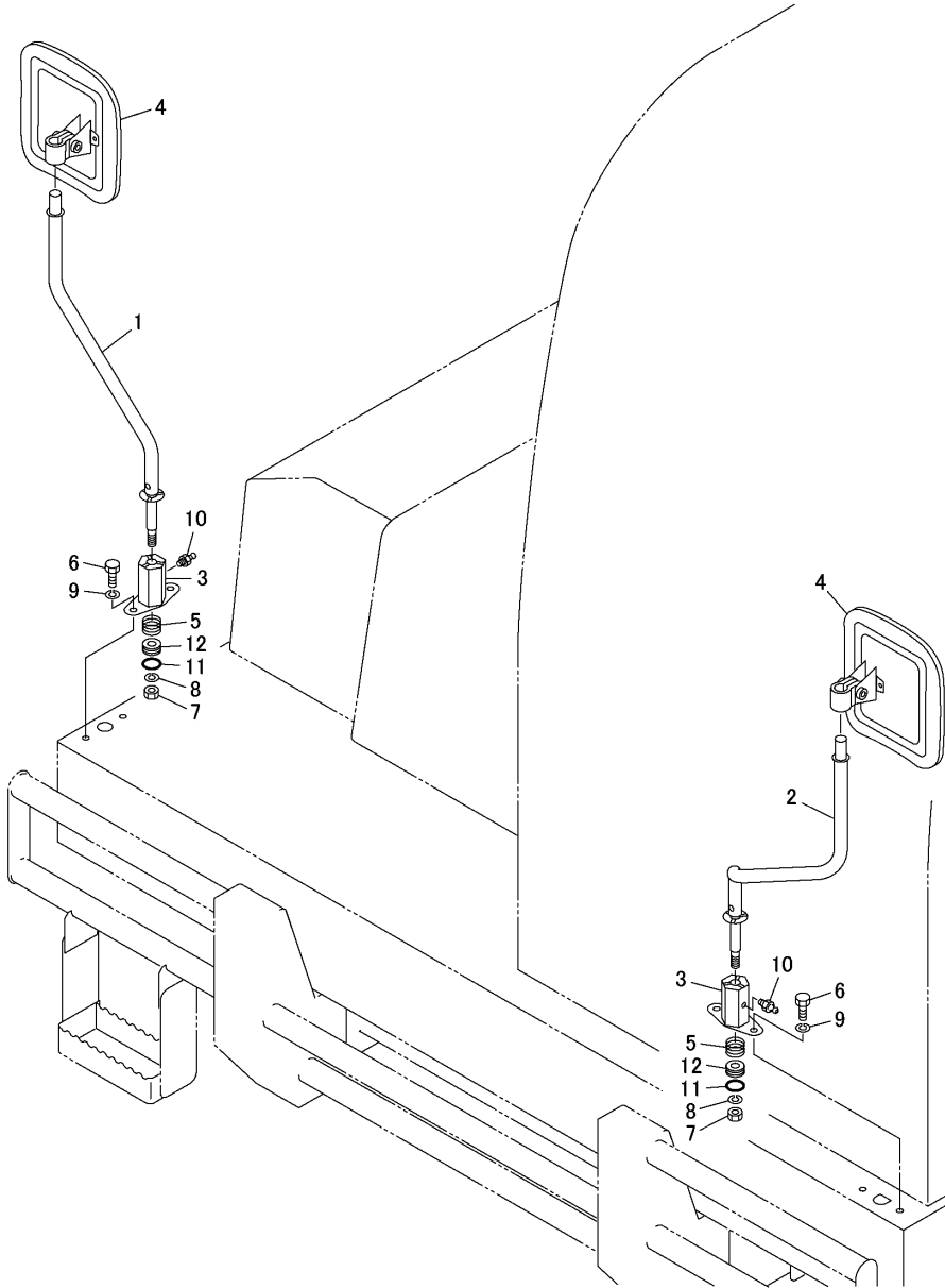
Fig.55. BACK MIRROR
