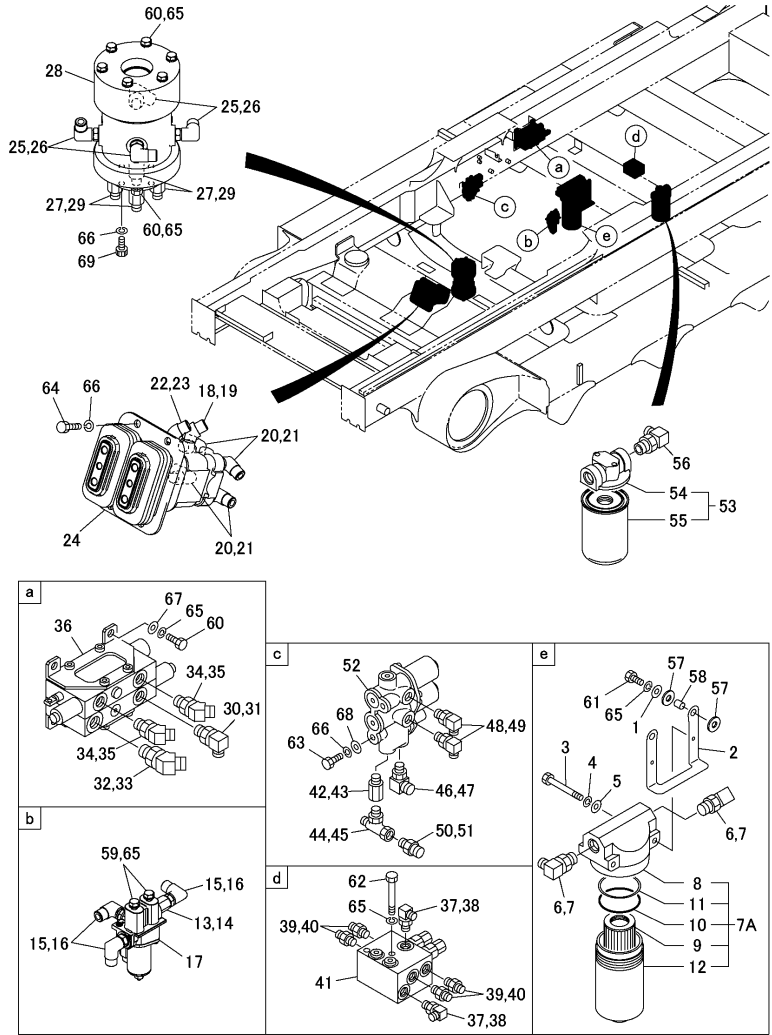
Fig.33. VALVE & ACCESSORY
