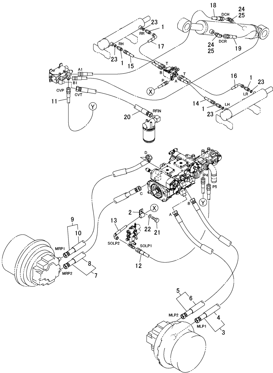
Fig.36. HYDRAULIC PIPING(2/2)
