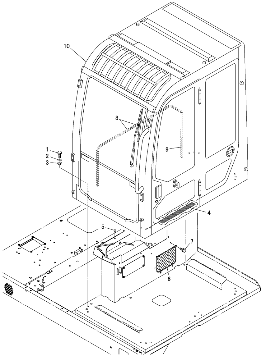
Fig.60. CAB MOUNTING
