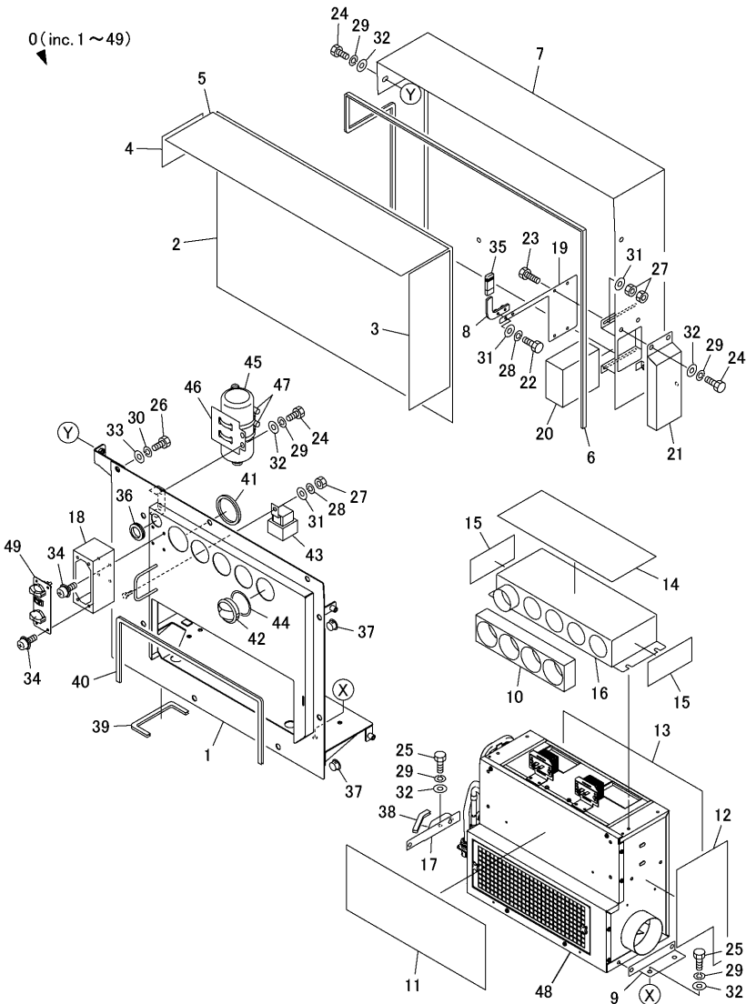
Fig.72. AIR CONDITIONER(3/4)(UNIT-1)
