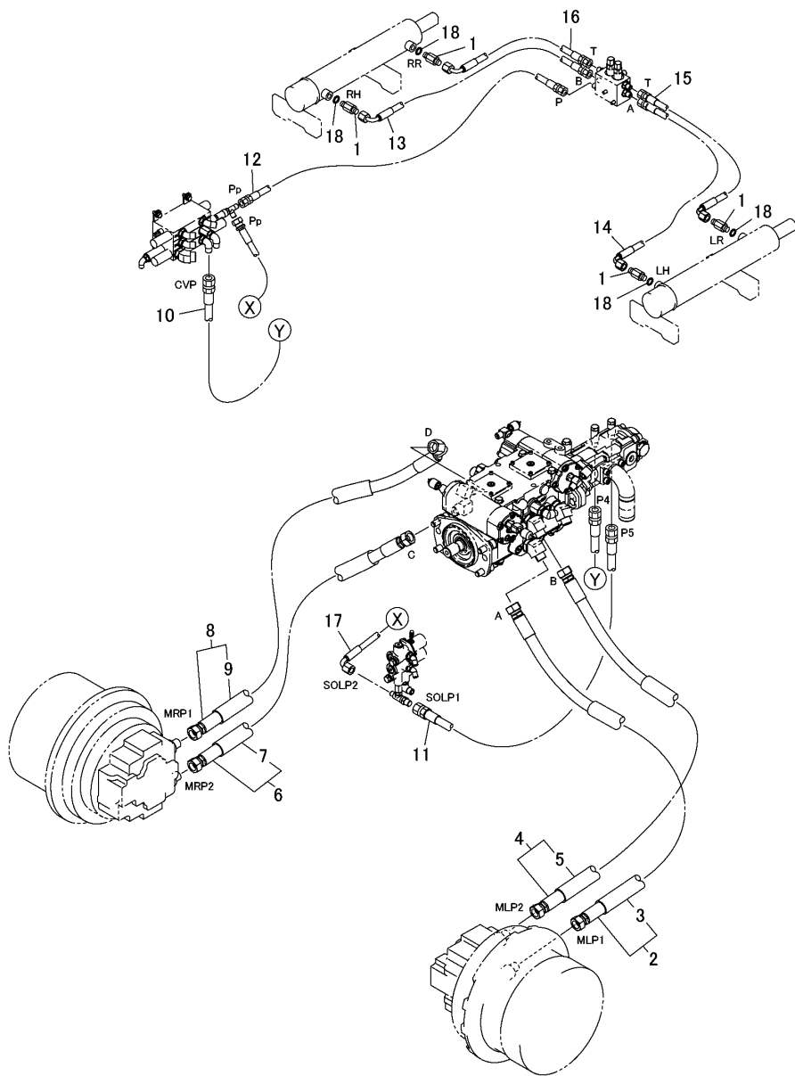
Fig.38. HYDRAULIC PIPING(2/2)(TURNING VESSEL SPEC.)
