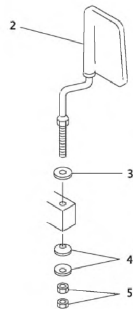
"A" DETAIL
