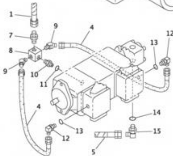
"A" 詳細 DETAIL
