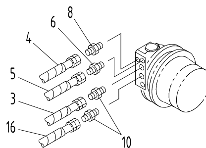
"B" DETAIL
