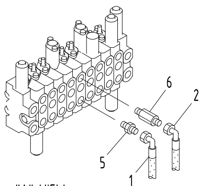
"A" VIEW
