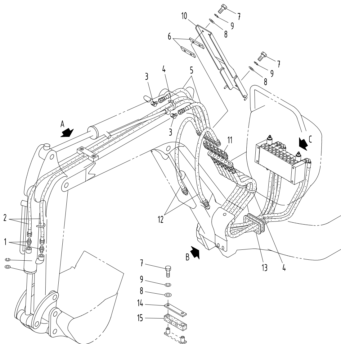
"A" DETAIL
