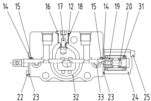
"F" DETAIL
