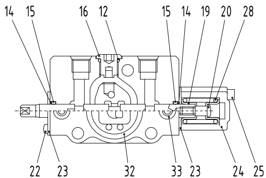
"E" DETAIL
