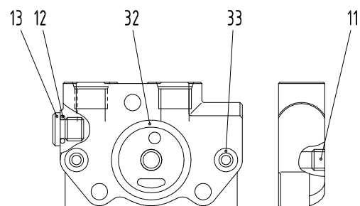
"H" DETAIL
