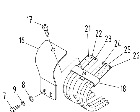
"A" DETAIL
