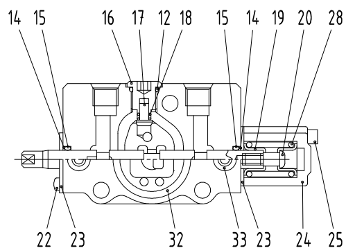
"H" DETAIL
