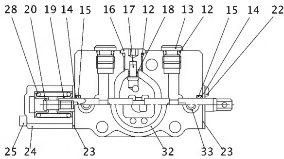
"G" 詳細 DETAIL
