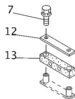
"A" 詳細 DETAIL
