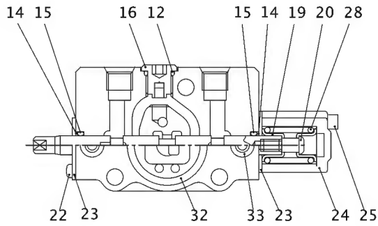
"E" 詳細 DETAIL
