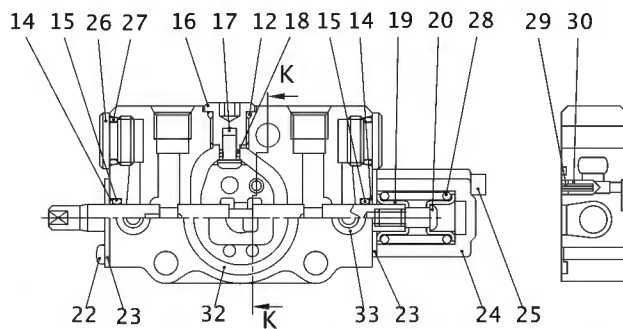
"C" 詳細 DETAIL
