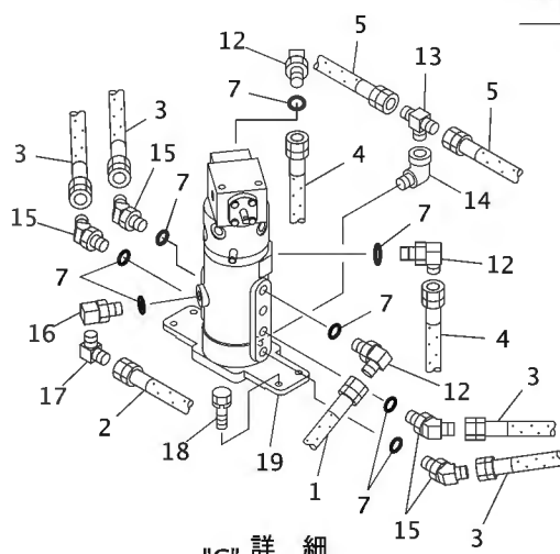
"C" 詳細 DETAIL
