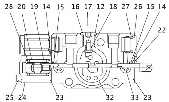
"D" 詳細 DETAIL
