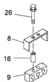
"G" DETAIL
