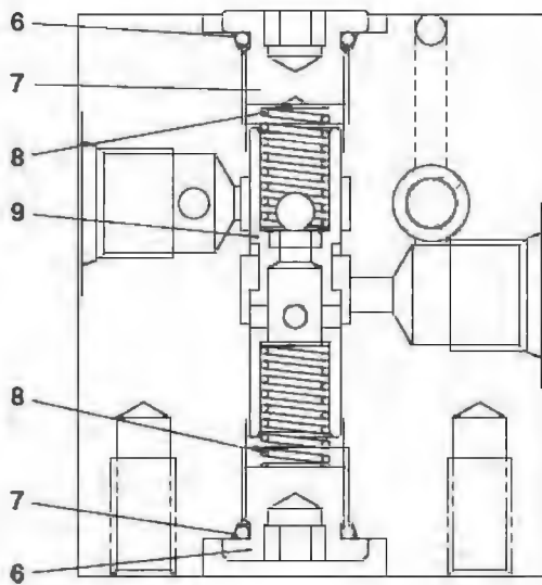
"B-B" SECTION
