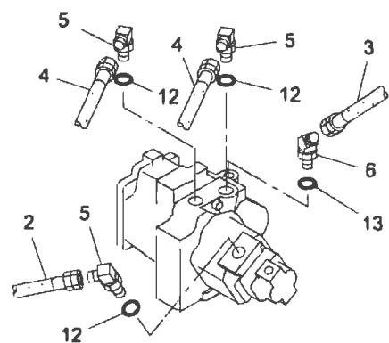
"F" DETAIL
