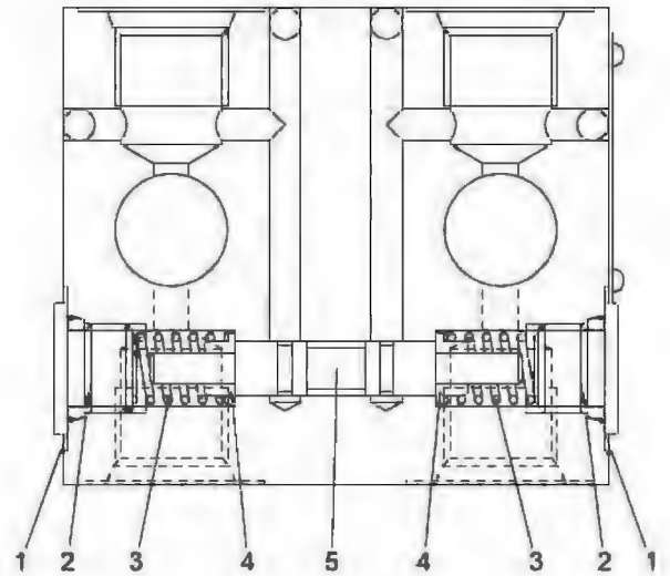
"A-A" SECTION
