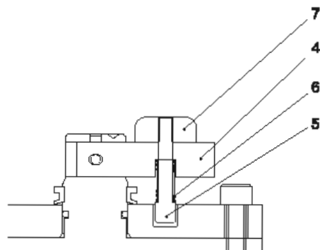
"A" SECTION
