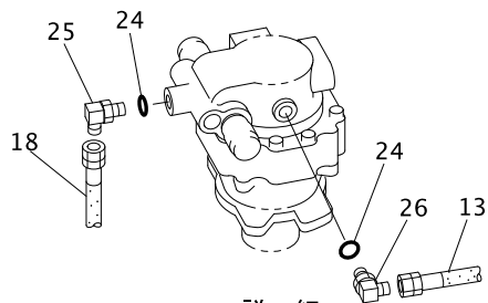
"C" 詳細 DETAIL
