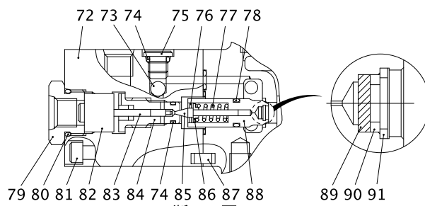
"N-N" 断面 SECTION
