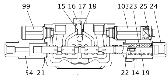
"O-O" 断面 SECTION
