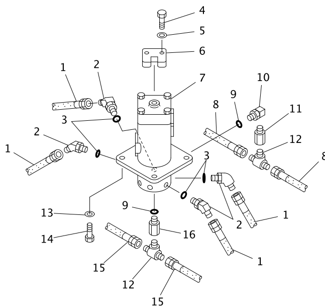
"A" 詳細 DETAIL
