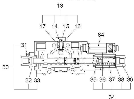
"K-K" SECTION
