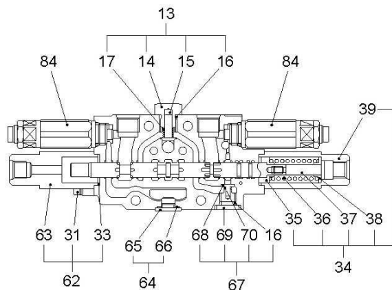
"G-G" SECTION
