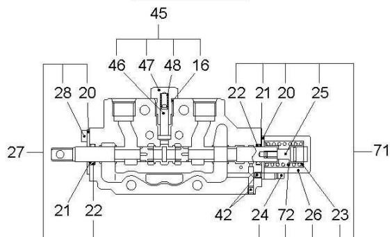
"H-H" SECTION
