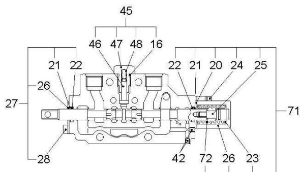
"H-H" SECTION
