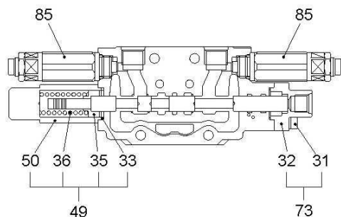
"I-I" SECTION
