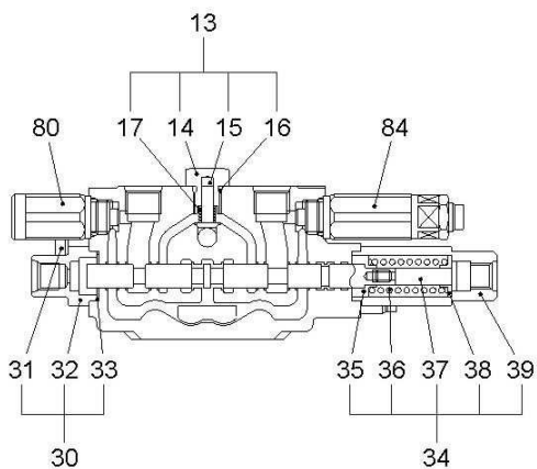
"M-M" SECTION
