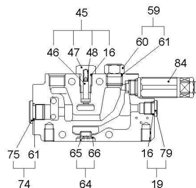
"L-L" SECTION
