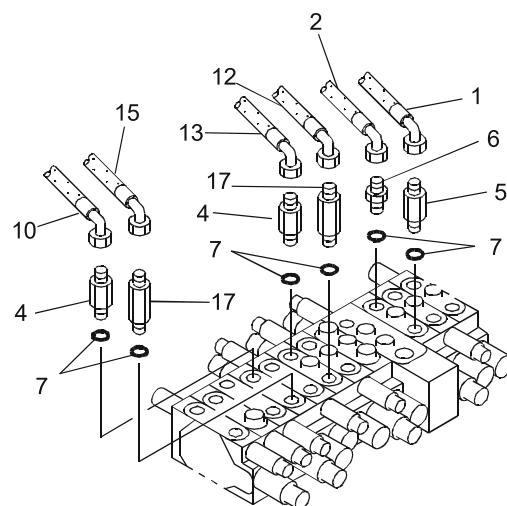
"D" DETAIL
