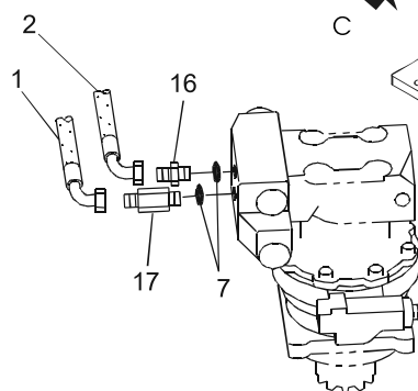
"A" DETAIL
