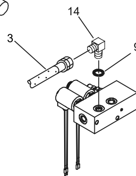
"B" DETAIL
