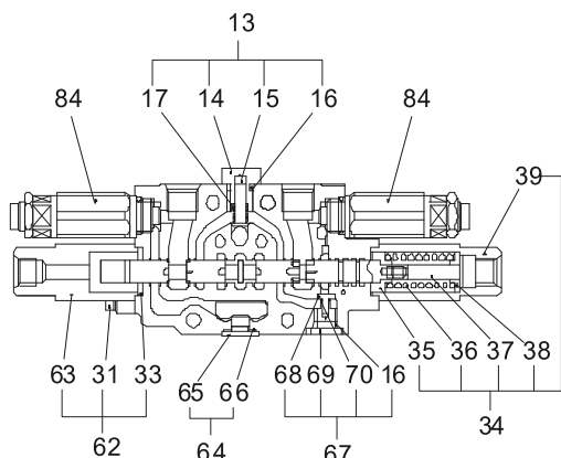
"G-G"SECTION
