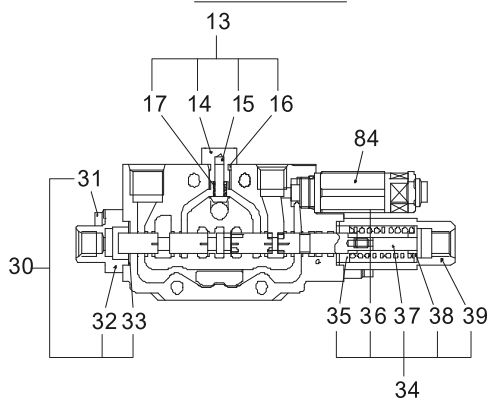
"K-K"SECTION
