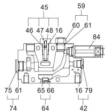
"L-L"SECTION
