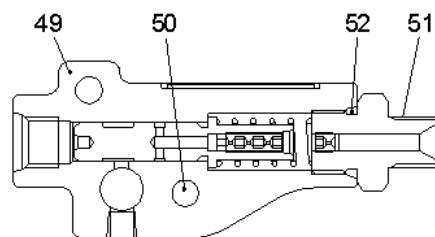
"E-E" SECTION
