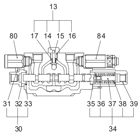
"M-M"SECTION
