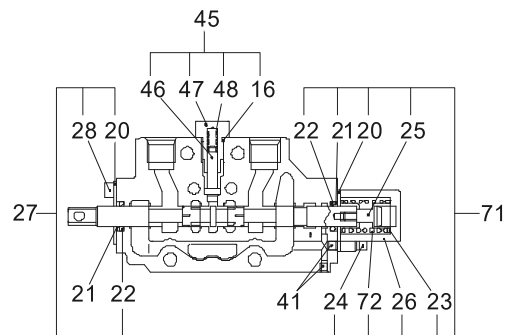
"H-H"SECTION
