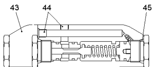
"C-C" SECTION
