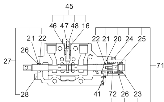
"H-H"SECTION
