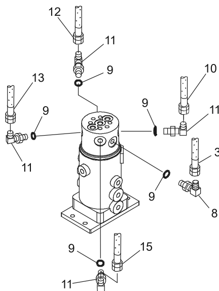
"C" DETAIL
