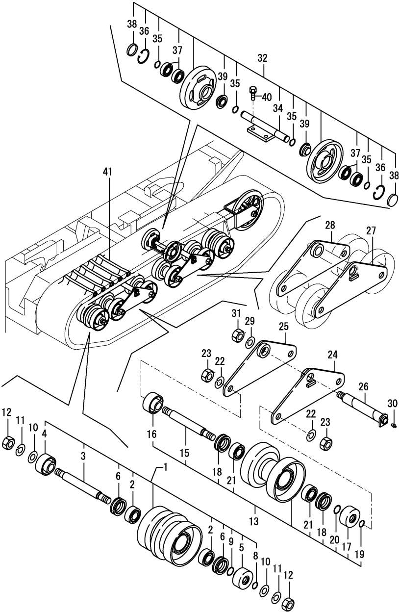
Fig.24. ROLLER & CRAWLER
