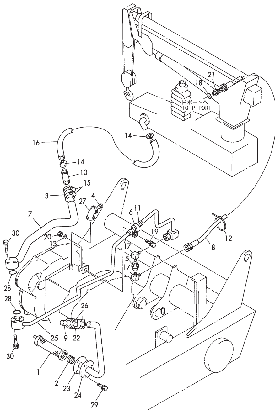
Fig. 69 油圧配管 (C30R-1K) HYD. OIL PIPING (C30R-1K)
