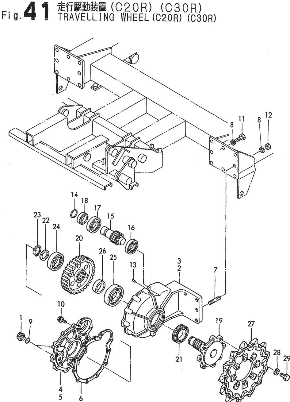
Fig.41. TRAVELLING WHEEL(C20R)(C30R)
