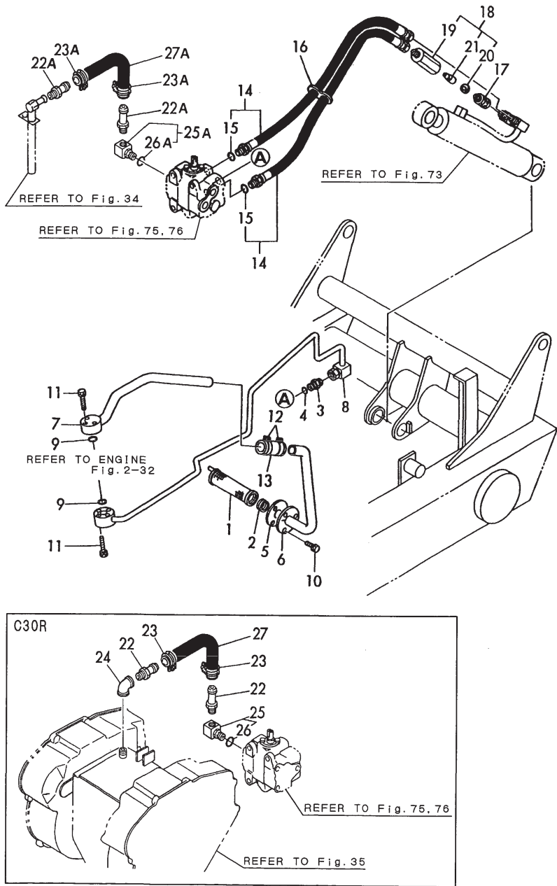
Fig.67 油圧配管 (C25W) (C30R) HYD.OIL PIPING (C25W) (C30R)
