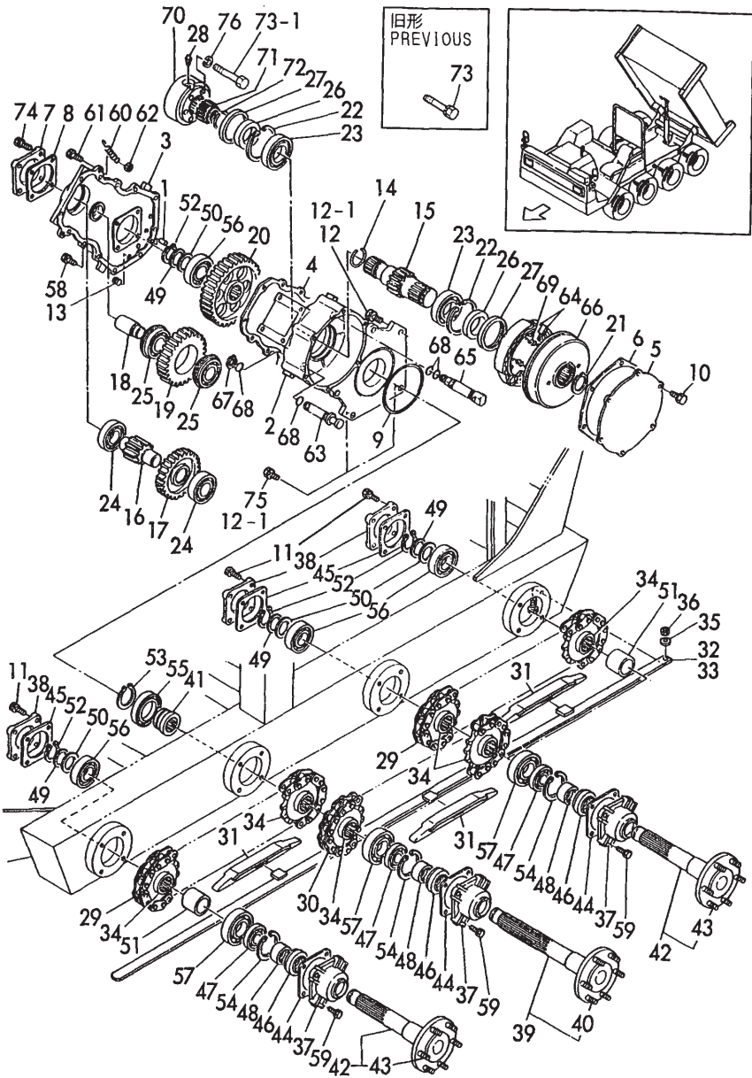
Fig.40 走行駆動装置 (C25W) TRAVELLING WHEEL (C25W)
