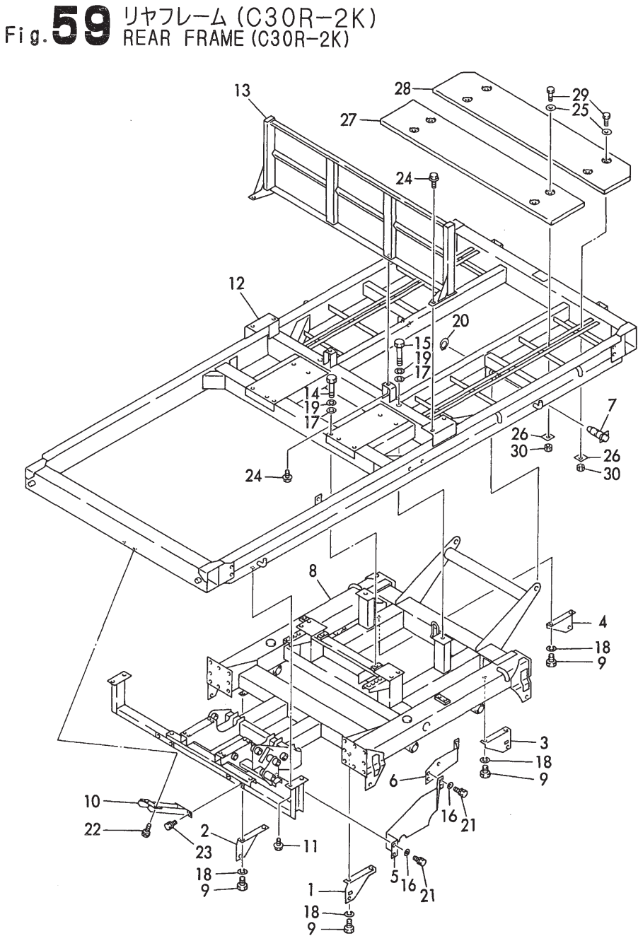
Fig.59. REAR FRAME(C30R-2K)
