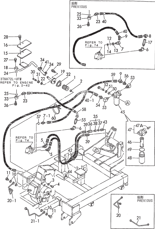
Fig.66 油圧配管 (C20R) HYD.OIL PIPING (C20R)
