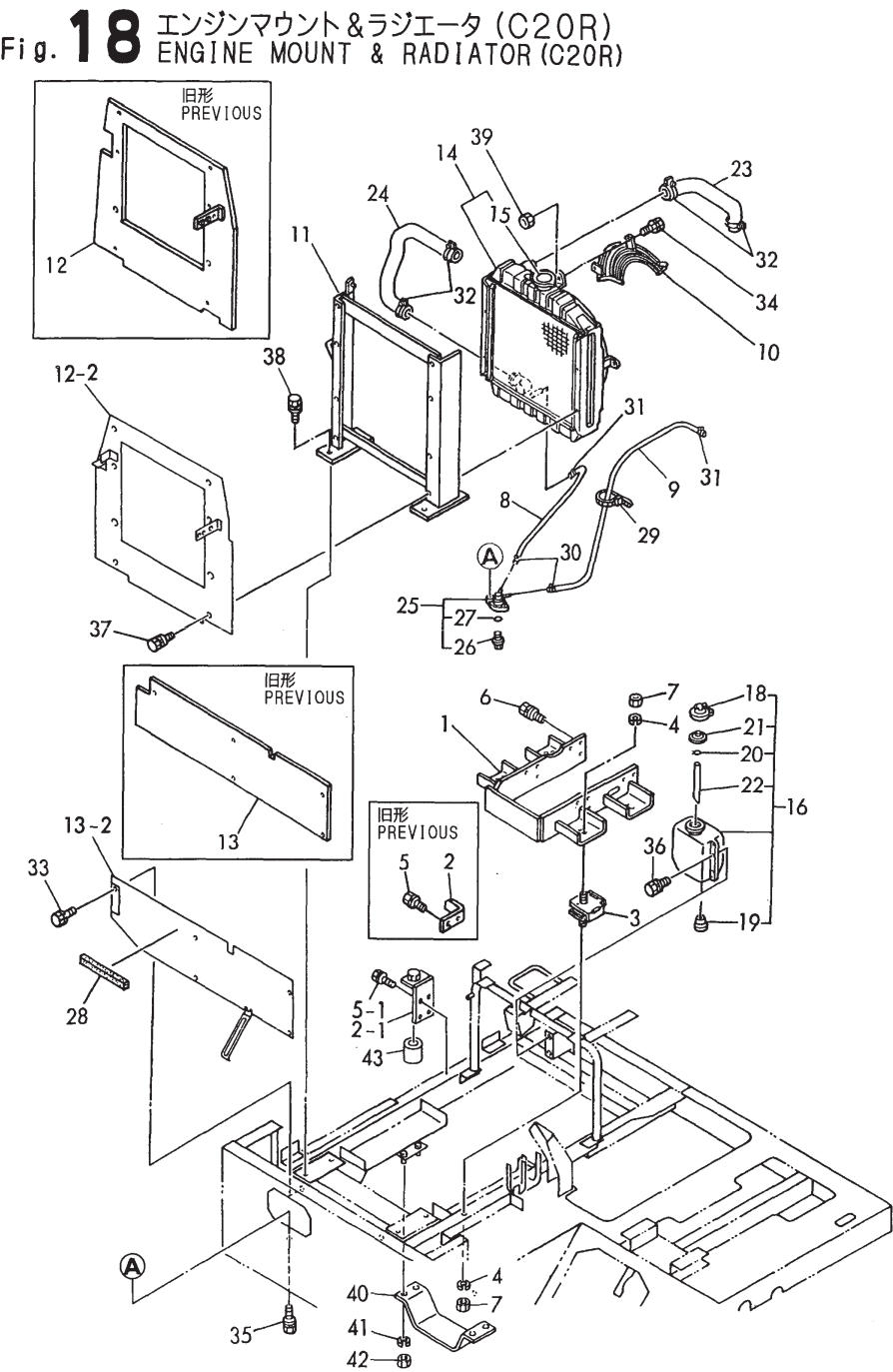
Fig.18. ENGINE MOUNT & RADIATOR(C20R)
