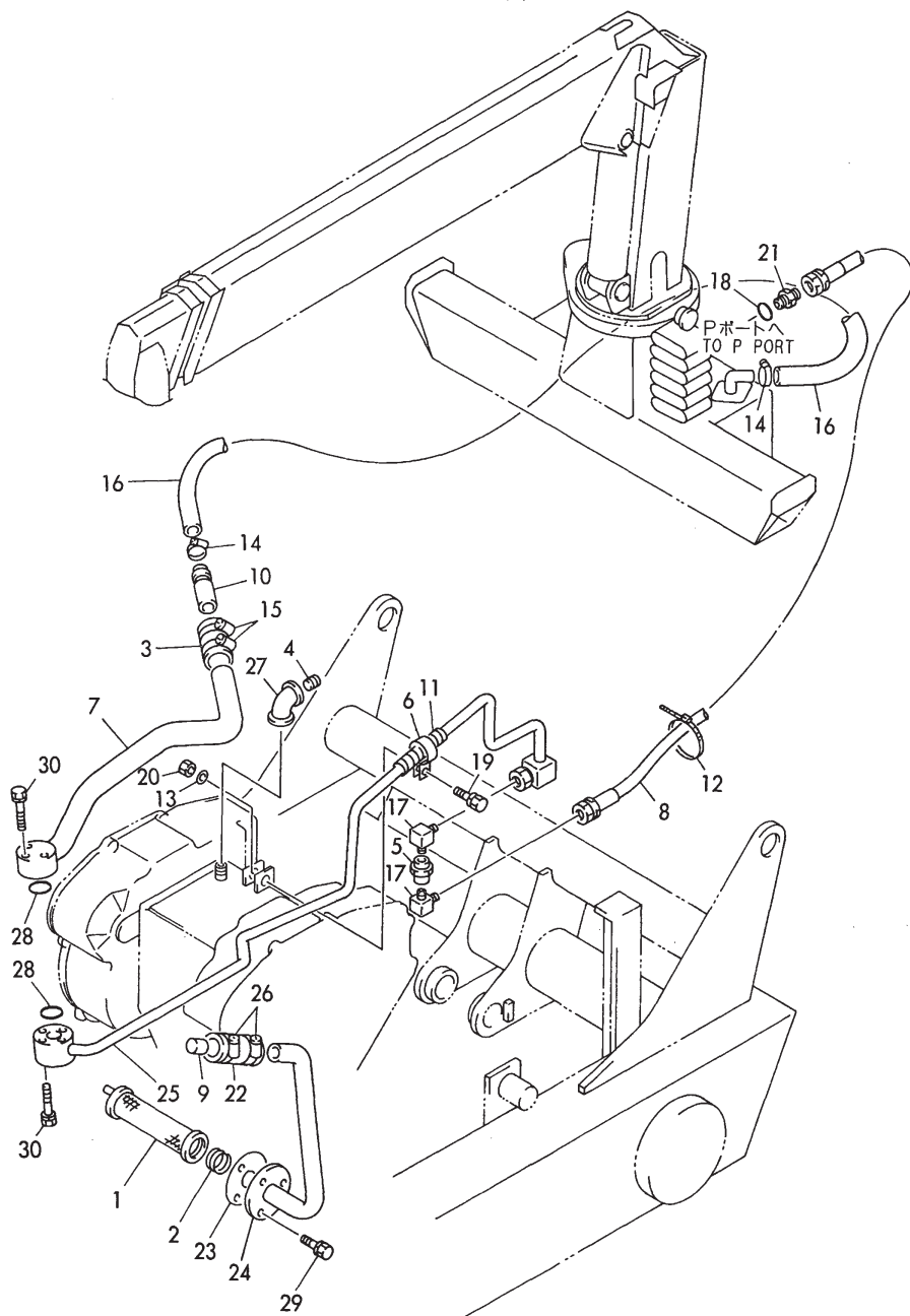
Fig. 70 油圧配管 (C30R-2K) HYD. OIL PIPING (C30R-2K)
