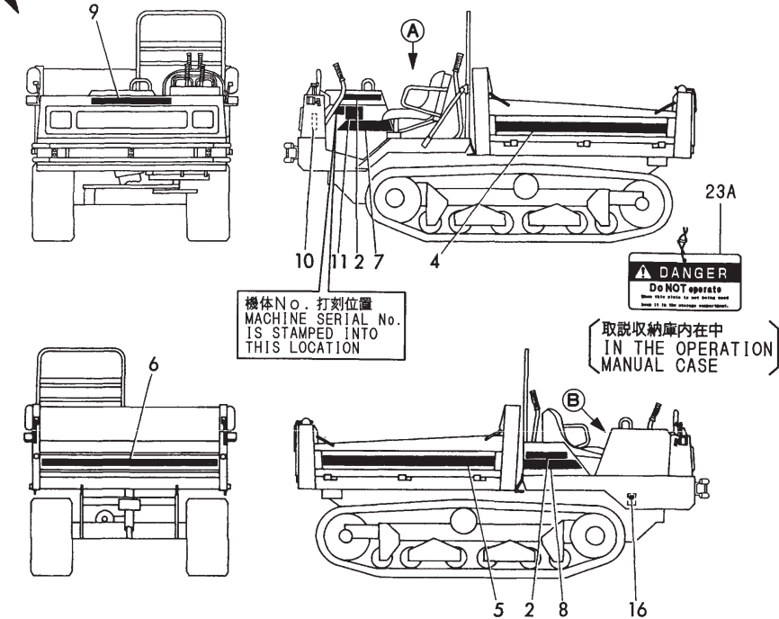
Fig.8 銘板 (C30R) (UK) LABEL (C30R) (UK)
