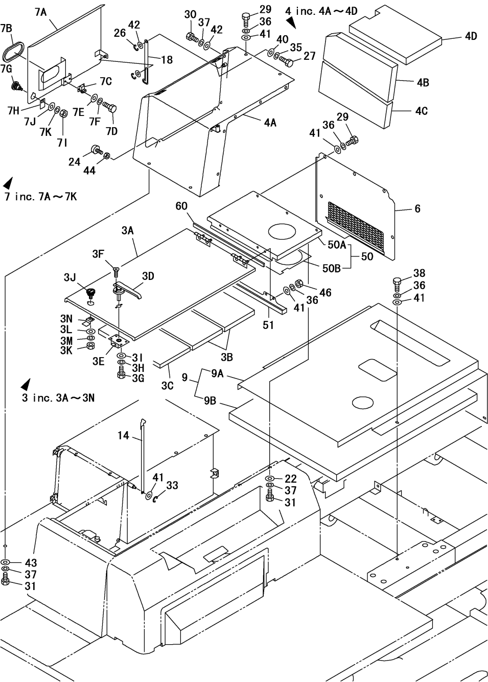
Fig.44. COVER(2/4)
