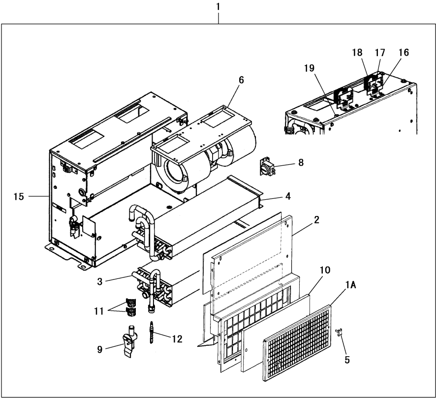
Fig.64. COOLER(4/5)(COOLER UNIT:2)
