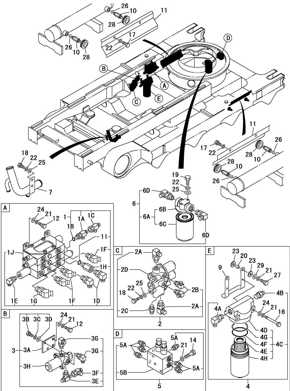
Fig.33. VALVE(TURNING)
