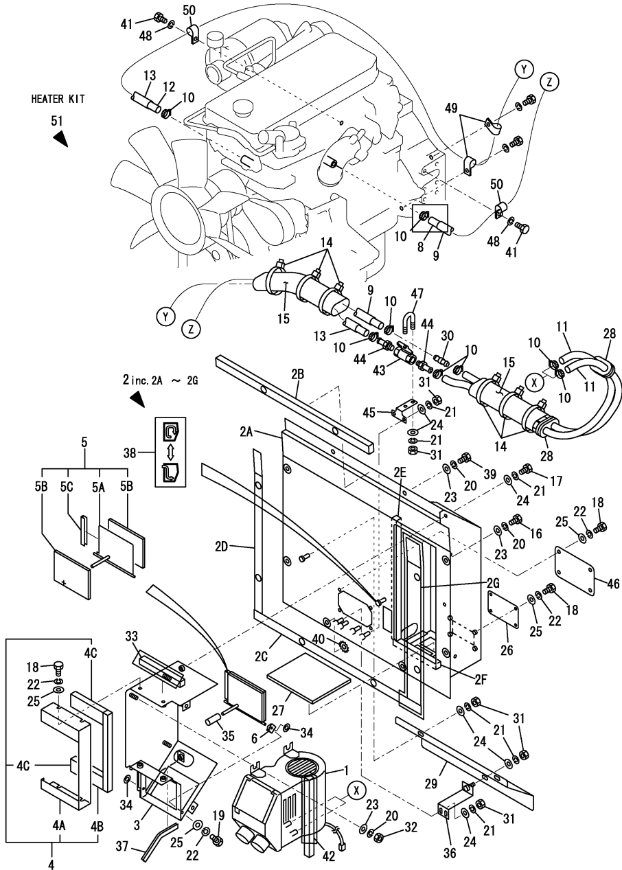
Fig.59. HEATER
