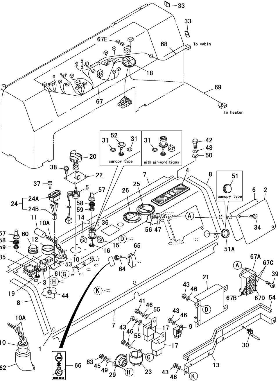
Fig.19. CONTROL BOX
