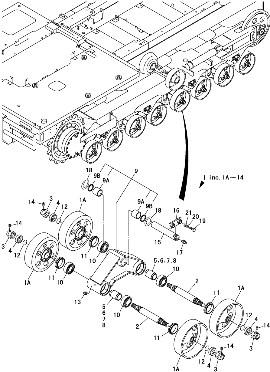
Fig.5. TRUCK ROLLER
