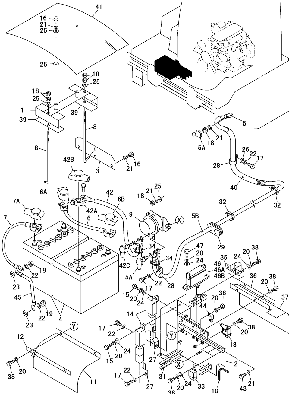
Fig.21. BATTERY
