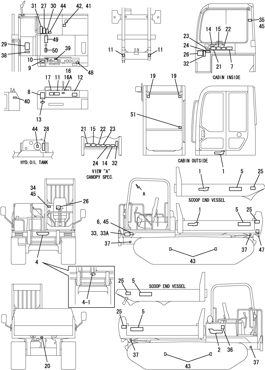
Fig.72. LABEL(1/2)
