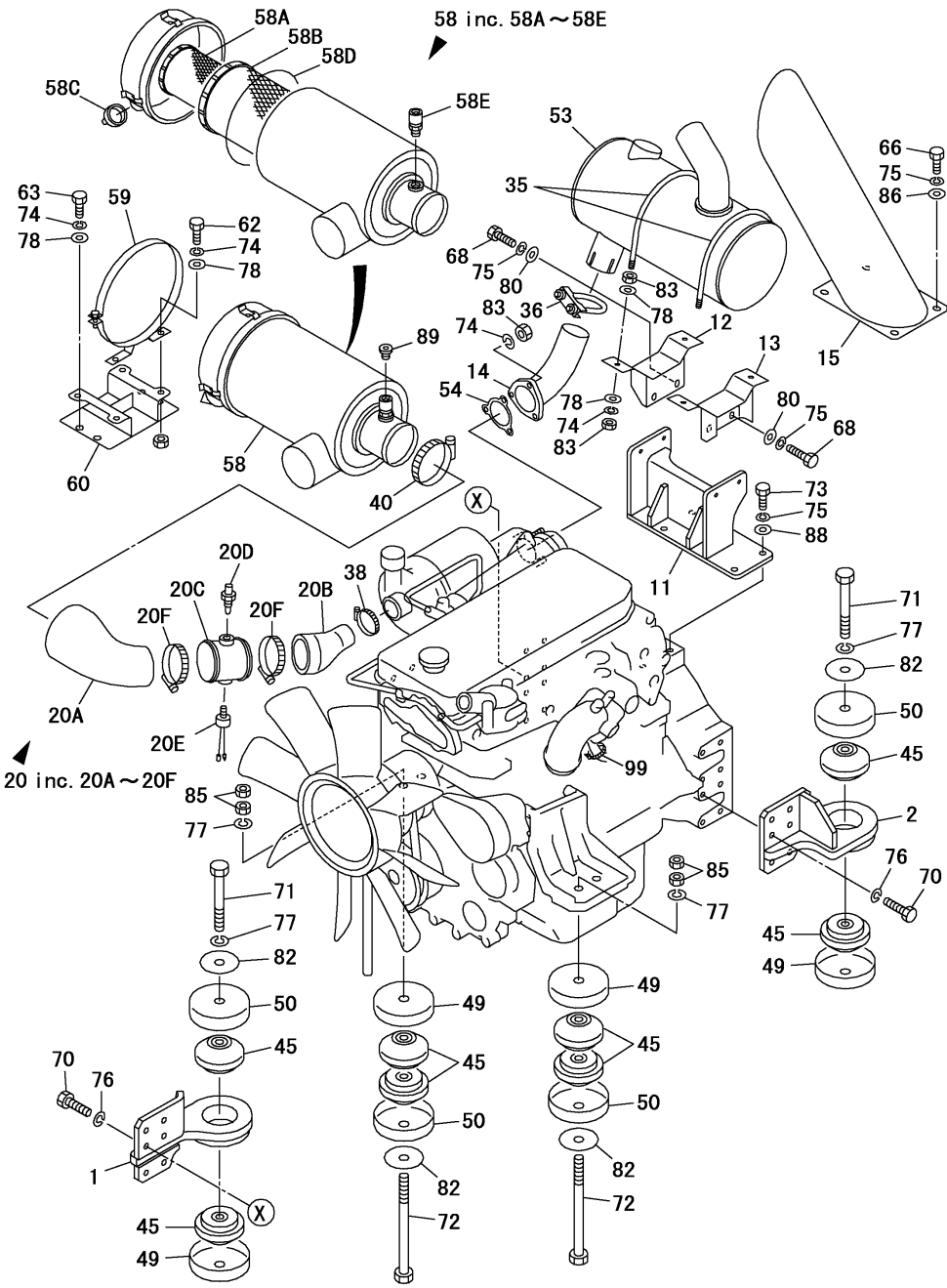
Fig.16. ENGINE & RELATED DEVICE(1/3)
