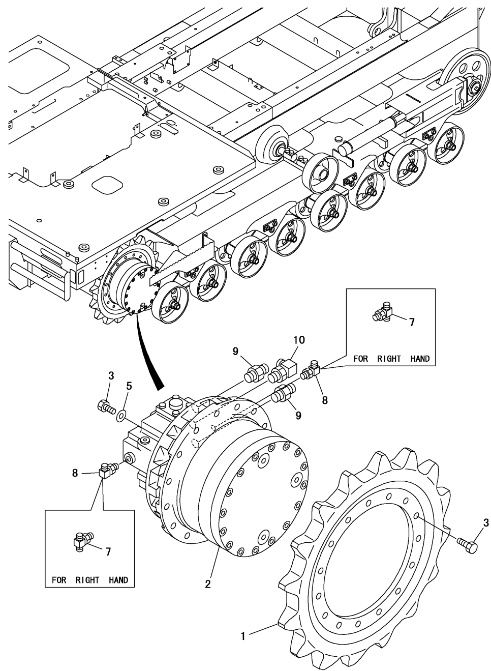
Fig.8. TRAVEL DEVICE
