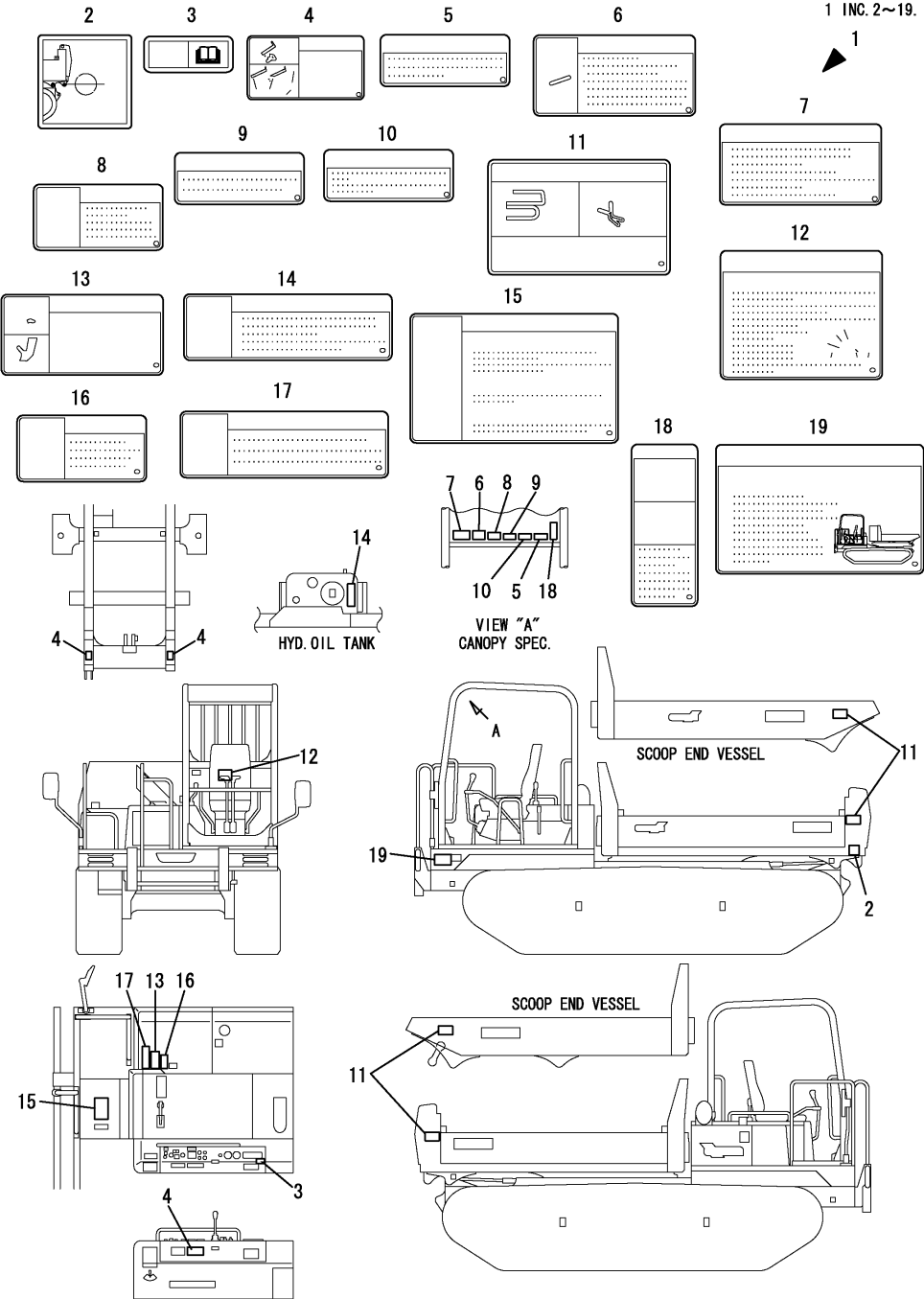
Fig.103. (73A)SAFETY LABEL(CANOPY)
