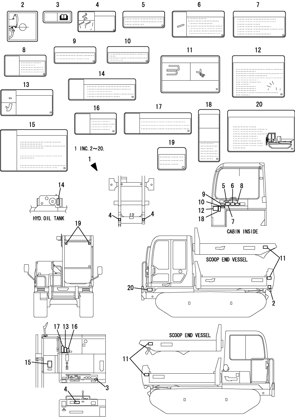
Fig.104. (73B)SAFETY LABEL(CABIN)
