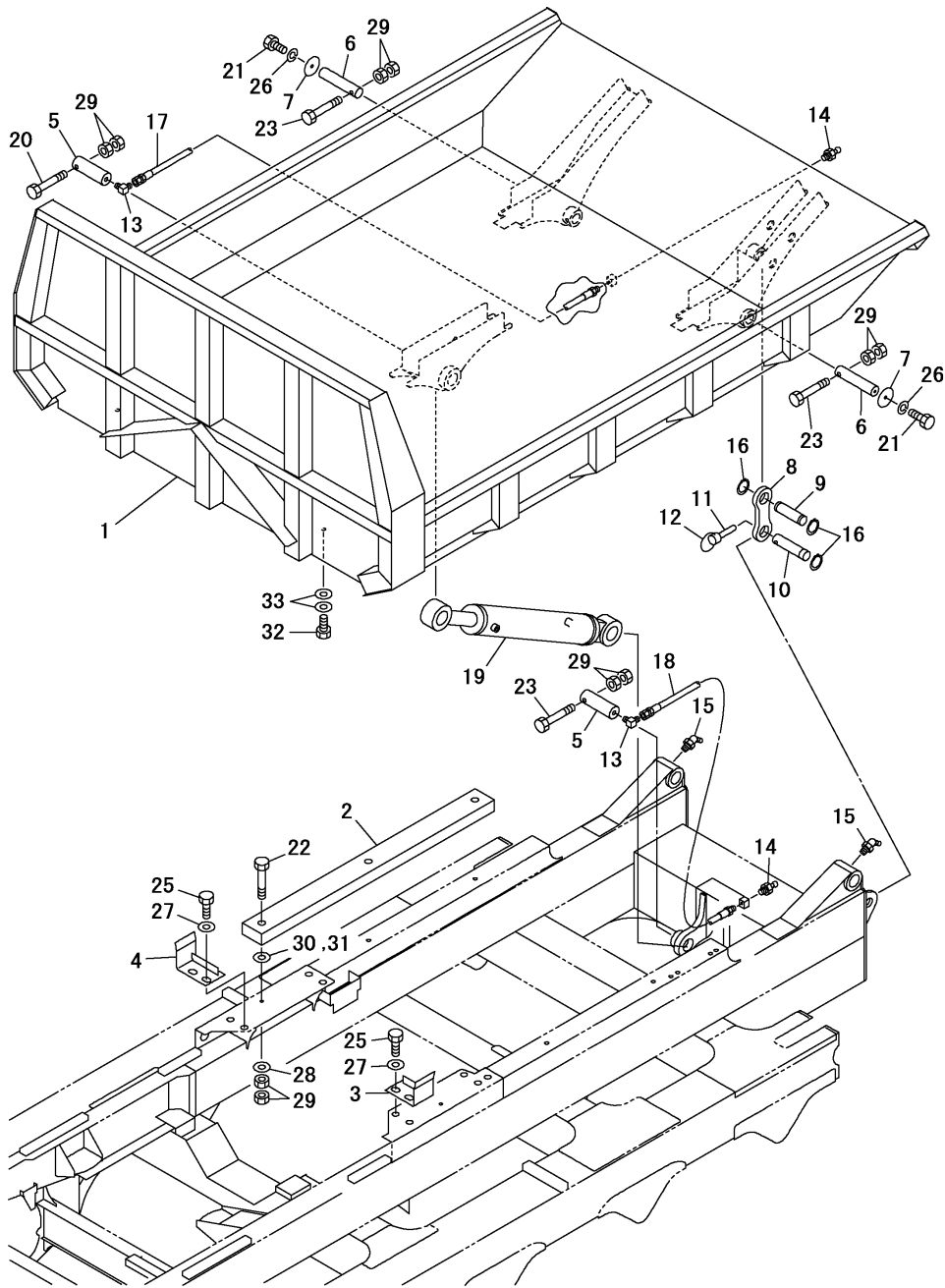
OCS10-G55100 Fig.66. VESSEL
