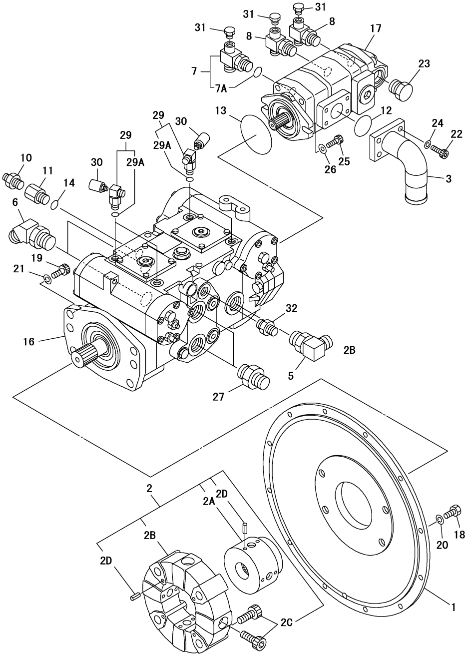
Fig.39. PUMP DRIVING
