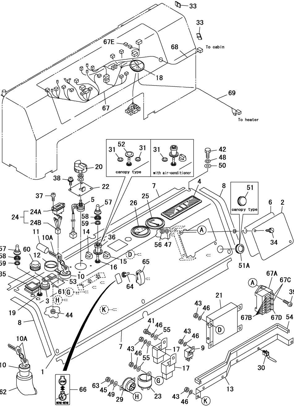
Fig.19. CONTROL BOX
