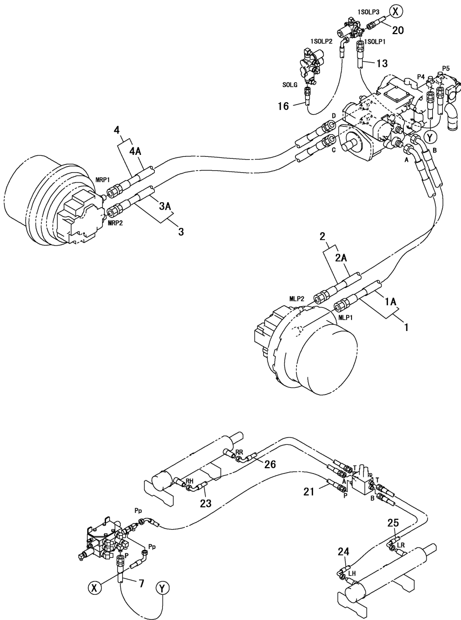
Fig.37. HYD.OIL PIPING(2/2)(TURNING)
