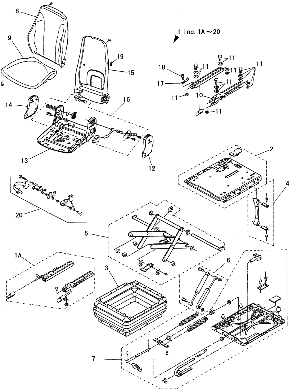
Fig.51. SEAT(2/2)
