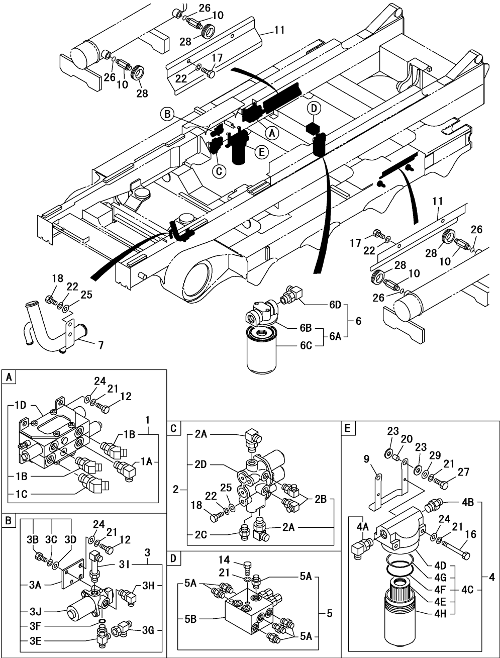
Fig.32. VALVE
