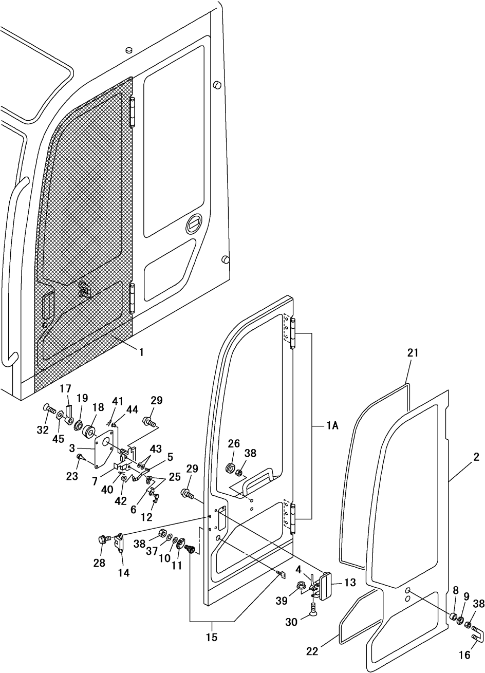
Fig.57. CABIN(6/6)(DOOR)
