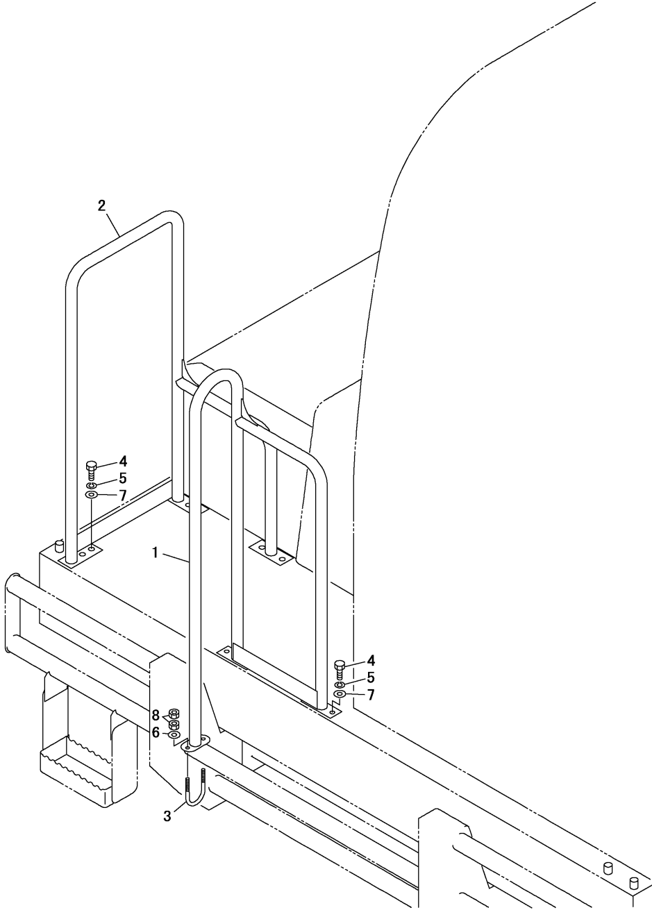
OCS10-G55100 Fig.47. BALUSTRADE
