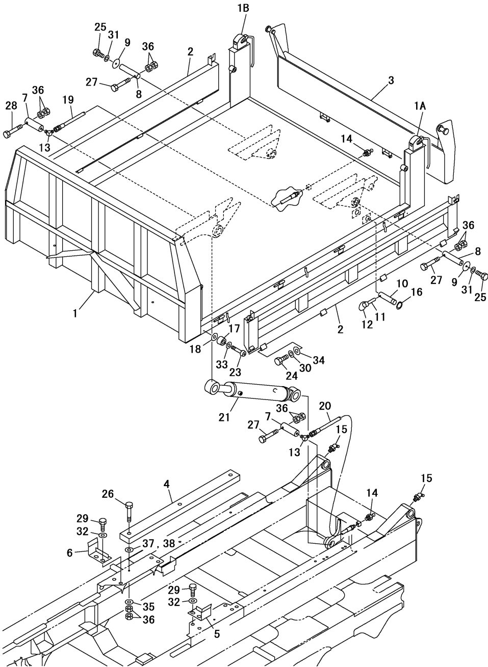
Fig.69. DUMP BODY
