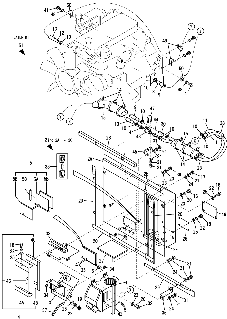
OCS10-G55100 Fig.59. HEATER
