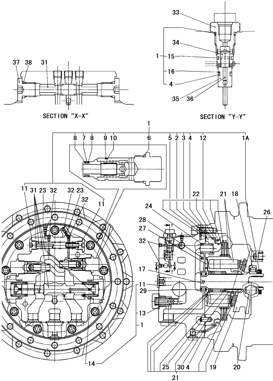
Fig.93. TRAVEL MOTOR(2/3)
