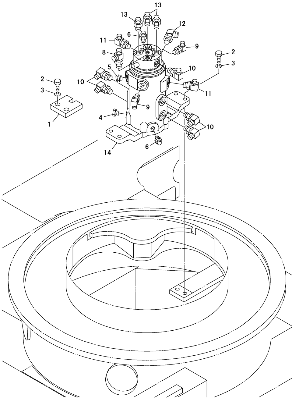
Fig.10. SWIVEL JOINT
