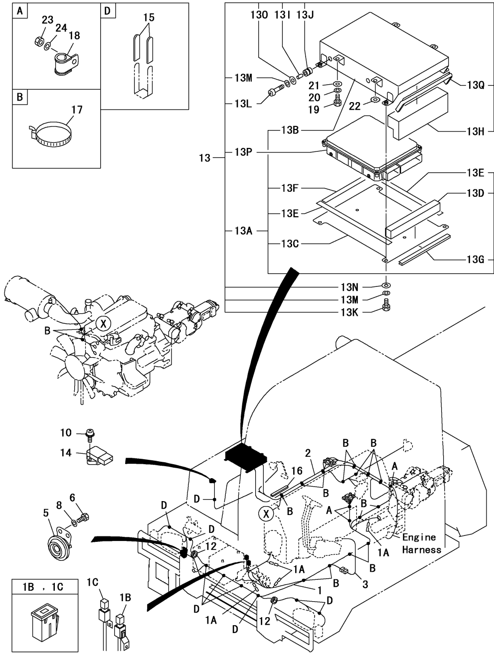
Fig.20. ELECTRIC PART
