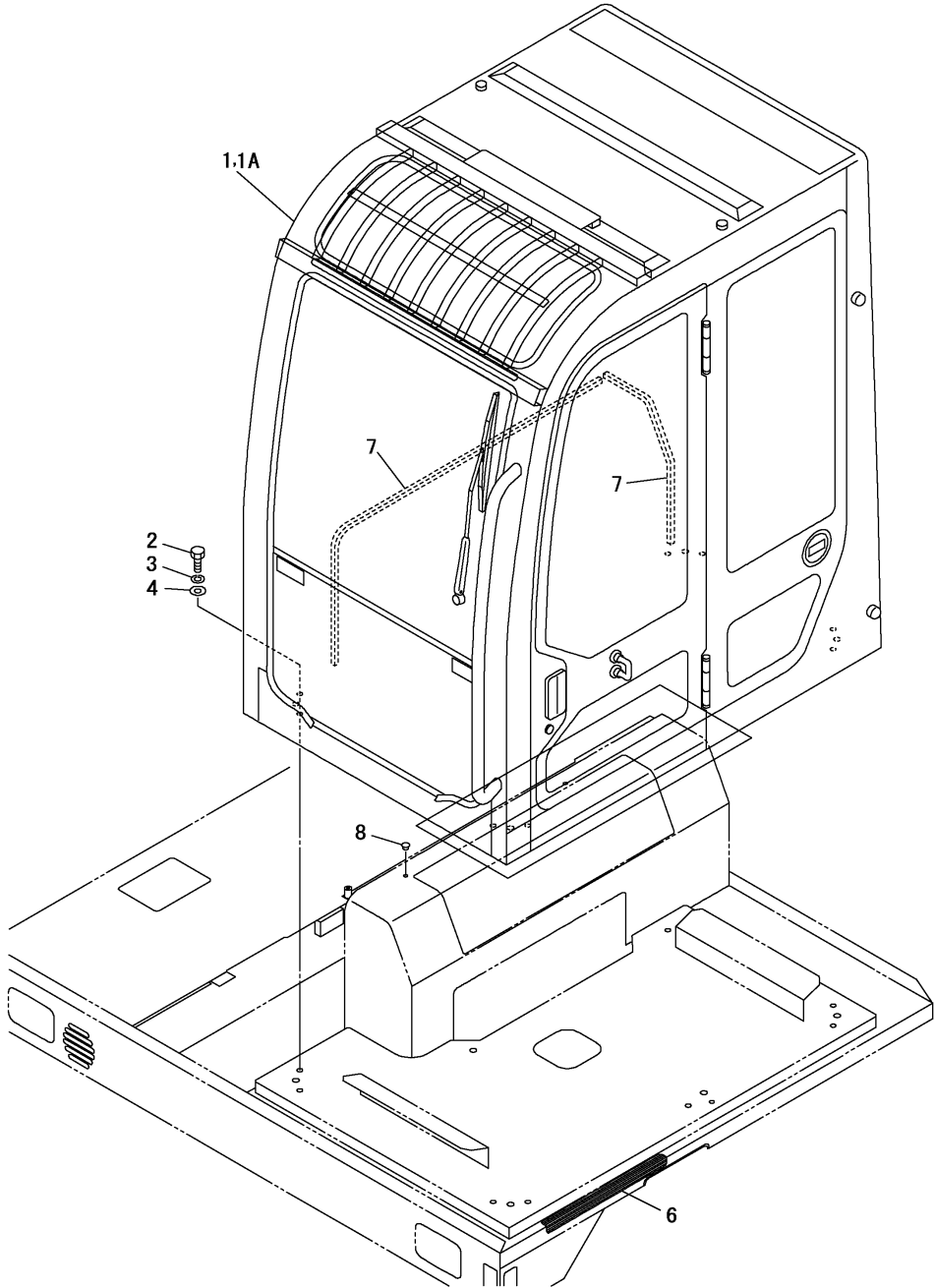
OCS10-G55100 Fig.52. CABIN(1/6)
