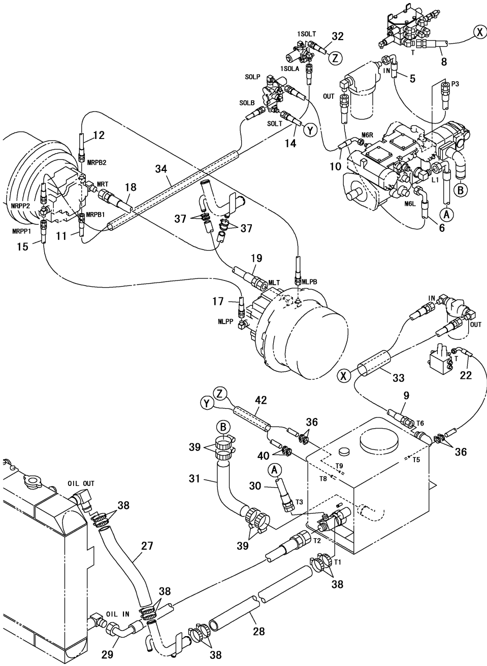
Fig.36. HYD.OIL PIPING(1/2)(TURNING)
