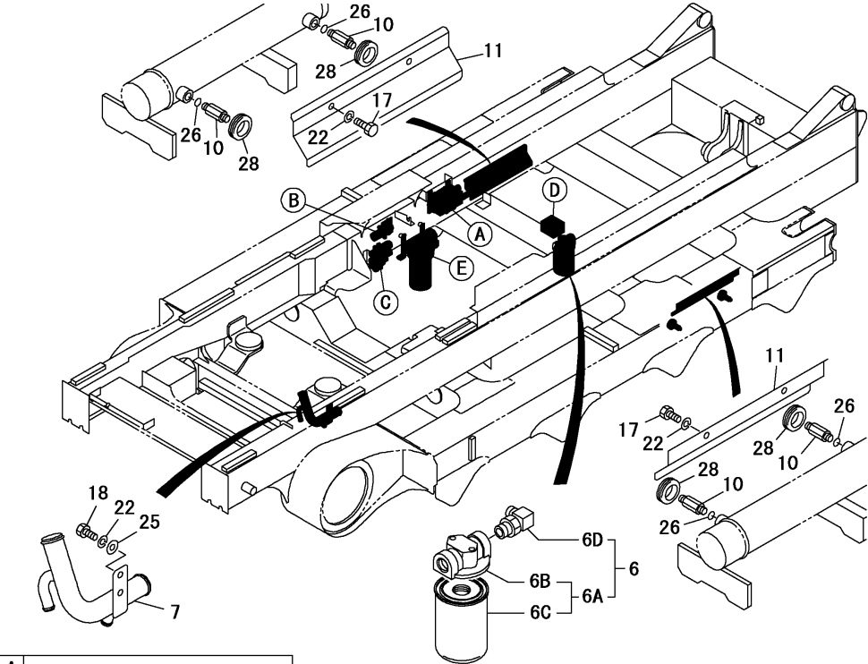
OCS10-G55100 Fig.32. VALVE
