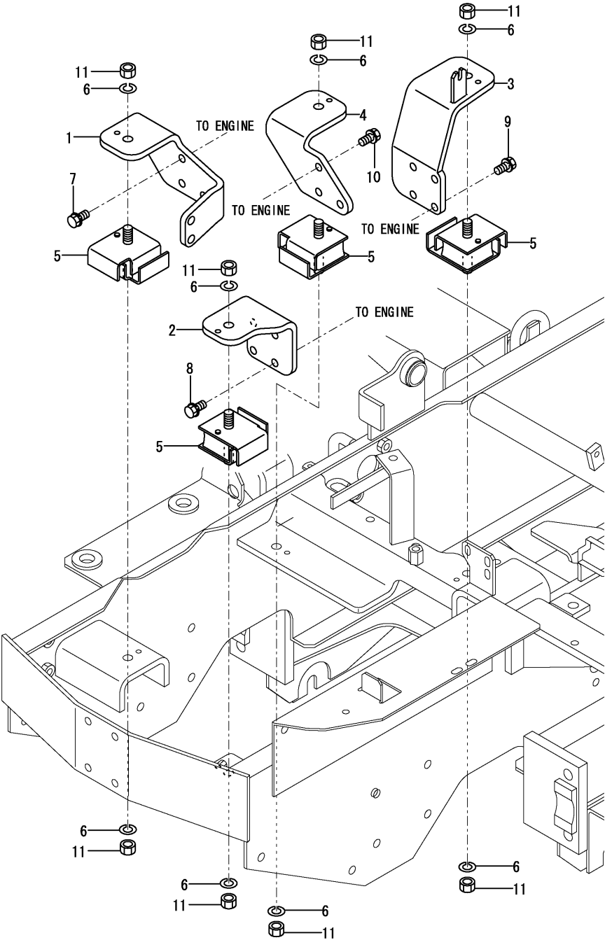
Fig.8. ENGINE MOUNT
