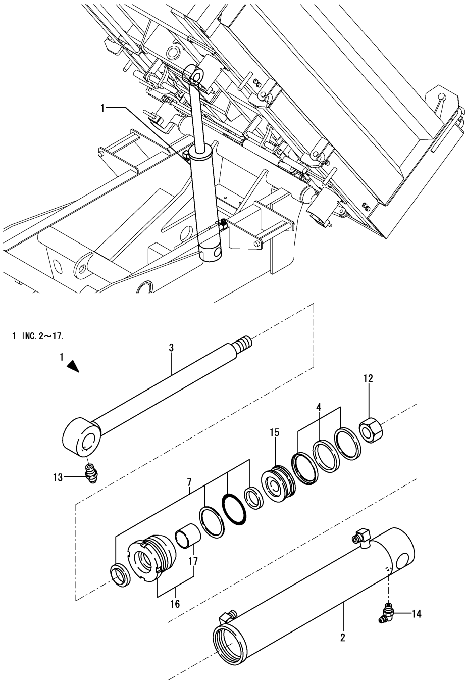
Fig.33. HYD.OIL CYLINDER
