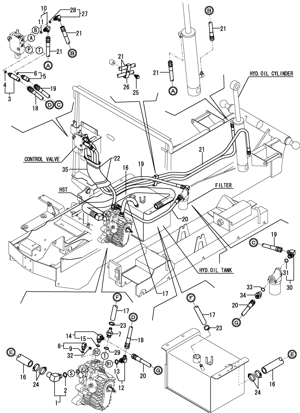
Fig.37. HYD.OIL PIPING
