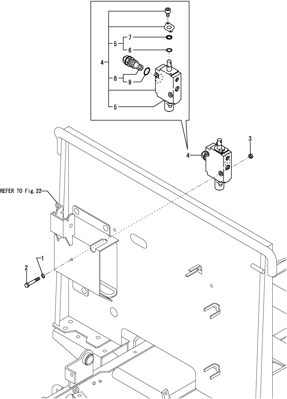
Fig.36. CONTROL VALVE
