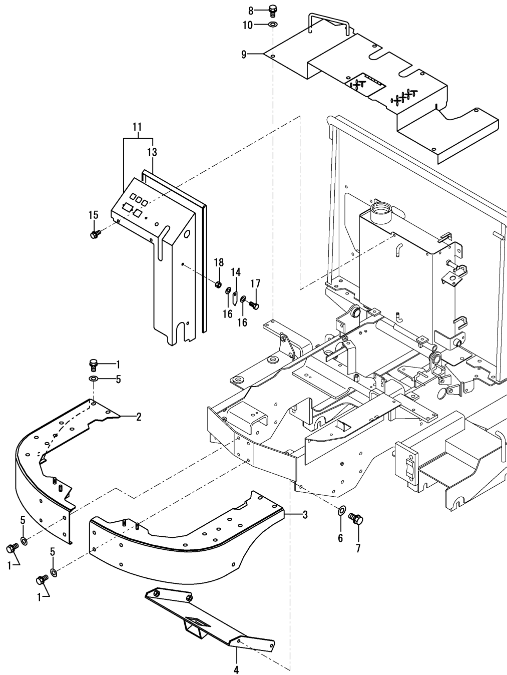
Fig.27. COVER, STEP & INSTRUMENT PANEL
