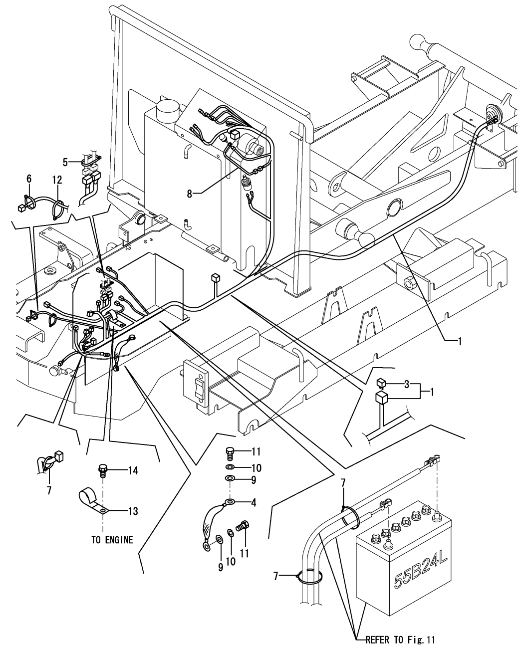
Fig.12. ELECTRIC PART(WIRING)
