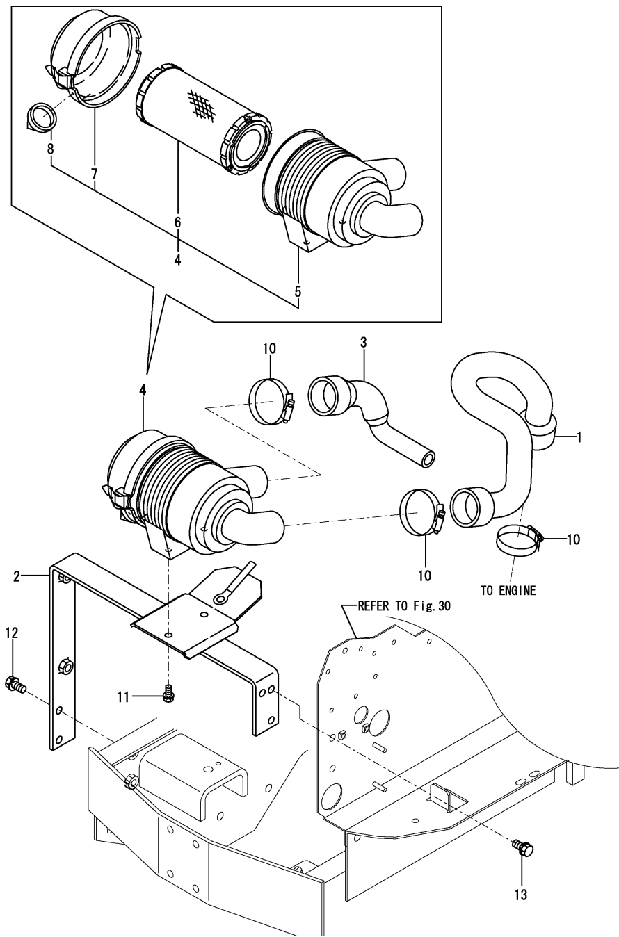
Fig.6. AIR CLEANER
