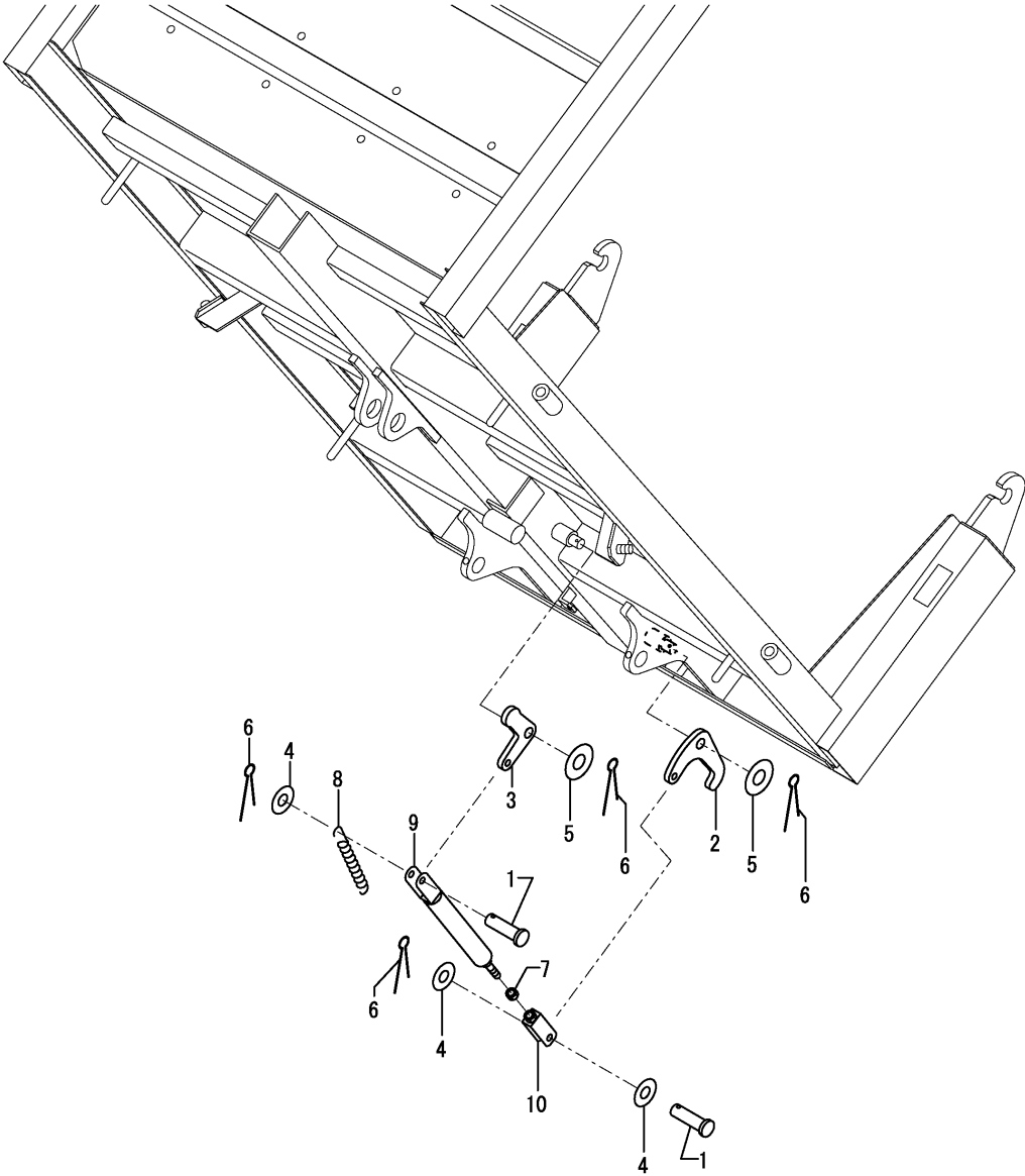
Fig.41. HOOK(STANDARD SPEC.)
