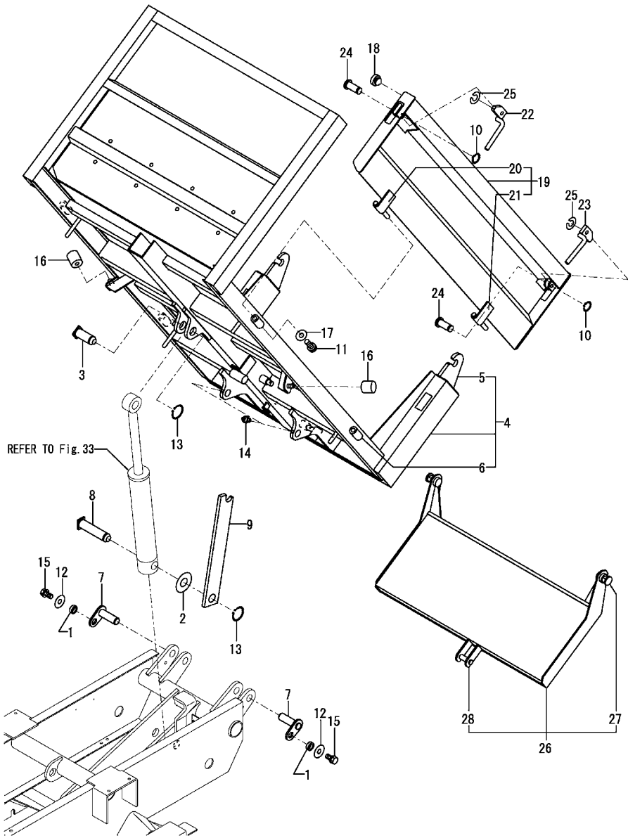
Fig.39. WAGON(STANDARD SPEC.)
