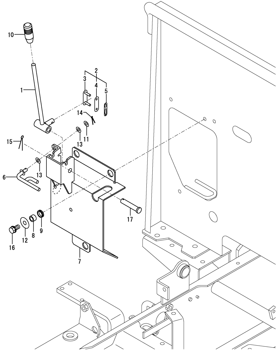
Fig.22. CONTROL EQUIPMENT(DUMP LEVER)
