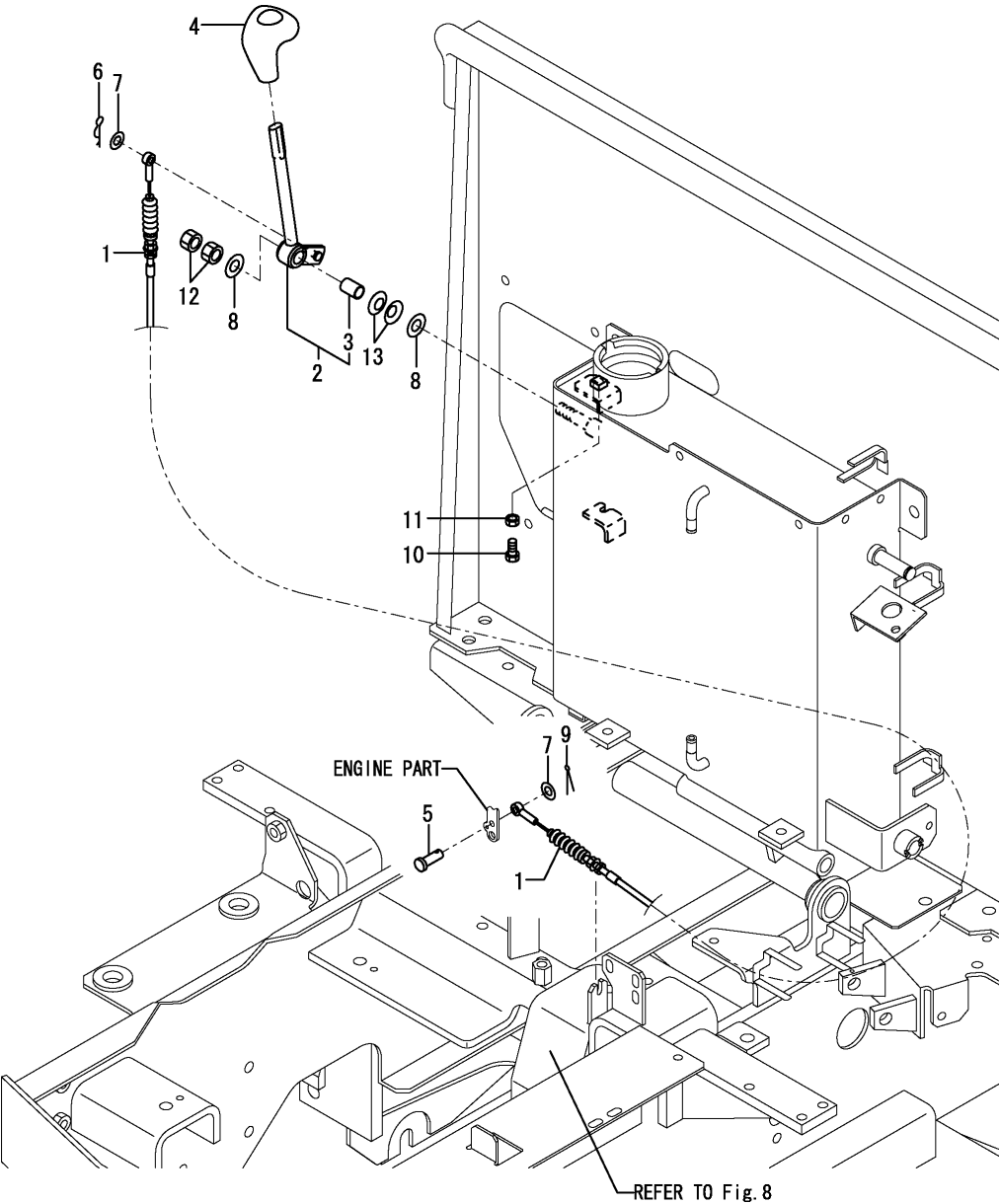
Fig.7. ACCELERATOR LEVER
