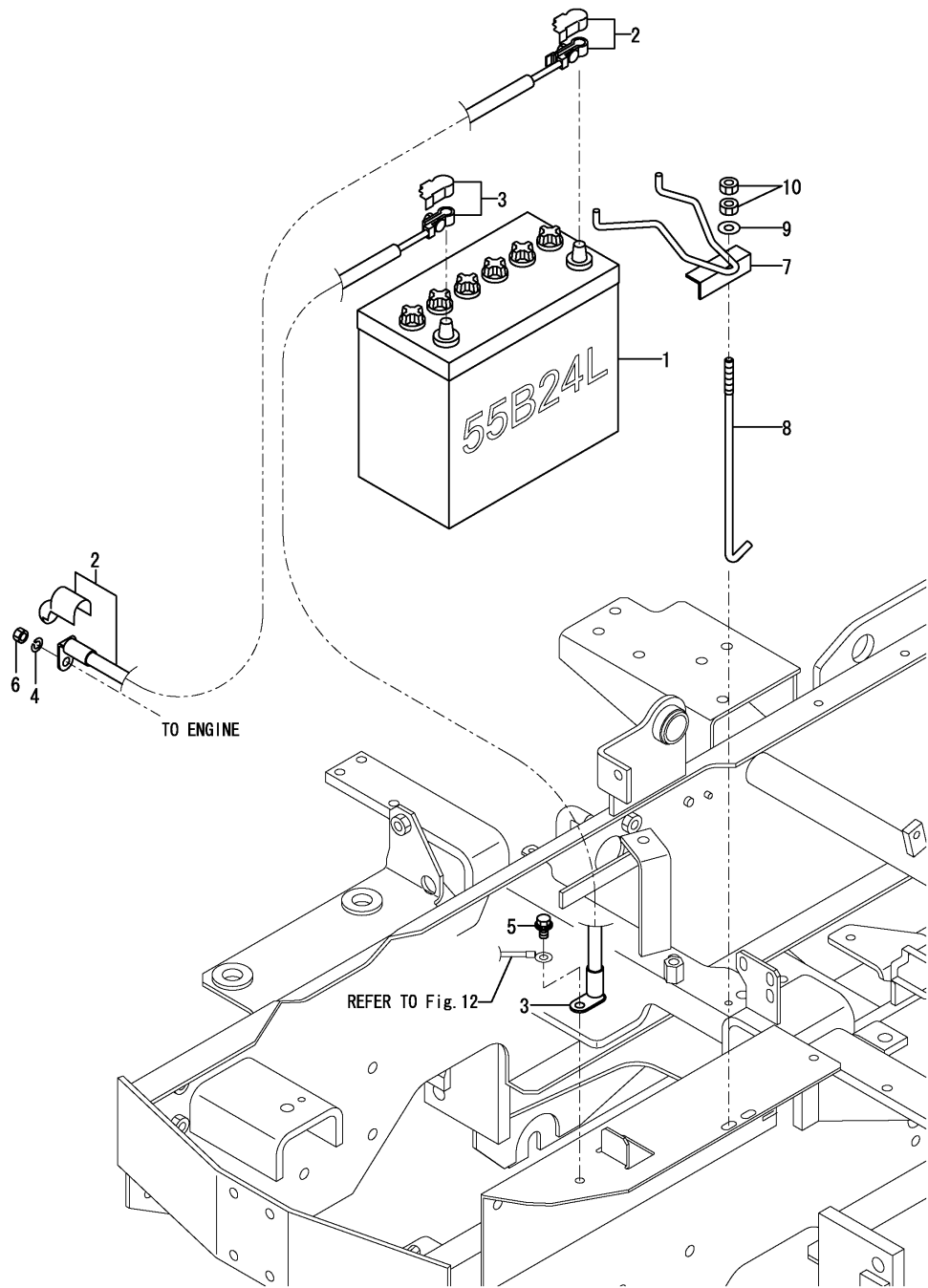
Fig.11. BATTERY & CABEL
