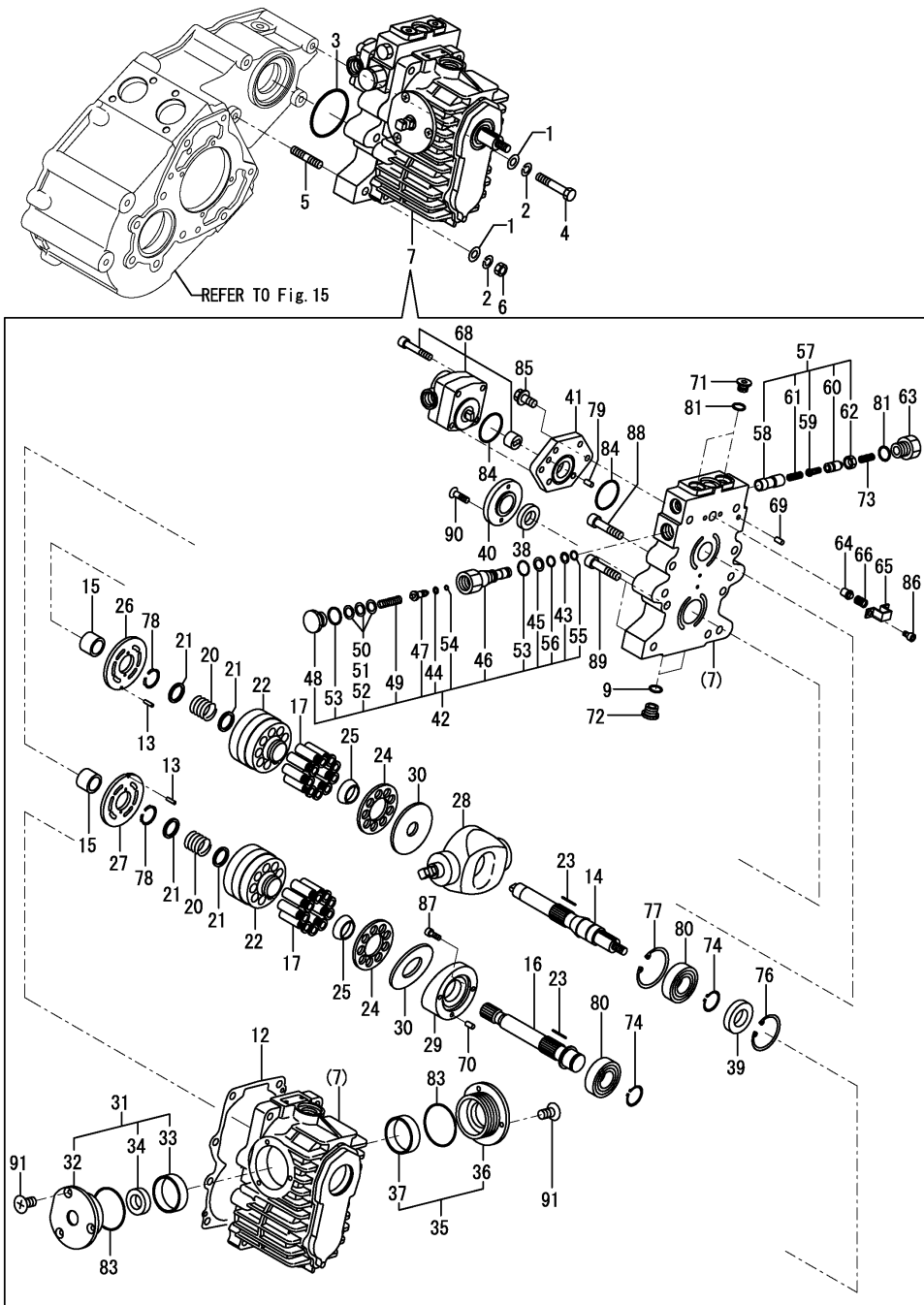
Fig.34. HST
