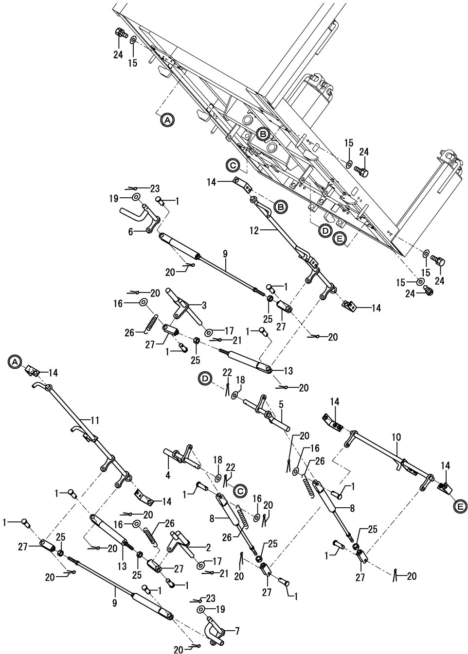
Fig.40. HOOK(3WD SPEC.)
