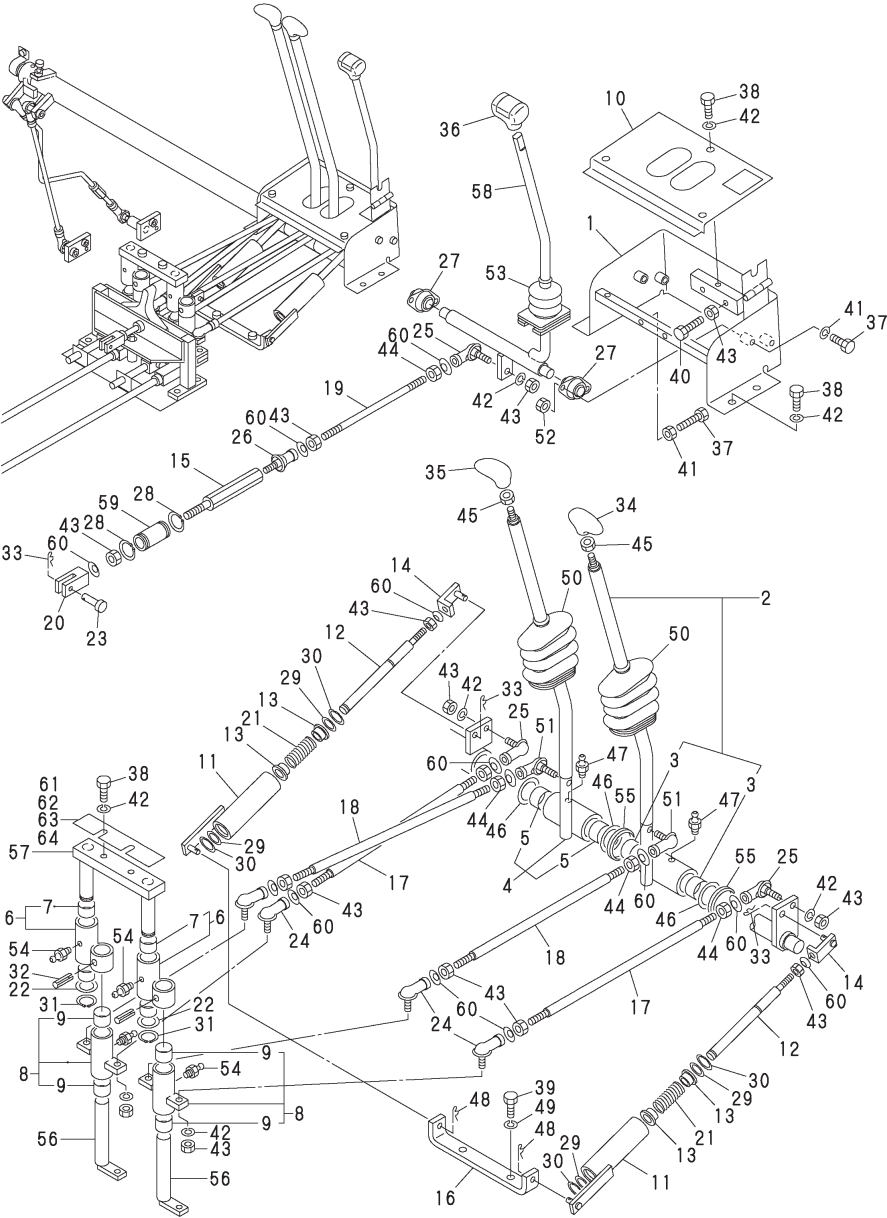
Fig.6. CONTROL LEVER(2)
