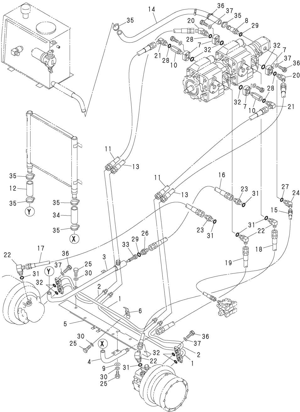
Fig.15. HYD. OIL PIPING(1)
