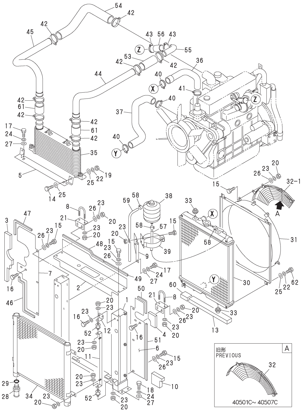
Fig.9. ENGINE&RELATED DEVICE(2)
