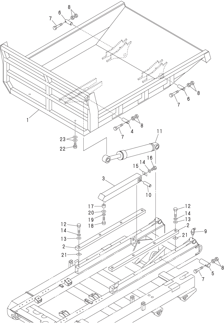
Fig.21. VESSELL
