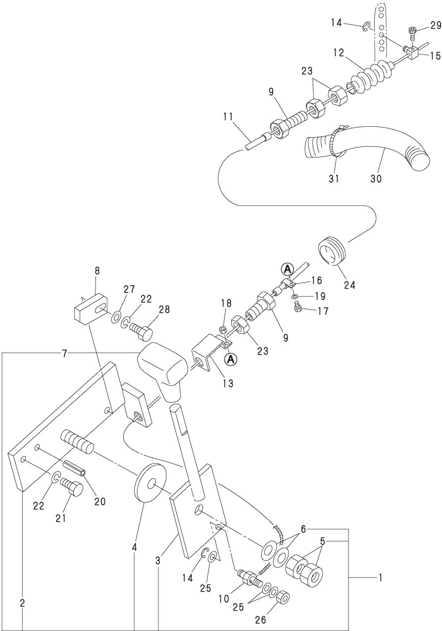
Fig.11. ENGINE CONTROL
