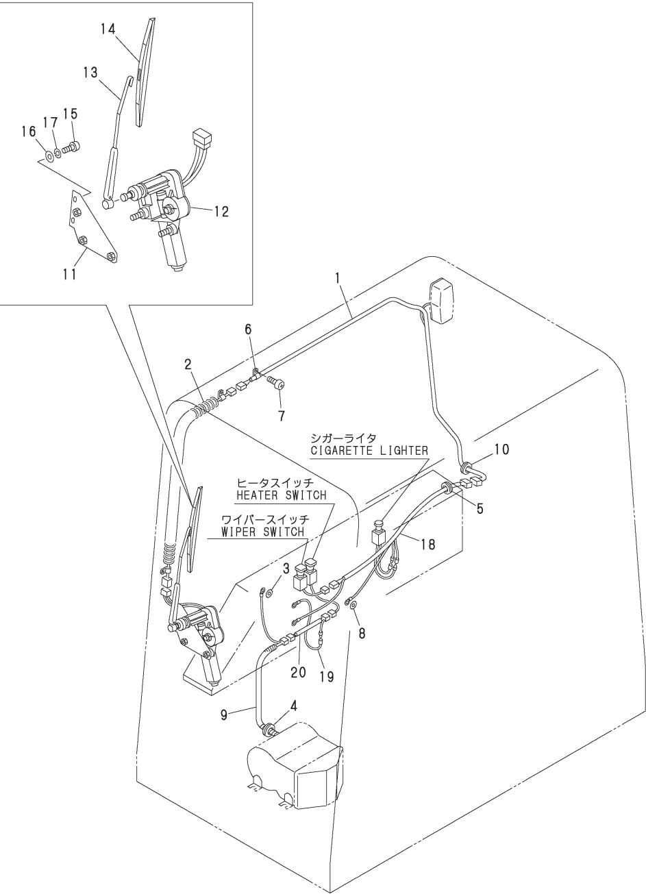
Fig.14. CABIN WIRING
