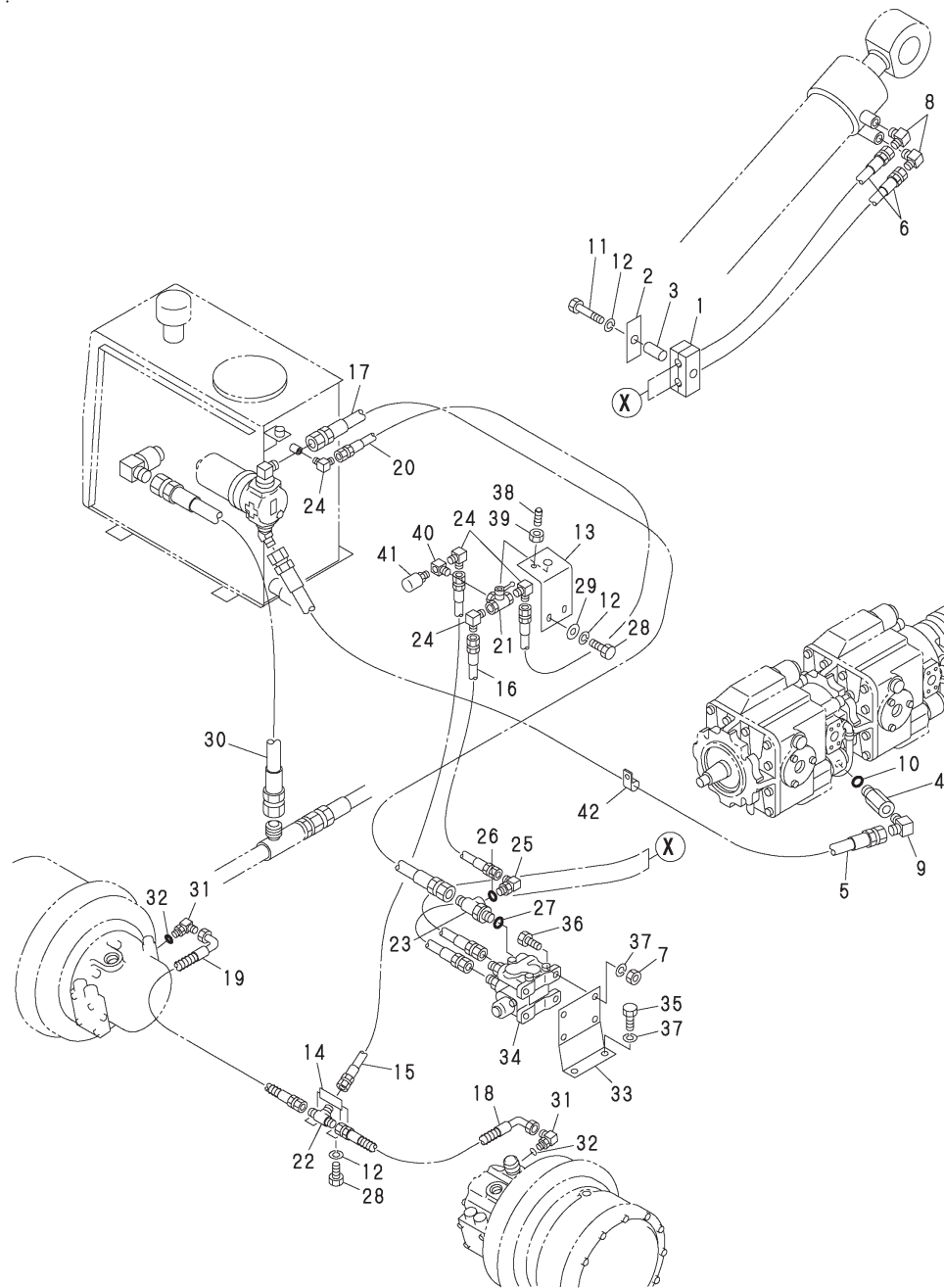
Fig.16. HYD. OIL PIPING(2)
