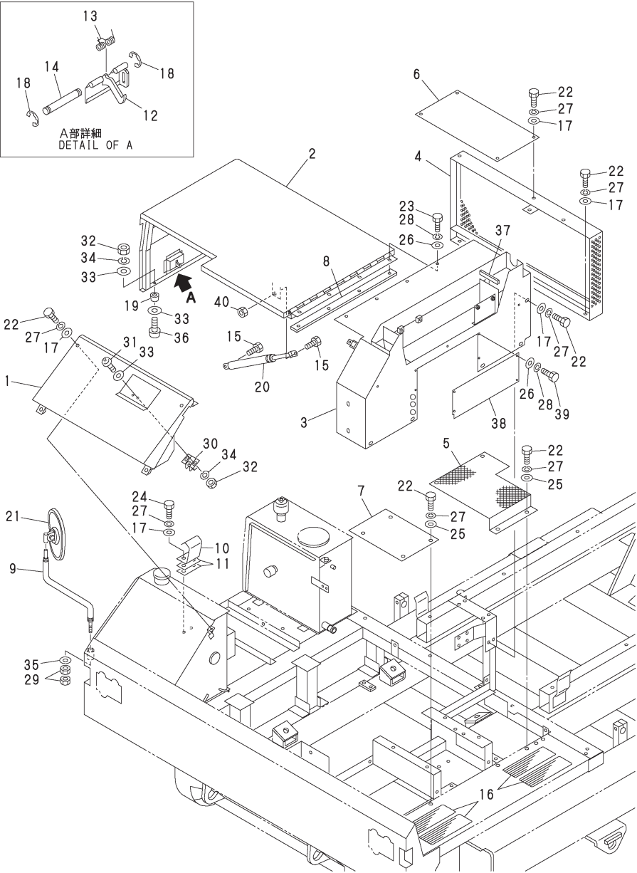
Fig.20. COVER
