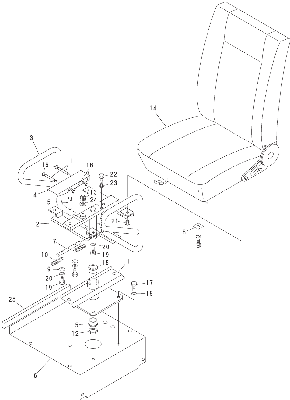
Fig.22. SEAT
