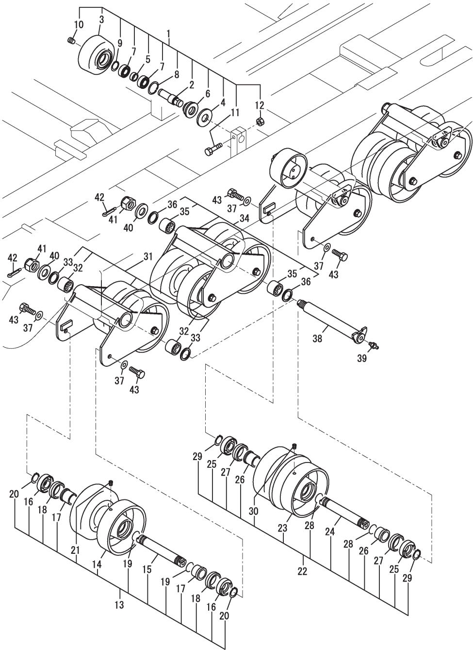
Fig.2. CARRIER ROLLER,TRUCK ROLLER
