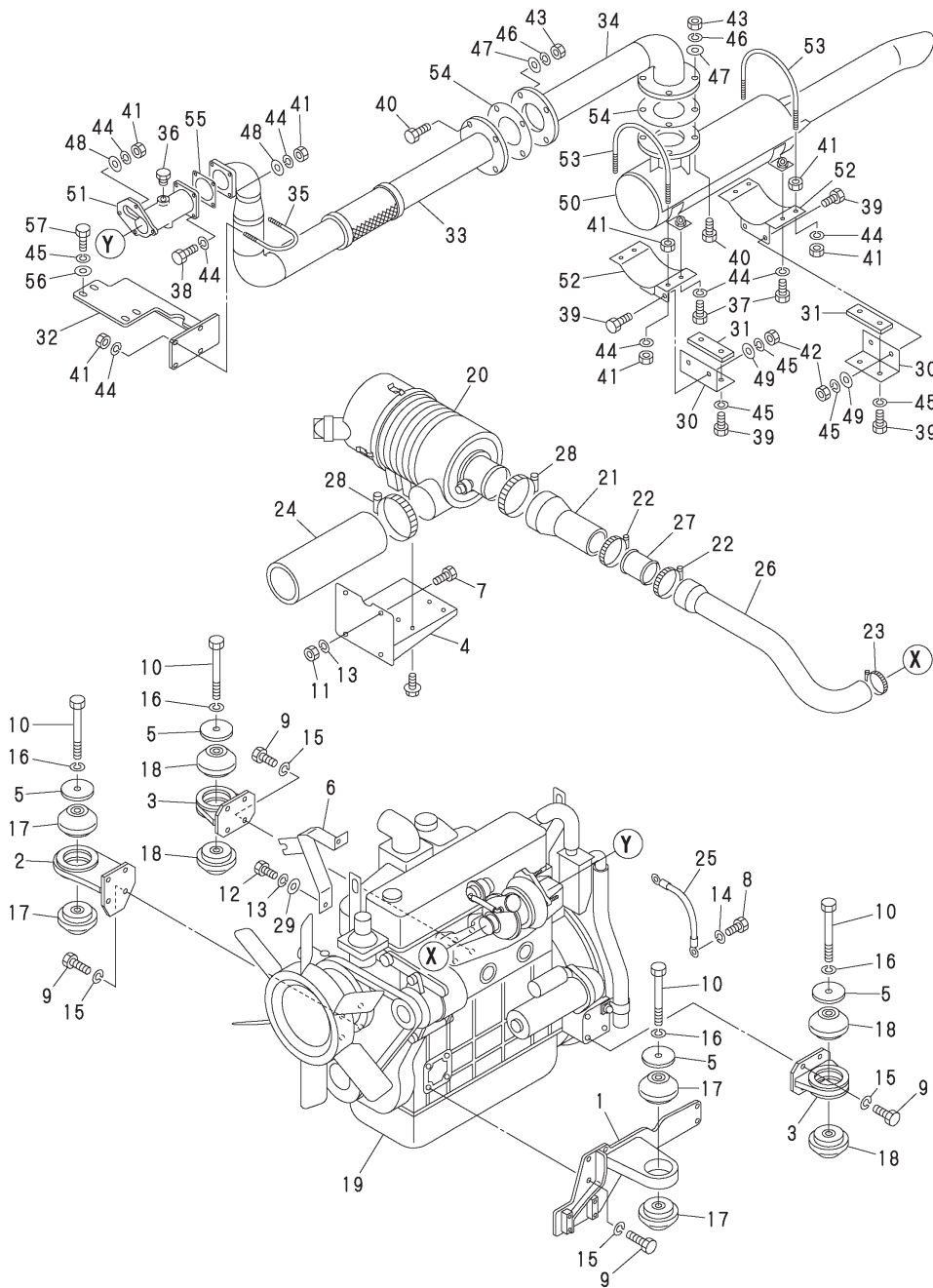
Fig.8. ENGINE&RELATED DEVICE(1)
