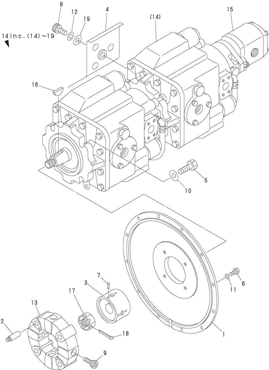
Fig.17. PUMP DRIVING
