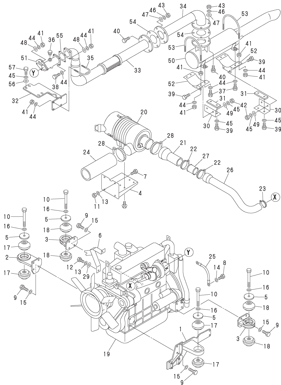
Fig.8. ENGINE&RELATED DEVICE(1)
