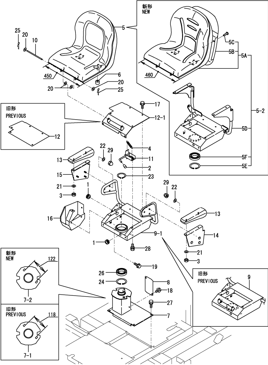
Fig.38. SEAT & MOUNT
