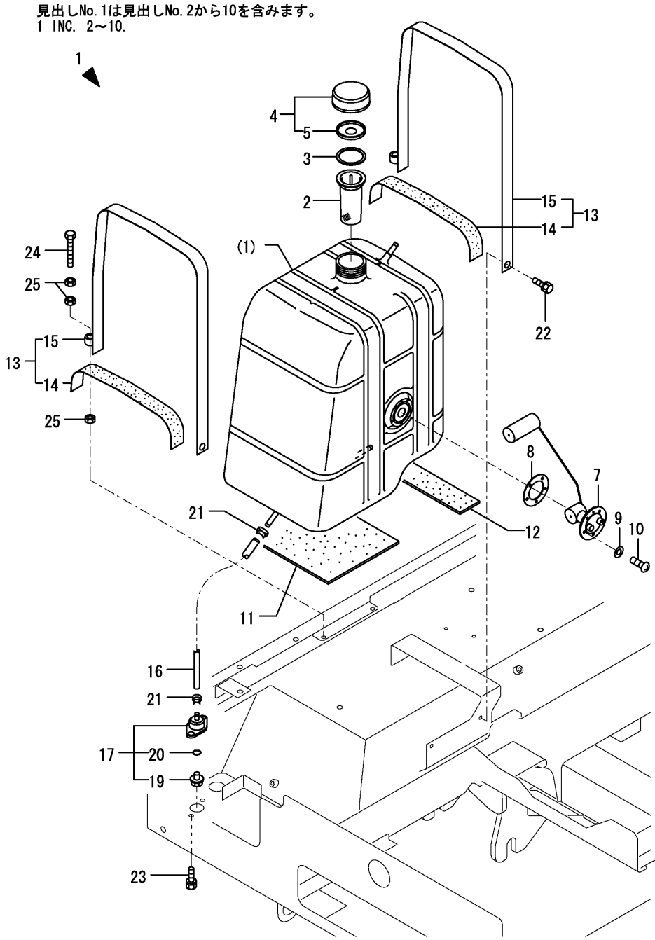
Fig.13. FUEL TANK
