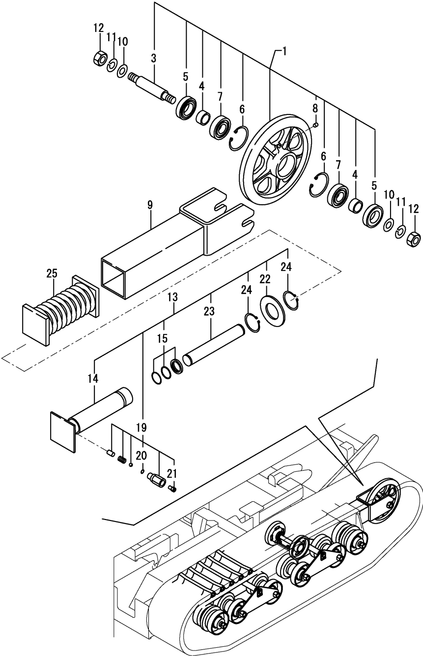
Fig.23. IDLER & CRAWLER ADJUST
