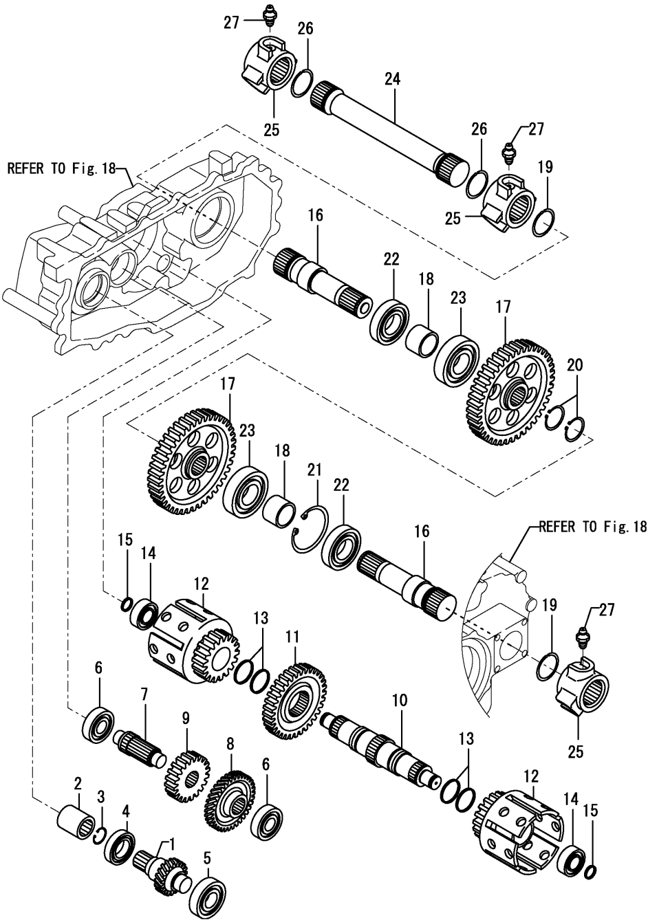
Fig.19. TRANSMISSION GEAR
