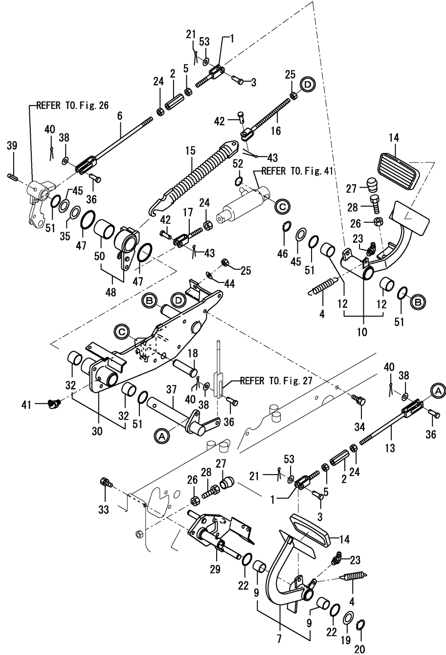
Fig.28. BRAKE(PEDAL & ROD)
