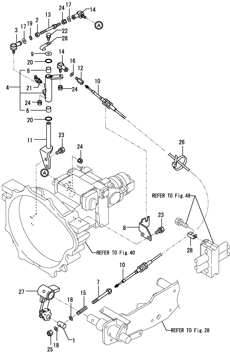
Fig.26. INCHING LINK
