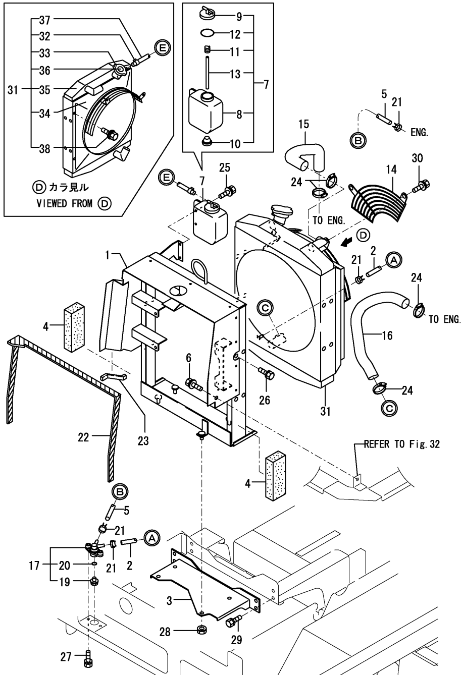
Fig.12. RADIATOR & MOUNT
