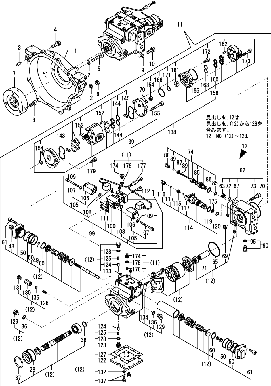
Fig.40. HYD.OIL PUMP & JOINT
