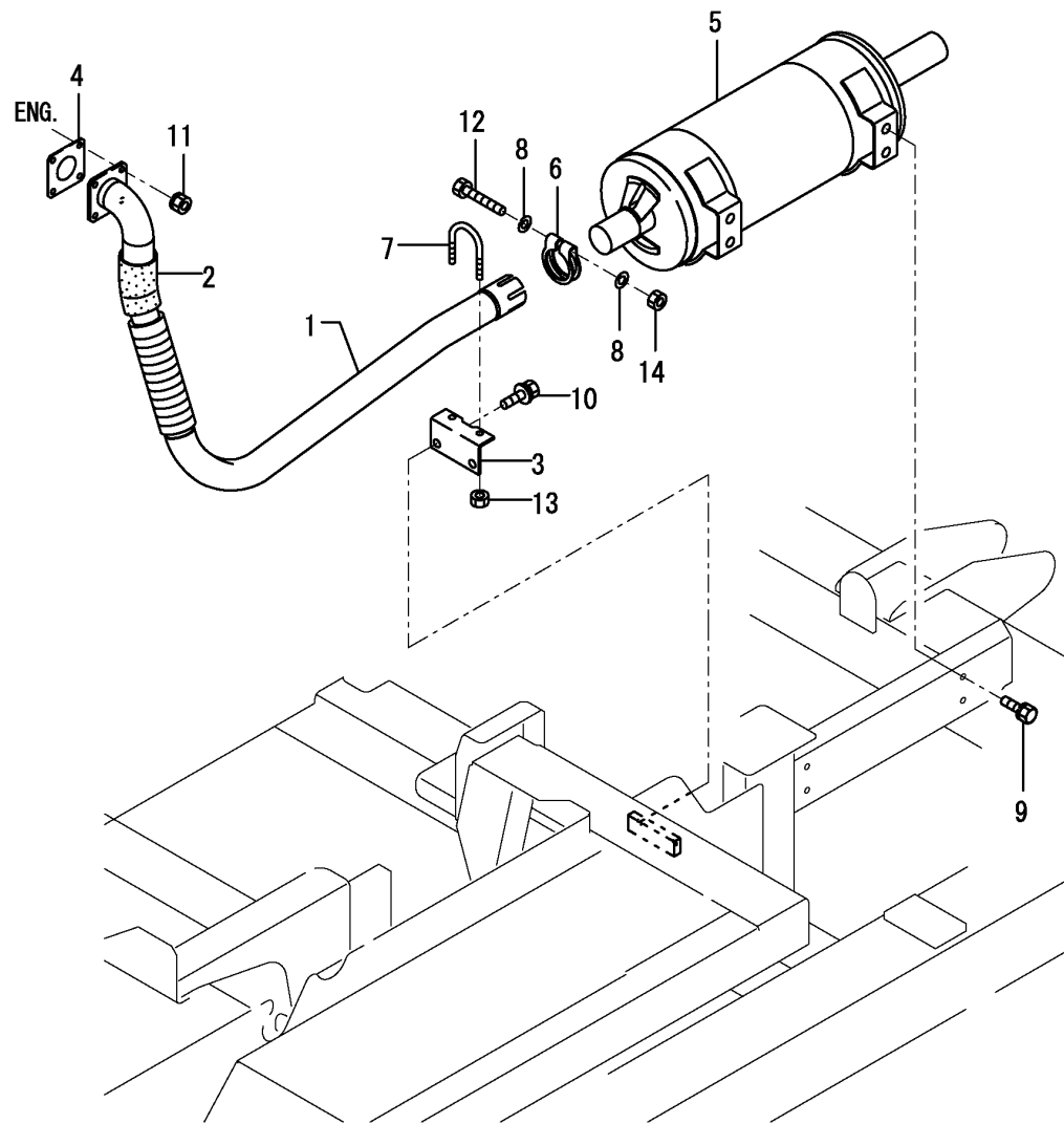
Fig.8. EXHAUST PIPE
