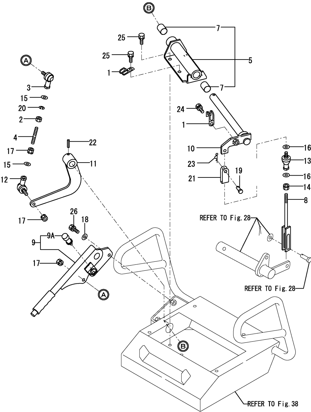
Fig.27. BRAKE(PARKING)
