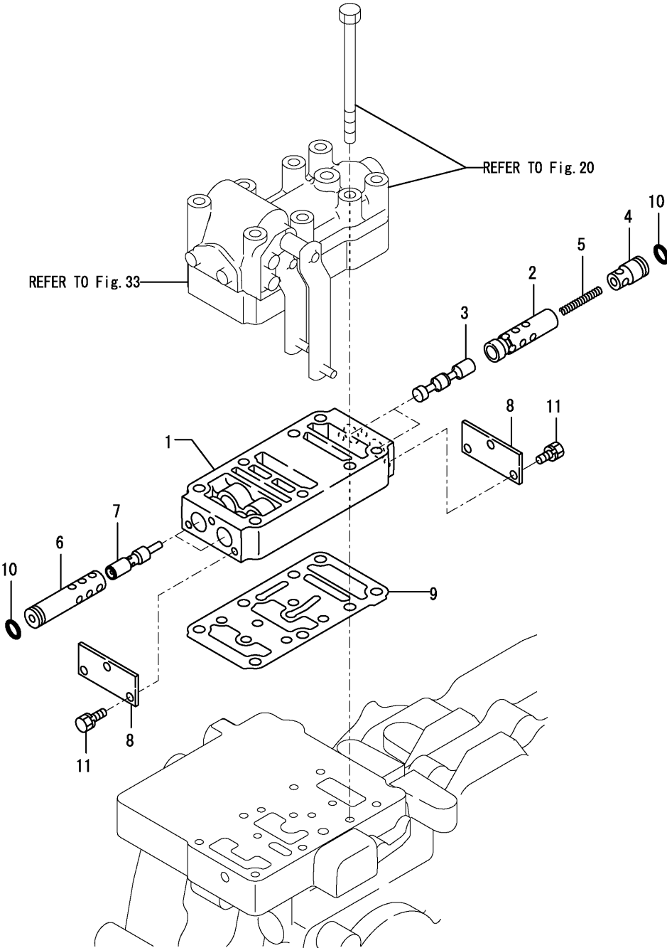
Fig.34. CLUTCH VALVE
