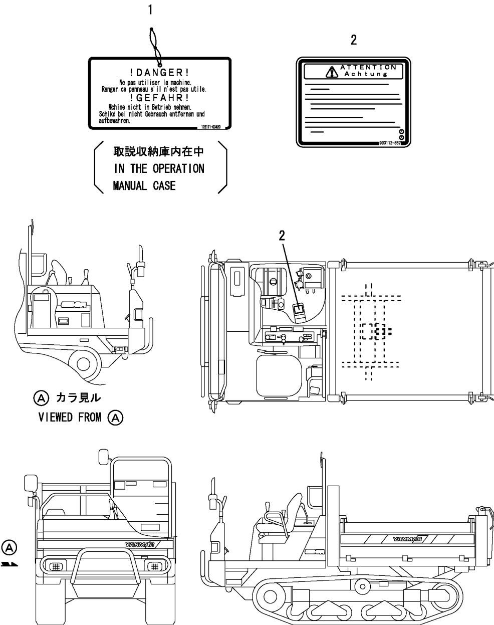
Fig.5. SAFETY LABEL(EP)
