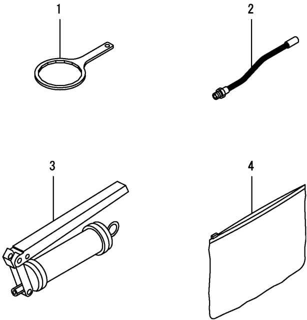
Fig.6. TOOL & ATTACHED
