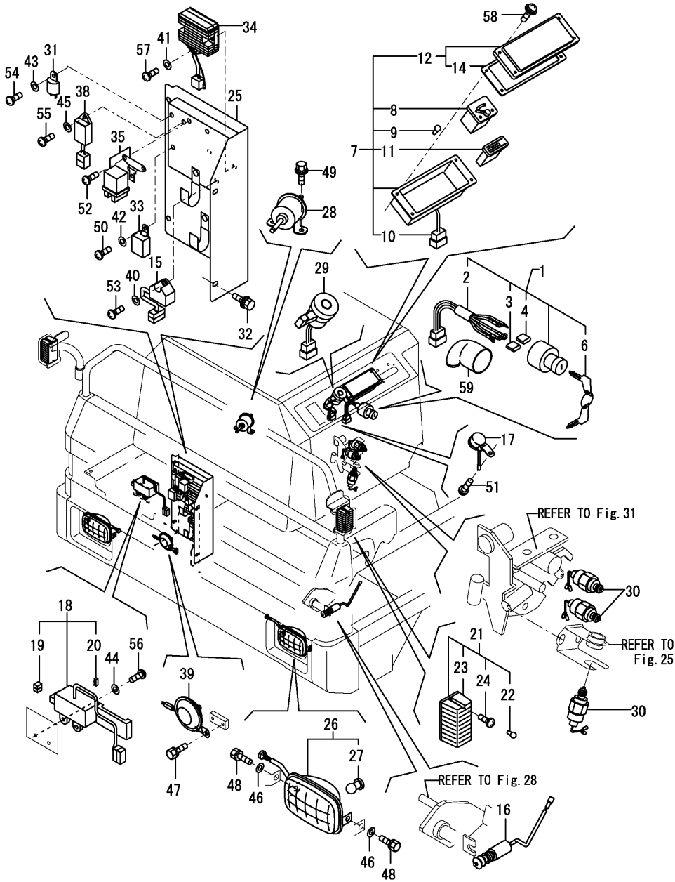
Fig.17. ELECTRIC PART(EQUIPMENT)
