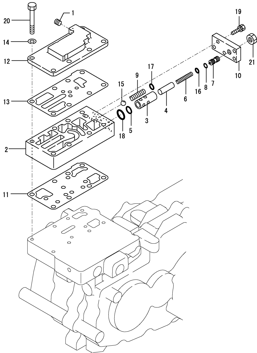
Fig.35. RELIVE VALVE
