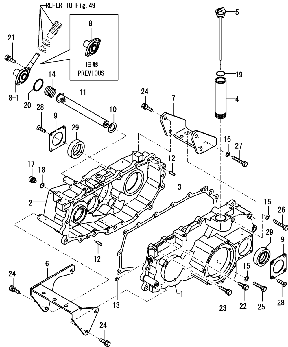
Fig.18. TRANSMISSION CASE
