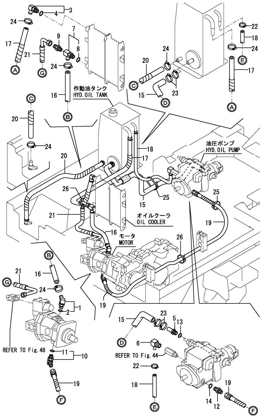
Fig.45. HYD.OIL PIPING(TANK - PUMP)
