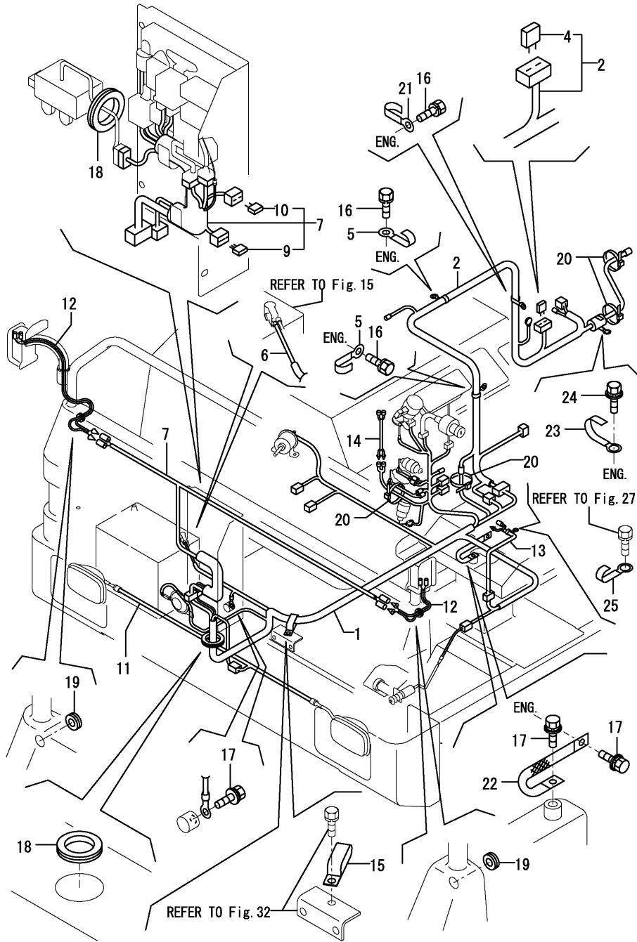
Fig.16. ELECTRIC PART(WIRING)
