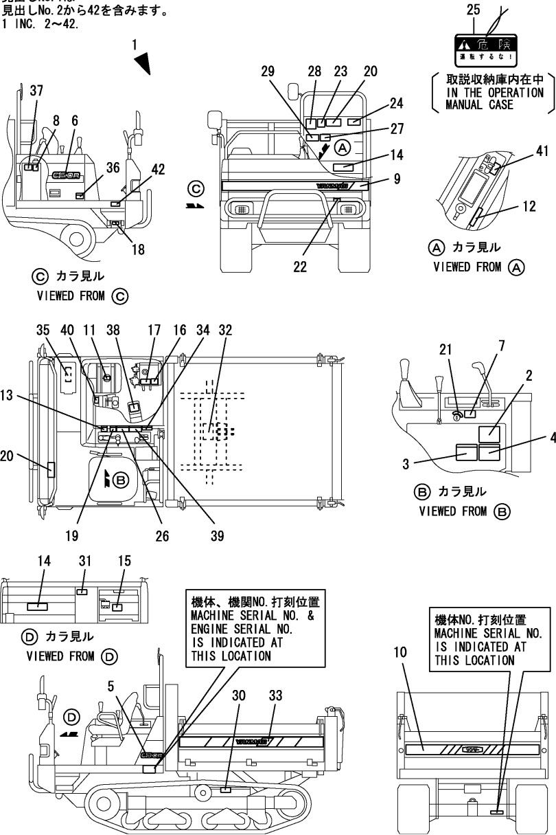
Fig.1. LABEL(JP)
