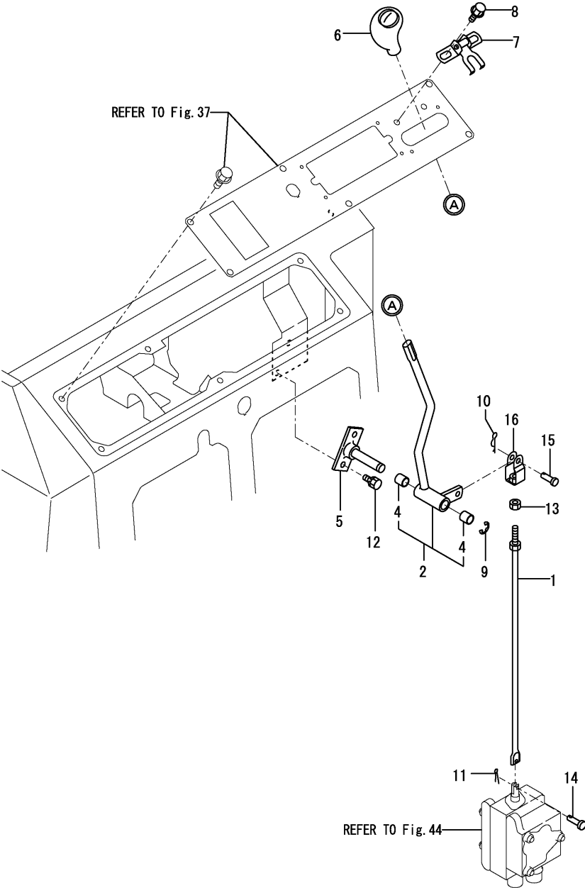
Fig.30. HYD.OIL LEVER
