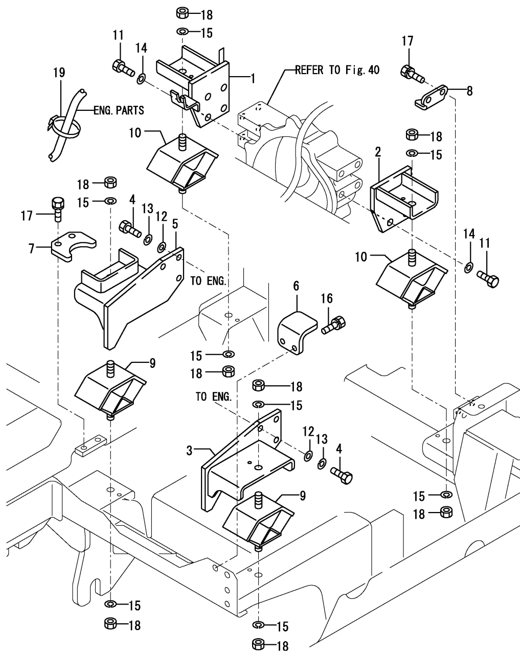
Fig.11. ENGINE MOUNT
