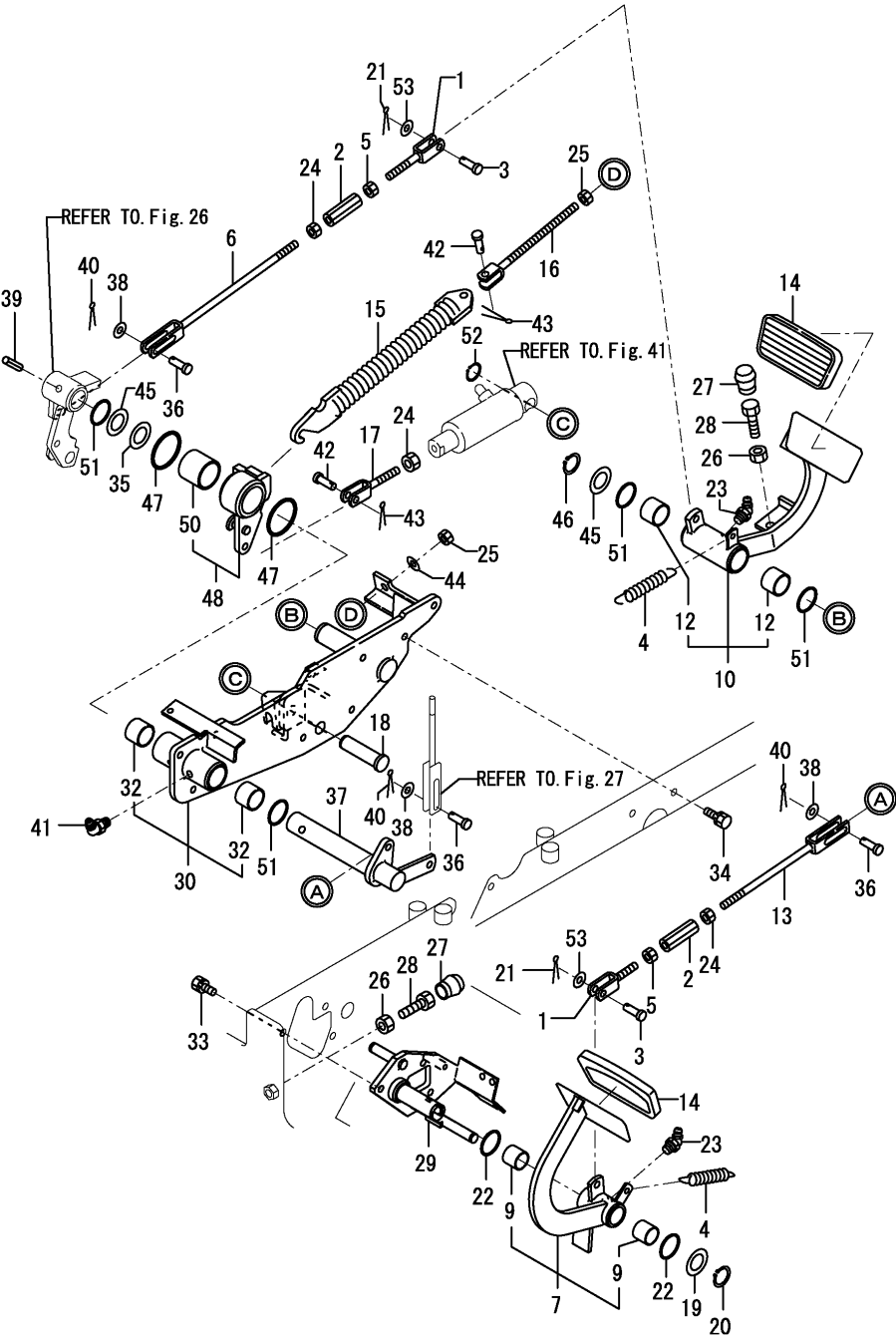
Fig.28. BRAKE(PEDAL & ROD)
