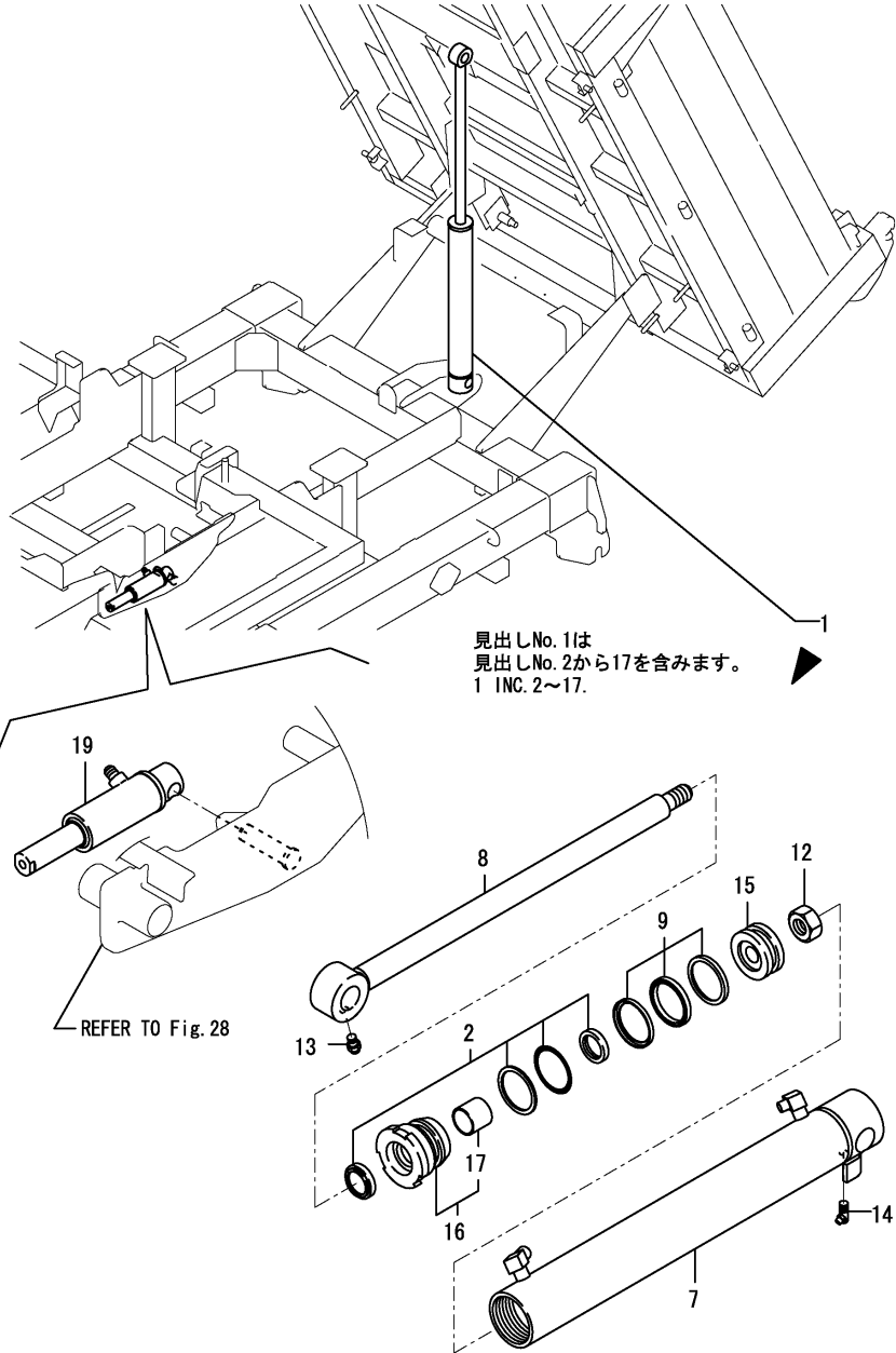
Fig.41. HYD.OIL CYLINDER
