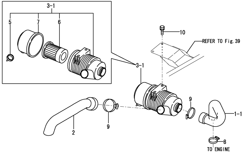
Fig.9. SUCTION PIPE
