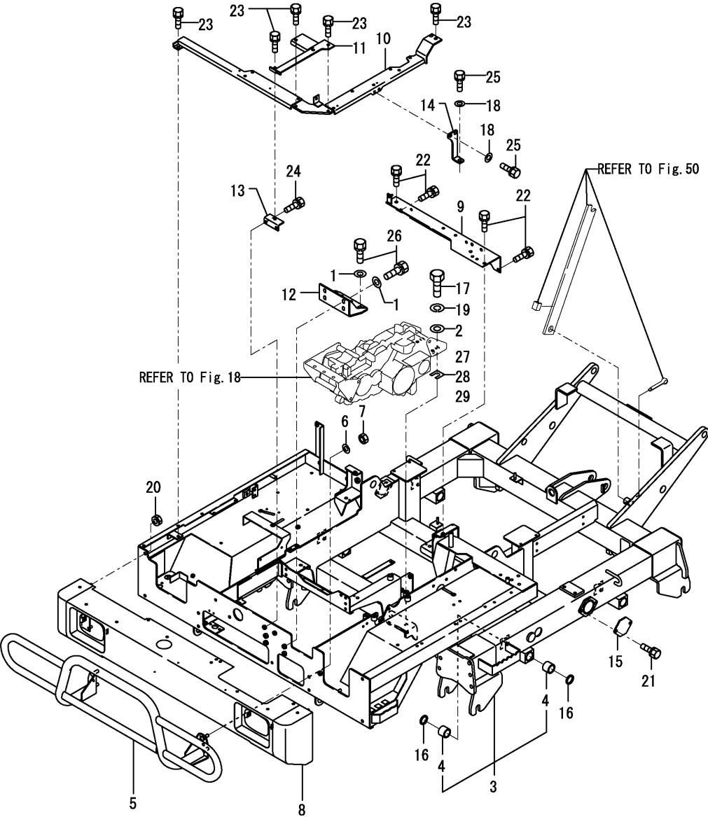
Fig.32. FRAME & BUMPER
