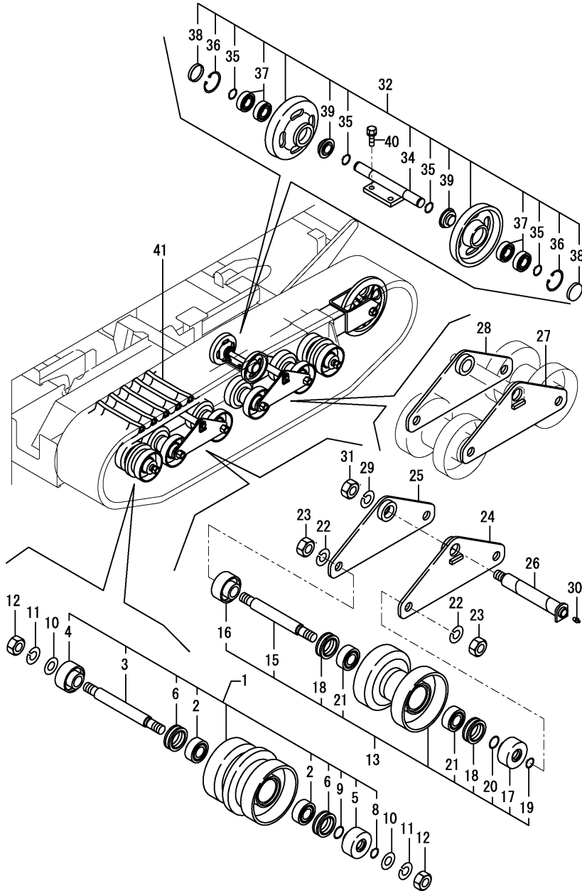
Fig.24. ROLLER & CRAWLER
