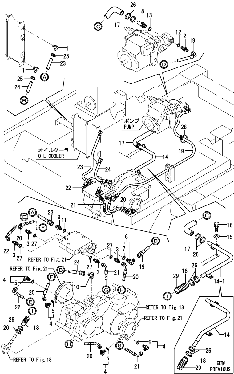
Fig.49. HYD.OIL PIPING(REDUCTION)
