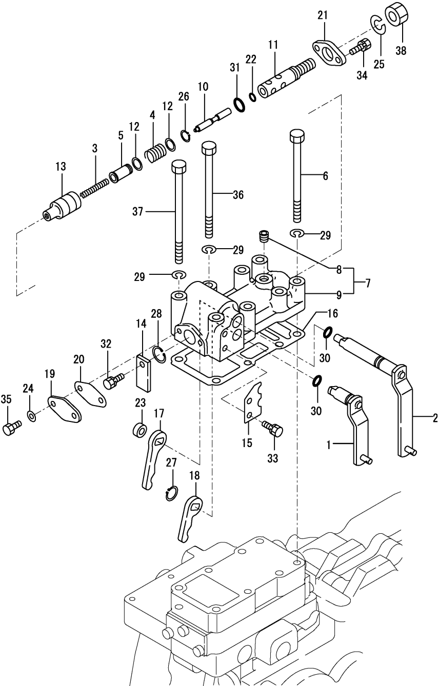
Fig.20. HYD.OIL CONTROL
