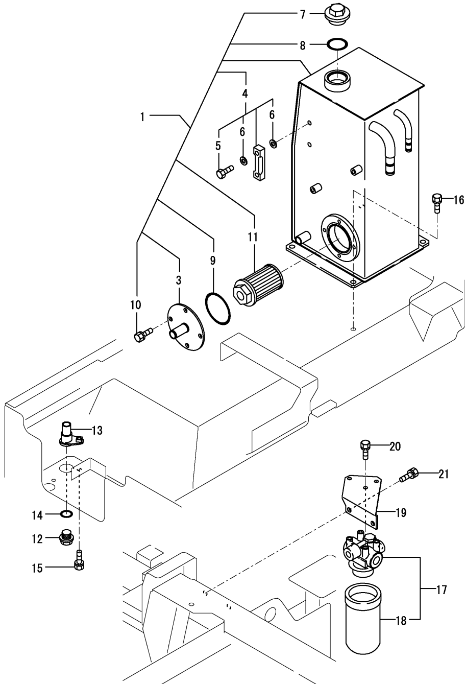
Fig.43. HYD.OIL TANK & FILTER
