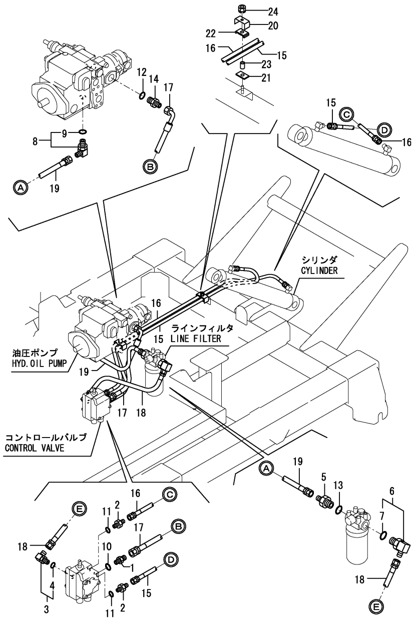
Fig.46. HYD.OIL PIPING(PUMP - CONTROL VALVE - CYLINDER)
