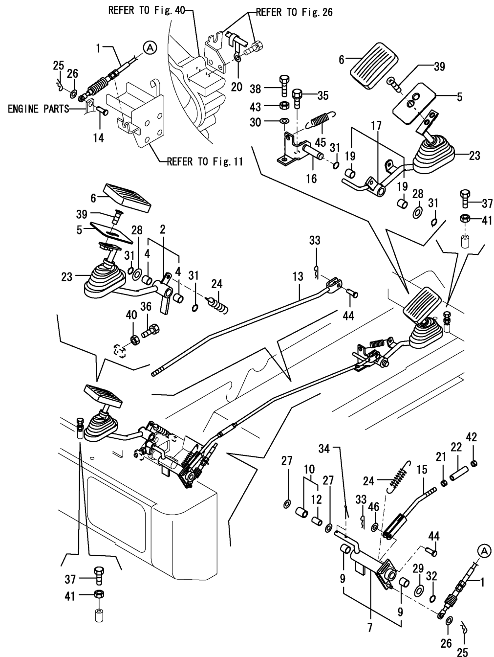
Fig.10. FOOT ACCELERATOR
