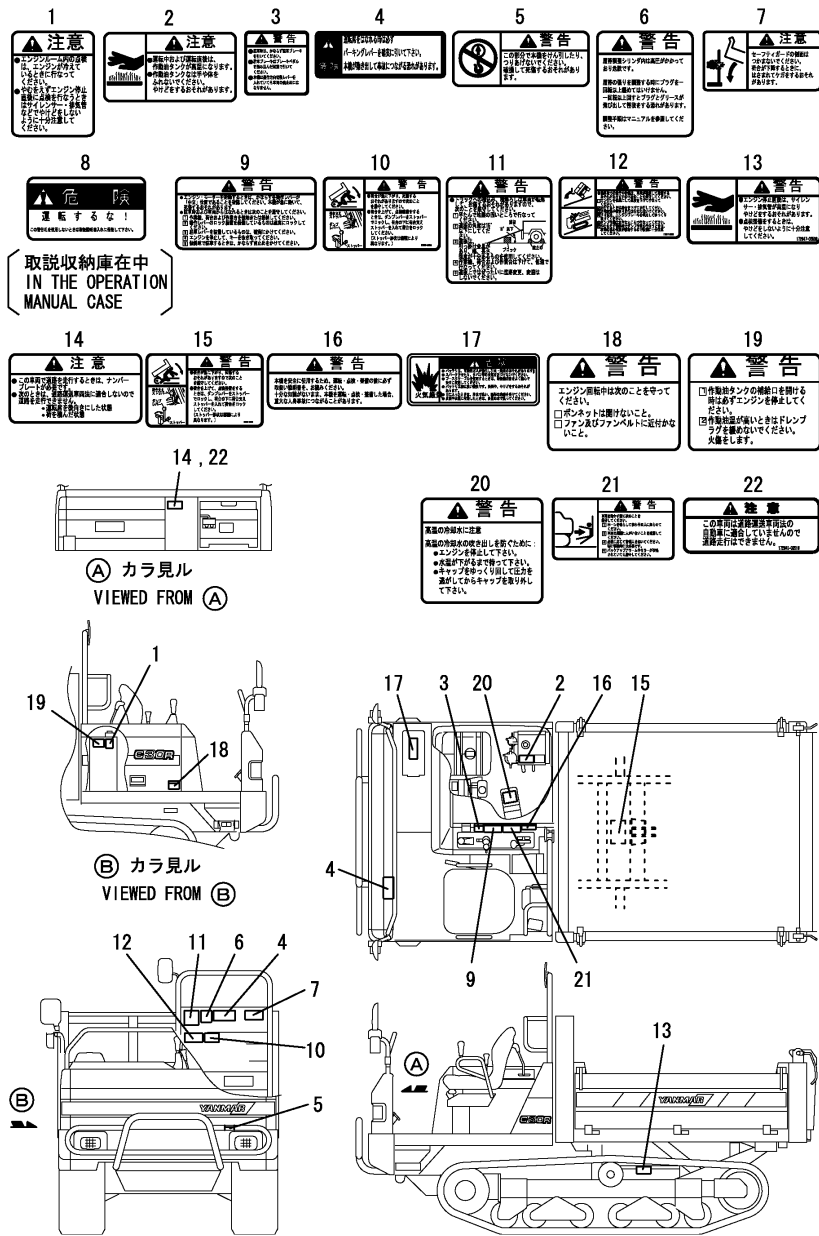
Fig.4. SAFETY LABEL(JP)
