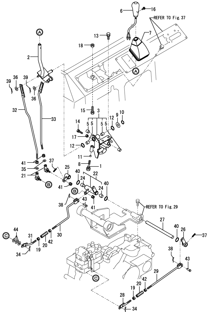
Fig.31. STEERING
