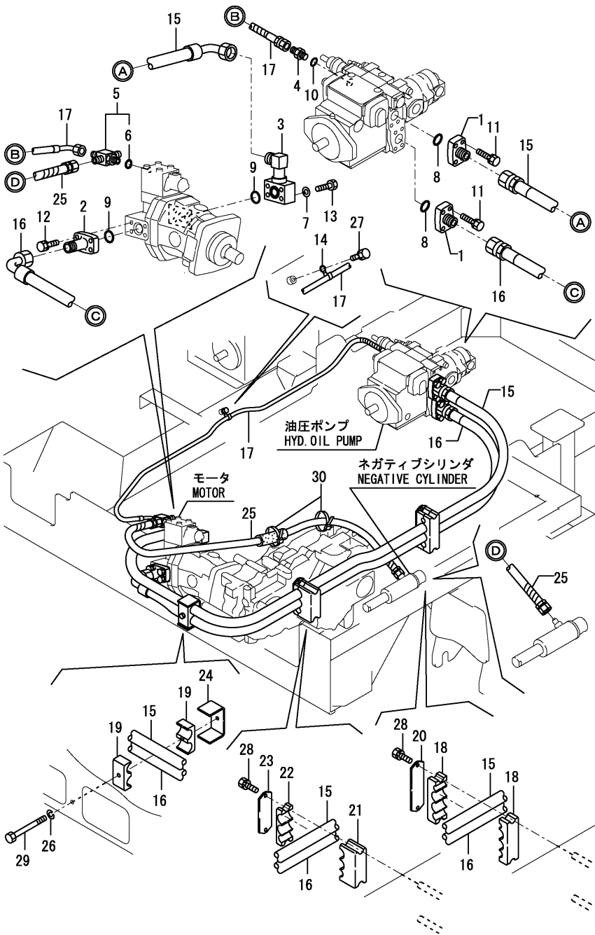
Fig.48. HYD.OIL PIPING(PUMP - TRAVEL MOTOR - NEGATIV CYLINDER)
