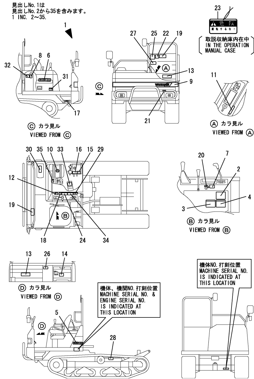
Fig.3. LABEL(W/O WAGON)(JP)
