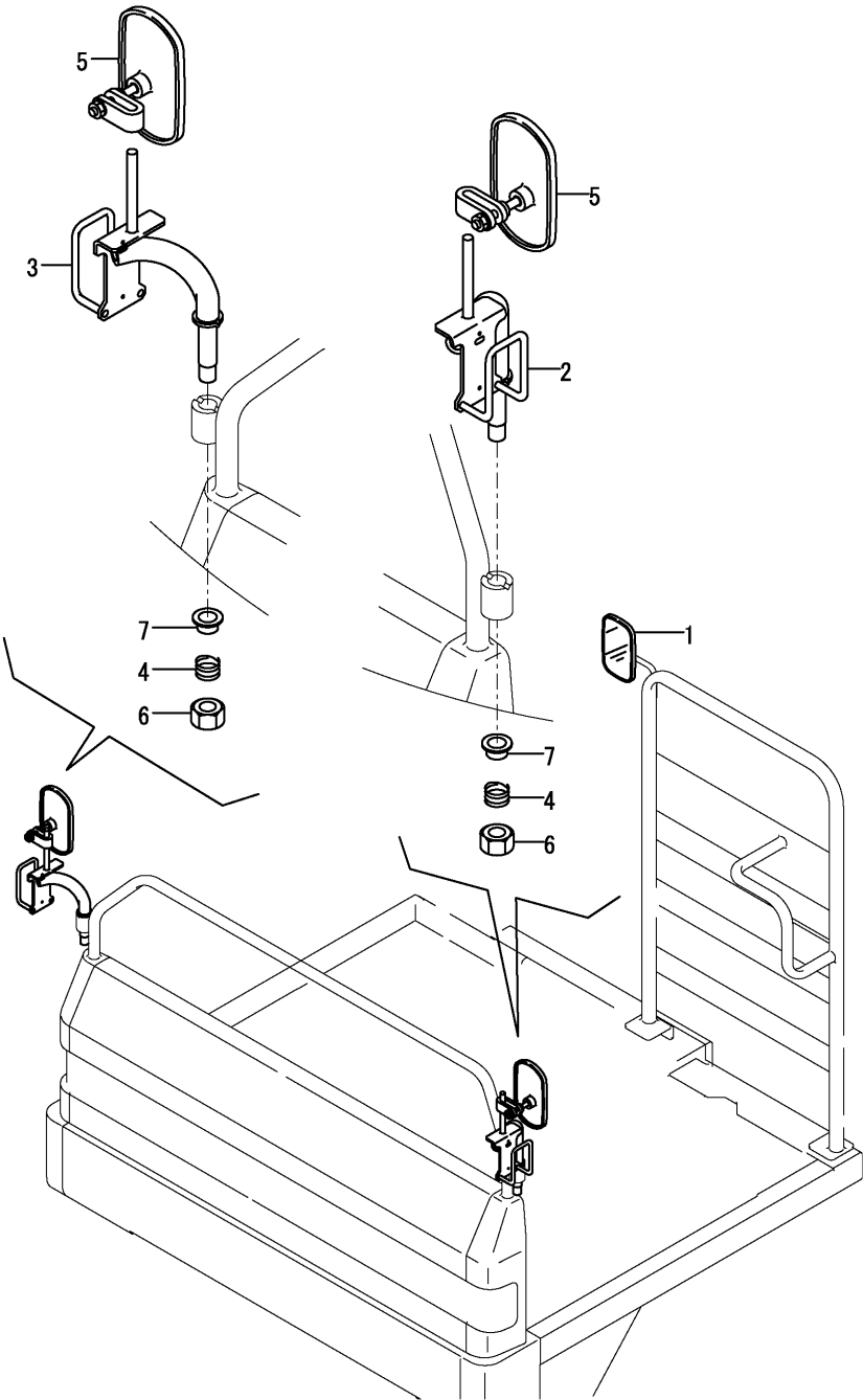
Fig.7. REARVIEW MIRROR
