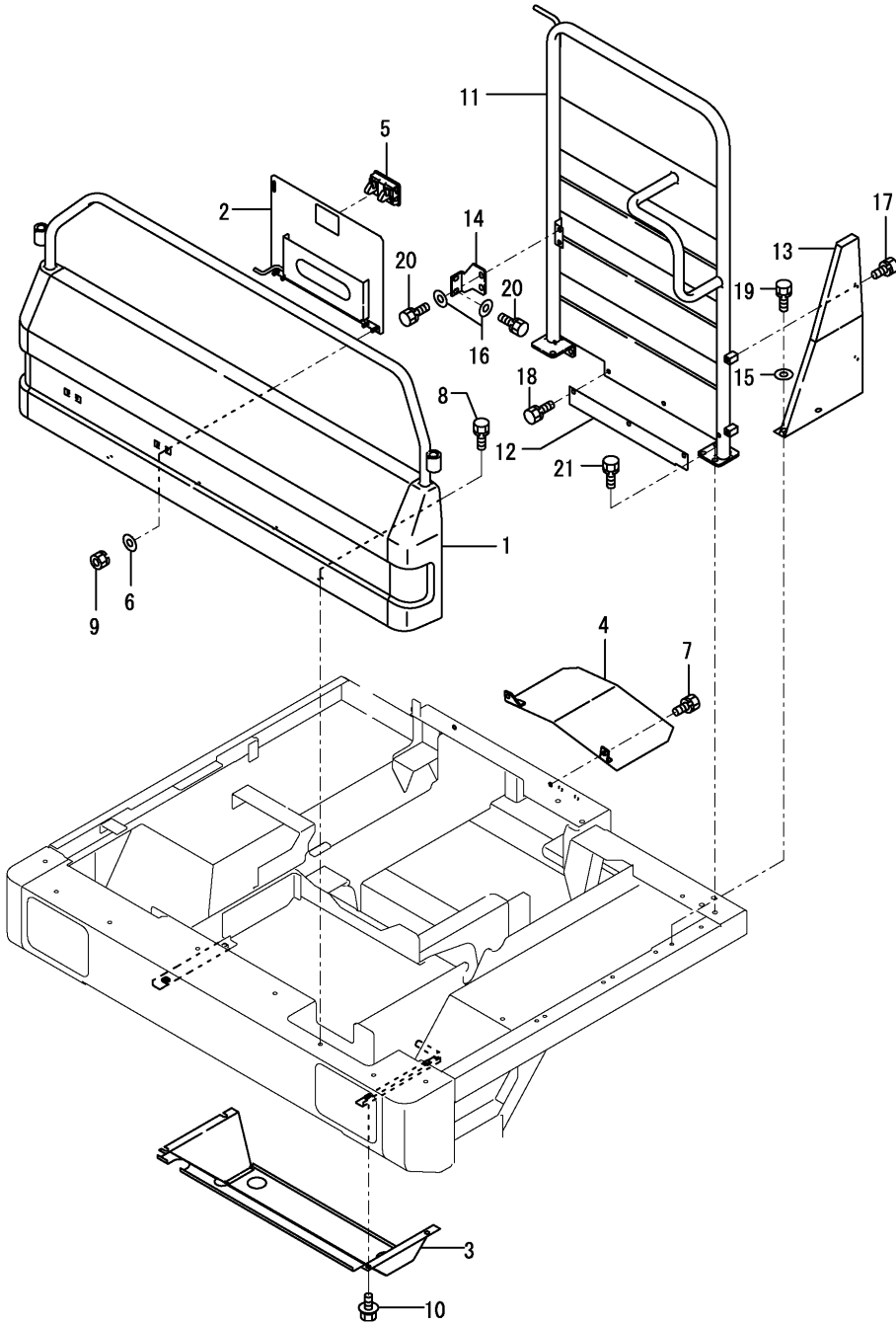
Fig.36. COVER & SAFETY GUARD
