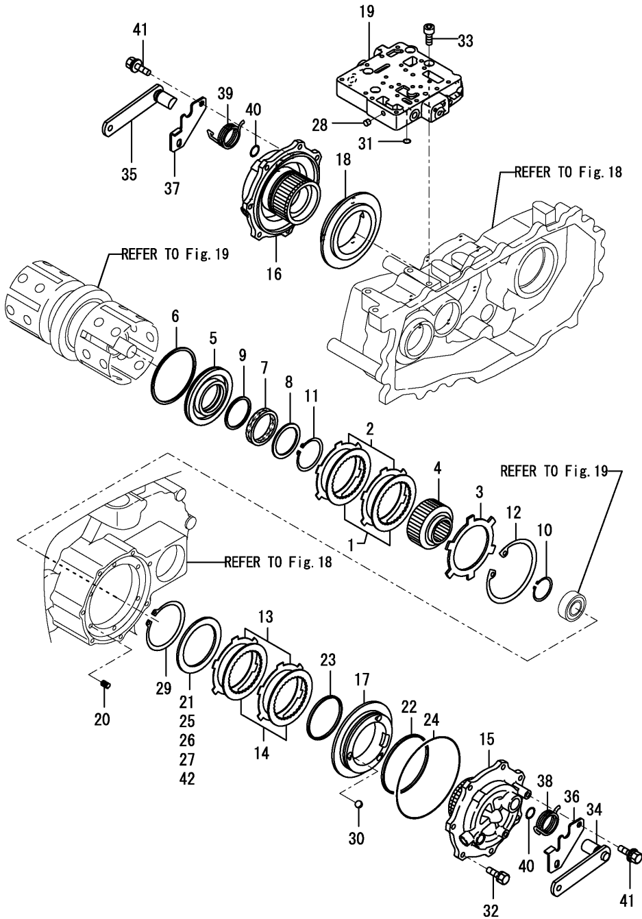
Fig.21. CLUTCH & BRAKE
