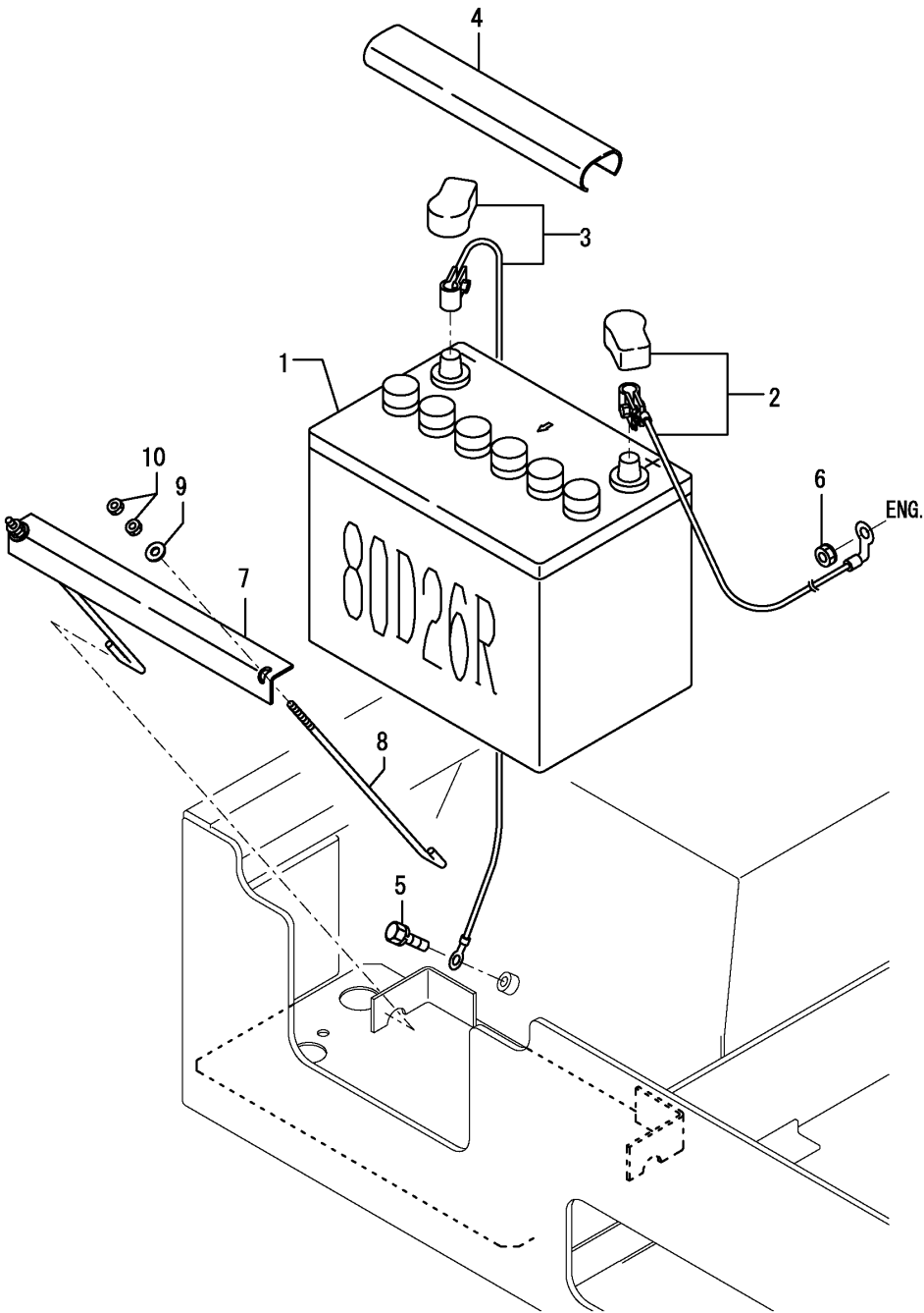
Fig.15. BATTERY
