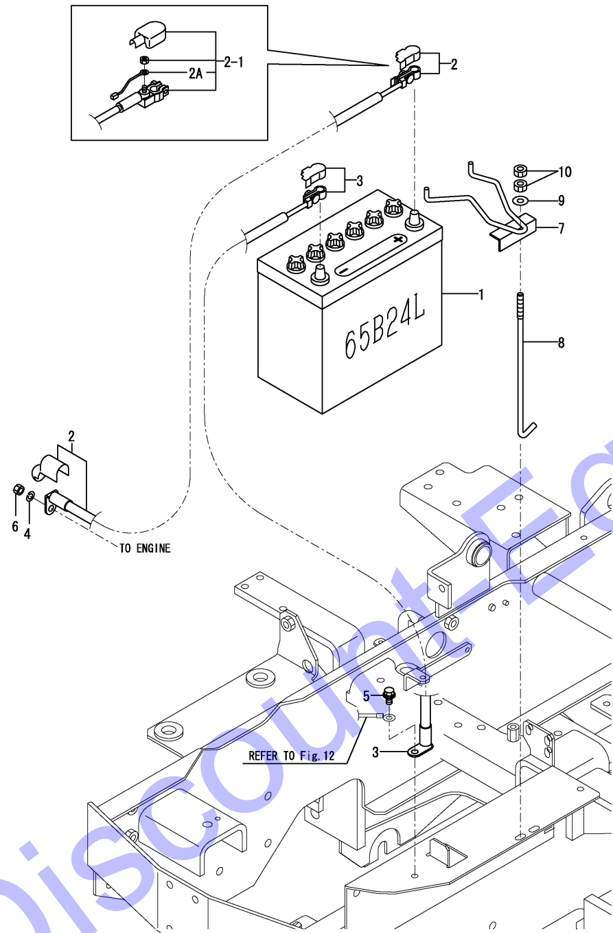
Fig.11. BATTERY & CABLE
