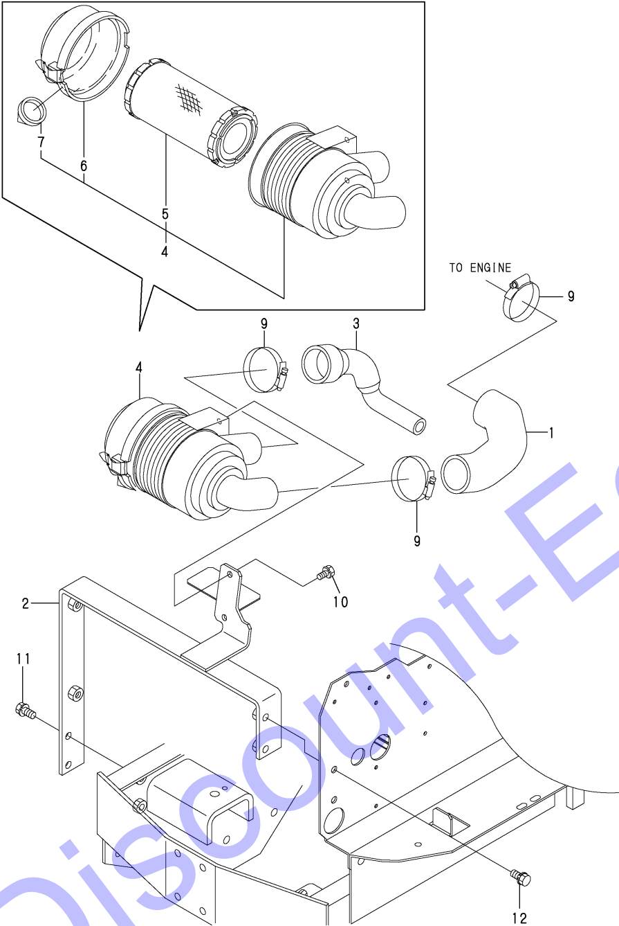
Fig.6. AIR CLEANER
