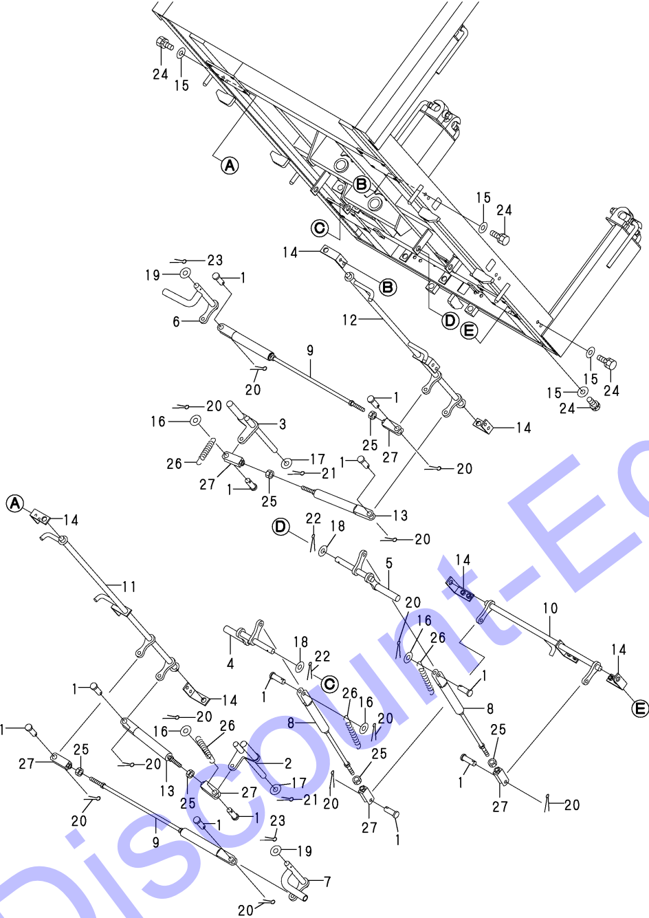
Fig.40. HOOK(3WD SPEC.)
