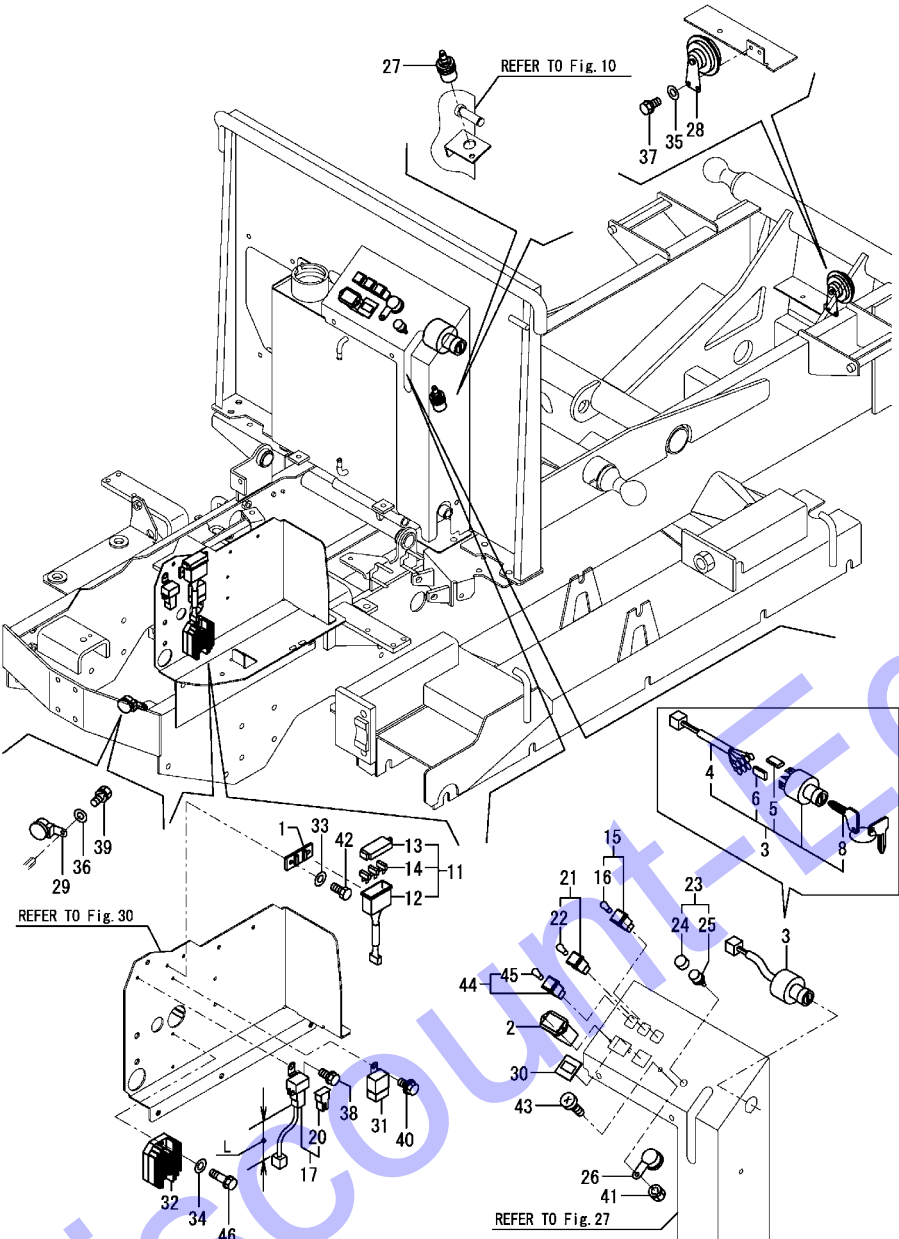
Fig.13. ELECTRIC PART(EQUIPMENT)
