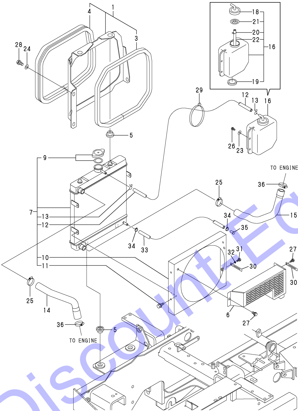
Fig.9. RADIATOR & MOUNT
