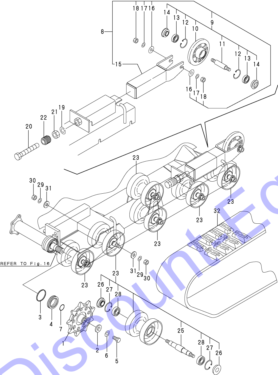
Fig.18. SPROCKET,ROLLER & CRAWLER
