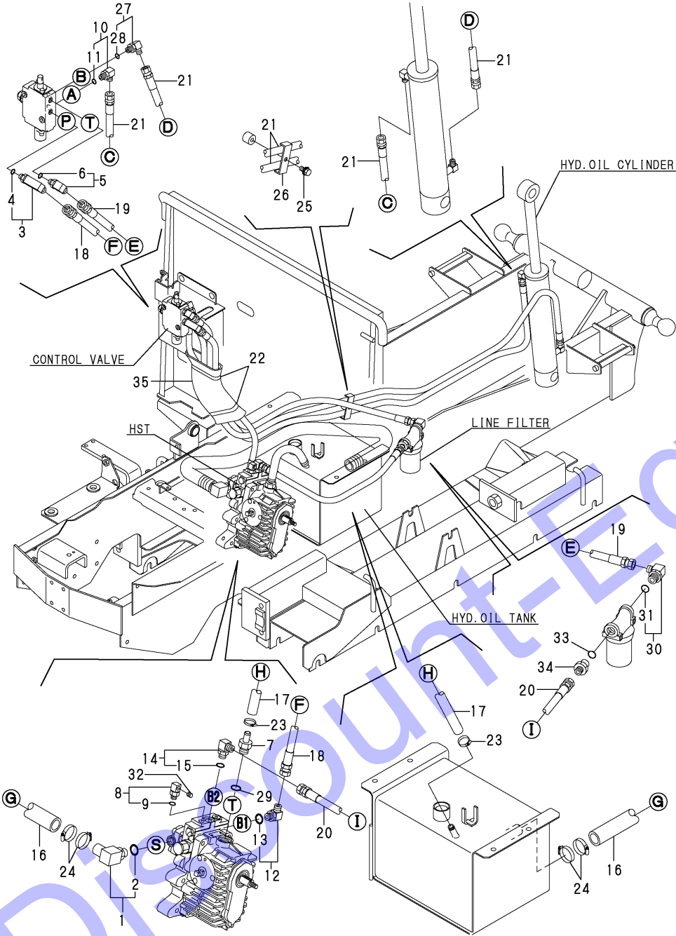
Fig.37. HYD.OIL PIPING
