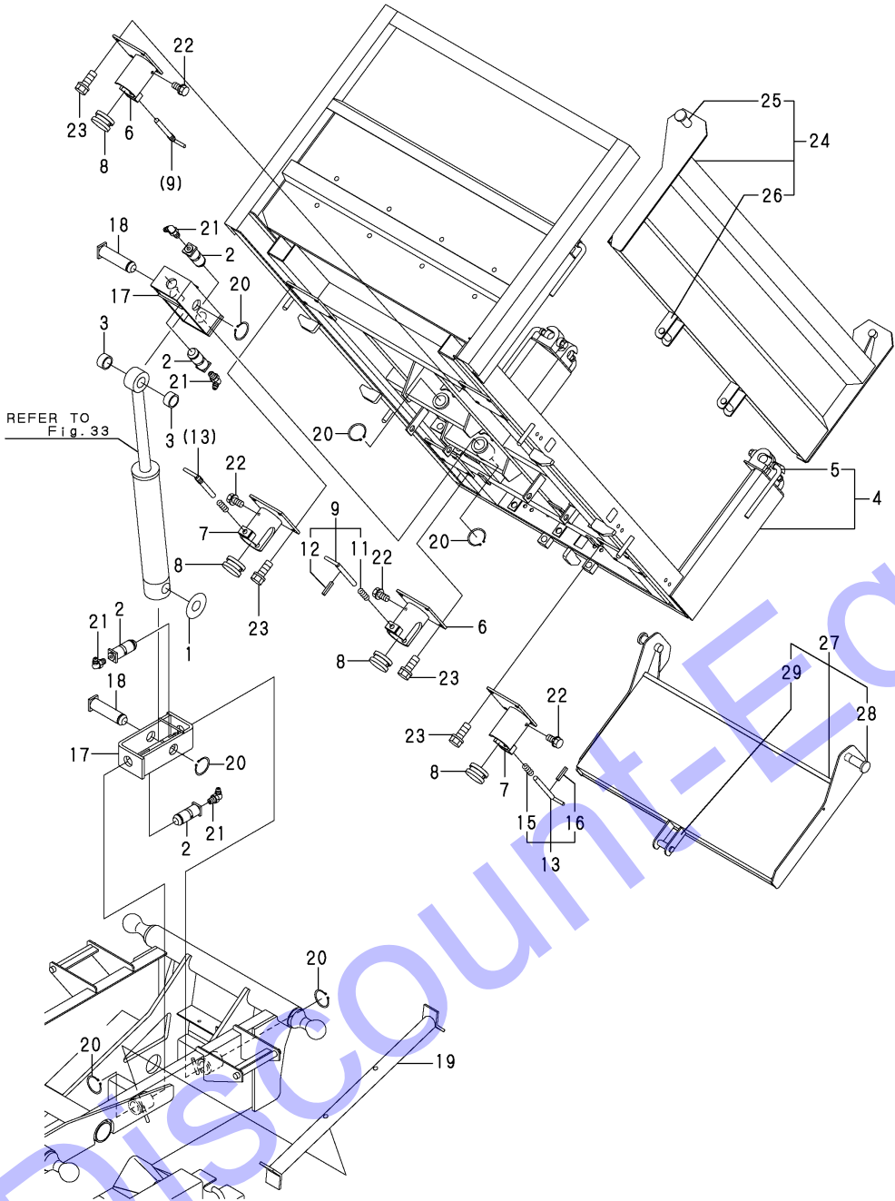
Fig.38. WAGON(3WD SPEC.)
