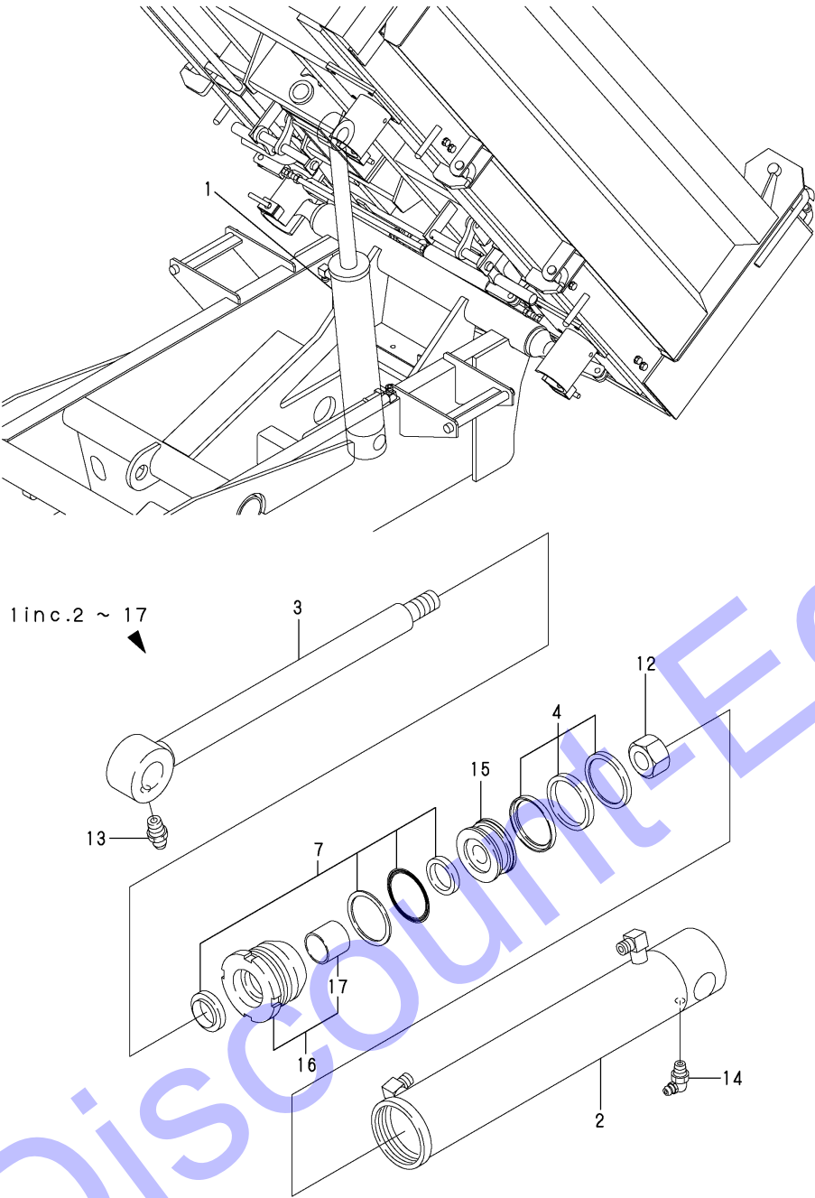
Fig.33. HYD.OIL CYLINDER
